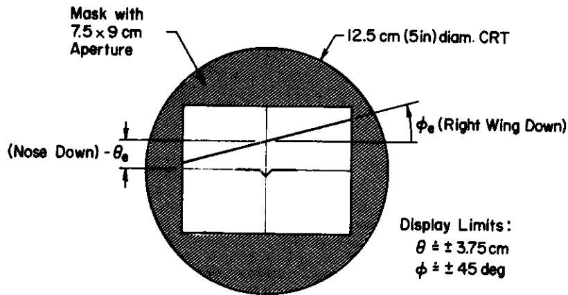
Figure 10. CRT Display for Single-Loop Plus Secondary Tasks
