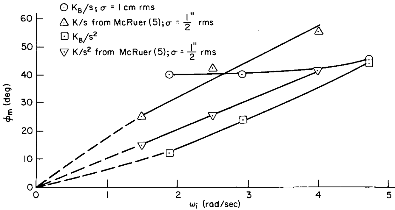
Figure 18. Variation of Phase Margin with Input Bandwidth
