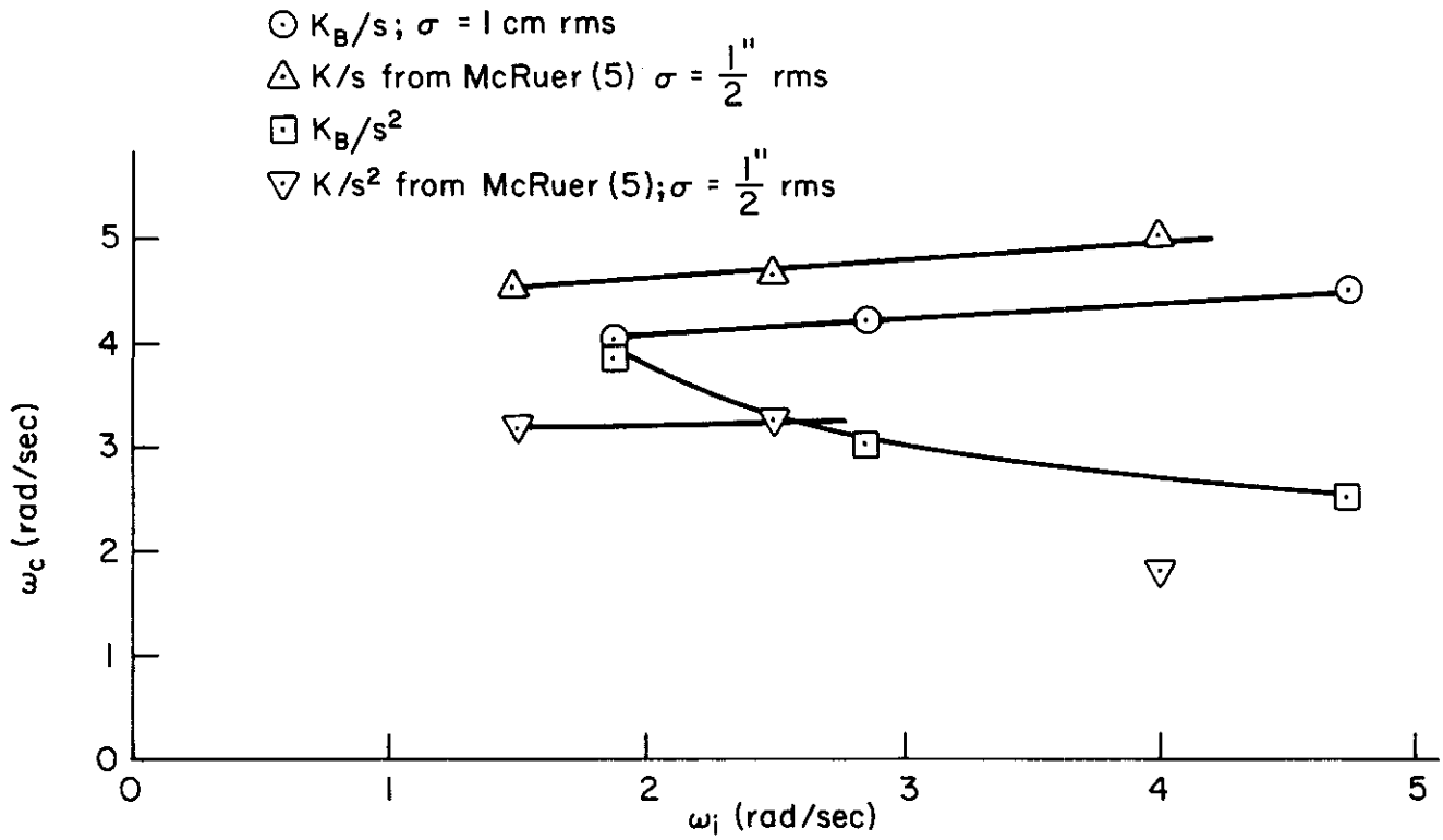
Figure 17. Variation of Crossover Frequency with Input Bandwidth
