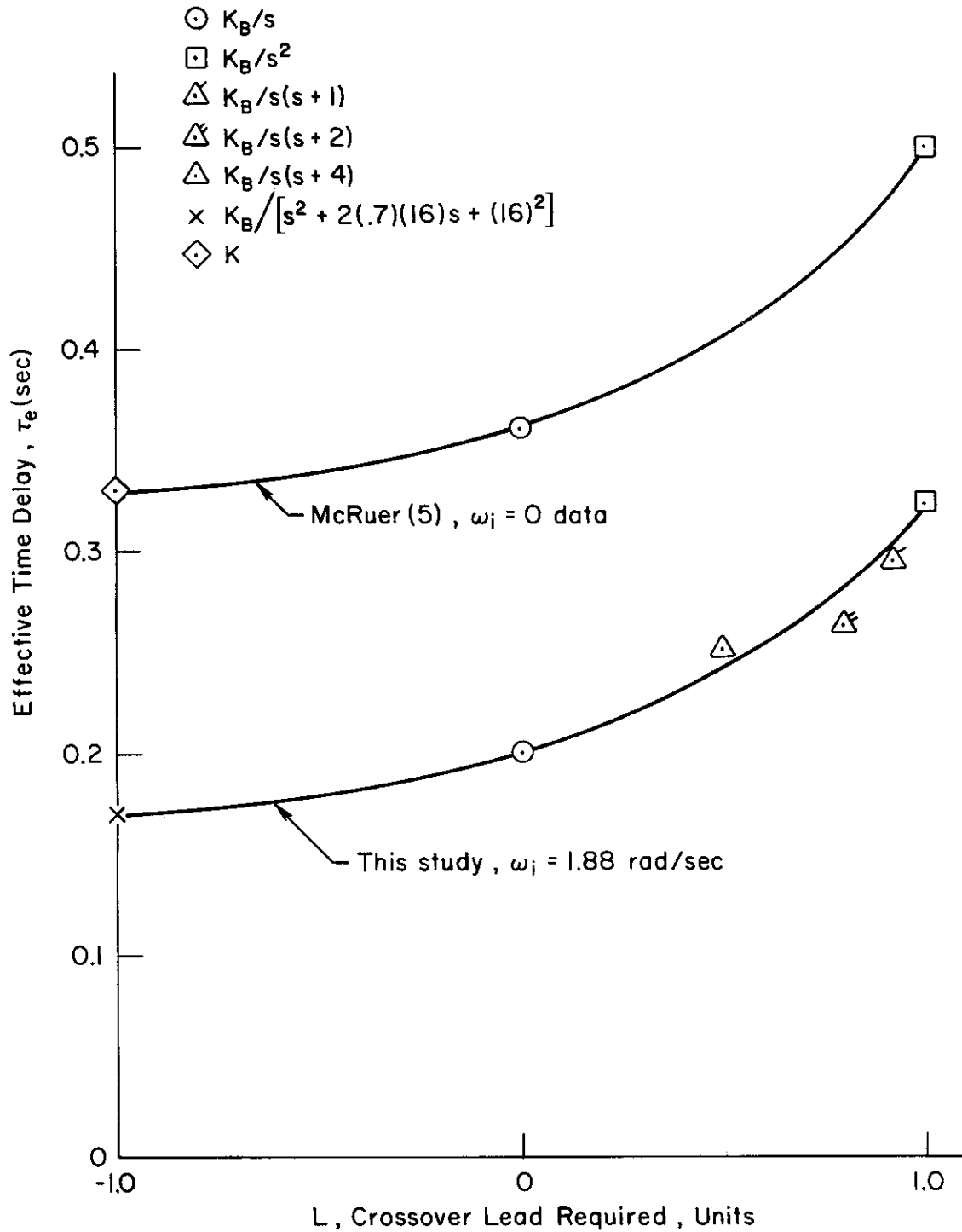
Figure 19. Variation of Effective Time Delay with Slope of Pilot Equalization
