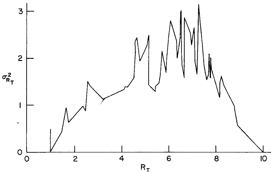
b) Variance of Transformed Scores (Matrix = 64 x 63)
