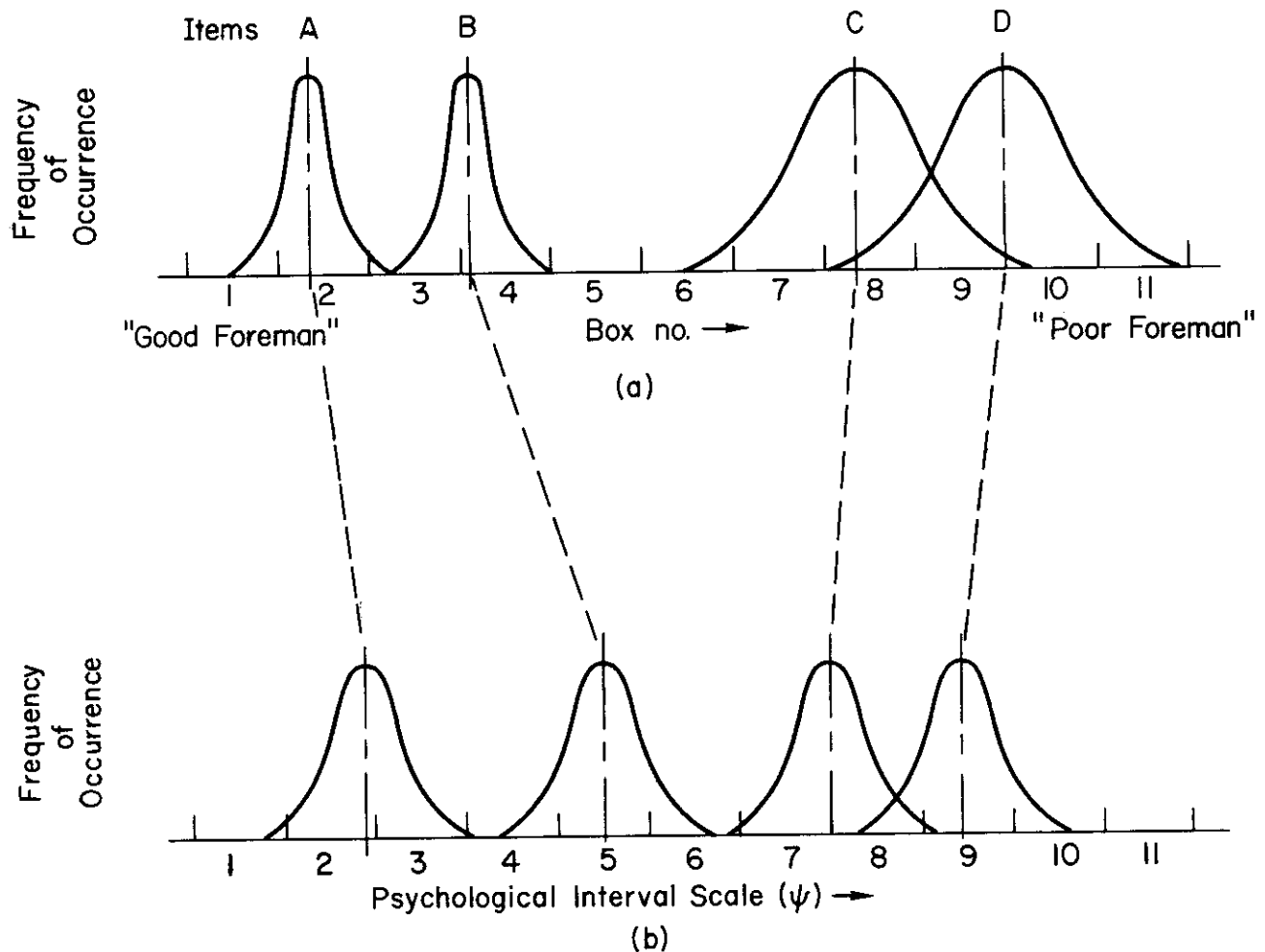
Figure 2. Hypothetical Results of Uhrbrock's (9) Rating Scale Results
