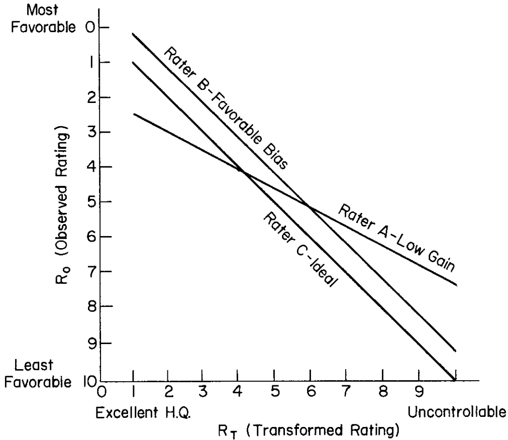
Figure 4. Possible Effects of a Linear Transformation on the Observed Scores
