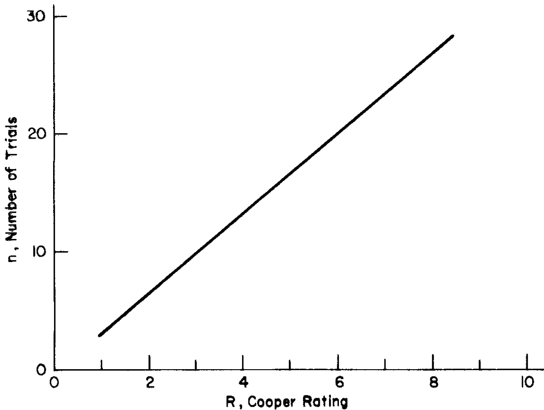
Figure 9. Minimum Number of Trials Required in Each of Two Independent Samples to Determine that the Sample Means are Different by One Cooper Unit with 95 Percent Confidence
