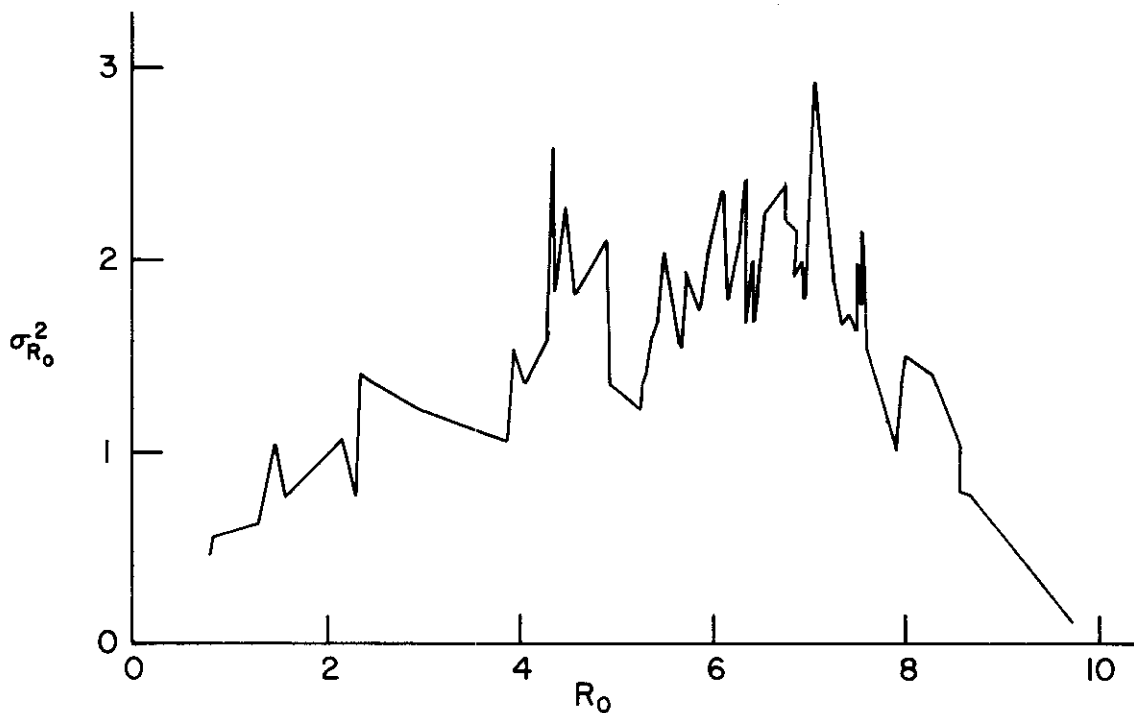
a) Variance of Observed Scores
