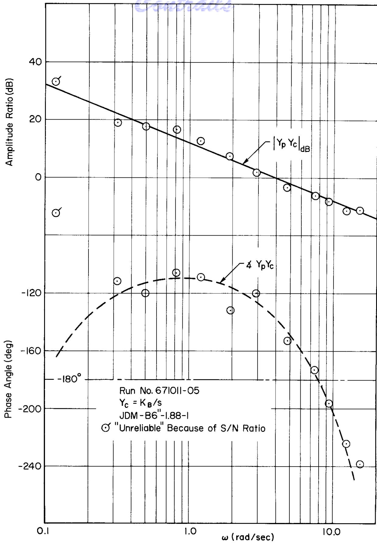
Figure 15. Total Open-Loop Describing Function Computed for Y_c = K/s
