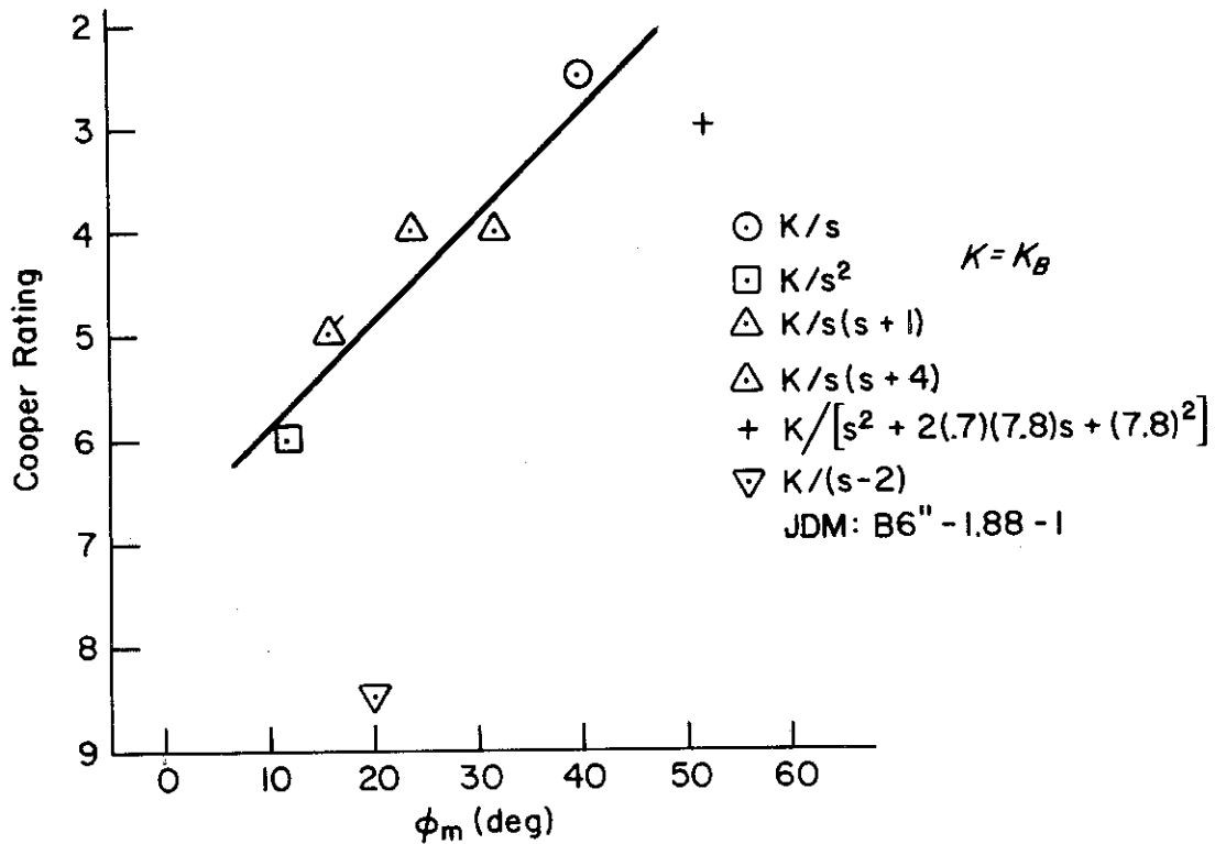
Figure 24. Variation of Cooper Rating with Phase Margin
