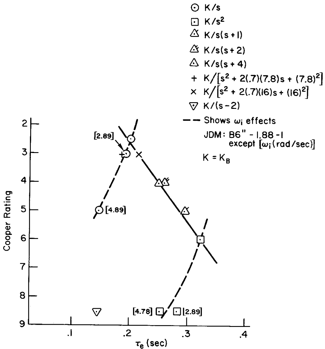
Figure 21. Variation of Pilot Rating with Effective Time Delay
