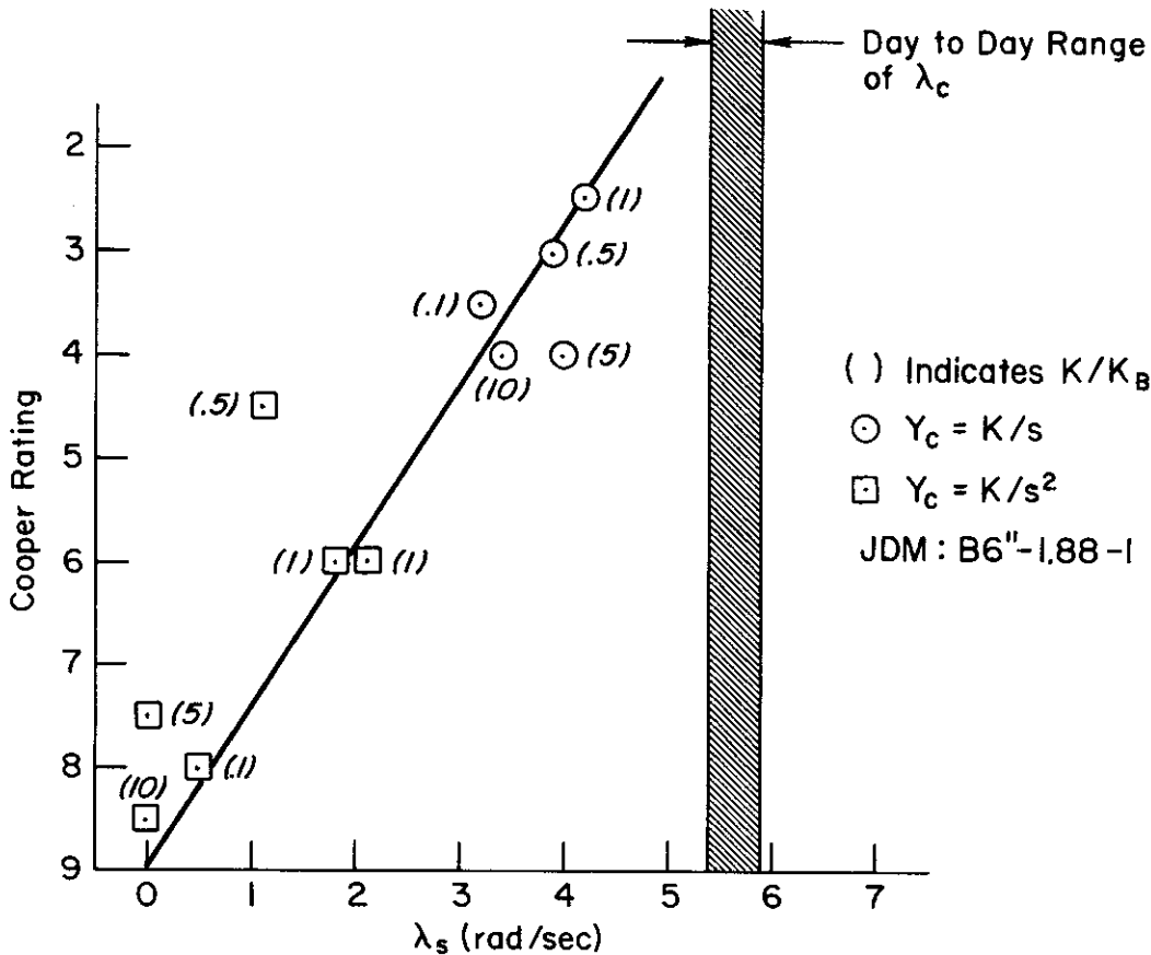
Figure 34. Variation of Secondary Task Score with Controlled Element Gain
