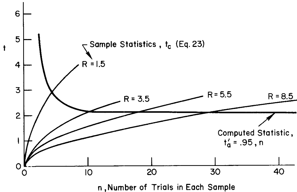
Figure 8. Trial Size Determination from the t-Test
