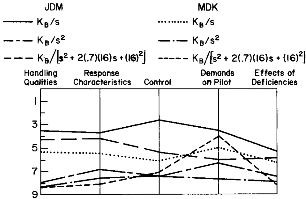
Figure 45. Controlled Element Form Effects on Trait Ratings
