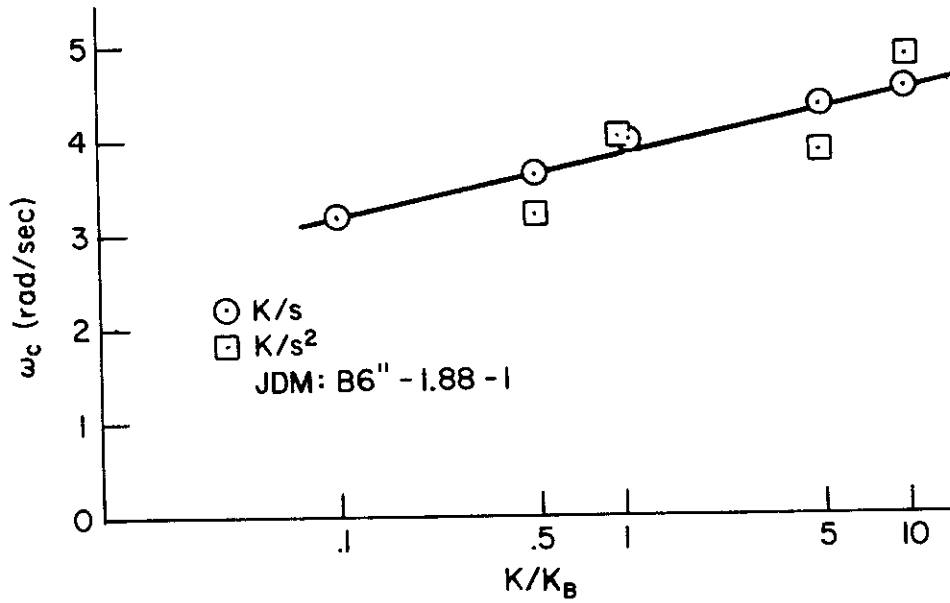
Figure 23. Variation of Crossover Frequency with Gain
