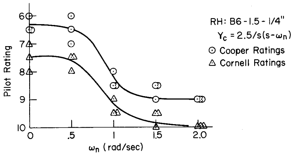
Figure 39. A Comparison of Cooper and Cornell Ratings for an Unstable Second-Order Controlled Element
