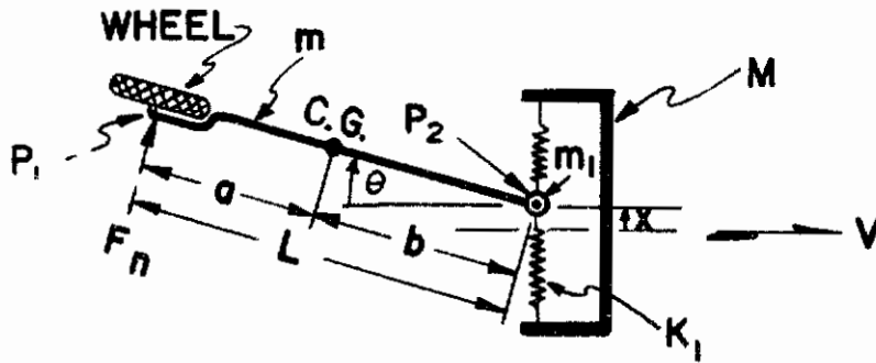
SCHEMATIC OF NOSE WHEEL ASSEMBLY FOR THIRD ORDER SYSTEM
