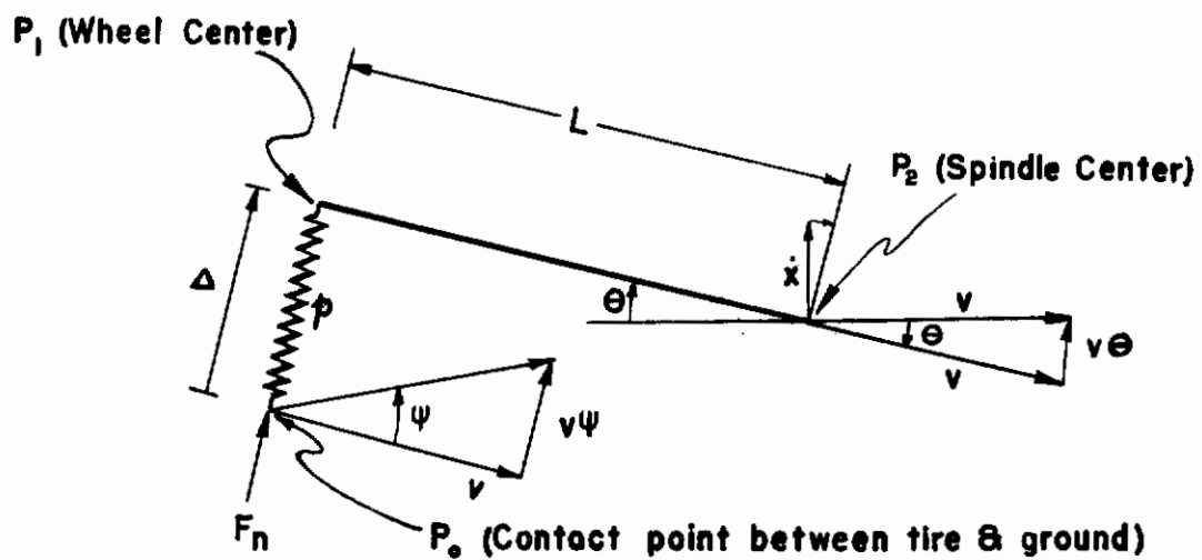
DIAGRAM OF TIRE CHARACTERISTICS
