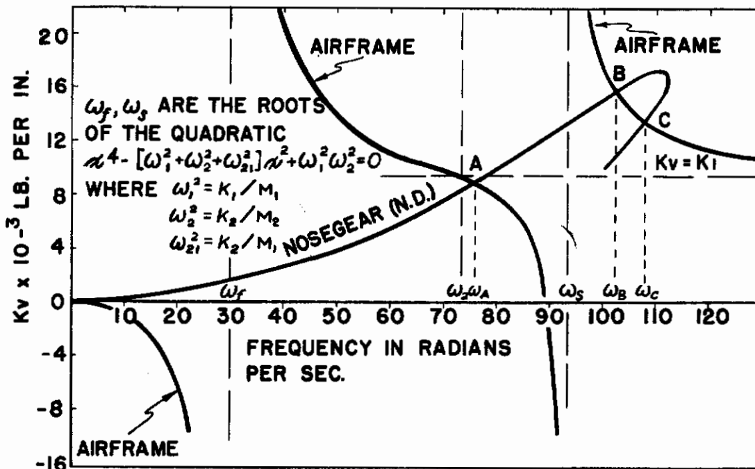
EFFECT OF AIRFRAME ELASTICITY ON NOSEGEAR STABILITY FOR MULTIPLE - MODE SYSTEM
