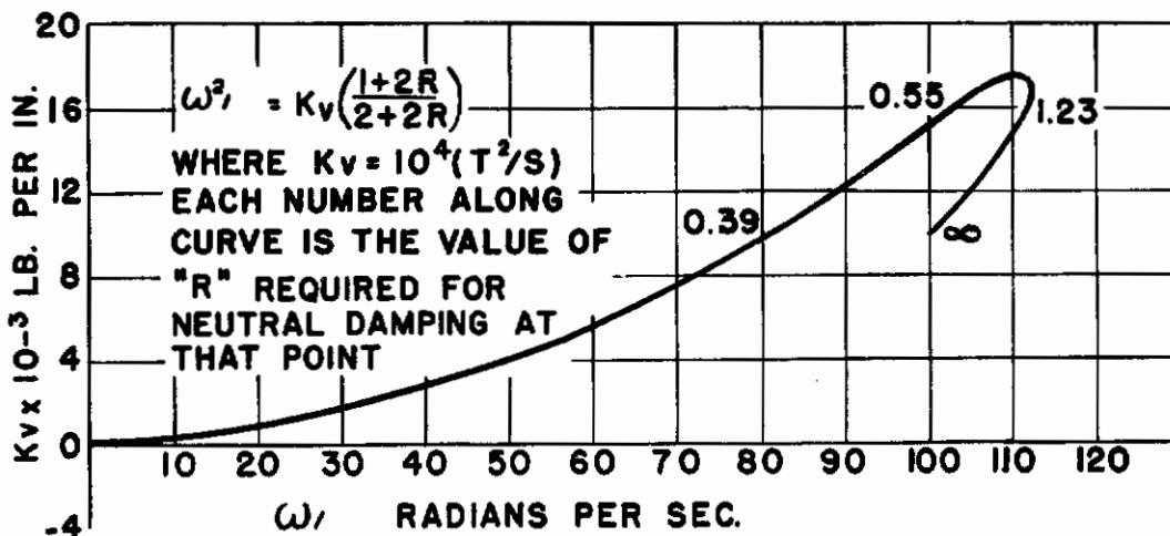
NOSEGEAR ELASTICITY vs FREQUENCY FIGURE 10
