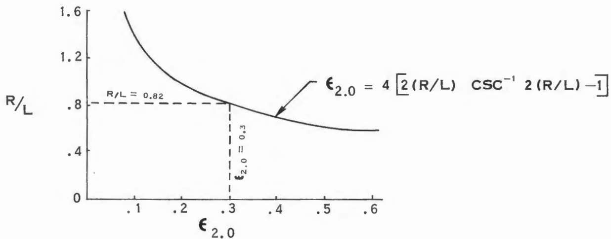
FINDING THE R/L VALUE FIG. IV A-6
