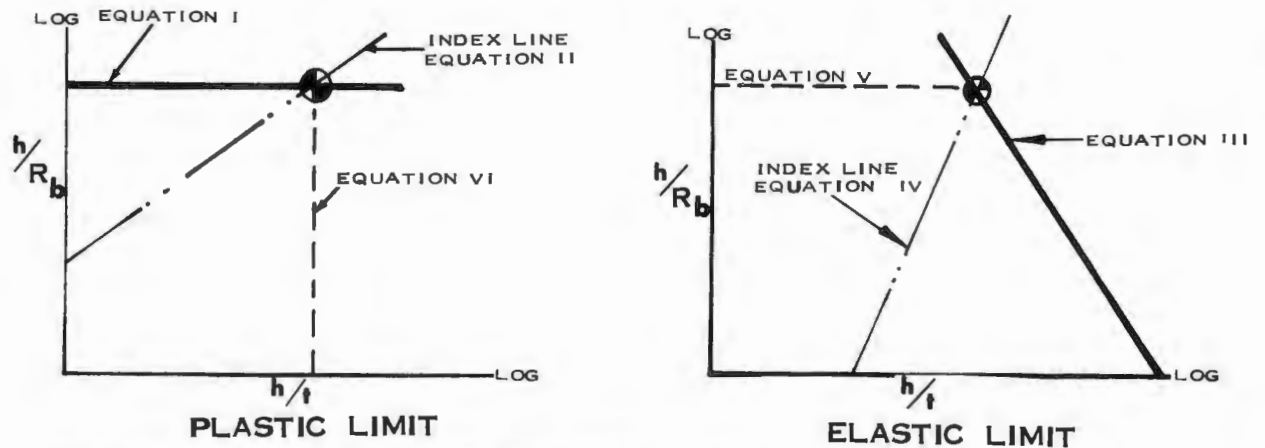
FIGURE VB-5 PLASTIC AND ELASTIC LIMITS
