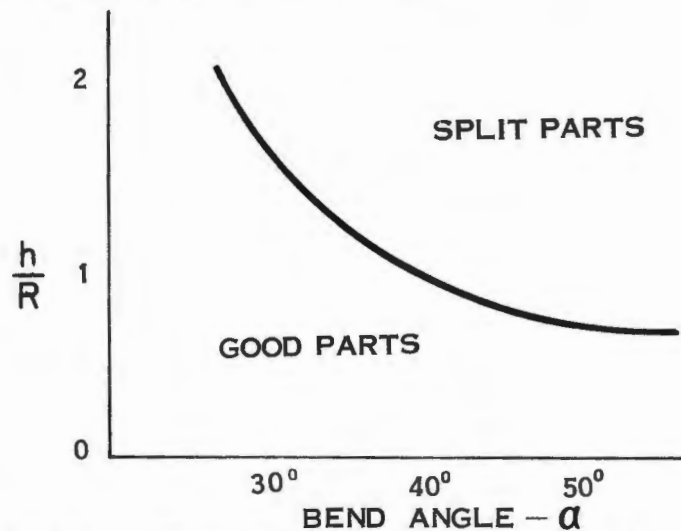
FIGURE II A-7 FORMABILITY CURVE FOR 2024-T3 ALUMINUM
