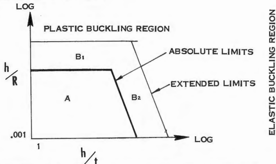
FIGURE II B-9 ABSOLUTE AND EXTENDED RUBBER SHRINK FORMABILITY LIMITS
