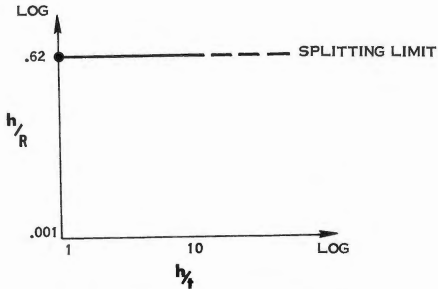
FIGURE II B-3 GRAPH CONSTRUCTION
