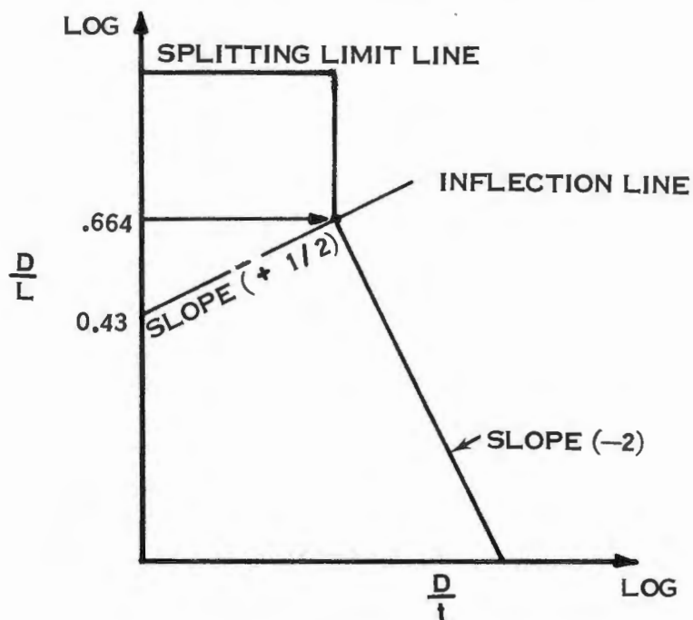
FIGURE IB-5 GRAPH CONSTRUCTION.
