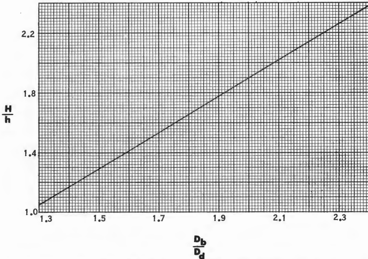
FIGURE VB-8 CURVE FOR CONVERTING FROM OVERHANG ( h ) TO FINAL CUP HEIGHT ( H )
