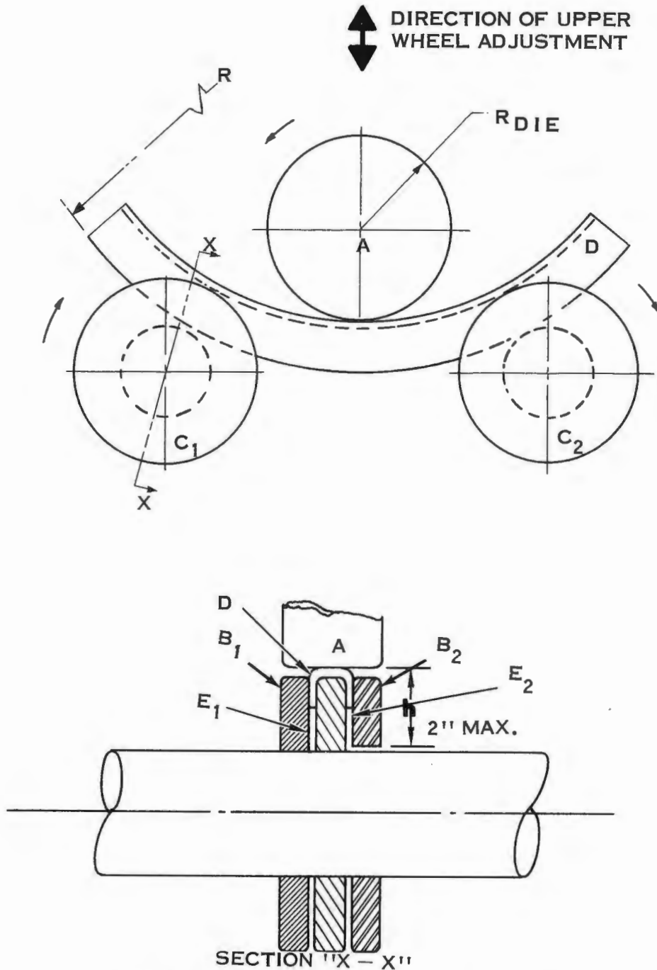
SECTION "X - X" LINEAR ROLL HEEL-IN MACHINE SET-UP FIGURE III B-2
