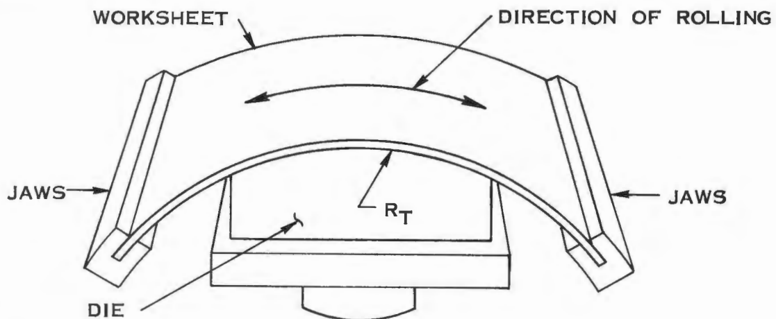
SET-UP CONSIDERING THE DIRECTION OF ROLL OF THE MATERIAL FIGURE IVA-3
