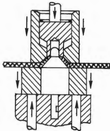
FIGURE II A-4 CROSS SECTION OF RAM COIN DIMPLING
