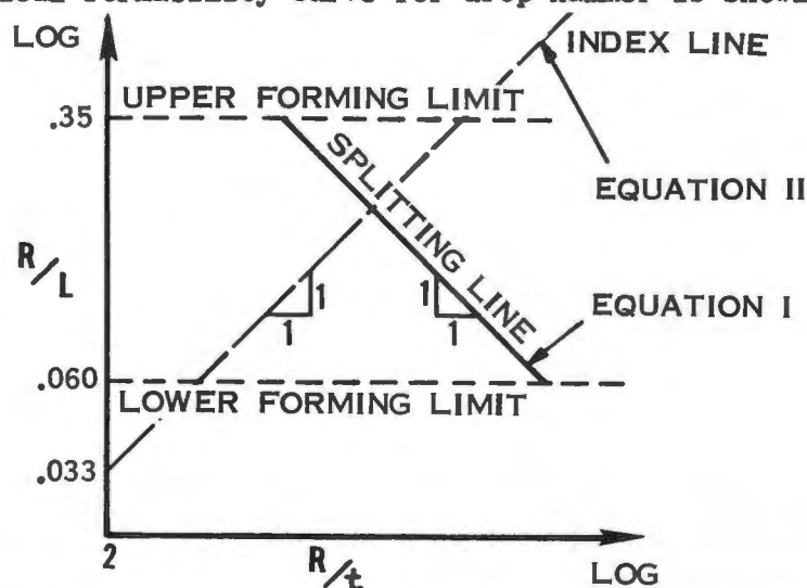
FIGURE VI B-7 TYPICAL DROP HAMMER FORMABILITY CURVE.
