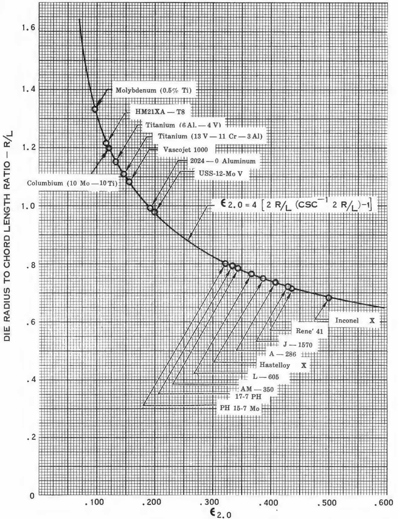
SHEET STRETCH CORRELATION GRAPH
