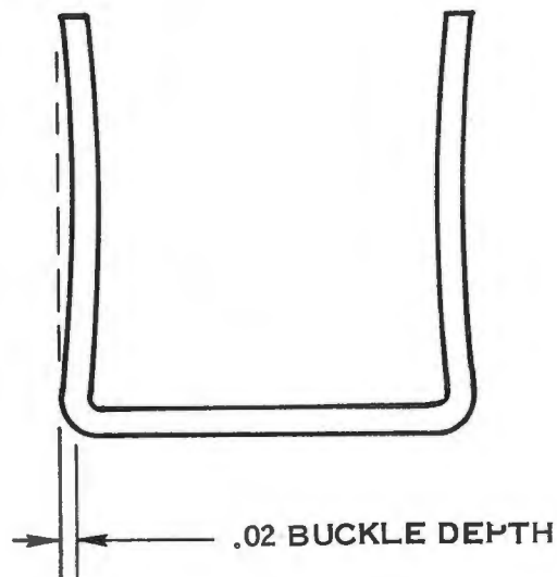
FIGURE III B-9 HEEL-IN CHANNEL DISTORTION
