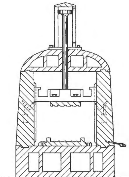
FIGURE VI B-1 DROP HAMMER SET-UP.
