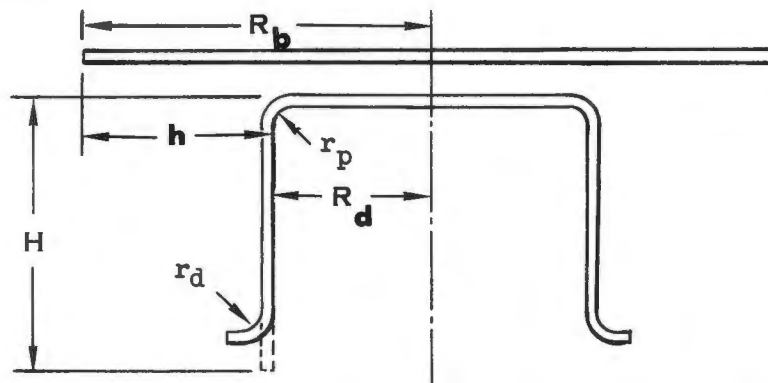
FIGURE V A-3 GEOMETRICAL VARIABLES FOR CUPPING
