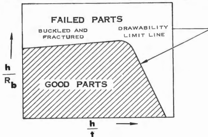
FIGURE V A-4 TYPICAL THEORETICAL FORMABILITY CURVE FOR THIN WALLED CYLINDRICAL CUPS
