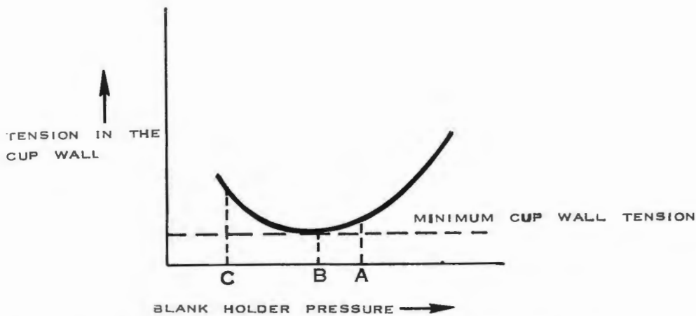
FIGURE VA-II CUP WALL TENSION VS. BLANK HOLDER PRESSURE
