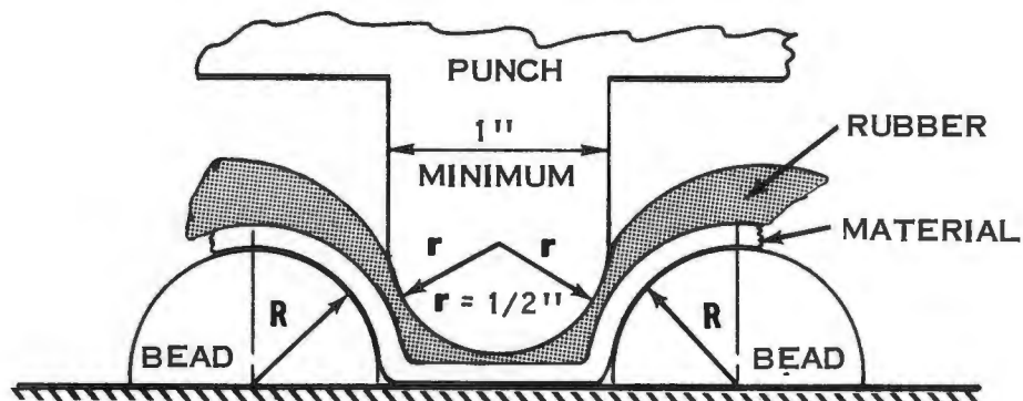
FIGURE VI B-13 SCHEMATIC OF A PUNCH AND BEAD.
