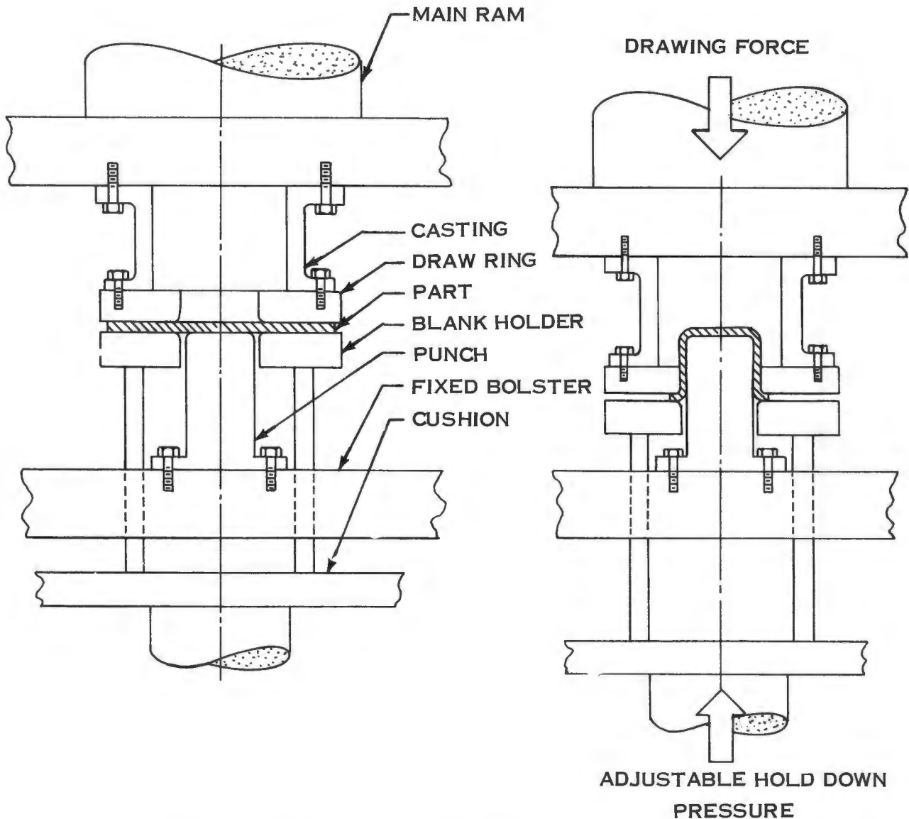
FIGURE V A-1 DOUBLE ACTION DRAW DIE
