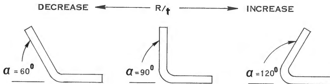
EFFECT OF PART ANGLE ON R/t VALUE FIG. 1 A-4
