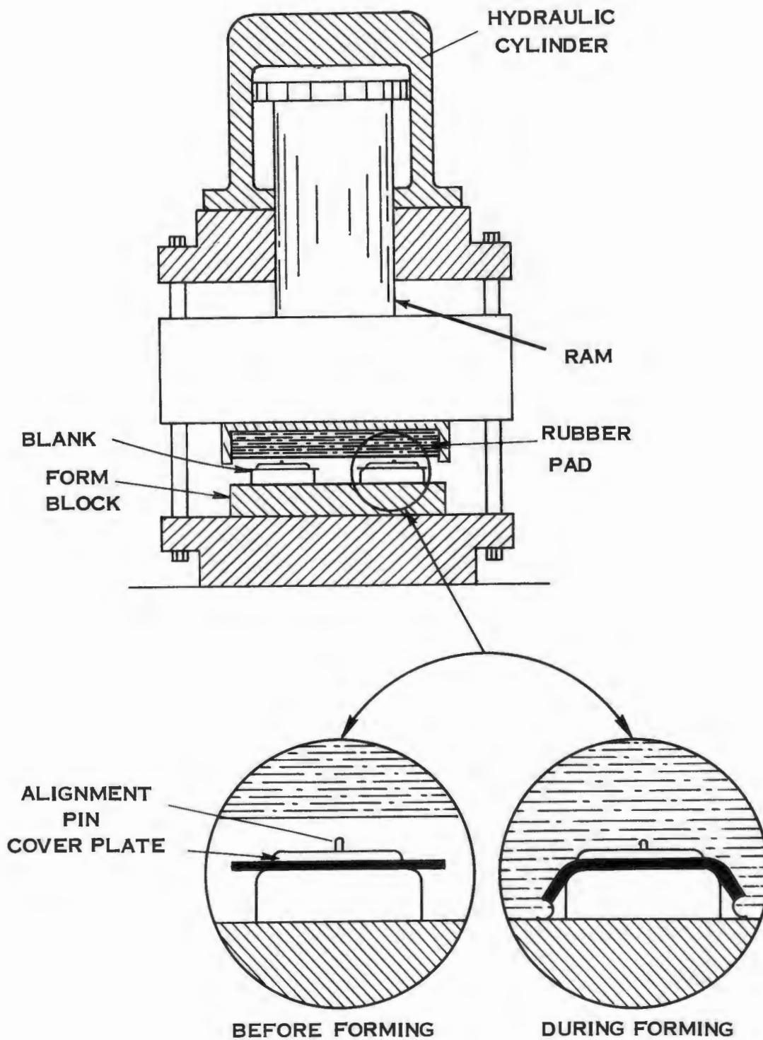
THE GUERIN RUBBER PROCESS 1925 PSI LAKE ERIE RUBBER PRESS FIGURE II B-1
