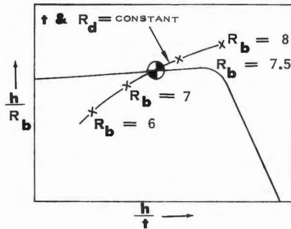
FIGURE V A-5 TYPICAL FORMABILITY CURVE SHOWING A CONSTANT R_d/t LINE
