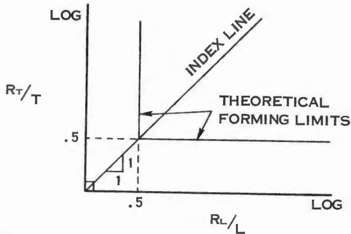
PLOTTING INDEX AND THEORETICAL LIMITS FIG. IV A-7
