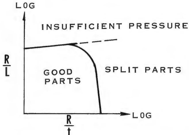
FIGURE VI A-5 TYPICAL FORMABILITY CURVE
