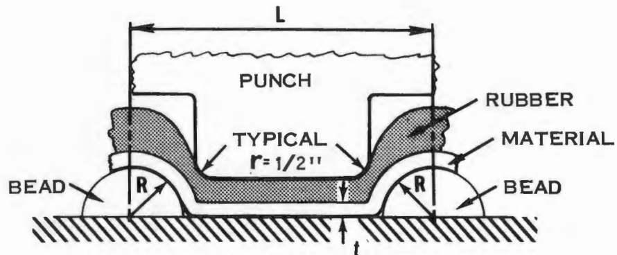
FIGURE VI B-4 GEOMETRICAL PARAMETERS.
