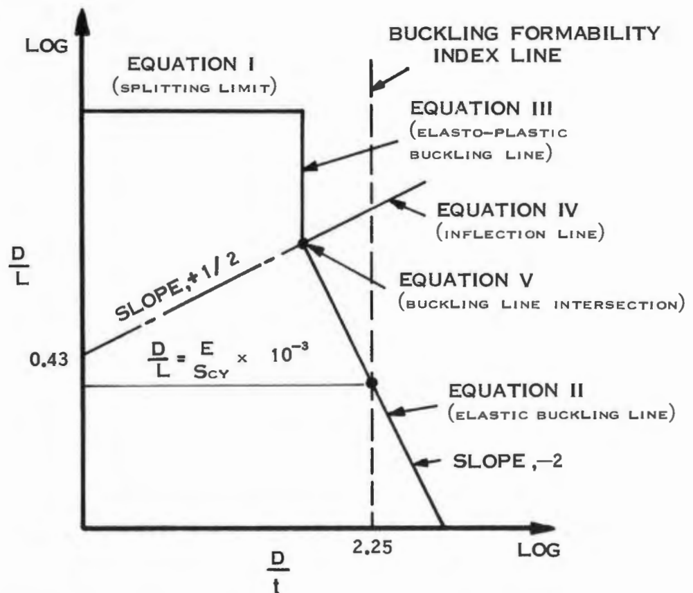
FIGURE IB-3 TYPICAL JOGGLING FORMABILITY CURVE.
