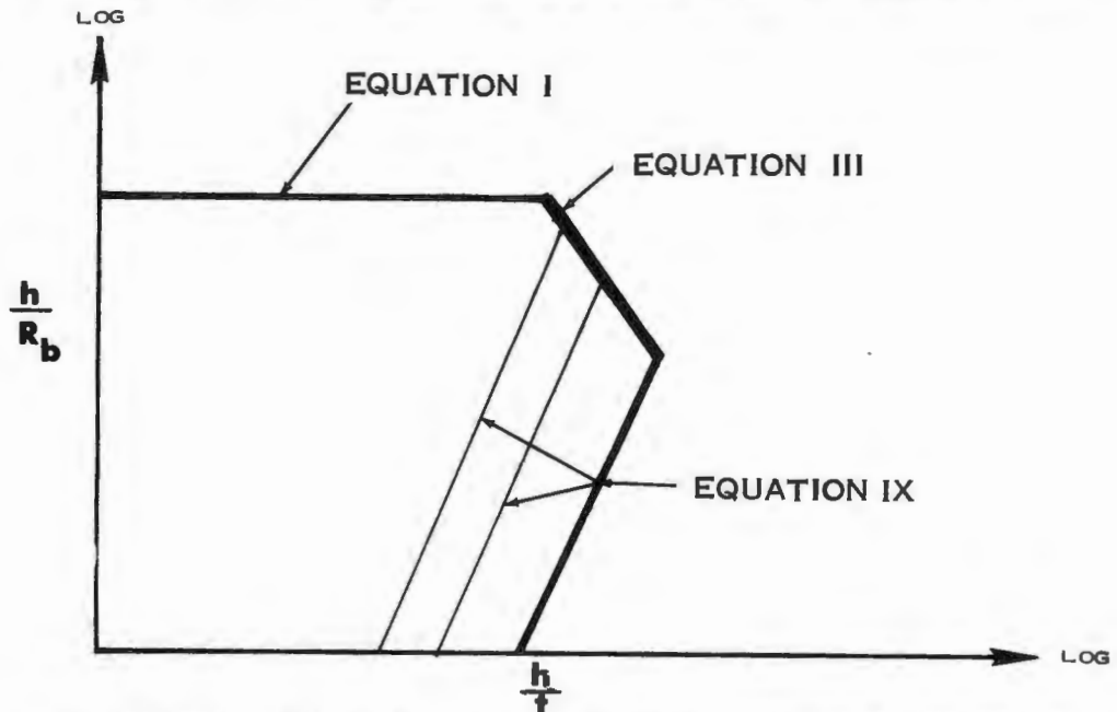
FIGURE VB-7 PREDICTABILITY EQUATION FOR SPINNING IN GRAPH FORM
