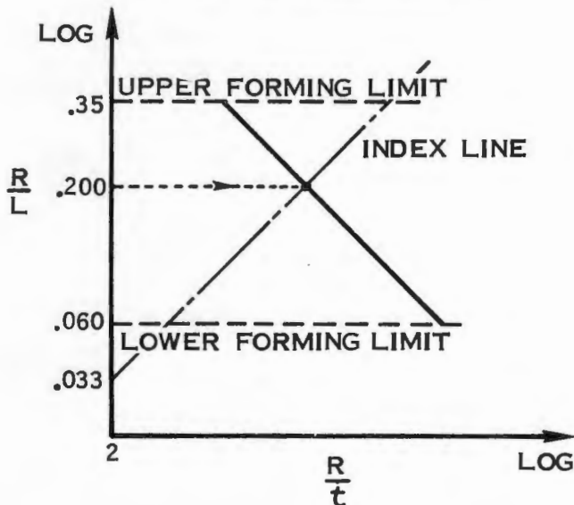
FIGURE VI B-10 GRAPH CONSTRUCTION.
