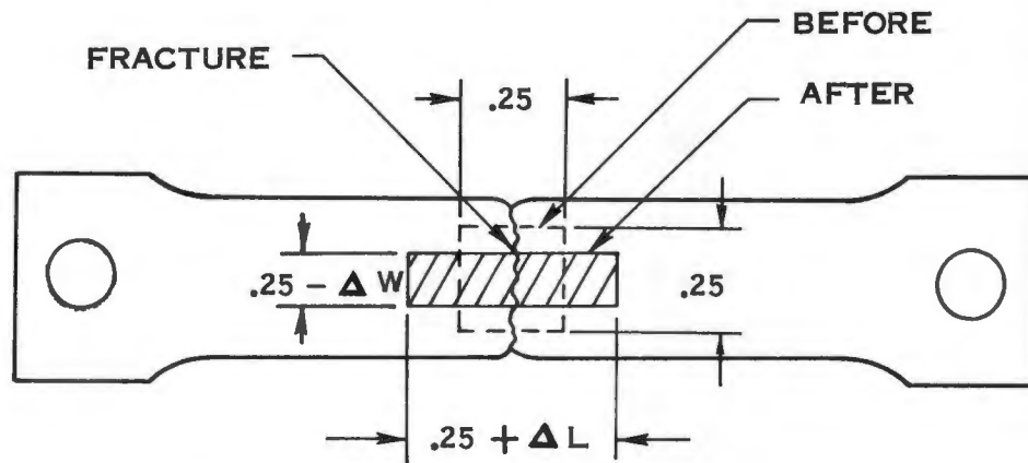
TYPICAL GRIDDED TENSION SPECIMEN FIG. I A-6
