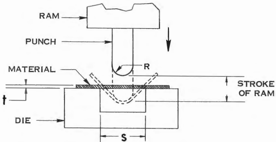
TYPICAL BRAKE FORMING SETUP FIG. I A-1
