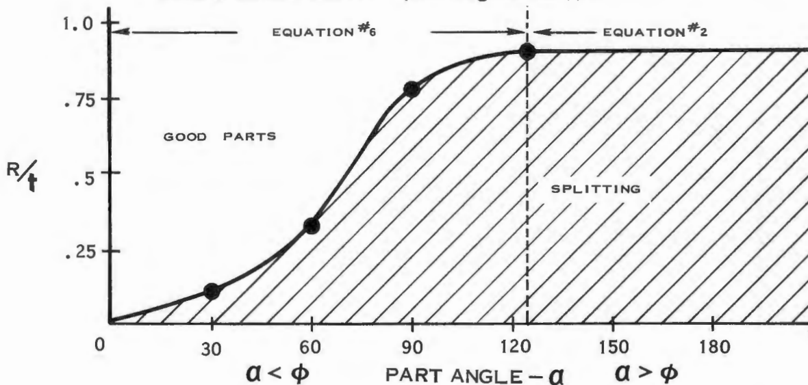
SPLITTING LIMIT CURVE FOR BRAKE FORMING FIG. IA-7
