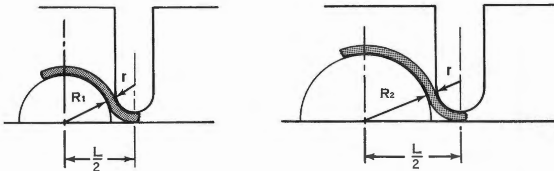
FIGURE VI B-5 RELATIONSHIP OF BEAD SPACING.
