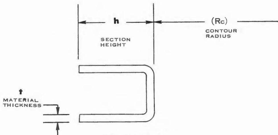
FIGURE IIIA-19 HEEL-IN CHANNEL
