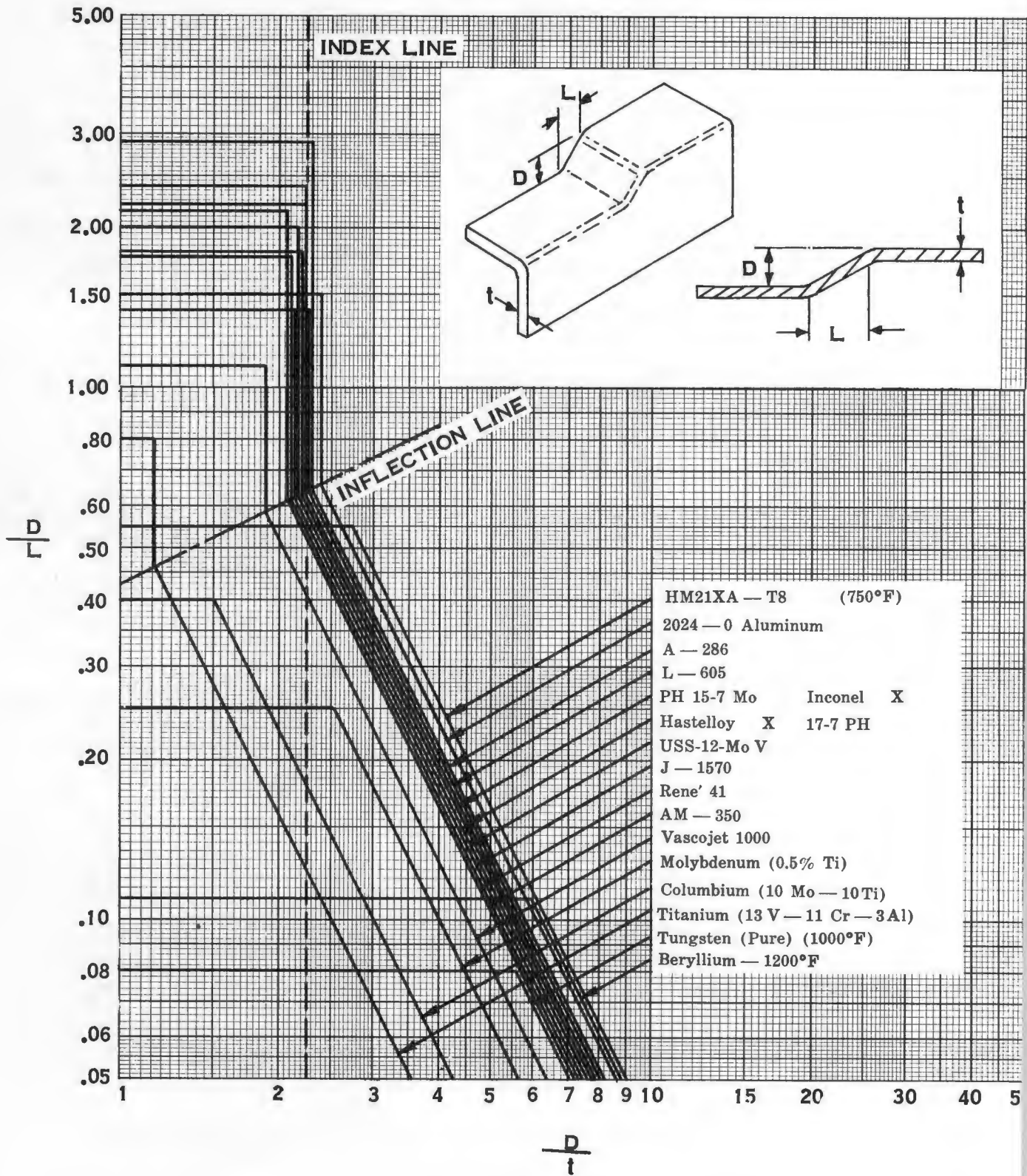
GRAPH I B-1 COMPOSITE GRAPH FOR JOGGLING
