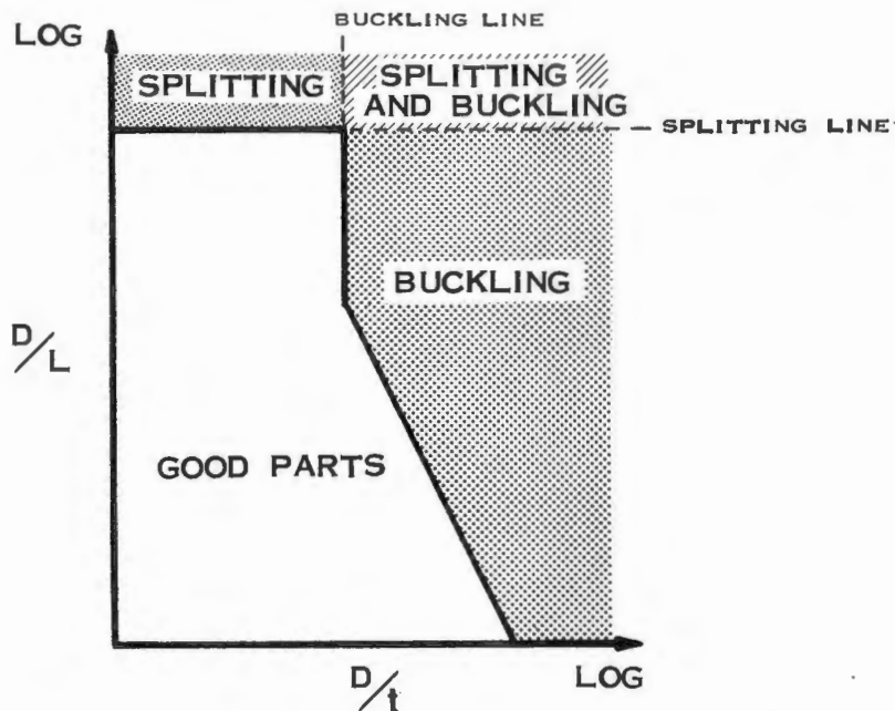
FIGURE IB-6 TYPICAL FORMABILITY ENVELOPE .
