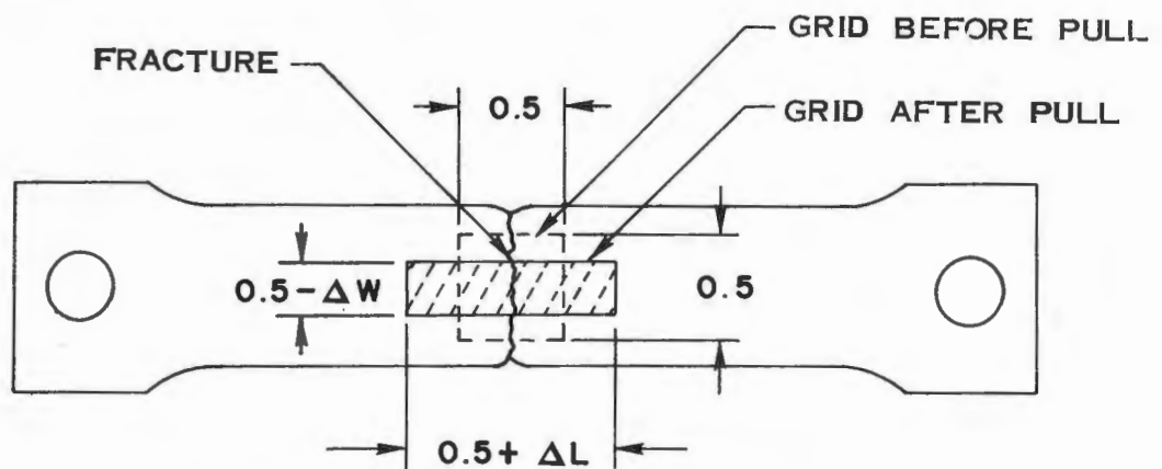
FIGURE VI B-8 1/2" WIDE TENSILE SPECIMEN.
