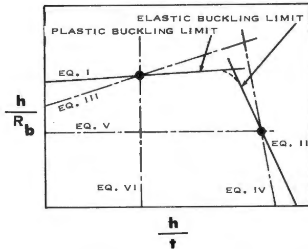
FIGURE V A-7 TYPICAL FORMABILITY CURVE AND INDEX LINES
