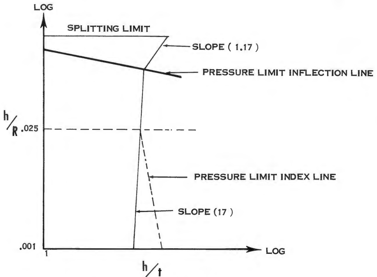
FIGURE II B-7 GRAPH CONSTRUCTION
