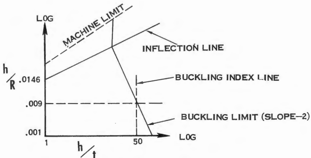
FIGURE III B-8 GRAPH CONSTRUCTION
