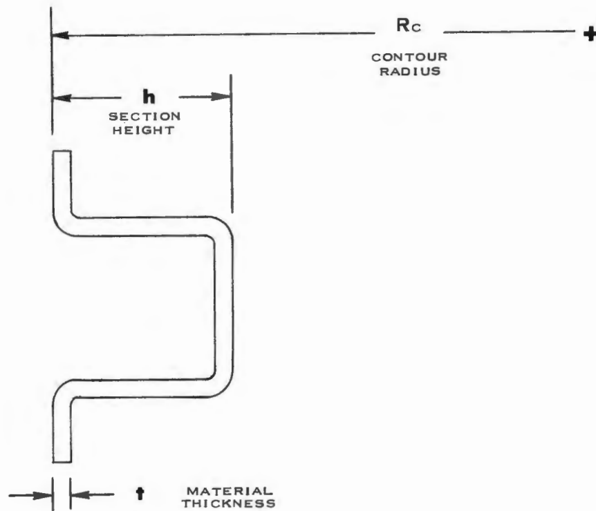
FIGURE IIIA-20 HEEL-IN HAT SECTIONS
