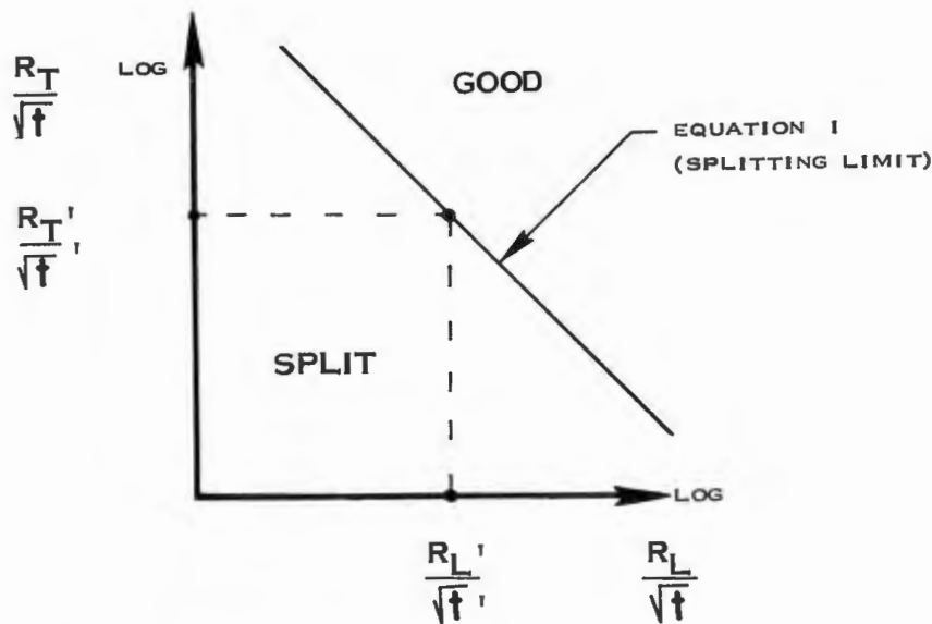
FIGURE IV B-6 PROCEDURE FOR FINDING THE SPLITTING LIMIT
