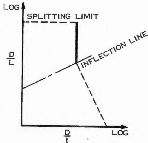
FIGURE IB-8 GRAPH CONSTRUCTION.
