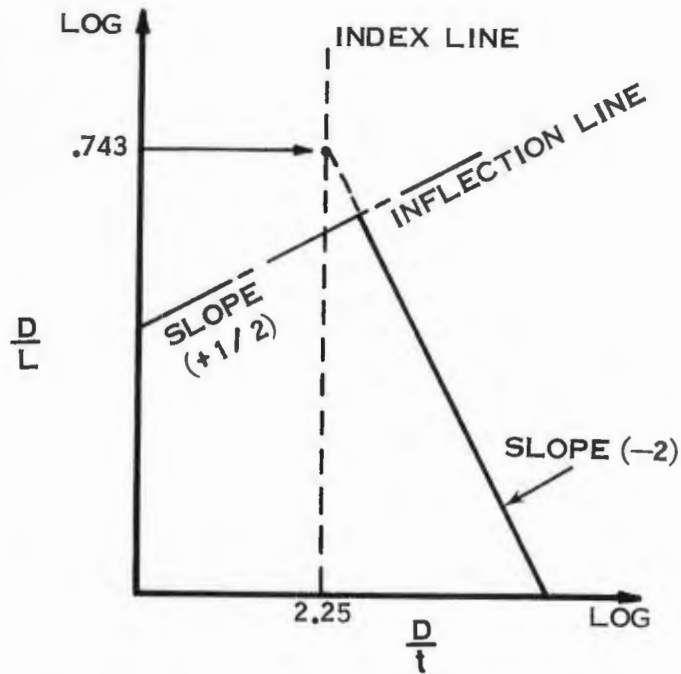
FIGURE IB-7 GRAPH CONSTRUCTION.
