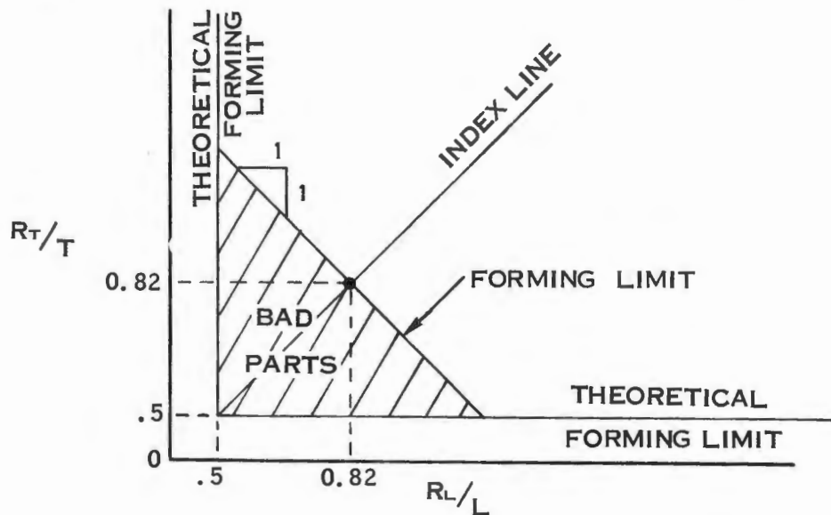
PLOTTING THE FORMING LIMITS FIG. IV A-8
