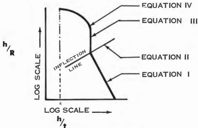
FIGURE III A-7 EQUATION APPLICATION FOR CLASS I FORMABILITY LIMIT CURVES
