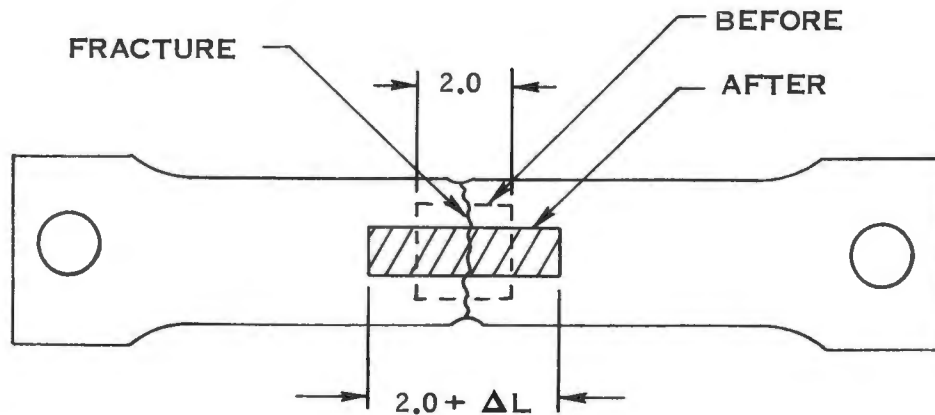
TYPICAL GRIDDED TENSION SPECIMEN FIG. IV A-4
