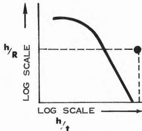
FIGURE III A-10 UNSATISFACTORY FORMABILITY
