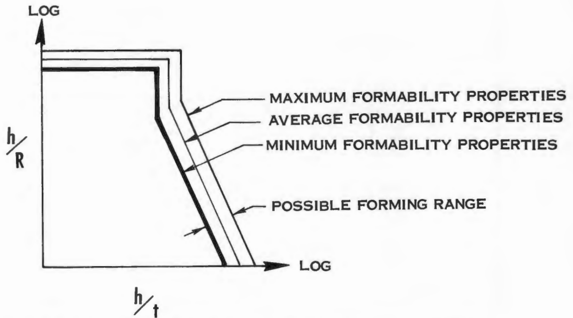
FIGURE II B-10 POSSIBLE RANGE IN FORMABILITY CURVES
