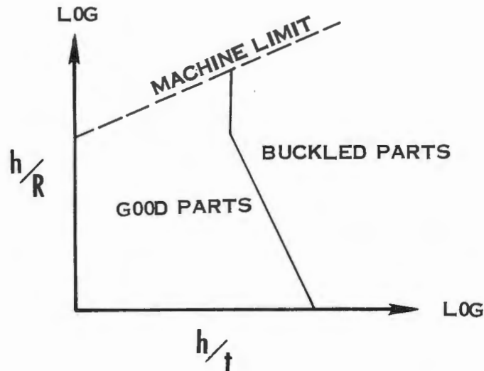
FIGURE III B-7 TYPICAL FORMABILITY CURVE
