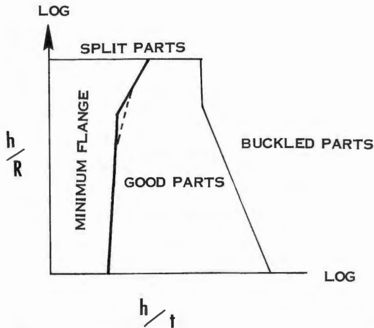
FIGURE II B-8 TYPICAL FORMABILITY CURVE
