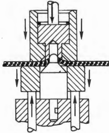
FIGURE II A-3 CROSS SECTION OF RAM COIN DIMPLING
