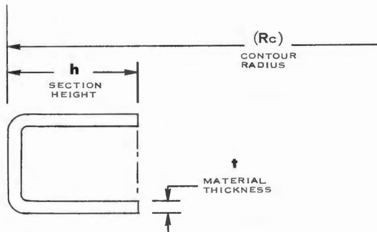
HEEL-OUT CHANNEL FIGURE IIIA-17
