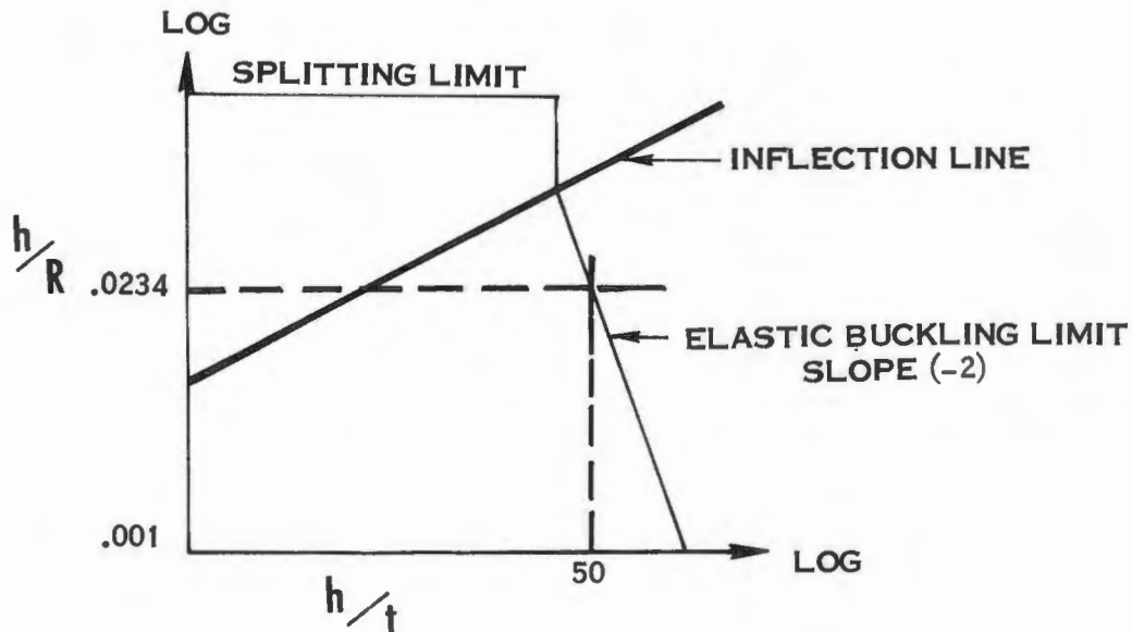
FIGURE II B-5 GRAPH CONSTRUCTION
