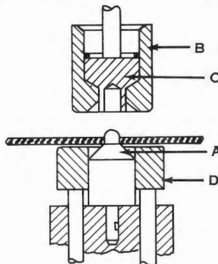
FIGURE II A-1 CROSS SECTION OF RAM COIN DIMPLING
