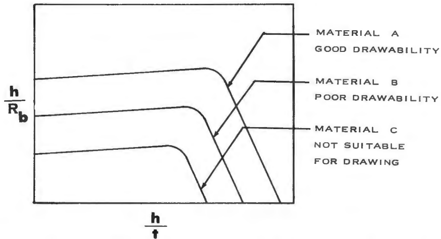
FIGURE V A-6 TYPICAL FORMABILITY CURVES ILLUSTRATING THE POSITION OF VARIOUS MATERIALS
