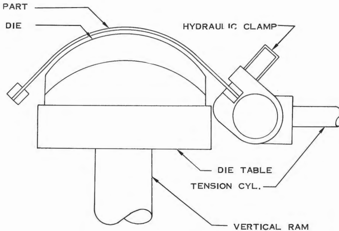
TYPICAL SHEET STRETCH SET-UP FIGURE IVA-1
