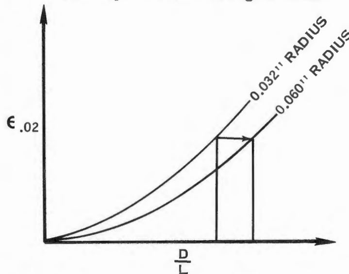
FIGURE IB-10 SPLITTING LIMIT LINE.
