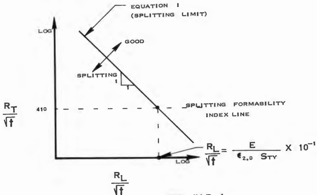
FIG. IV B-4 SPLITTING LIMIT CURVE
