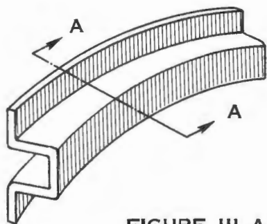
FIGURE III A-6 HEEL-IN HAT SECTION
