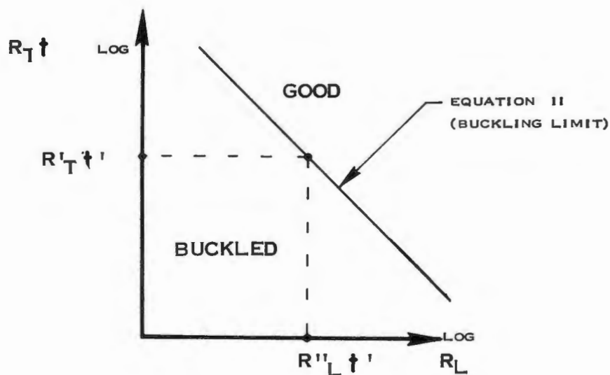
FIGURE IV B-7 PROCEDURE FOR FINDING THE BUCKLING LIMIT
