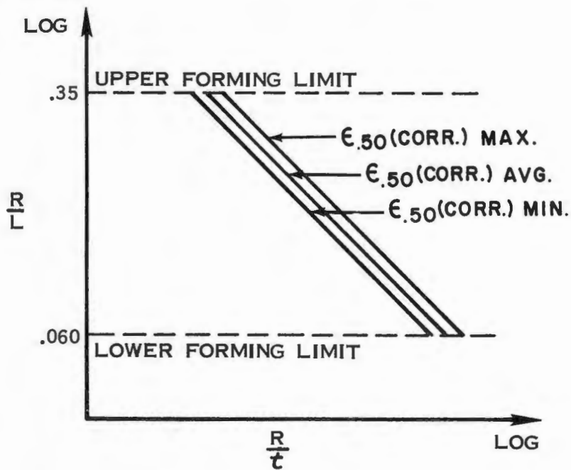
FIGURE VI B-12 VARIATION OF MATERIAL PROPERTIES.
