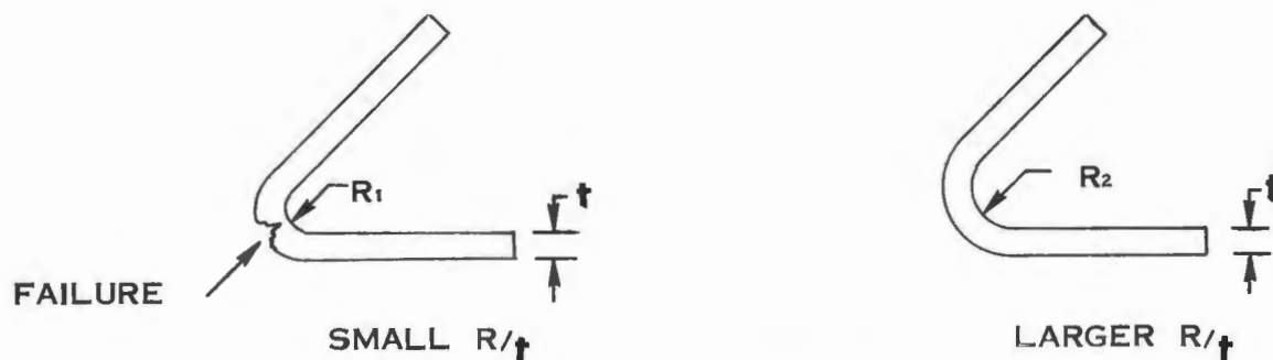
EFFECT OF VARYING R/t VALUES FIG. IA-3
