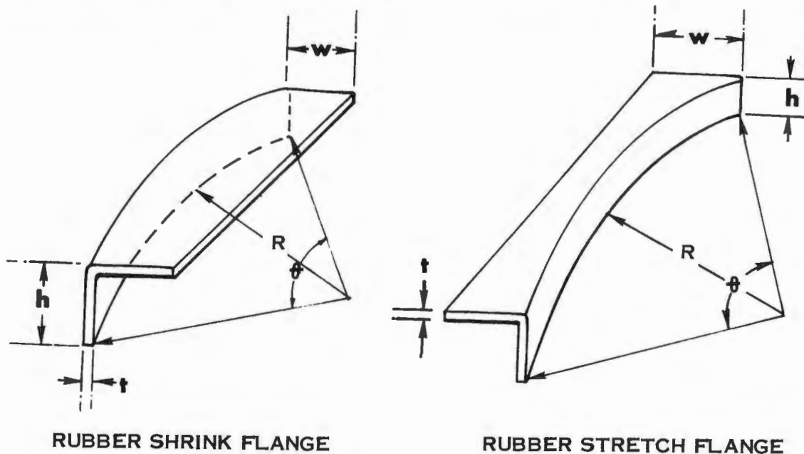
FIGURE II B-2 RUBBER SHRINK AND STRETCH PARTS
