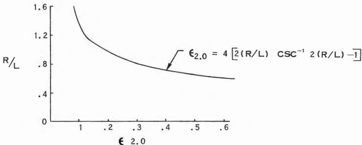
PLOTTING EQUATION II FIG. IV A-5
