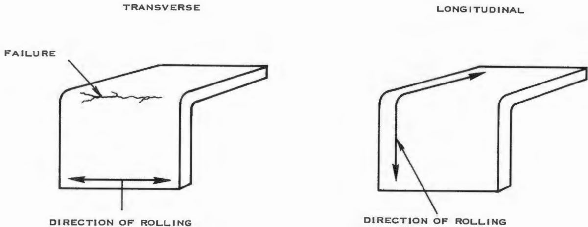
EFFECT OF DIRECTION OF ROLL ON BENDING FIG. 1 A-5
