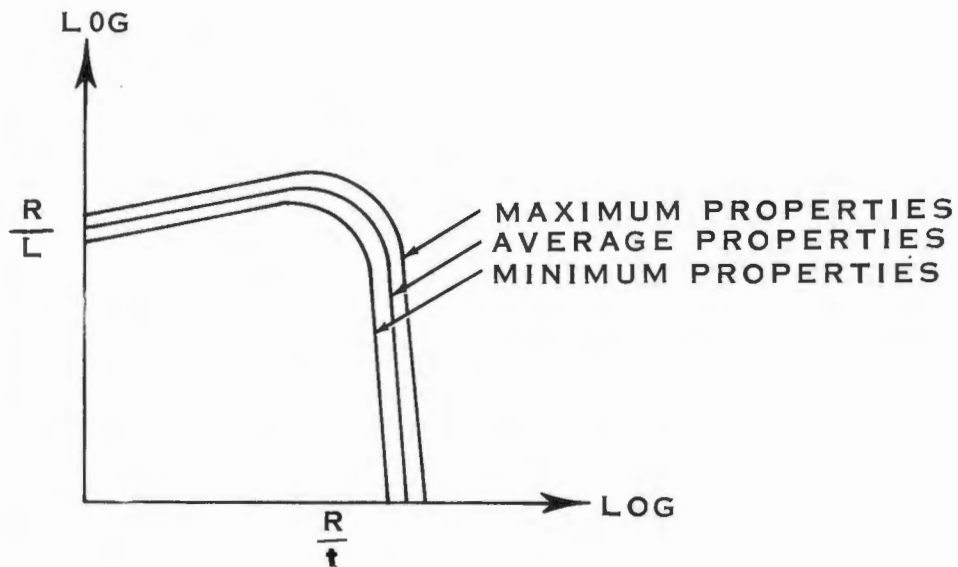
FIGURE VI A-6 RANGE IN FORMABILITY LIMITS
