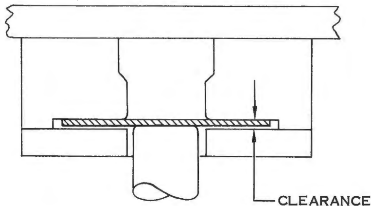
FIGURE V A-2 SINGLE ACTION DRAW DIE
