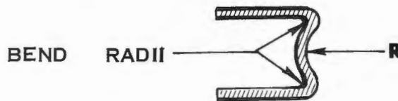
FIGURE III A-15 COLUMN COLLAPSE DUE TO LARGE BEND RADII
