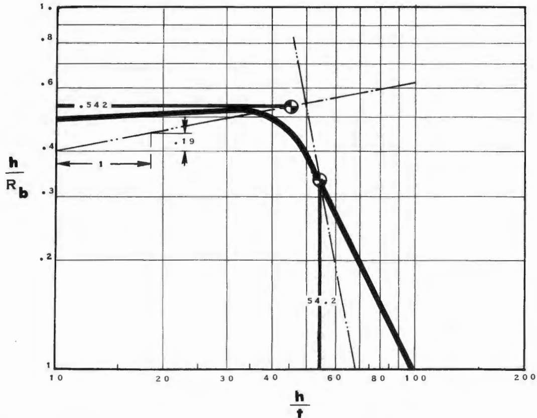
FIGURE V A-8 SAMPLE CONSTRUCTION OF THE THEORETICAL FORMABILITY LIMIT CURVE FOR TUNGSTEN AT 1000° F
