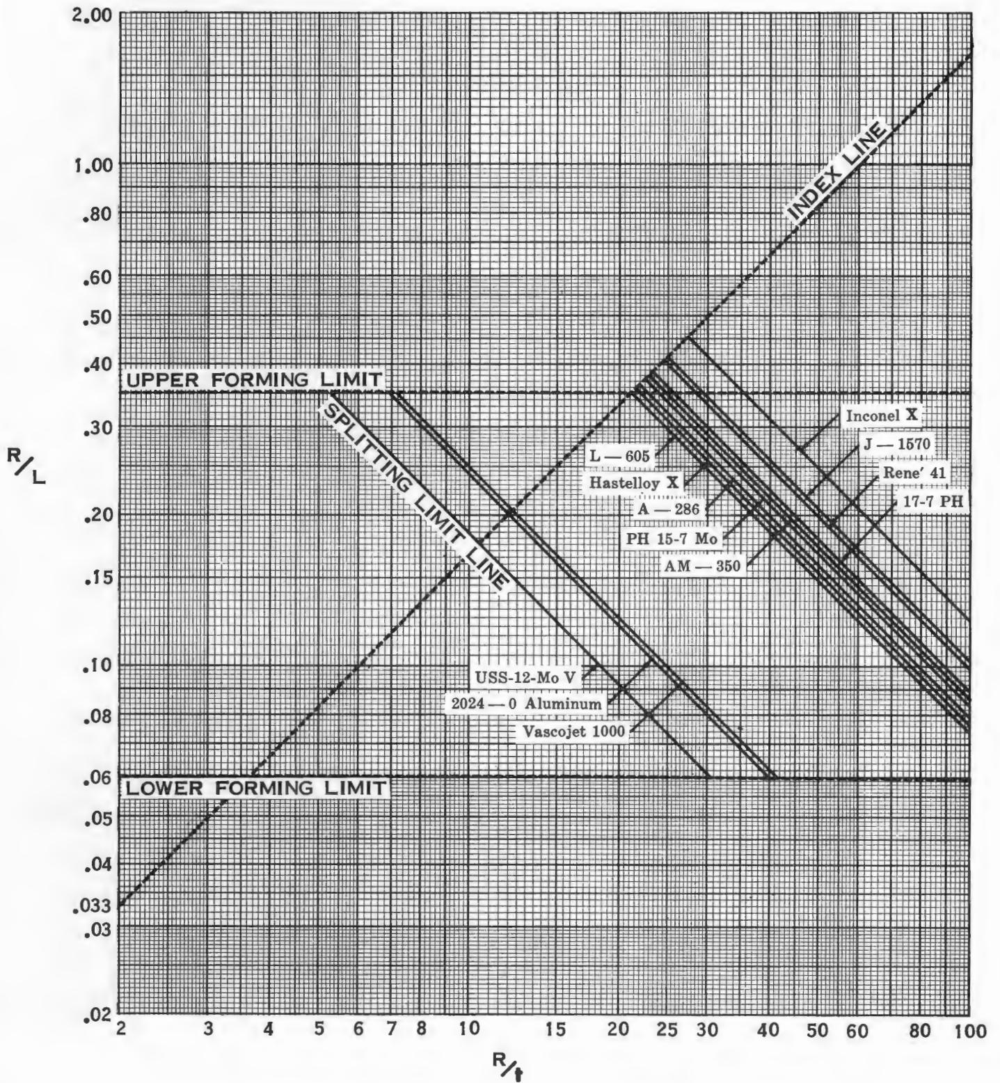
GRAPH VI B-1 COMPOSITE GRAPH FOR DROP HAMMER BEADED PANELS
