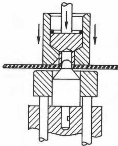
FIGURE II A-2 CROSS SECTION OF RAM COIN DIMPLING
