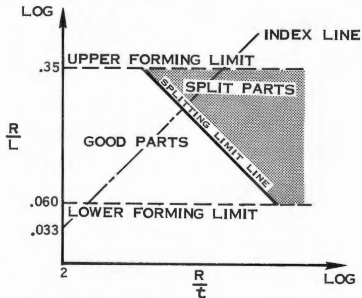
FIGURE VI B-11 TYPICAL FORMABILITY ENVELOPE.
