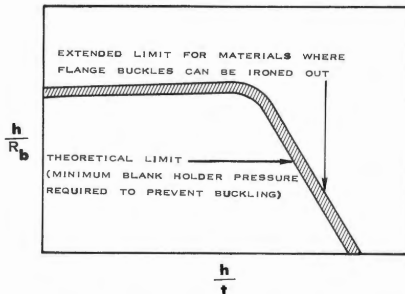
FIGURE V A-12 FORMABILITY LIMIT INCREASE FROM REDUCED BLANK HOLDER PRESSURE
