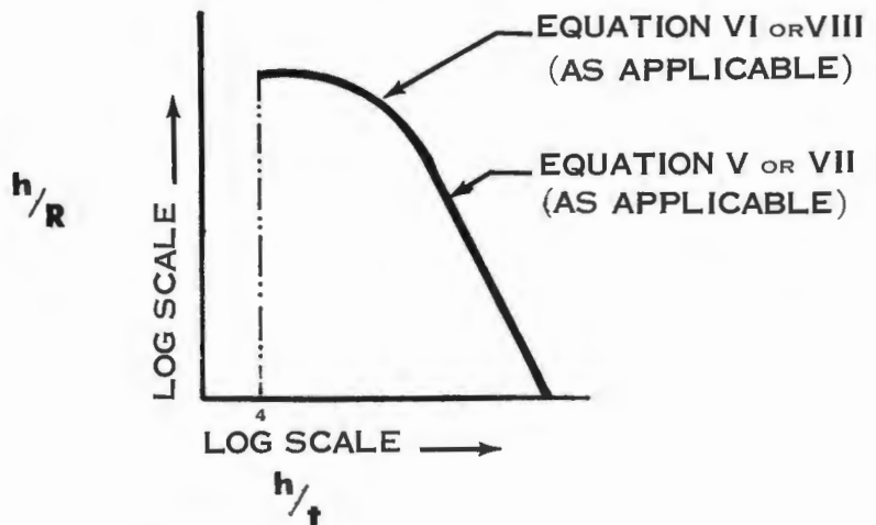
FIGURE III A-8 EQUATION APPLICATION FOR CLASS 2 AND CLASS 3 FORMABILITY LIMIT CURVES
