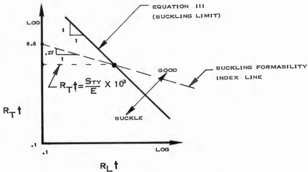
FIG. IV B-5 BUCKLING LIMIT CURVE
