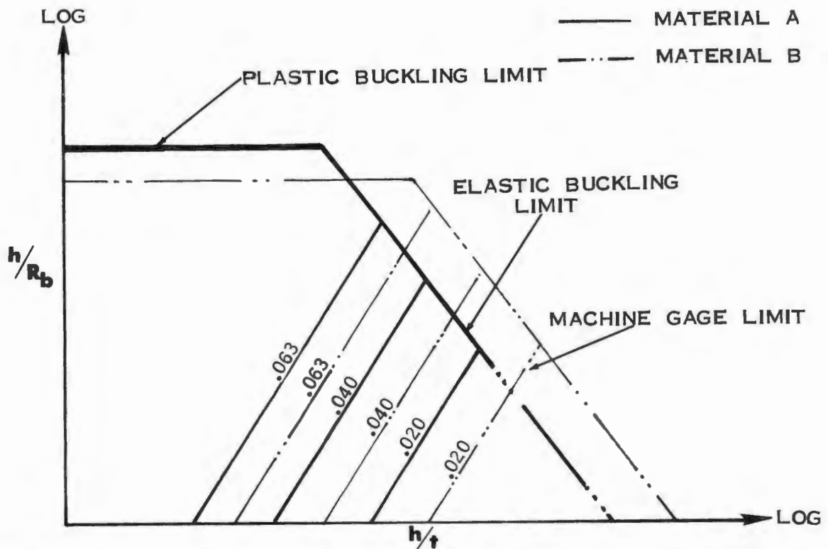
FIGURE VB-4 FORMING LIMIT CURVES FOR SPINNING SHOWING MACHINE LIMITS
