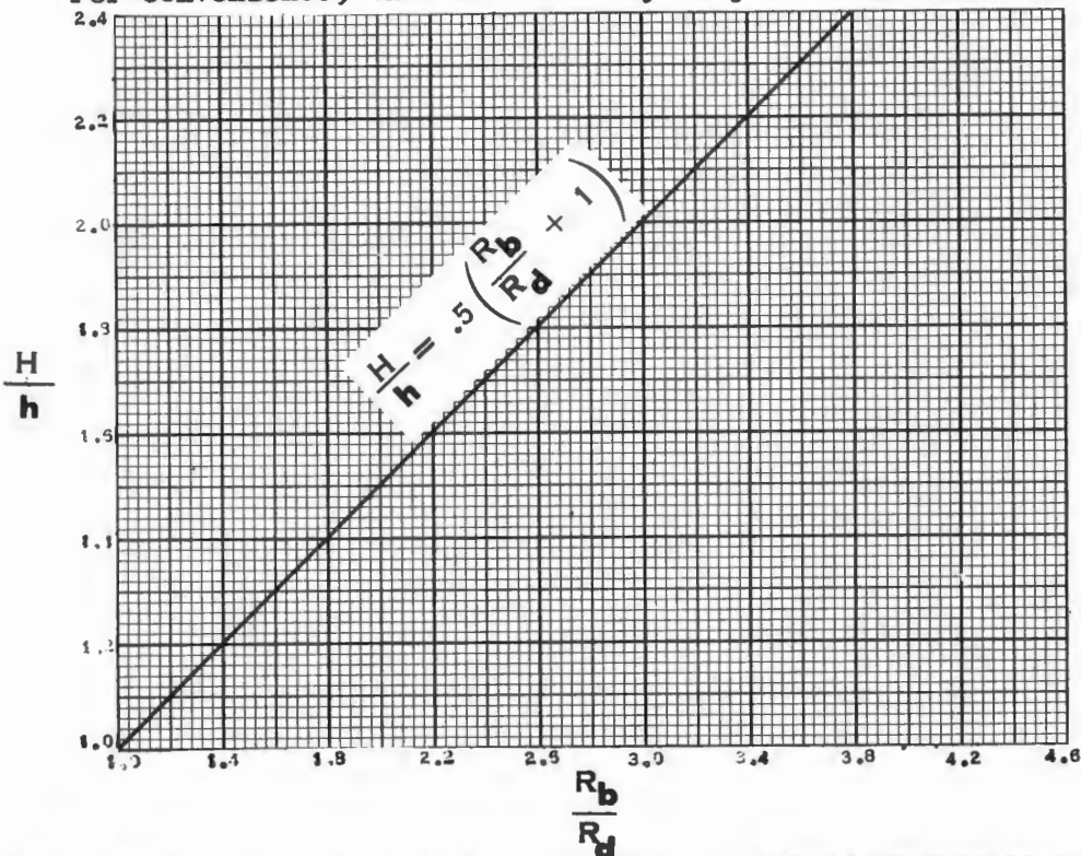
FIGURE V A-10 CURVE FOR CONVERTING FROM OVERHANG ( h ) TO FINAL CUP HEIGHT ( H )
