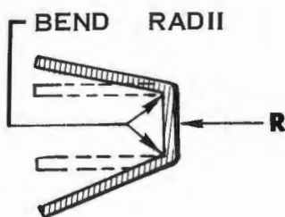
FIGURE III A-14 SPRING BACK DUE TO LARGE BEND RADII
