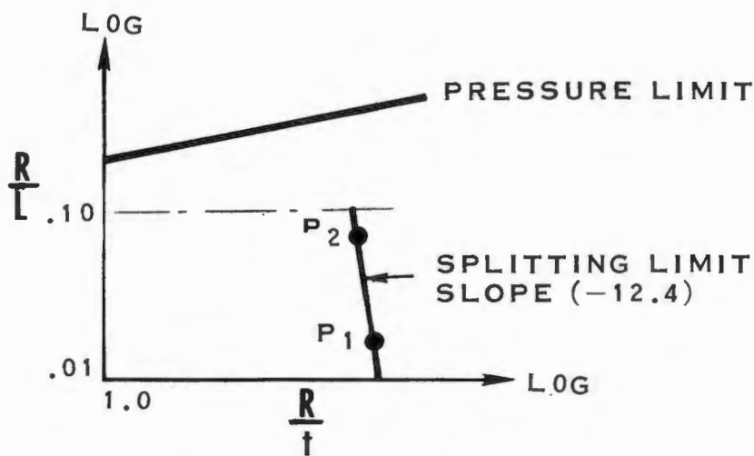
FIGURE VI A-3 GRAPH CONSTRUCTION
