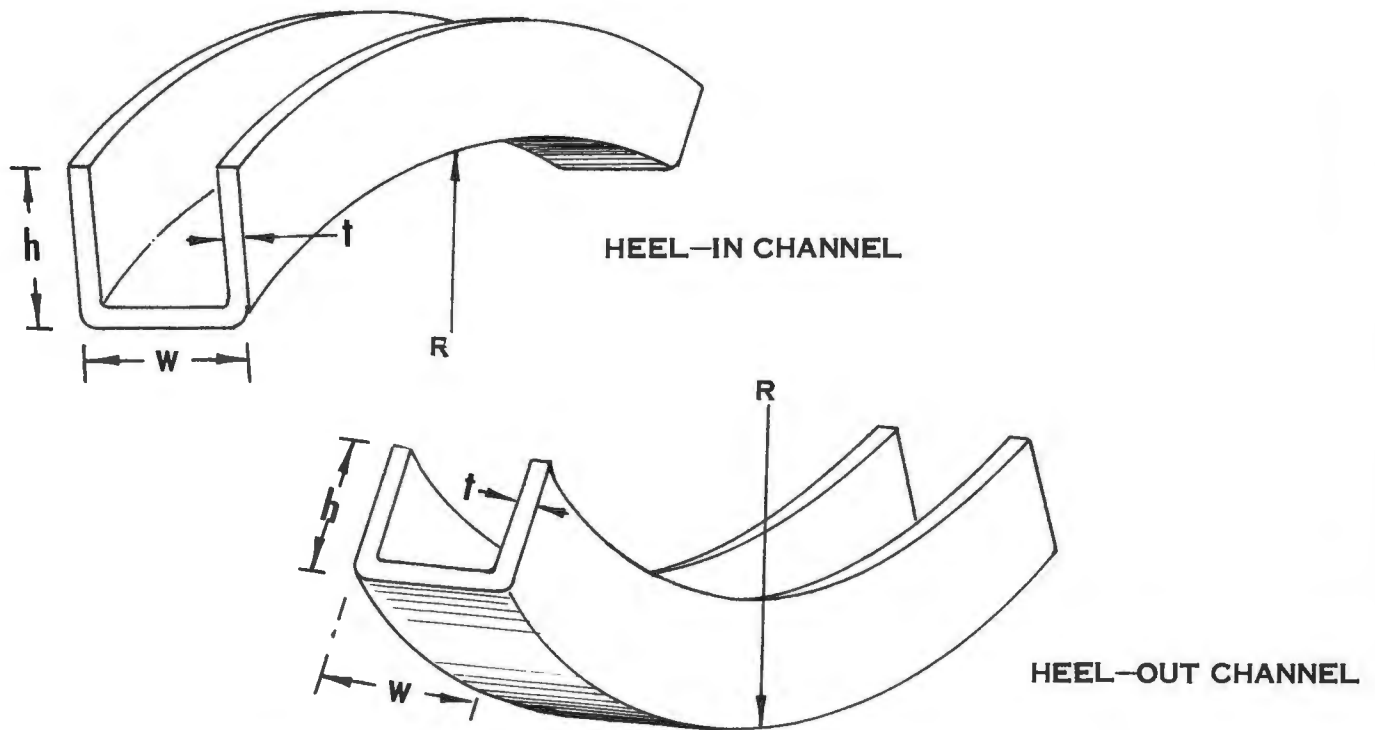
FIGURE III B-4 LINEAR ROLL HEEL-IN AND HEEL-OUT CHANNELS
