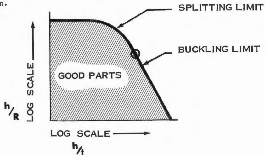
FIGURE III A-11 LOG TYPE FORMABILITY LIMIT CURVE
