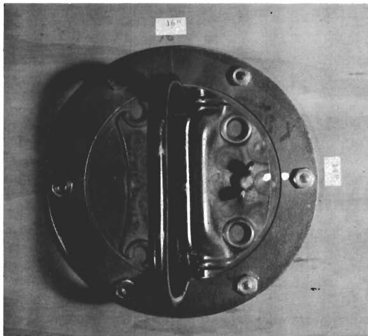
Figure 2. Details of Handle Construction The central ring holding the handle can turn 90^\circ , and is locked in either position by the wing-nut. Outer ring is 5-1/4 inches in diameter; inside dimension of handle is 3-3/4 inches. The diameter of the handle grip itself is 3/8-inch.
