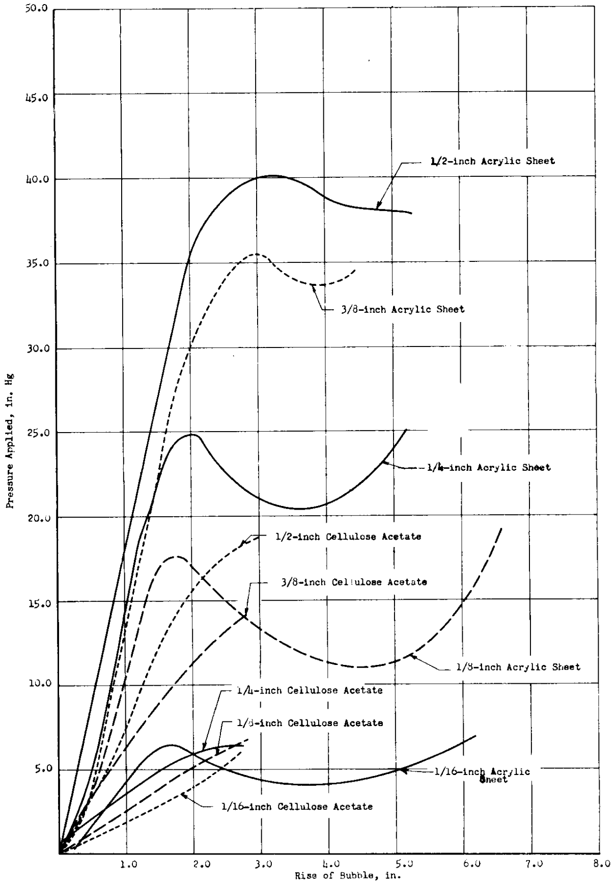
Fig. 6 PRESSURE-DEFORMATION CURVES FROM UNCONFINED BUBBLE TEST, LUBRICATED SPECIMEN, 4-INCH DIAMETER AT BASE
