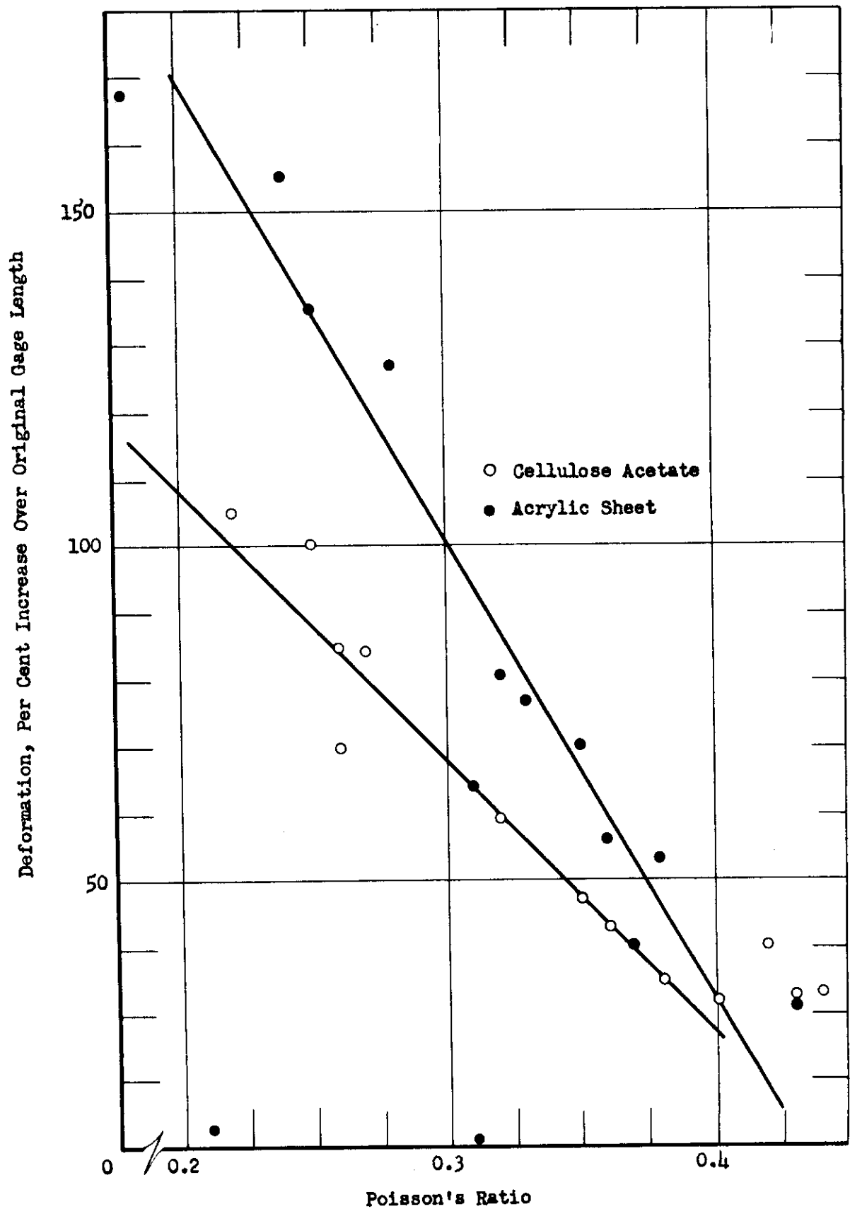
Fig. 12 POISSON'S RATIO VERSUS DEFORMATION
