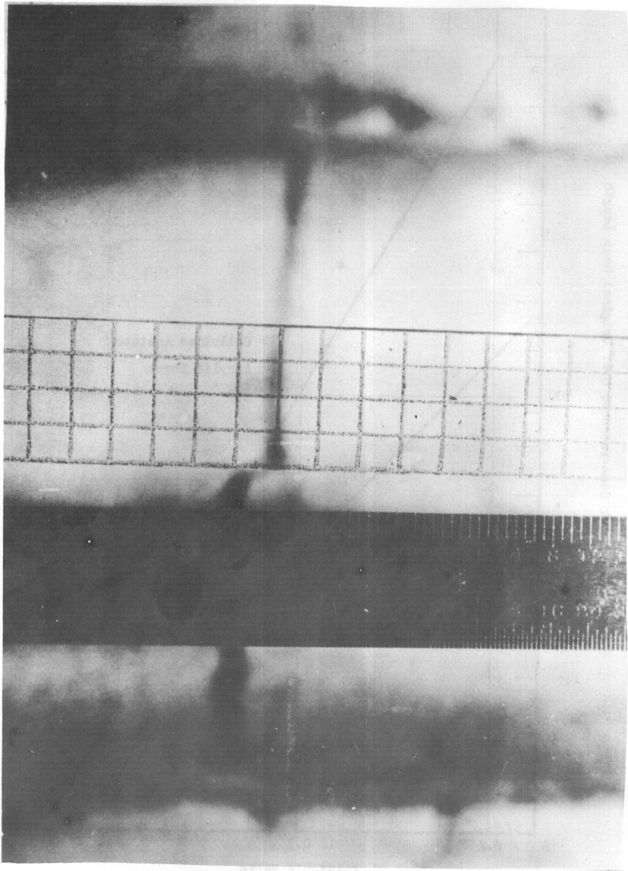
Fig. 13 EXAMPLE OF PHOTOGRAPHIC ENLARGEMENT USED IN DETERMINATION OF POISSON'S RATIO AT VARIOUS STRAINS
