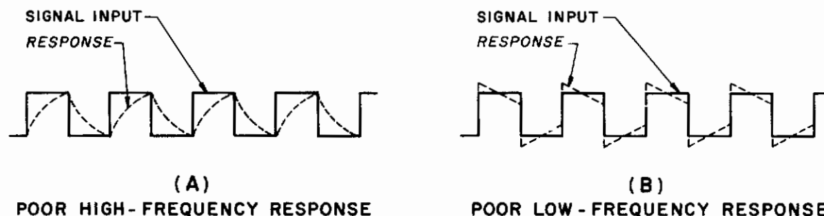
Figure 19. Frequency Distortion of a Square Wave
