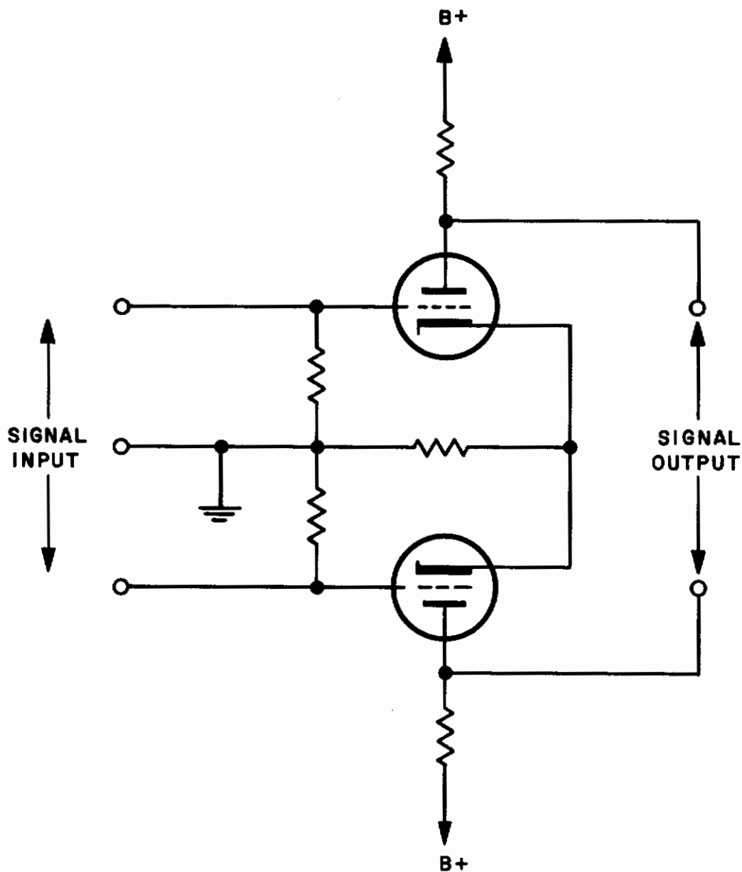
Figure 26. Simplified Balanced Amplifier
