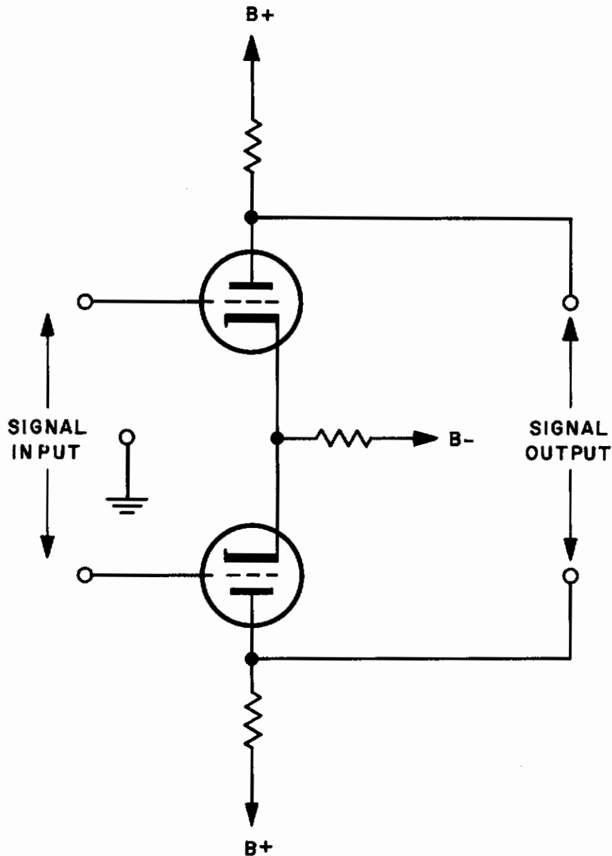
Figure 27. Simplified Differential Amplifier
