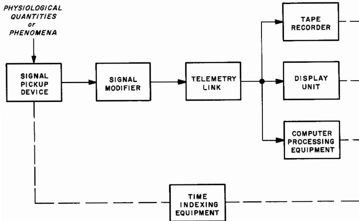
Figure 28. Physiological Measuring System with Accessories
