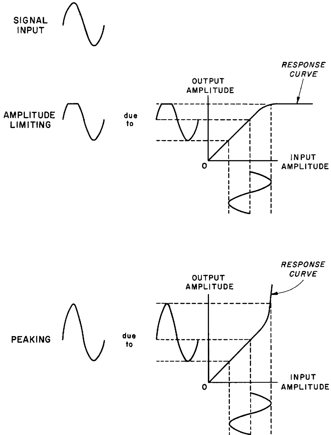
Figure 21. Nonlinearity of a Sine Wave
