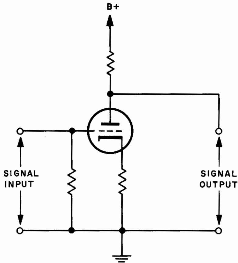
Figure 25. Simplified Single-Ended Amplifier
