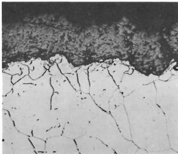
Fig. 8 - PHOTOMICROGRAPH OF TYPICAL ZIRCONIUM OXIDE - INCONEL BOND. The section shown is adjacent to the 1/8 inch defect. The coarse surface of the substrate was produced by sandblasting before applying 2 - 3 mil of zirconia.
