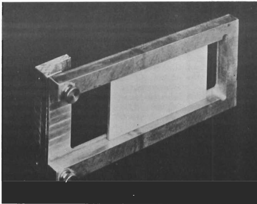
Fig. 2 - PRECISION SAMPLE HOLDER. This holder maintains the required parallelism between the sample and the image converter face.
