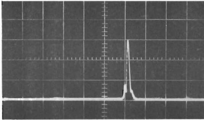
Fig. 23 - SIGNAL PRODUCED BY MODE CONVERSION OF A SURFACE WAVE TO A COMPRESSIONAL WAVE AT A LIQUID-SOLID INTERFACE. The submerged receiver in Fig. 21 detects compressional energy re-radiated into the liquid after transmission as a surface wave along the steel plate.
