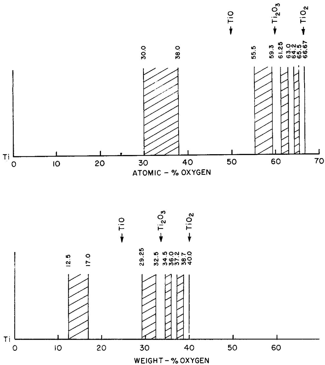
Fig. 61 - Phases and Phase Ranges in the System Titanium-Oxygen (Ehrlich)
