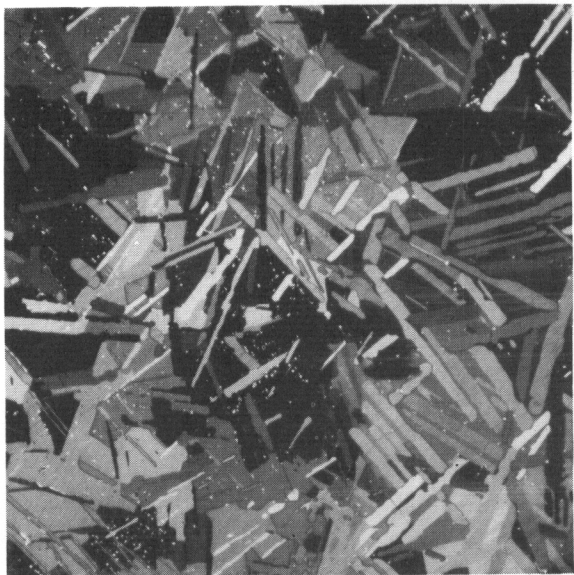
Neg. No. 3490 X100 Polarized light Unetched
