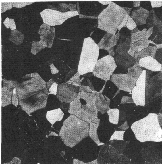
Neg. No. 3409 X150 Polarized light Unetched
