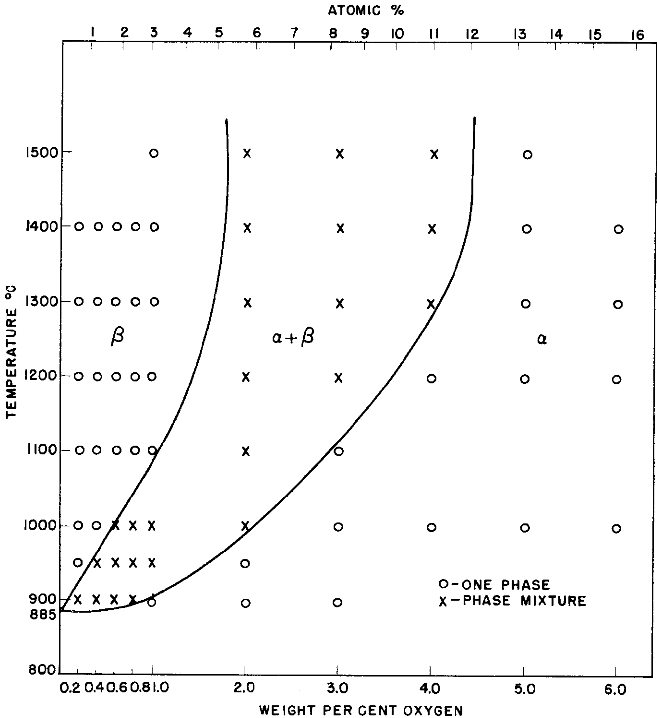
Fig. 63 - Titanium Rich Portion of the Titanium-Oxygen System
