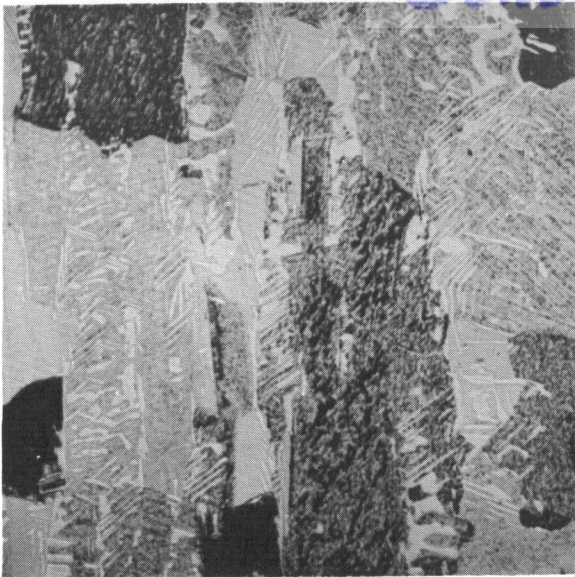
Neg. No. 3404 X250 2%HF, 3%HNO 3 in water
