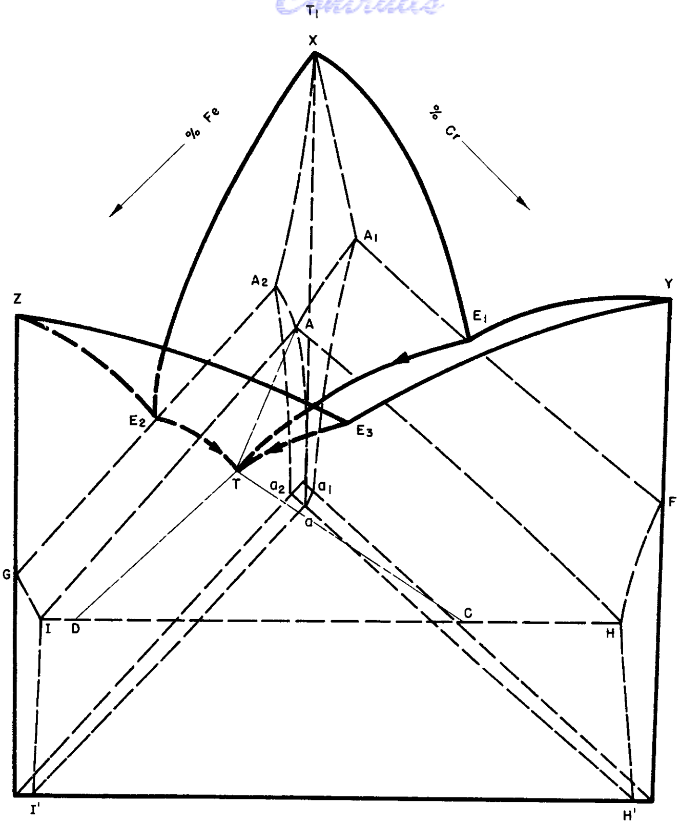
Fig. 44 - Space Model of the Solid State Reactions in the System Titanium-Chromium-Iron
