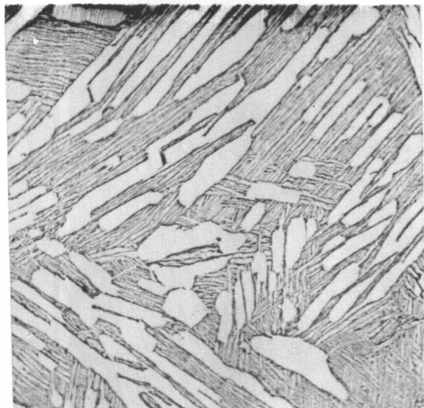
Neg. No. 3656 X150 Fig. 67 A 1.0% oxygen alloy quenched after 24 hours at 1000°C. Structure shows approximately 35% \alpha in a transformed \beta matrix.
