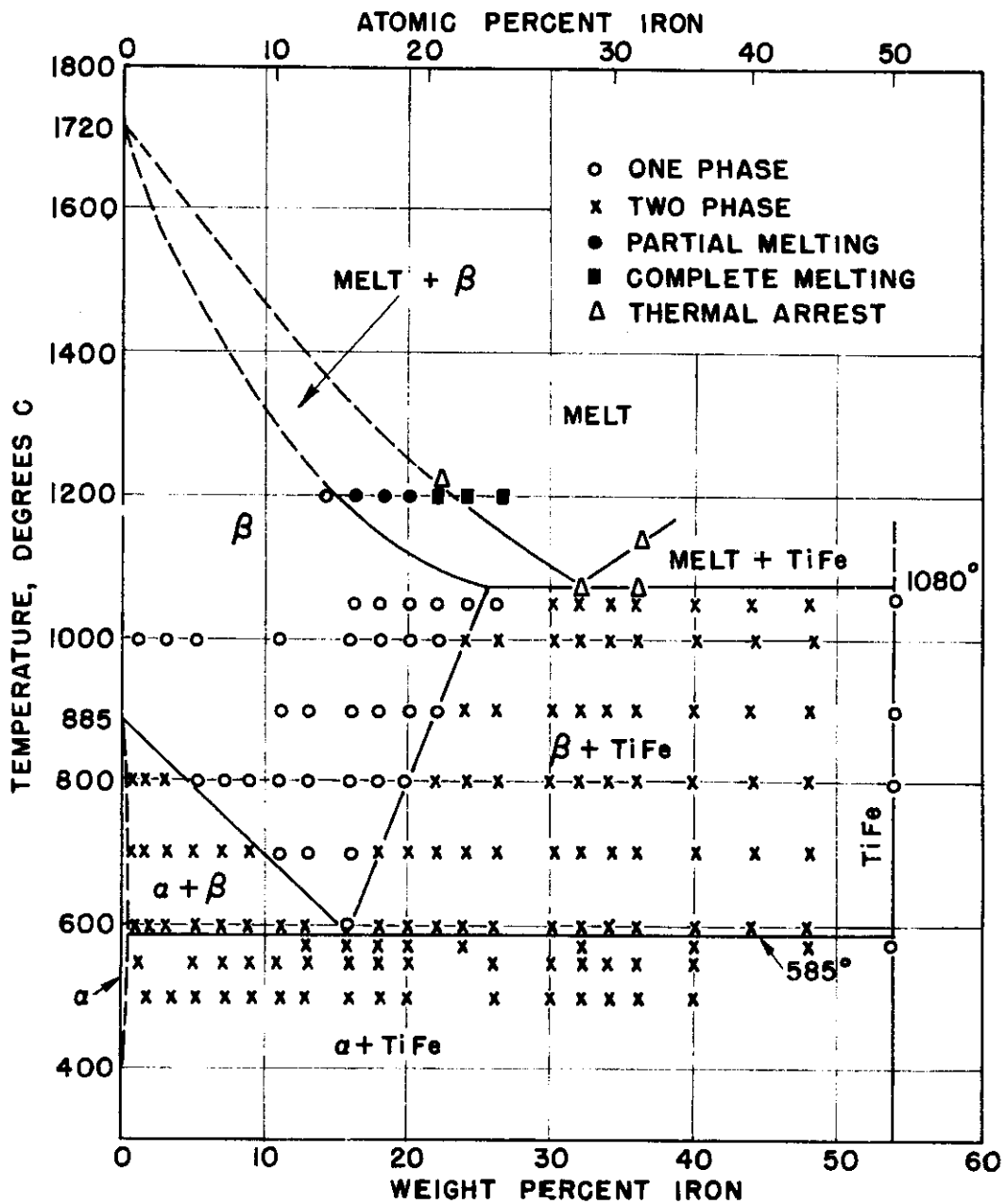
Fig. 33- Partial Phase Diagram of the Titanium-Iron System.
