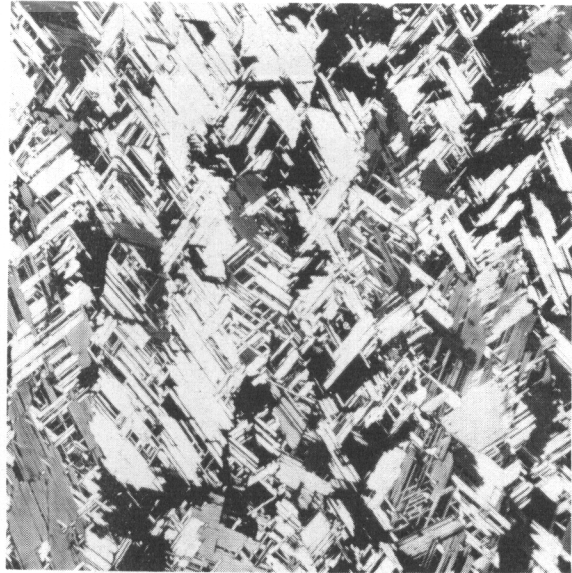
Neg. No. 3614 PL, X 75 Unetched
