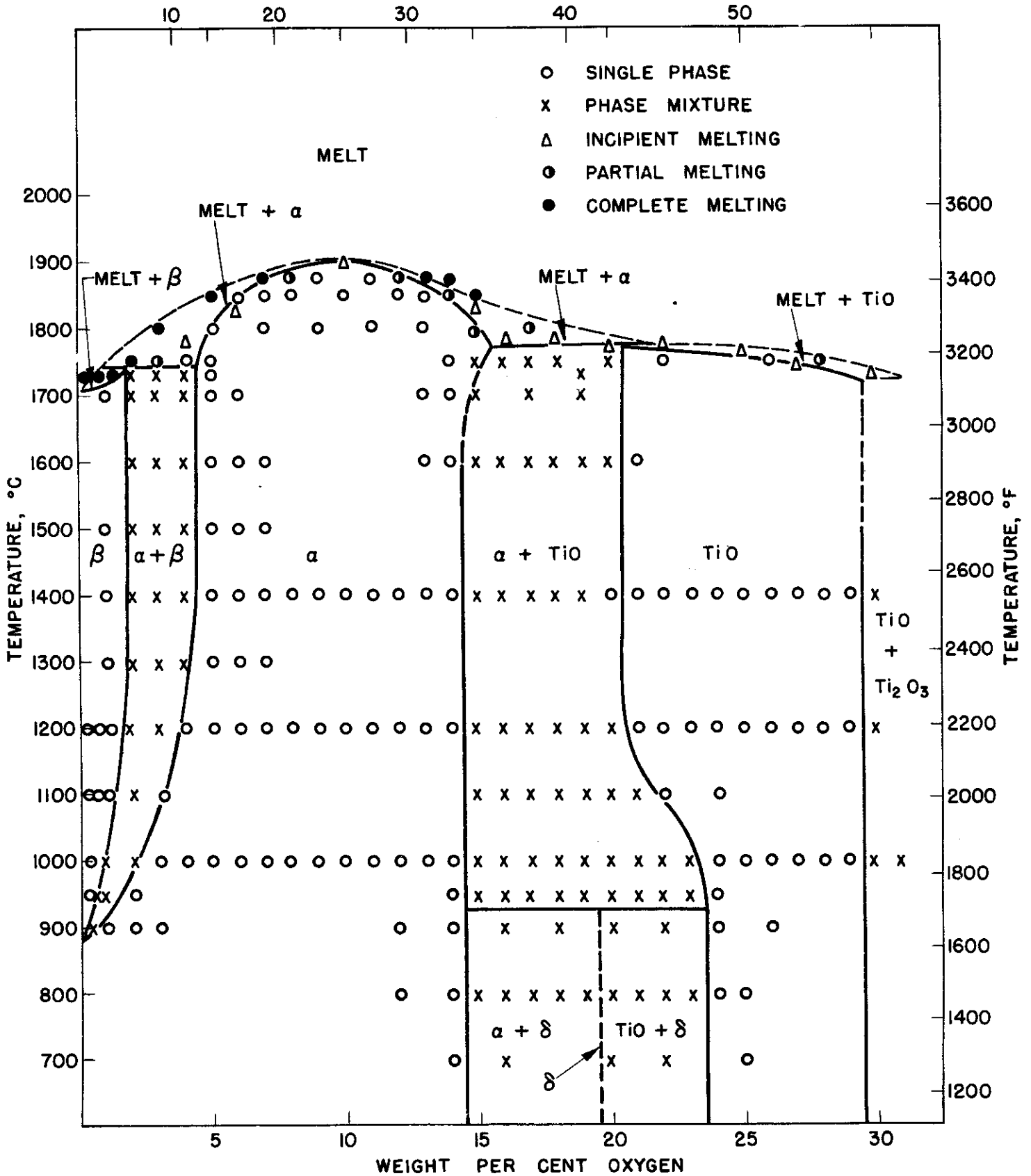
Fig. 62 - Partial Phase Diagram of the Titanium-Oxygen System
