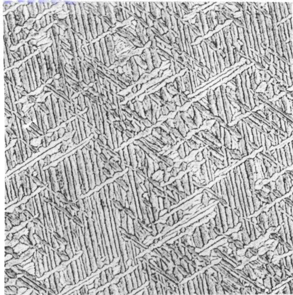
Neg. No. 3611 X150 Fig. 65 A 1.0% oxygen alloy quenched after 4 hours at 1200°C. Structure reveals a typical basket weave type of transformation structure.
