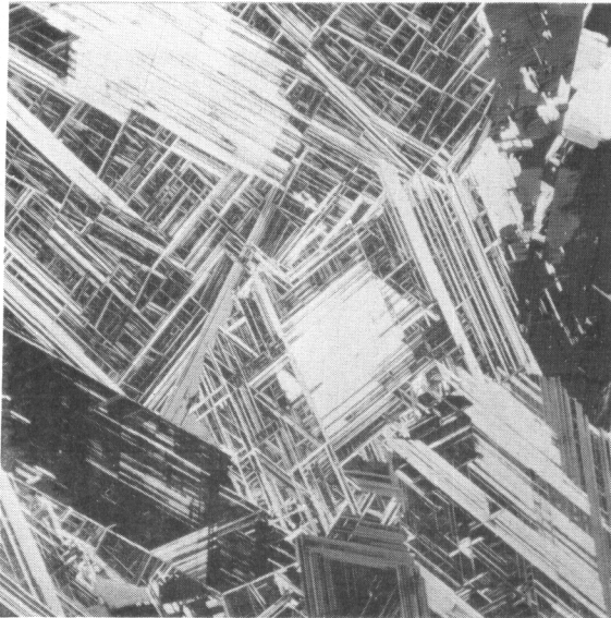
Neg. No. 3755 PL, X 75 Unetched
