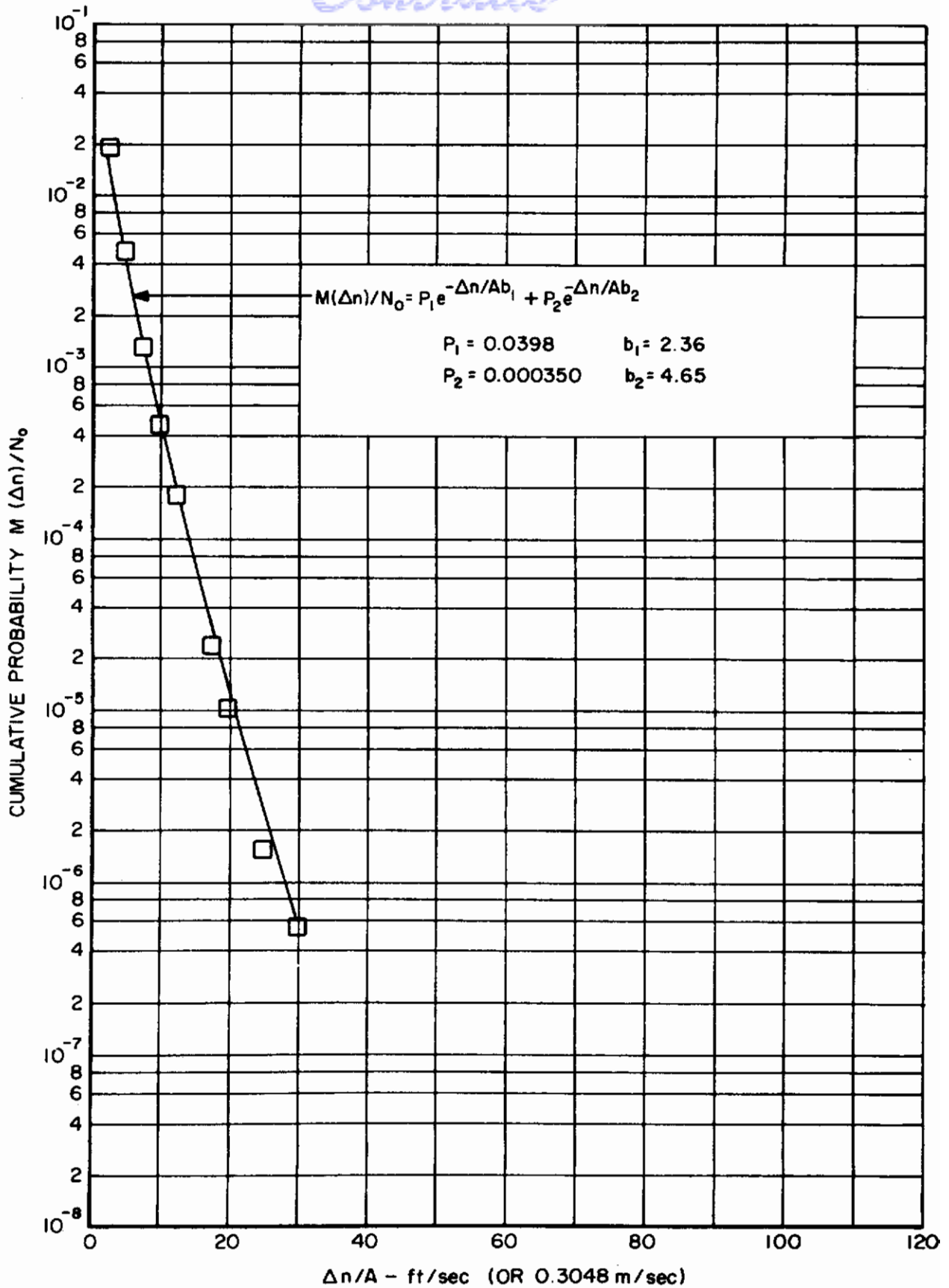
Figure 13 Combined Vertical Turbulence Environment and Severe Turbulence Encounters Altitude Range 40,000 - 50,000 feet (12,192 - 15,240 meters)
