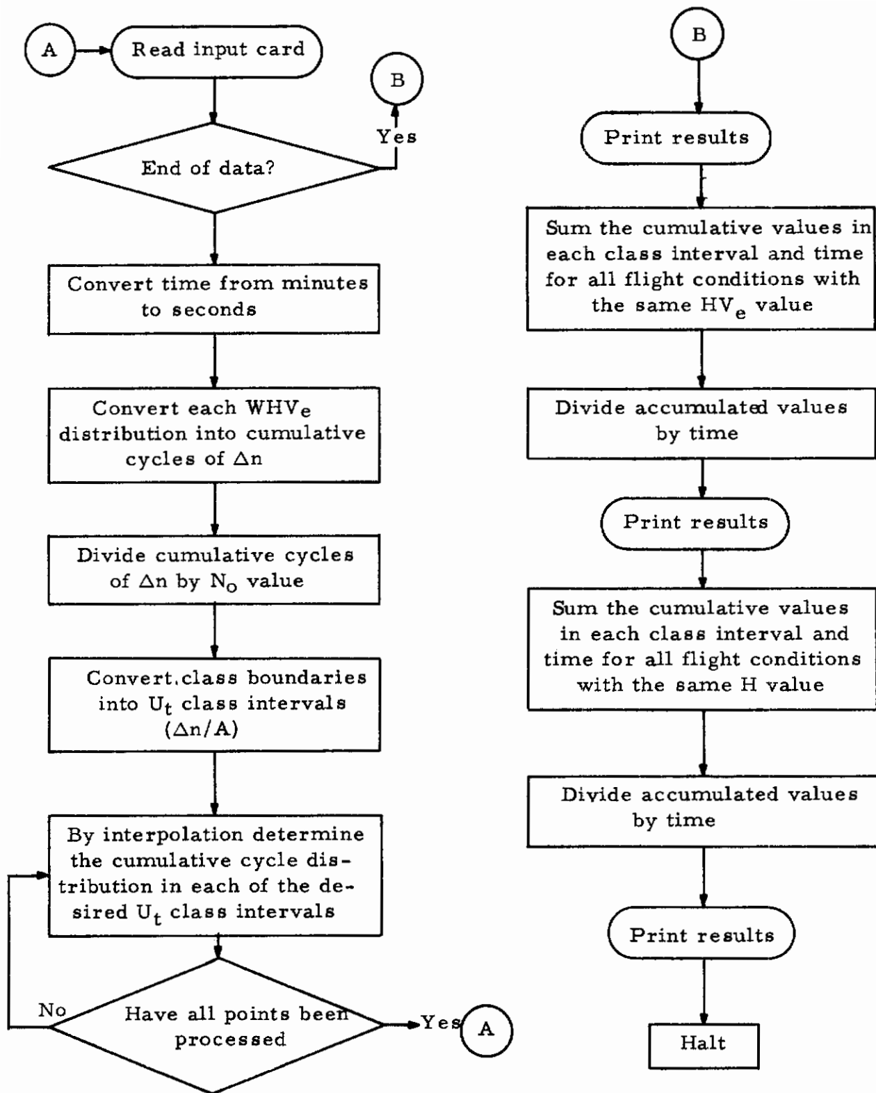
Figure 2 Noncoded Flow Chart, True Gust Velocity Distributions
