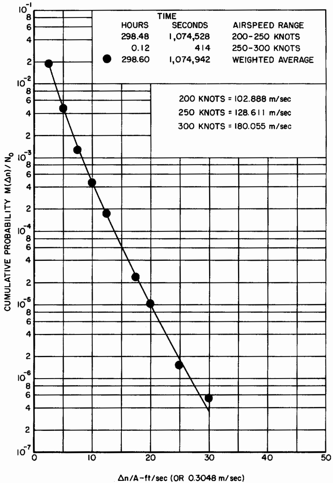
Figure 7 Vertical Turbulence Environment by Airspeed Altitude 40,000 - 50,000 feet (12,192 - 15,240 meters)
