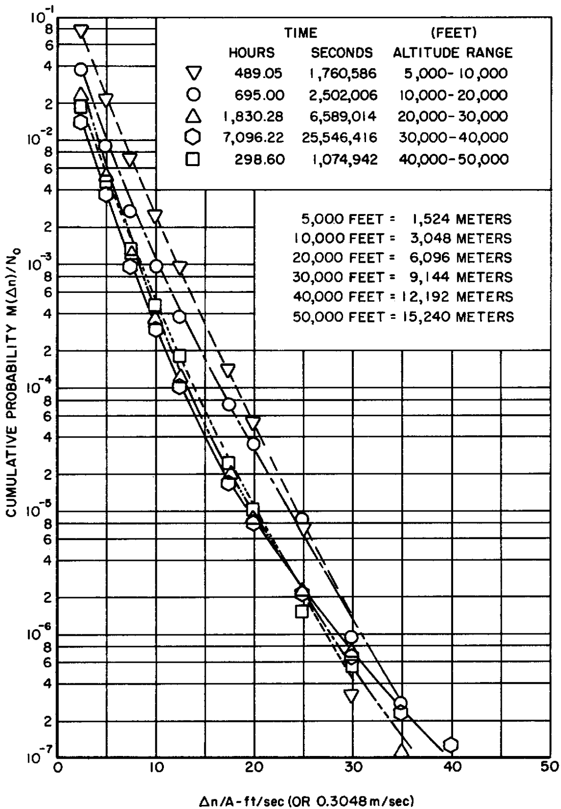
Figure 8 Vertical Turbulence Environment by Altitude Airspeed Range 200 - 350 Knots (102.888 - 180.055 ms -1 )
