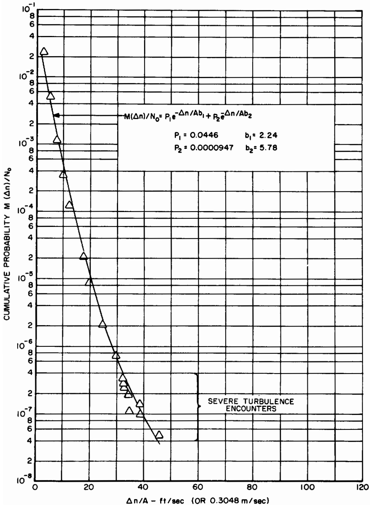
Figure 11 Combined Vertical Turbulence Environment and Severe Turbulence Encounters Altitude Range 20,000 - 30,000 feet (6,096 - 9,144 meters)
