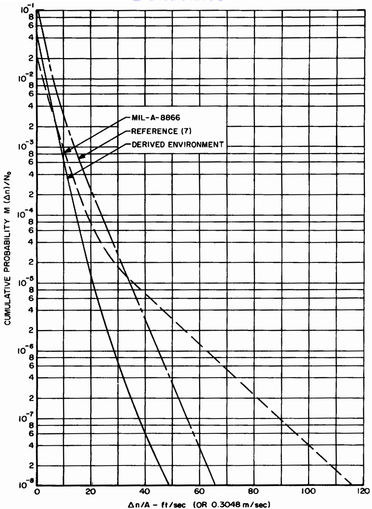
Figure 18 Comparison of Derived Vertical Turbulence Environments Altitude Range 40,000 - 50,000 feet (12,192 - 15,240 meters)
