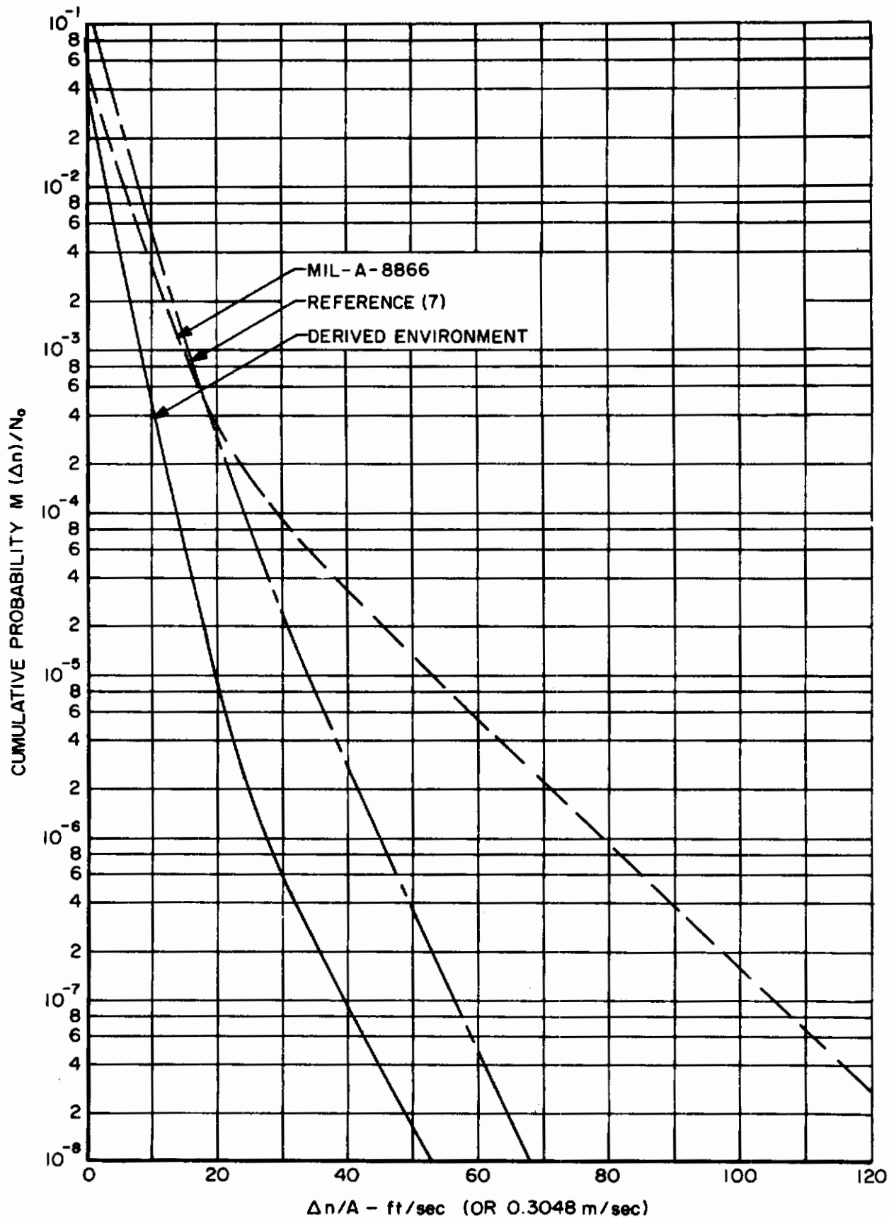
Figure 16 Comparison of Derived Vertical Turbulence Environments Altitude Range 20,000 - 30,000 feet (6,096 - 9,144 meters)
