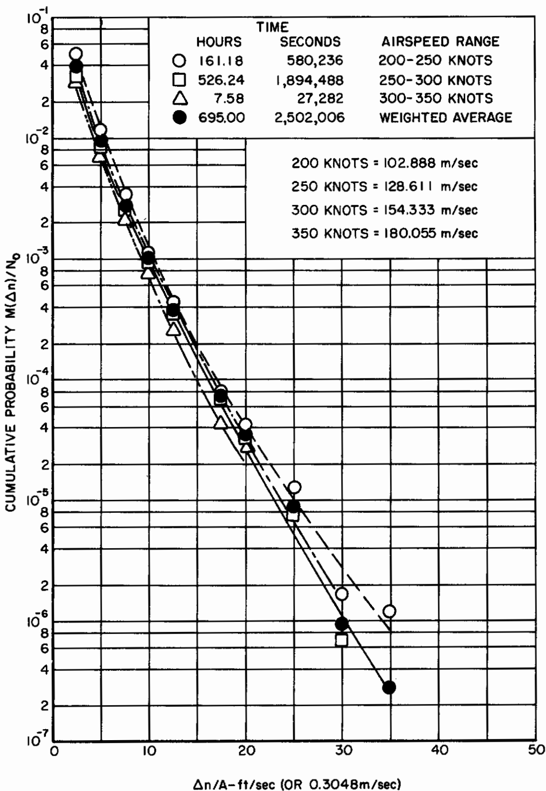
Figure 4 Vertical Turbulence Environment by Airspeed Altitude 10,000 - 20,000 feet (3,048 - 6,096 meters)
