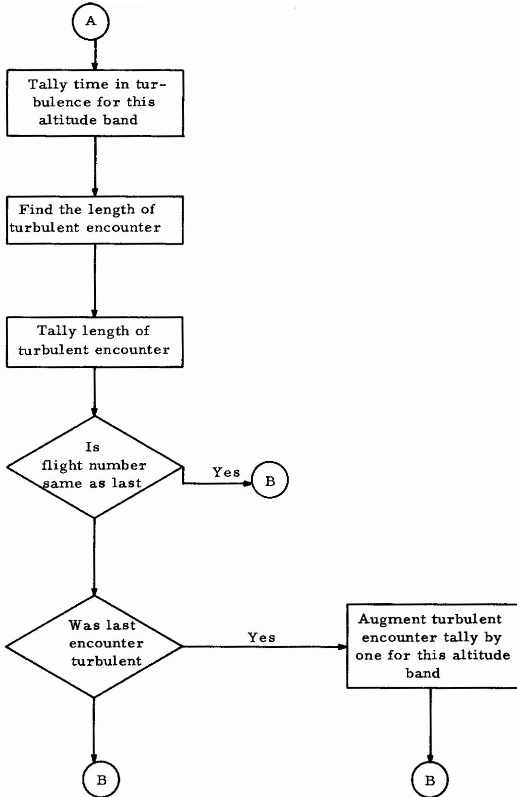
Figure 20 (b) Noncoded Flow Chart, Percent Time in Turbulence, (Continued)
