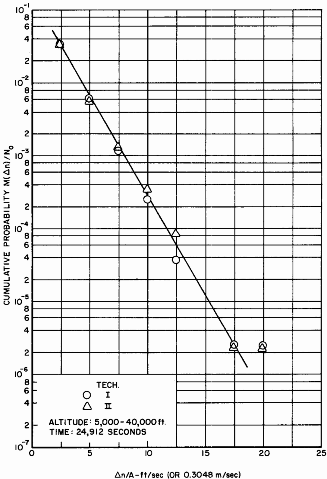
Figure 1 Comparison of M(\Delta n)/N_0 Versus \Delta n/A Data Determined From Two Techniques
