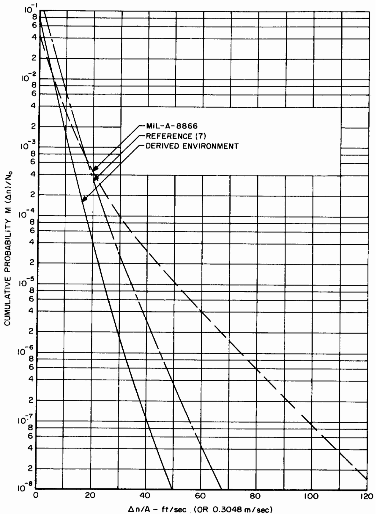
Figure 15 Comparison of Derived Vertical Turbulence Environments Altitude Range 10,000 - 20,000 feet (3,048 - 6,096 meters)
