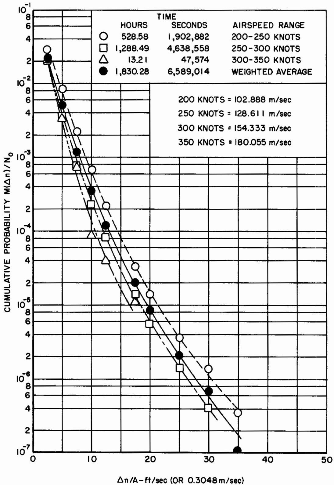
Figure 5 Vertical Turbulence Environment by Airspeed Altitude 20,000 - 30,000 feet (6,096 - 9,144 meters)
