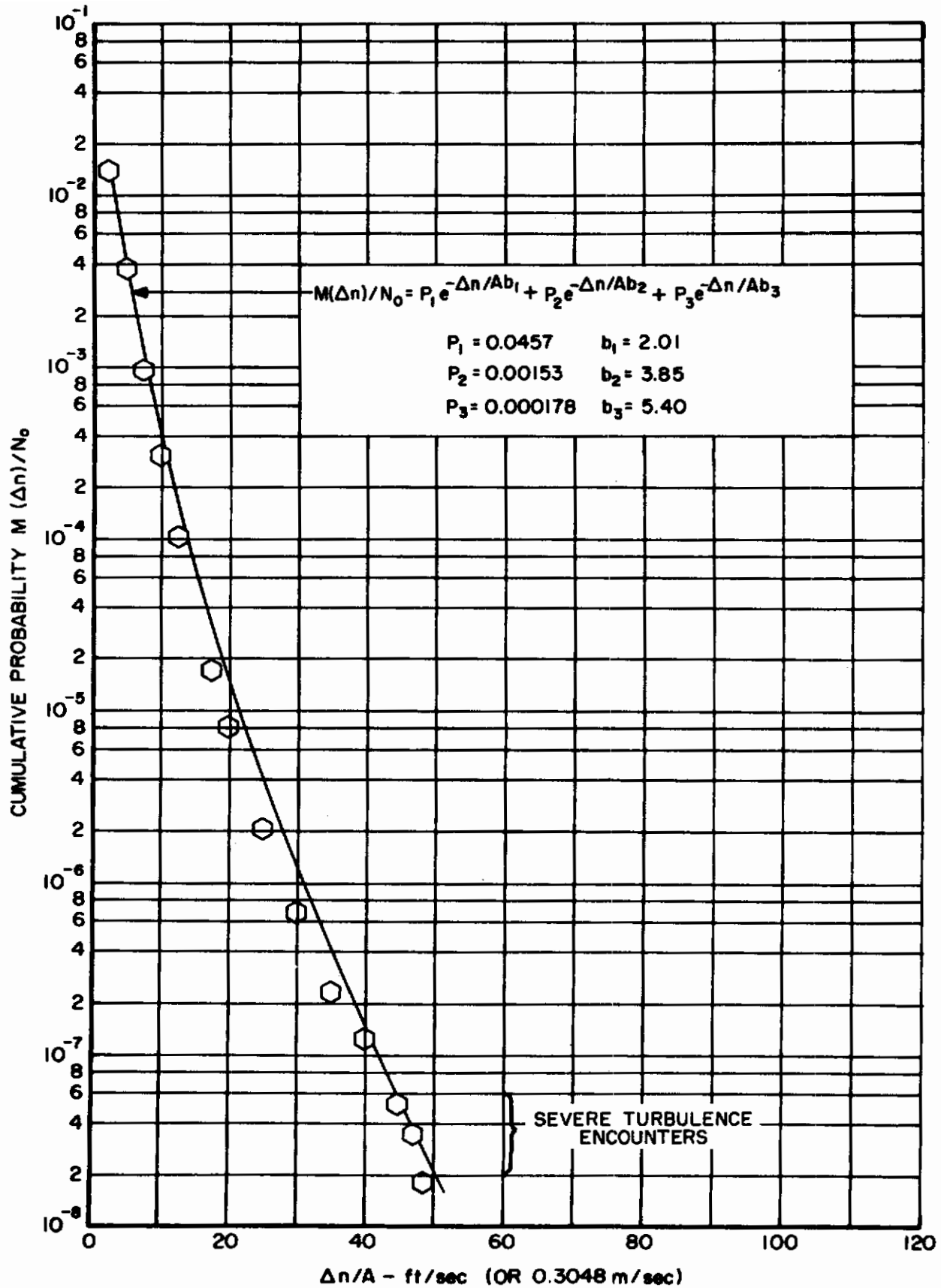
Figure 12 Combined Vertical Turbulence Environment and Severe Turbulence Encounters Altitude Range 30,000 - 40,000 feet (9,144 - 12,192 meters)
