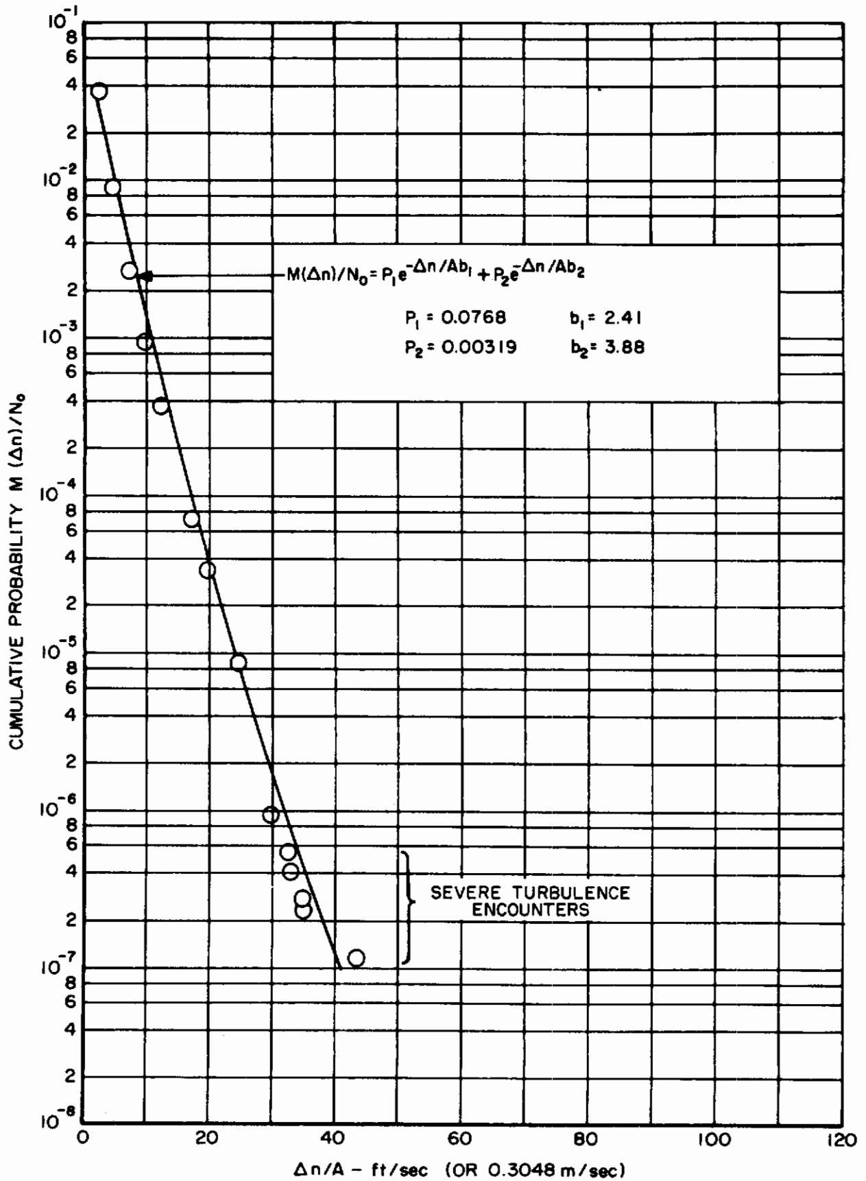
Figure 10 Combined Vertical Turbulence Environment and Severe Turbulence Encounter Altitude Range 10,000 - 20,000 feet (3,048 - 6,096 meters)
