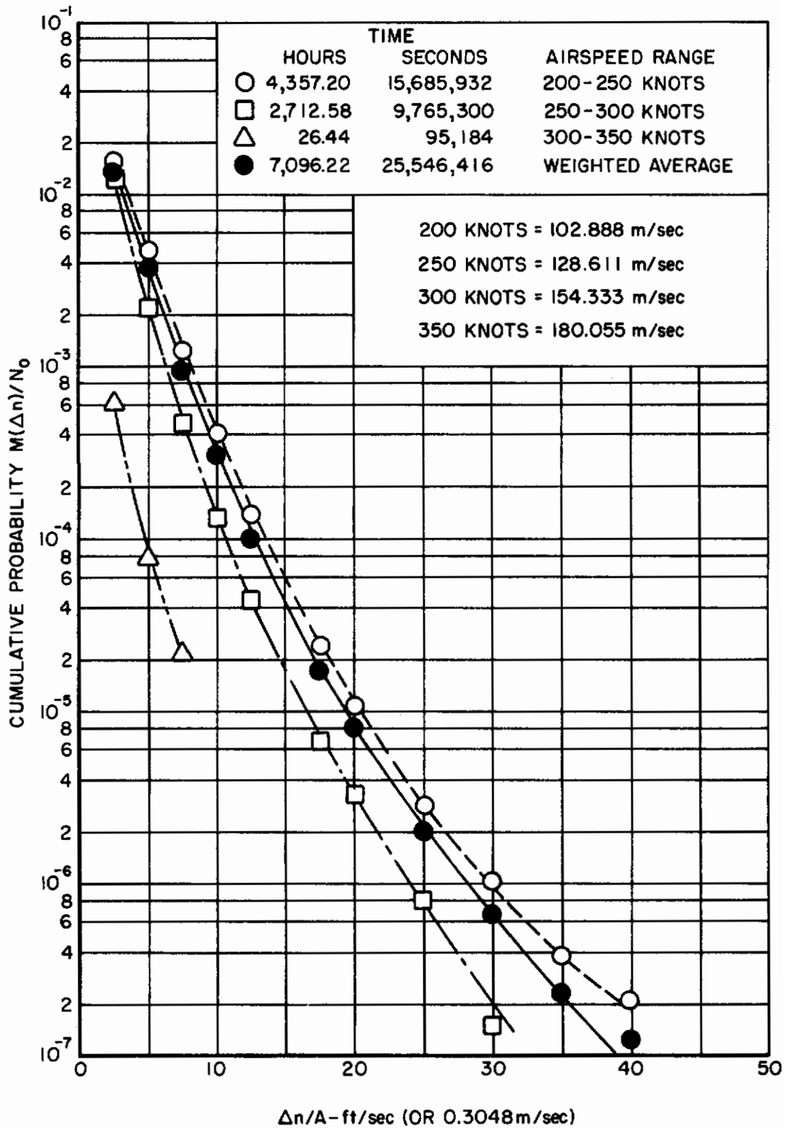
Figure 6 Vertical Turbulence Environment by Airspeed Altitude 30,000 - 40,000 feet (9,144 - 12,192 meters)
