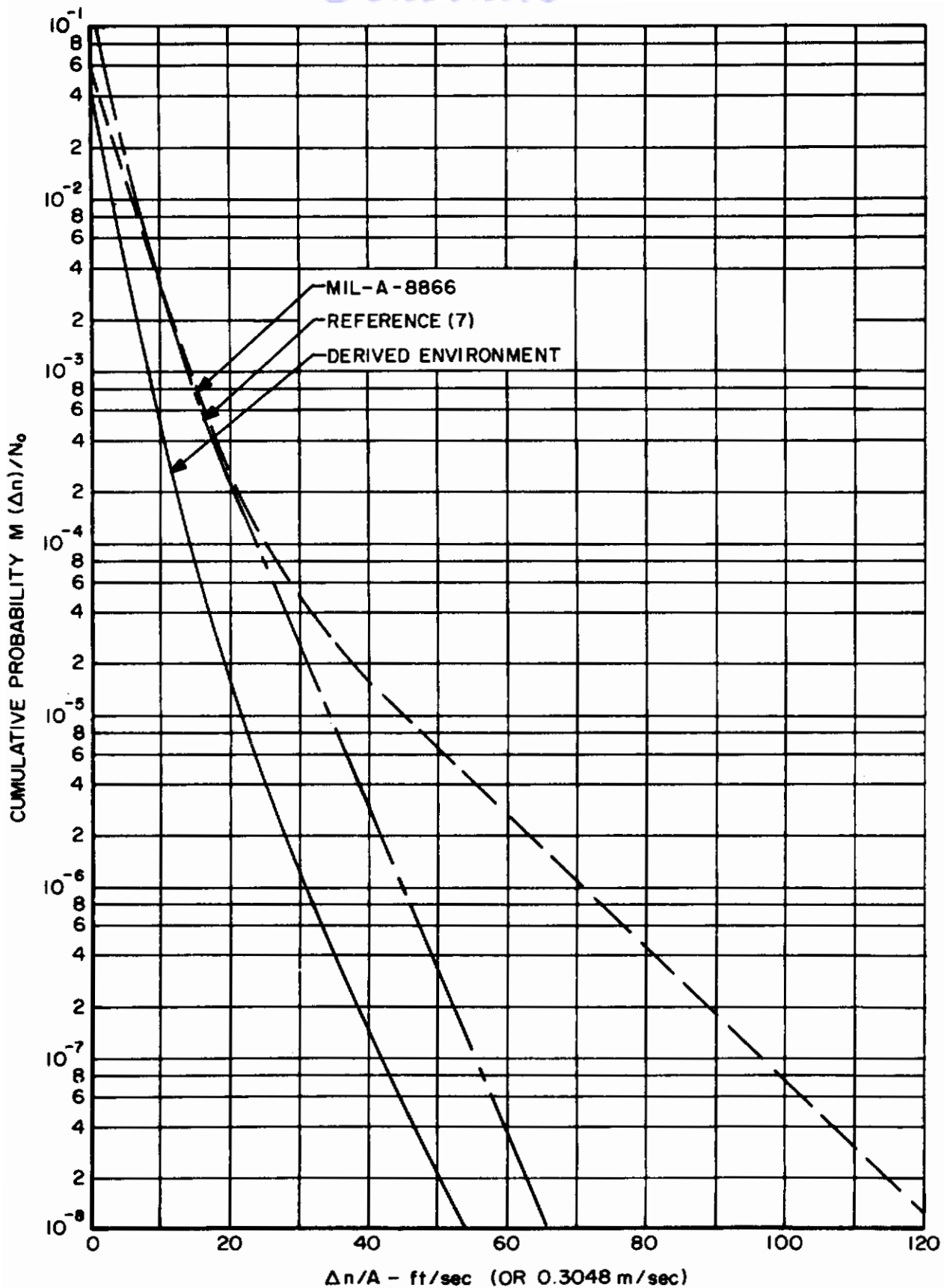
Figure 17 Comparison of Derived Vertical Turbulence Environments Altitude Range 30,000 - 40,000 feet (9,144 - 12,192 meters)
