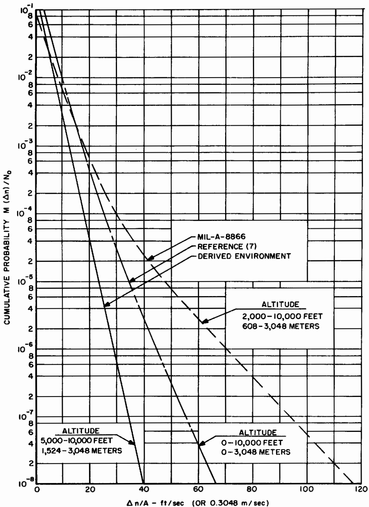
Figure 14 Comparison of Derived Vertical Turbulence Environments For Altitude Ranges Indicated
