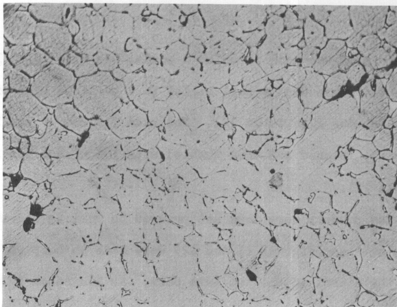
FIG. 12 ALK. SODIUM PICRATE ELECTROLYTIC ETCH 500X TiC LEACHED AND TUMBLED WITH 10% Ni
