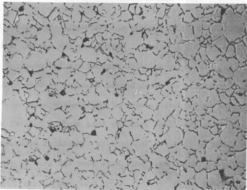
FIG 11 ALK. SODIUM PICRATE ELECTROLYTIC ETCH 500X TiC BALL MILLED WITH 10% Ni
