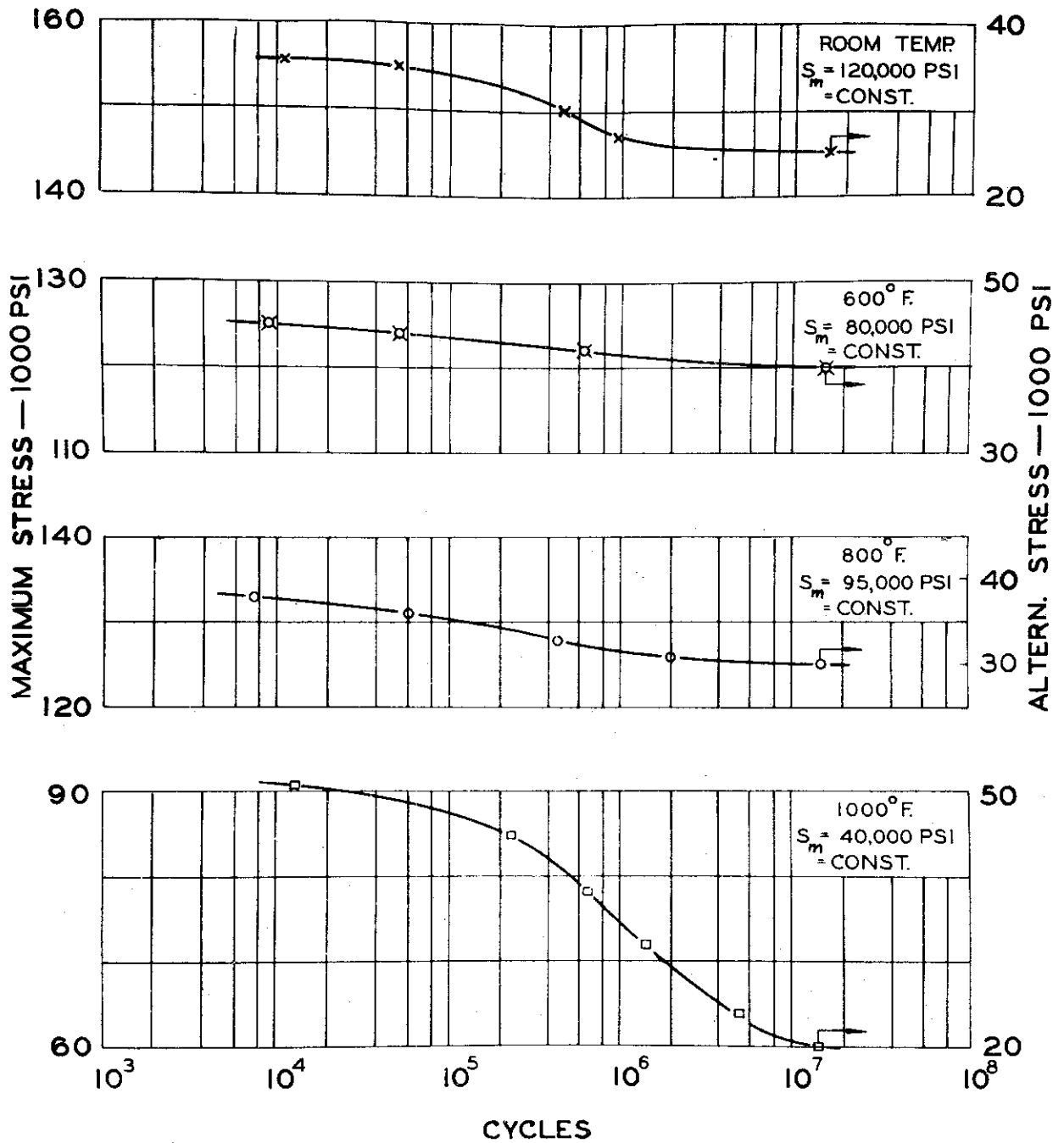
FIG. 8. S-N DIAGRAMS FOR HIGHER MEAN STRESSES, FOR ROOM AND ELEVATED TEMPERATURES, UNNOTCHED
