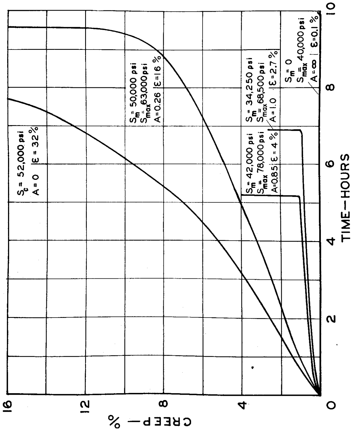
FIG. 37. CREEP TIME DIAGRAMS, EFFECT OF MEAN STRESS ON CREEP AT 1000° F., UNNOTCHED
