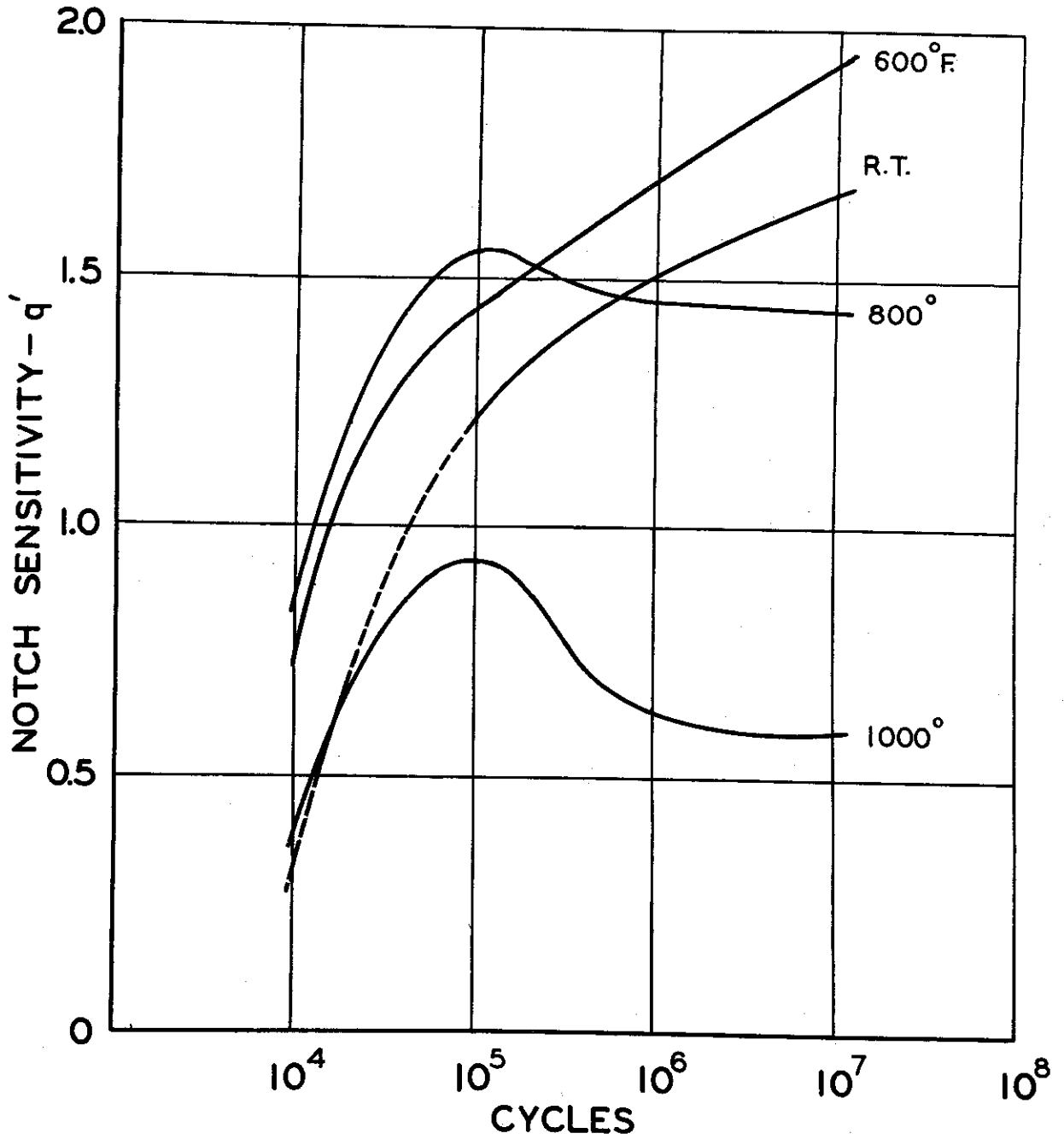
FIG. 34. FATIGUE NOTCH SENSITIVITY AS FUNCTION OF LIFE FOR ROOM AND ELEVATED TEMPERATURES, COMPLETELY REVERSED
