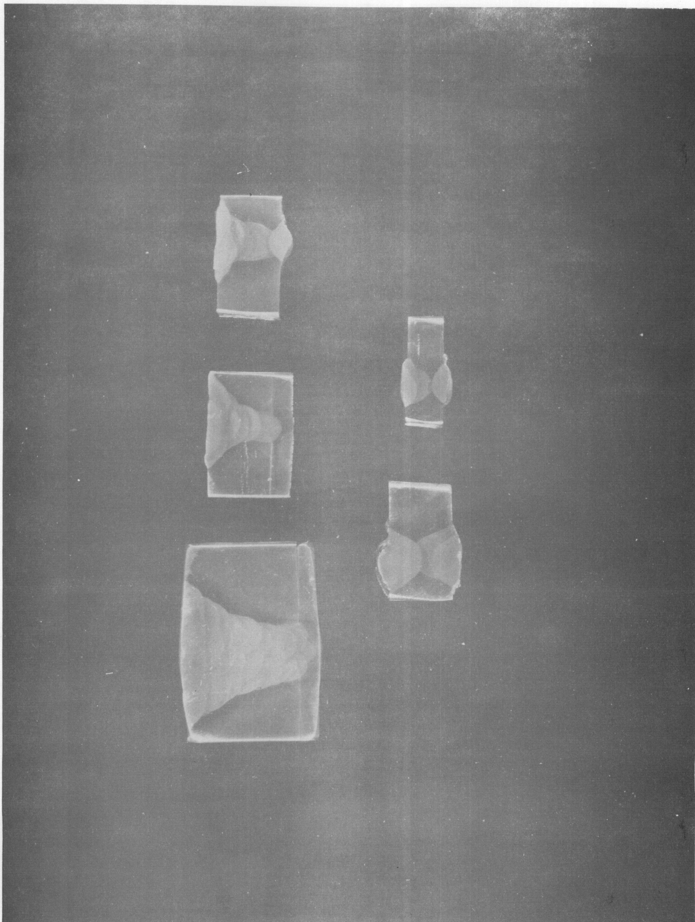
Figure 3. Appearance of Butt Weld Sections in HK31A Plate.
