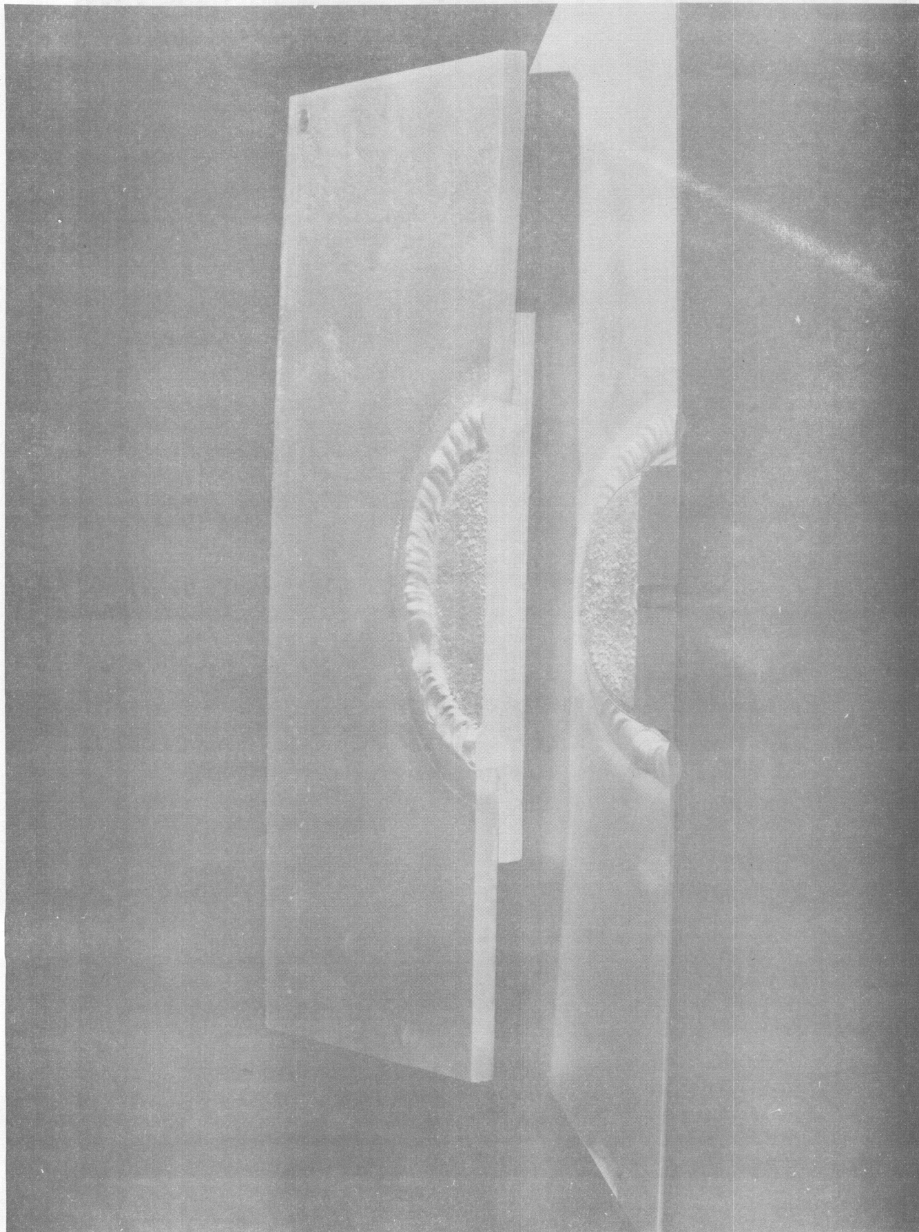
FIGURE 4. Circle Test Pieces of Cast Material Welded to Rolled Plate and Sheet.
