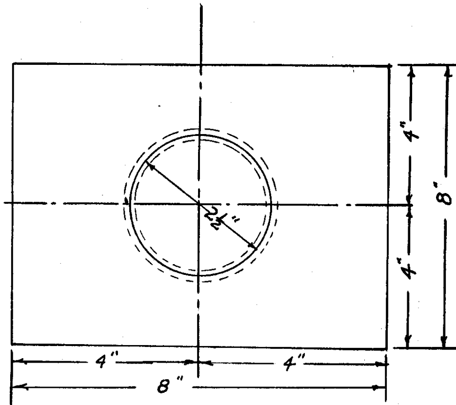
CIRCLE WELD - .064" SHEET
