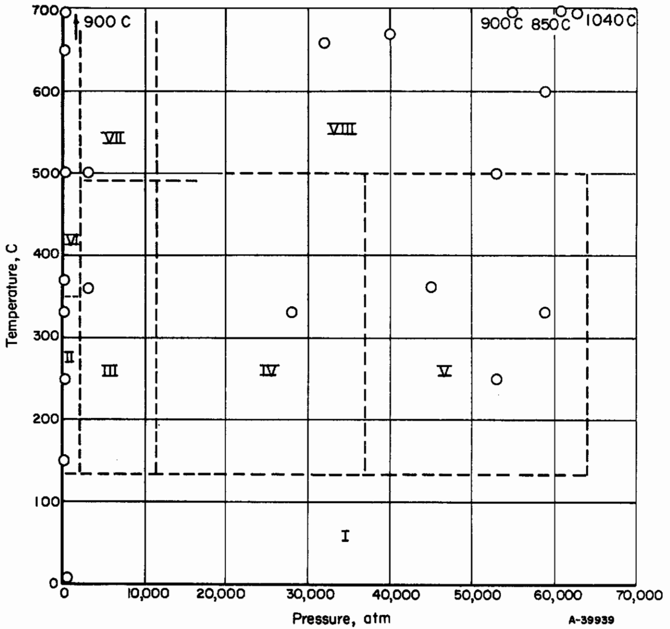
FIGURE 11. PILOT OF EXPERIMENTAL RUNS ON SILICOTUNGSTIC ACID
