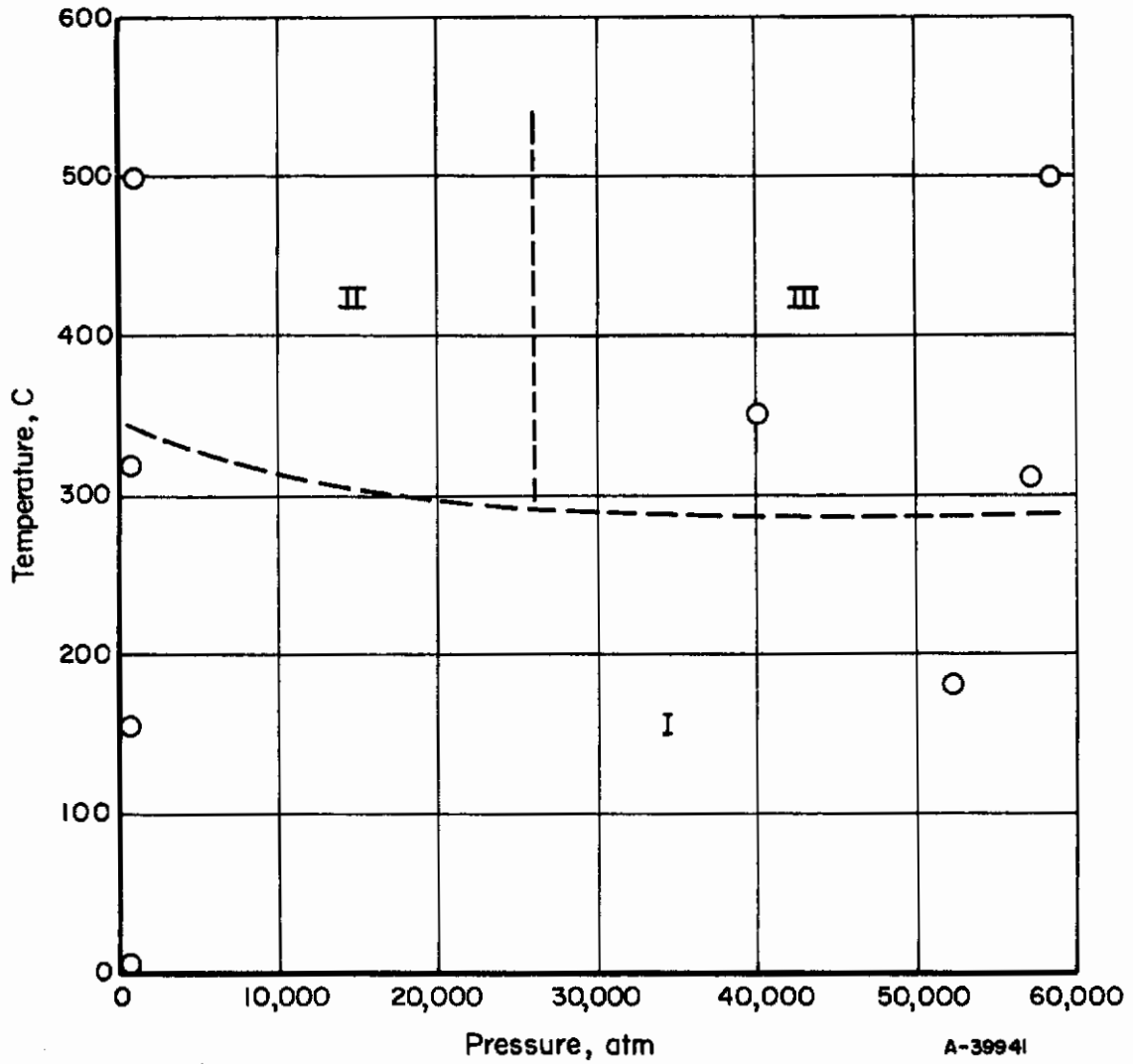
FIGURE 13. PLOT OF EXPERIMENTAL RUNS ON HYDRATED AMMONIUM-ARSENO-VANADO-TUNGSTATE
