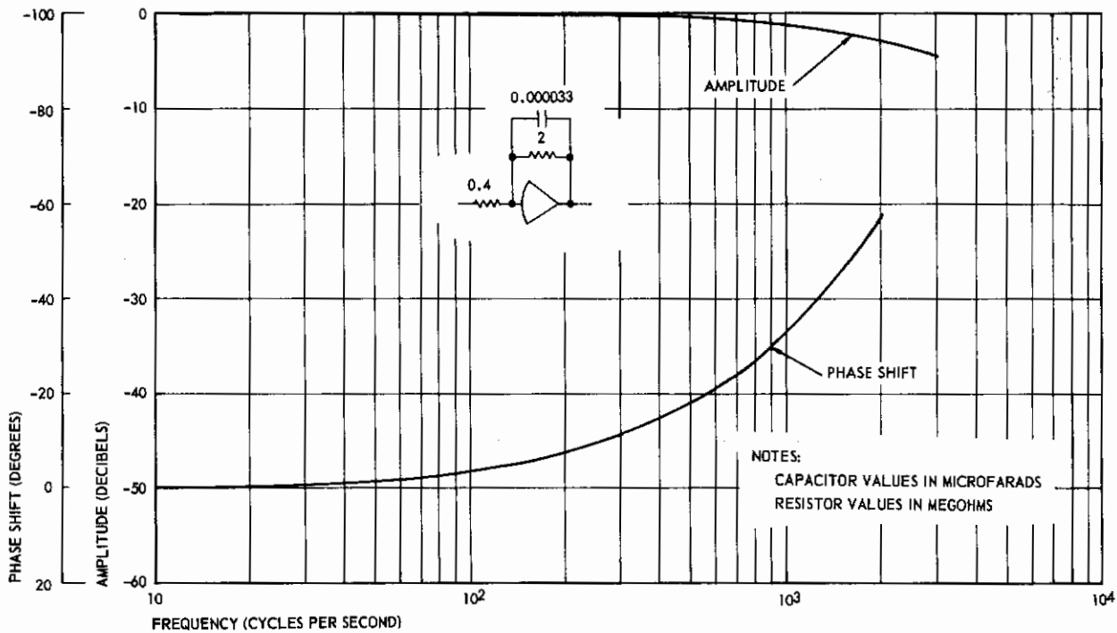
Figure 26 - Amplifier Characteristics
