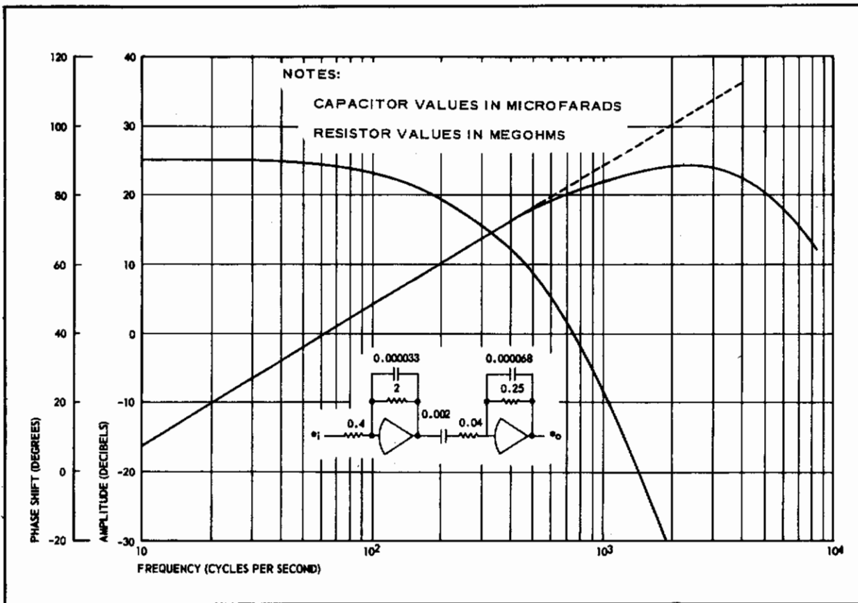
Figure 28 - Differentiator Characteristics
