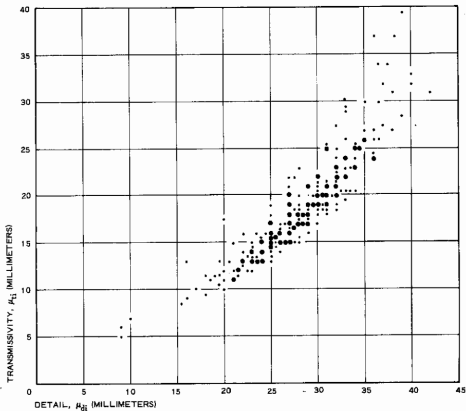
Figure 12 - Scatter Diagram of Cell-by-Cell Transmissivity versus Detail (Original Radar Plate 17)
