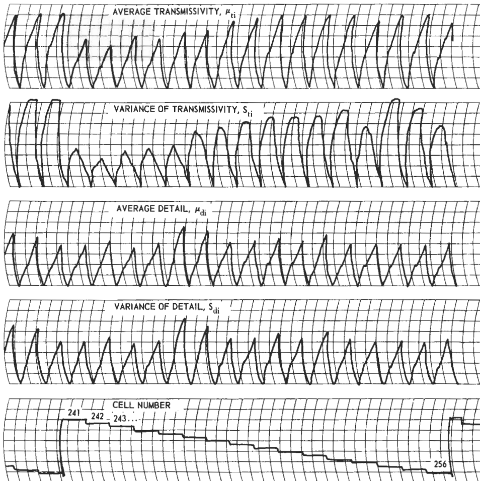
Figure 9 - Illustrative Analog Computer Outputs
