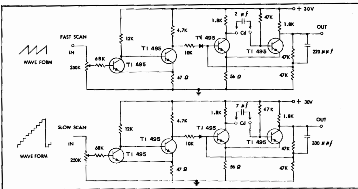
Figure 22 - Blanking Circuit
