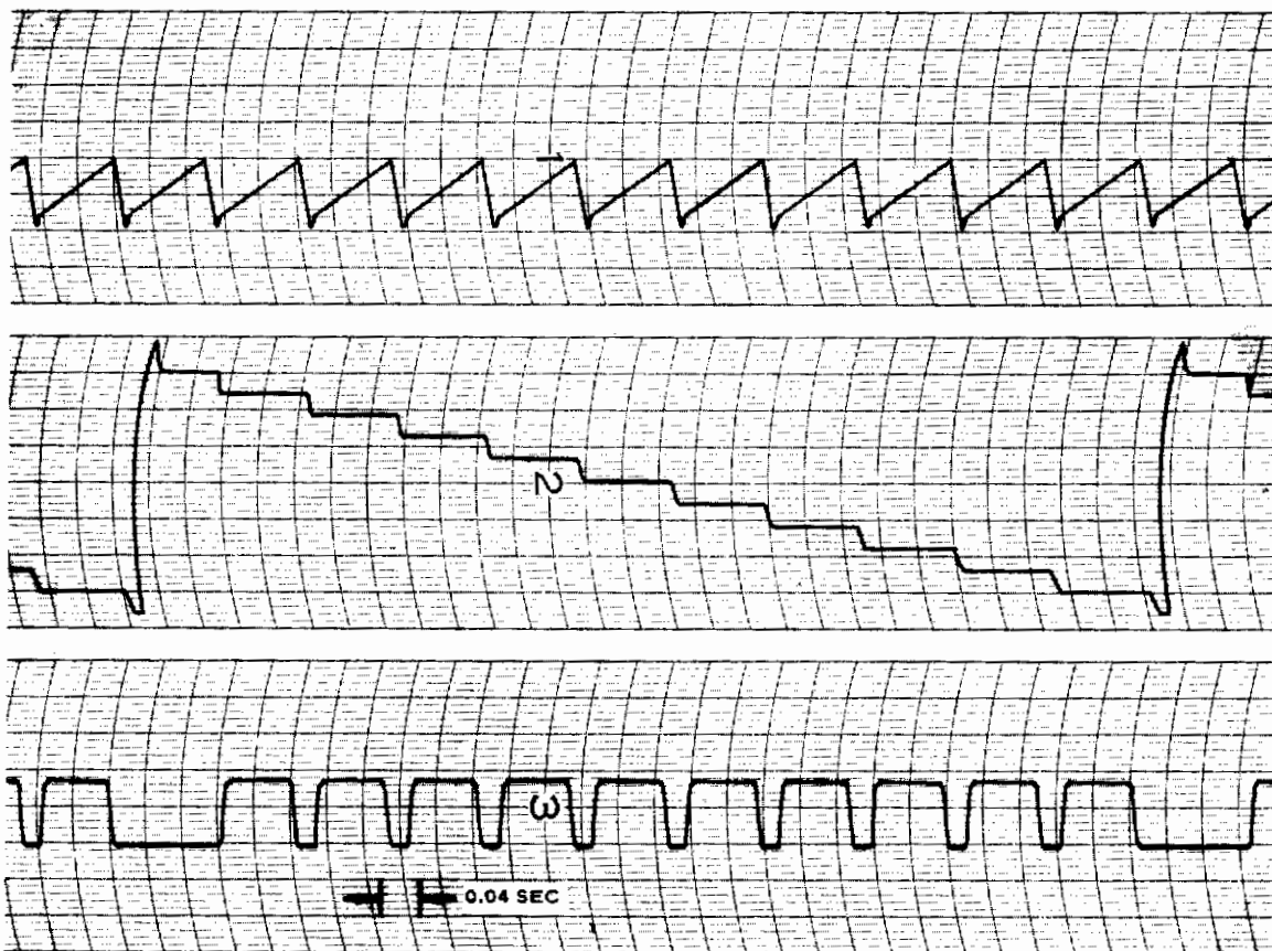
Figure 21 - Fast Scan Patterns
