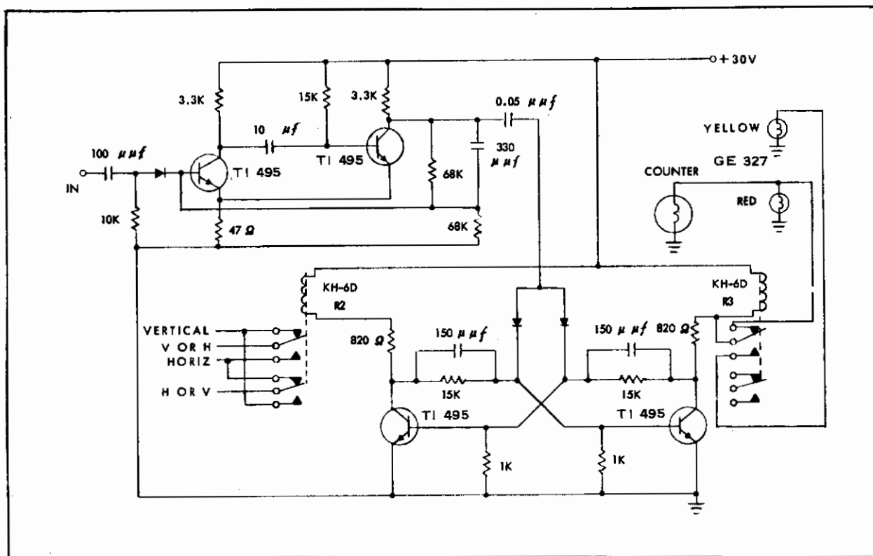
Figure 24 - Alternator Circuit
