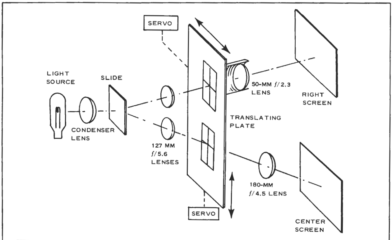
Figure 2 - Schematic of Projector-Viewer Center and Right-Hand Channels
