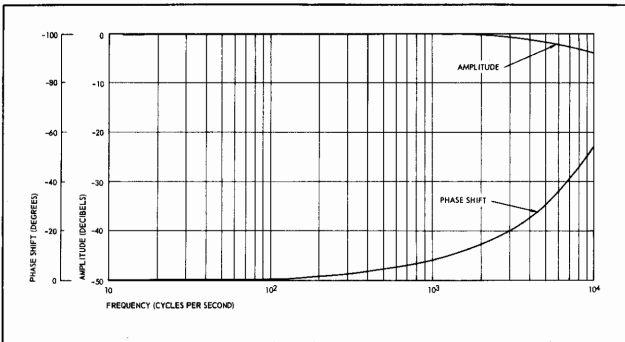
Figure 29 - Photomultiplier Amplifier Characteristics
