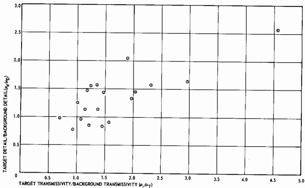
Figure 13 - Scatter Diagram of Transmissivity and Detail Ratios, Immediate Background, Original Radar Plates at Large Scale
