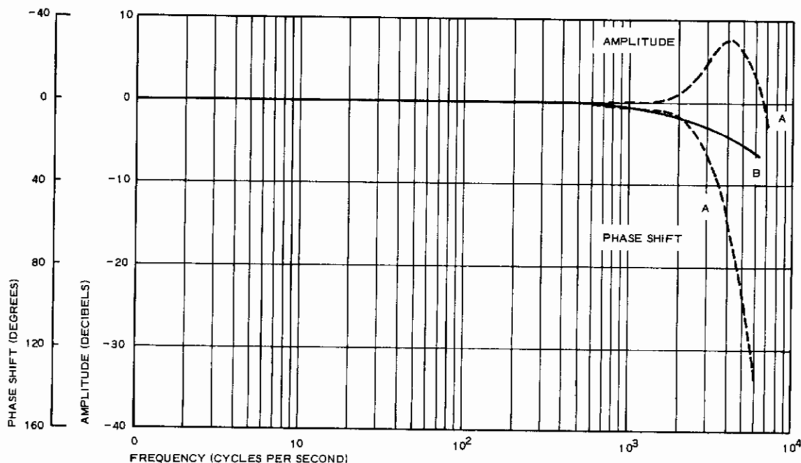
Figure 27 - Multiplier Frequency and Phase Characteristics
