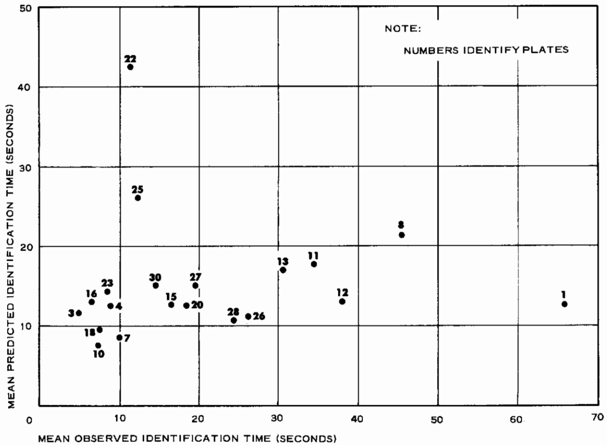
Figure 15 - Scatter Diagram of Metric I Predictions Applied to Original Radar Plates
