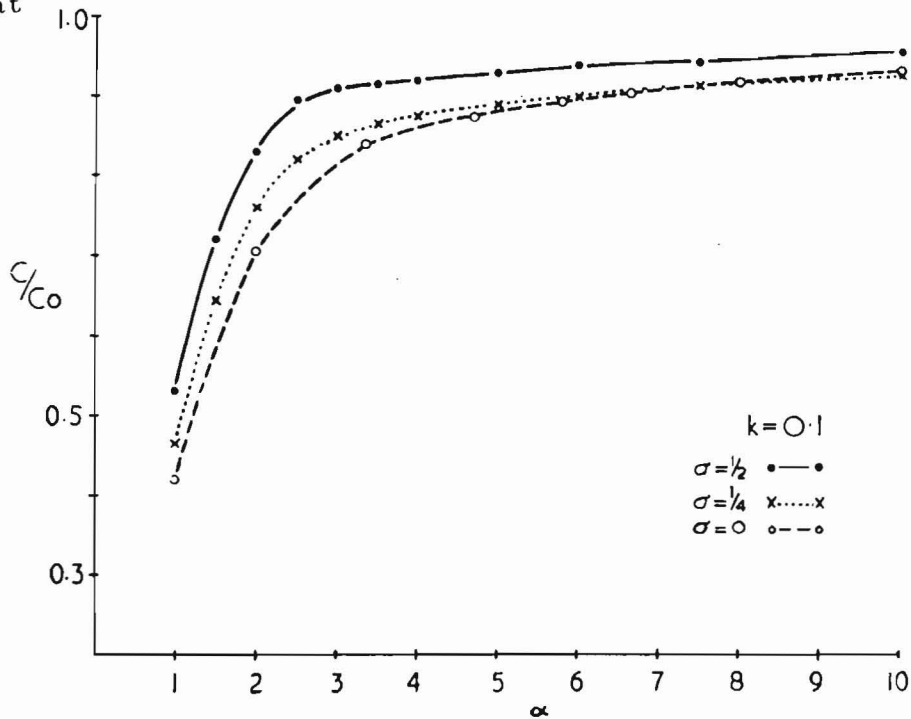
Fig.8 Ratio of wave-velocity to that for an inviscid fluid as a function of \alpha , for a wall-thickness ratio of 0.1 and Poisson's Ratios of 0.5, 0.25, 0.
