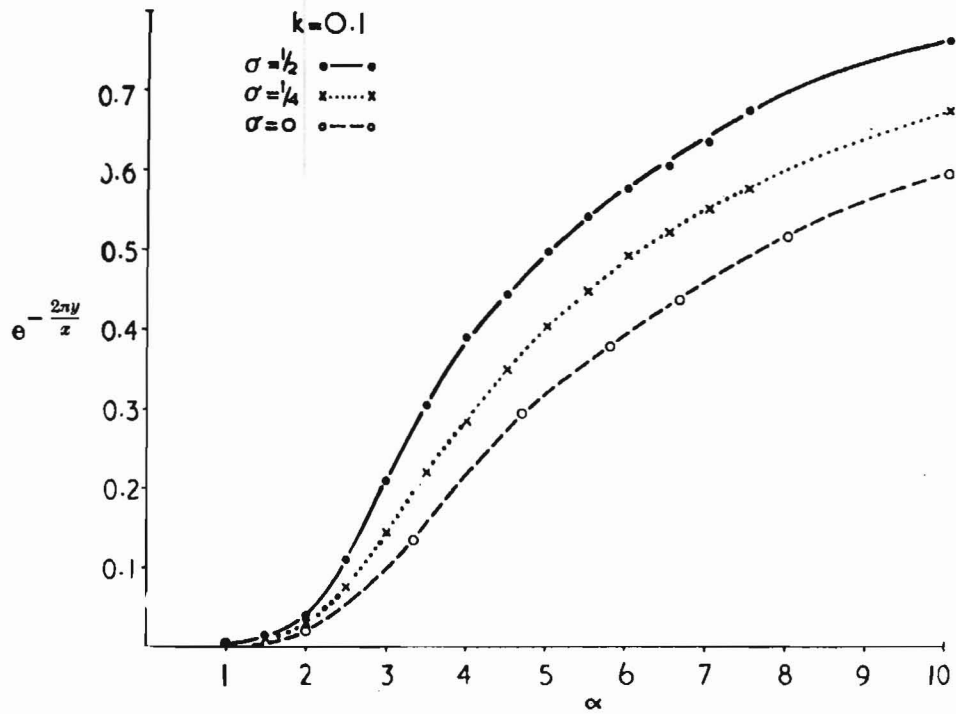
Fig. 9 Attenuation of wave amplitude over one wave-length as a function of \alpha , for the same conditions as Fig. 8.
