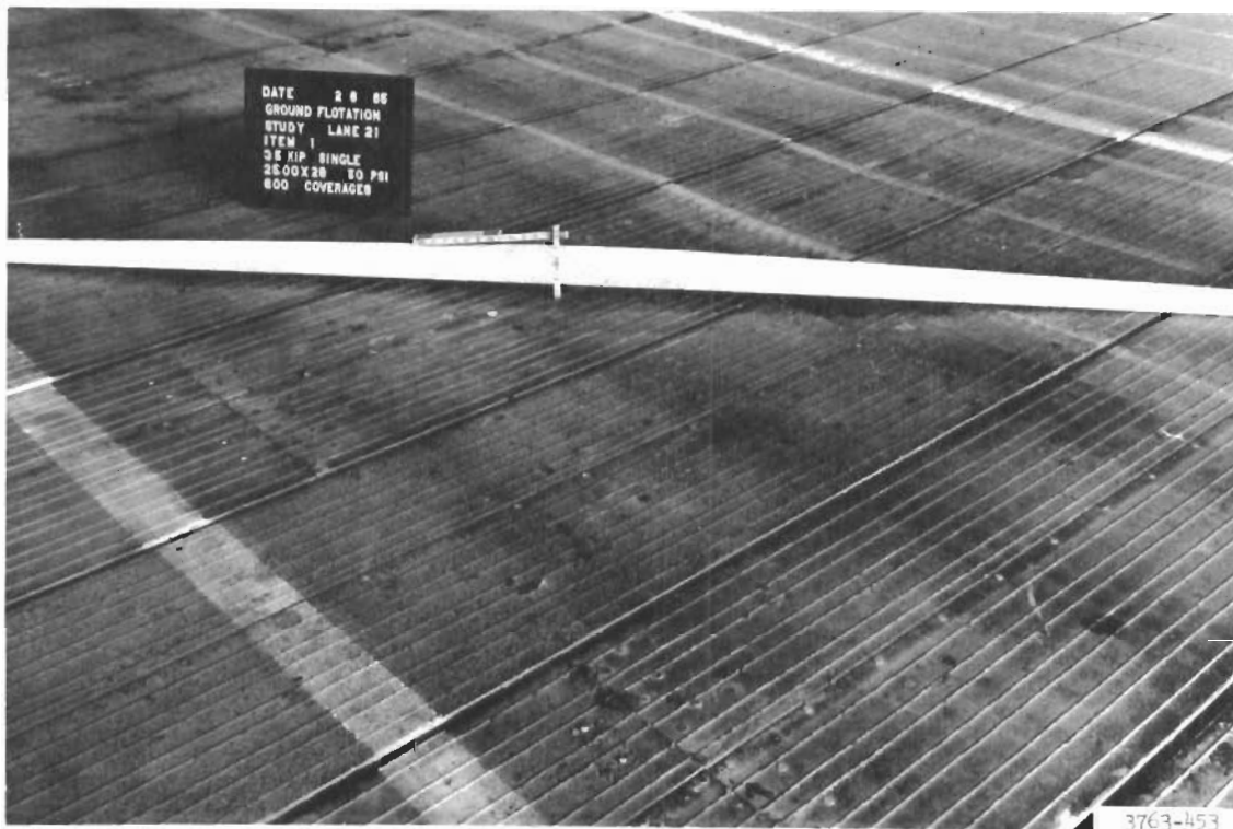
Figure 4. Lane 21, item 1. Diagonal straightedge shows small deformations existing at 600 coverages (traffic suspended)
