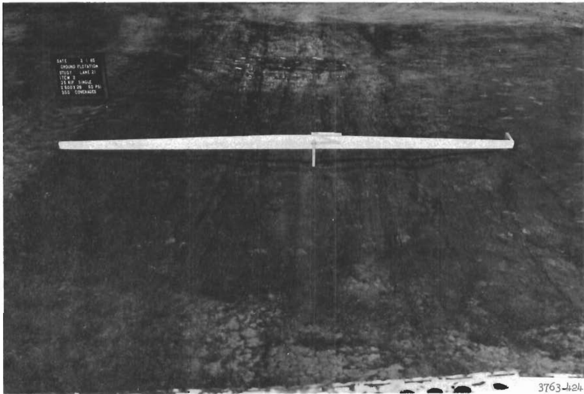
Figure 8. Lane 21, item 3. Transverse straightedge shows roughness at 300 coverages (failure)
