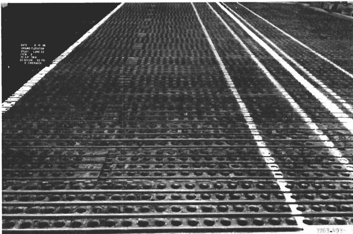
Figure 11. Lane 22, item 2, prior to traffic
