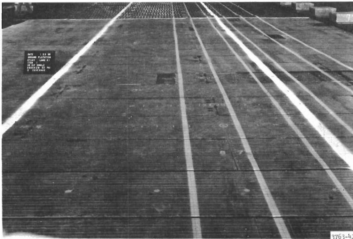
Figure 3. Lane 21, item 1, prior to traffic
