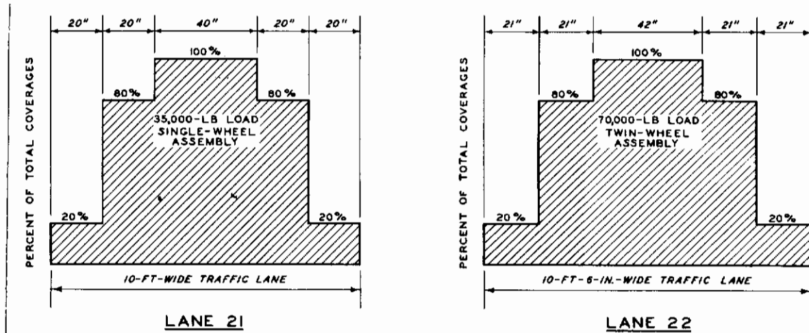
Figure 1. Traffic distribution patterns, Test Section 9
