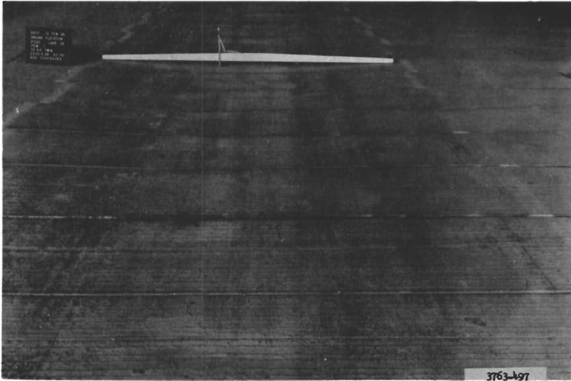
Figure 10. Lane 22, item 1. Transverse straightedge shows roughness at 400 coverages (failure)
