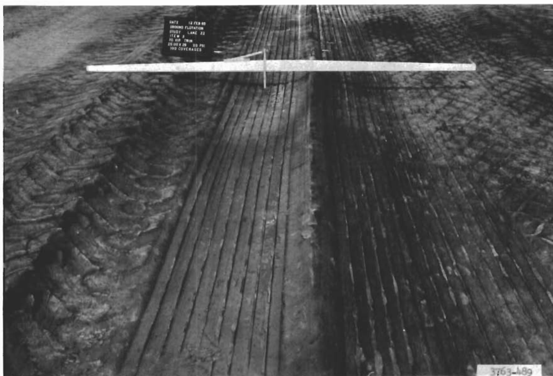
Figure 14. Lane 22, item 3. Transverse straightedge shows roughness at 100 coverages (failure)
