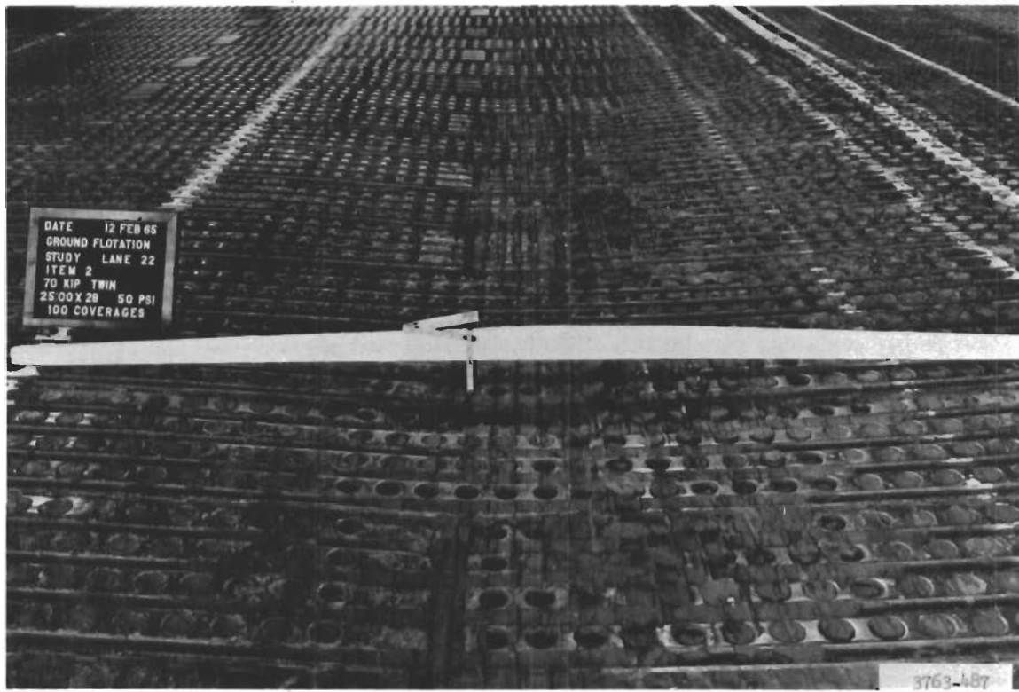
Figure 12. Lane 22, item 2. Transverse straightedge shows roughness at 100 coverages (failure)
