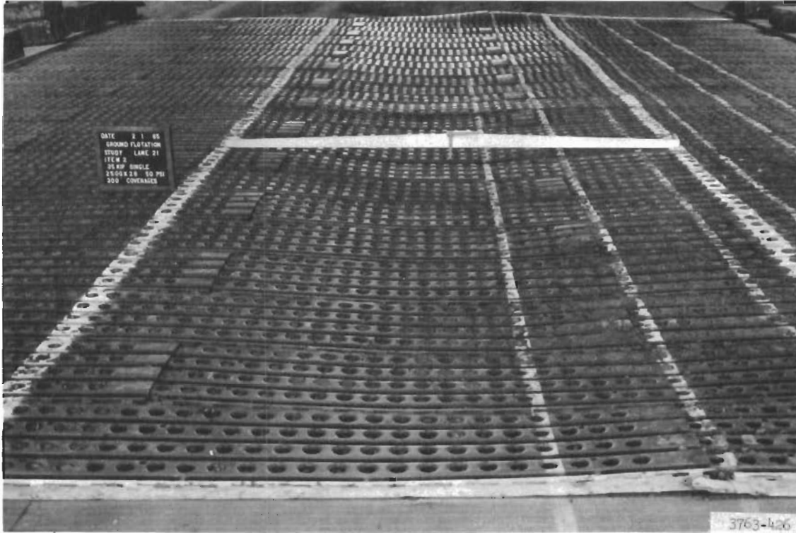
Figure 6. Lane 21, item 2. Transverse straightedge shows roughness at 300 coverages (failure)
