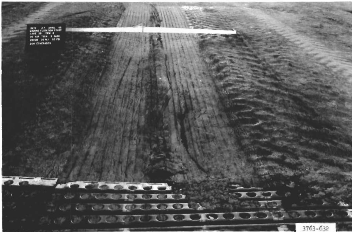
Figure 14. Lane 29, item 3, after 200 coverages of traffic (failure)
