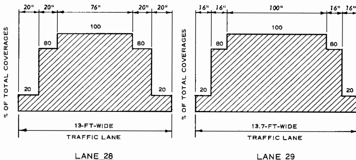
Figure 1. Traffic distribution patterns on Test Section 13
