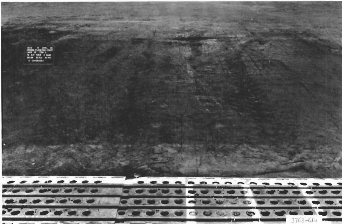
Figure 13. Lane 29, item 3, prior to traffic
