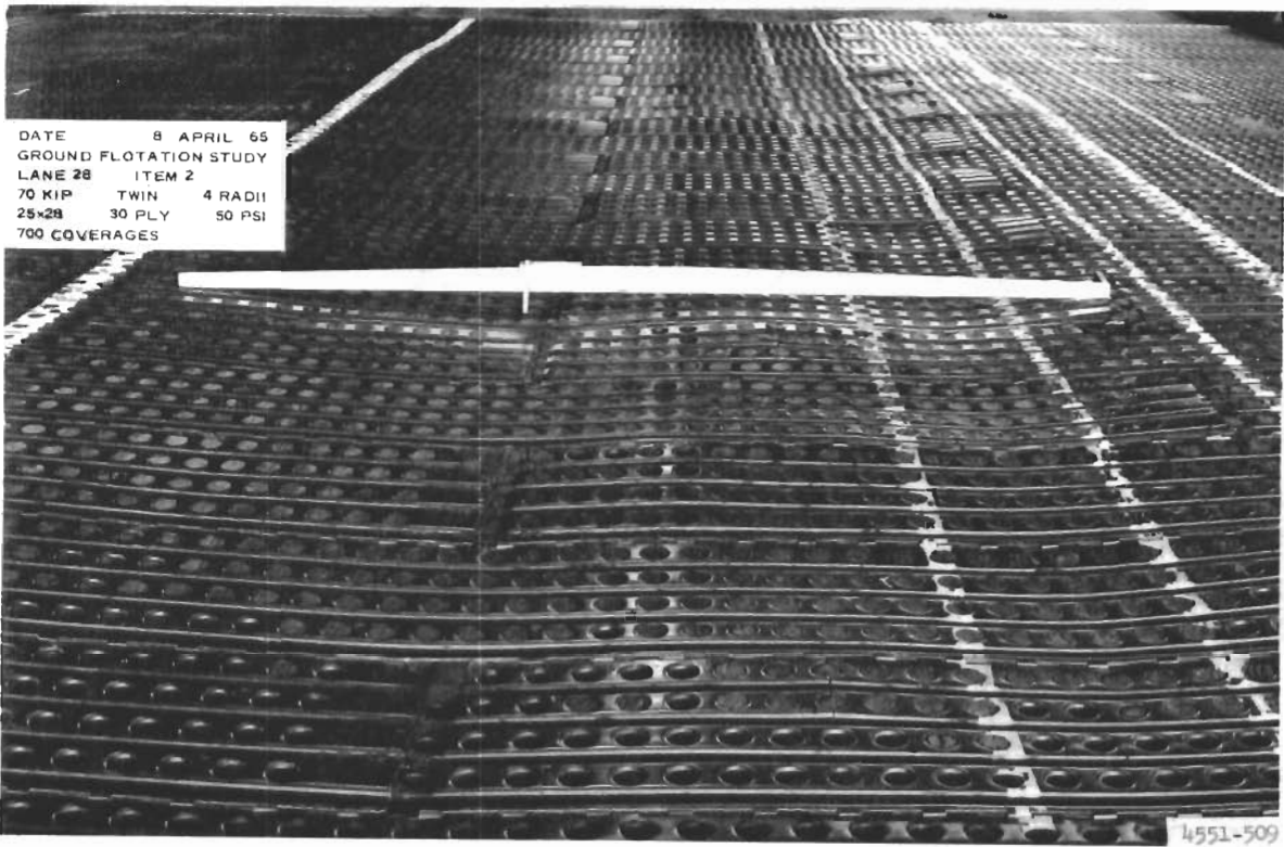
Figure 6. Lane 28, item 2, after 700 coverages of traffic (failure)
