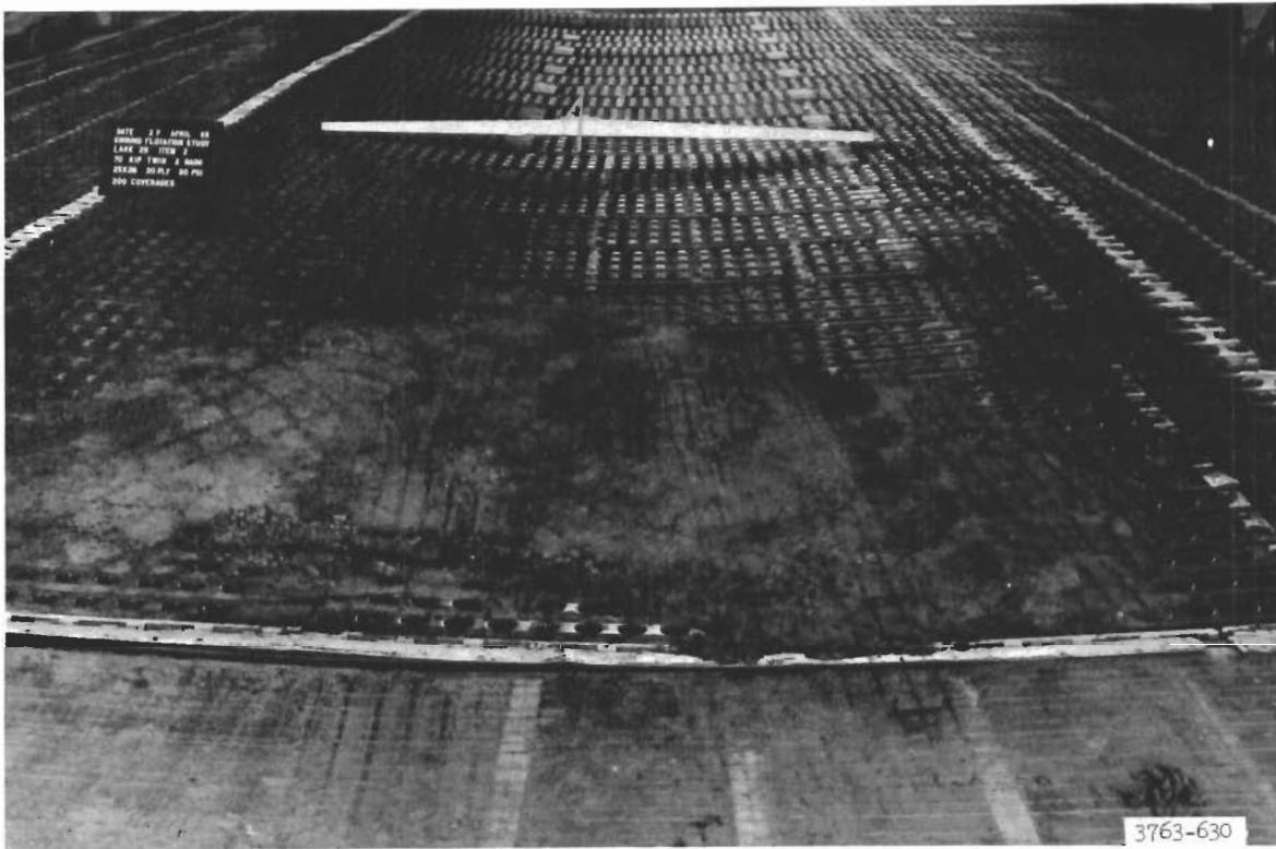
Figure 12. Lane 29, item 2, after 200 coverages of traffic (failure)
