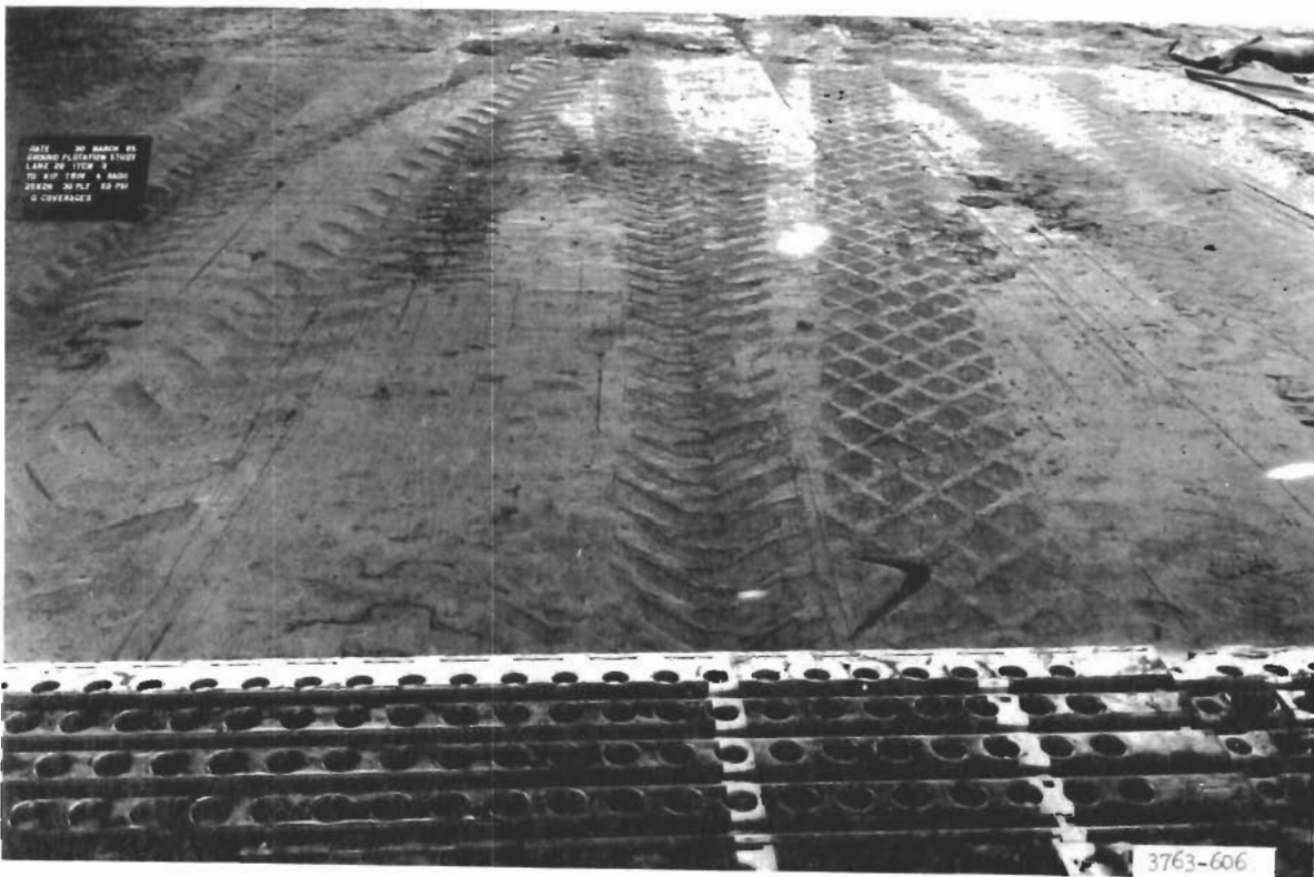
Figure 7. Lane 28, item 3, prior to traffic
