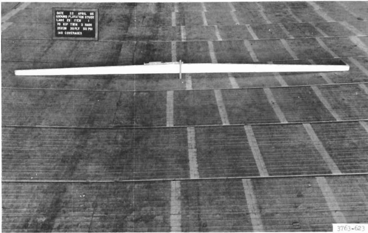
Figure 10. Lane 29, item 1, after 140 coverages of traffic (failure)
