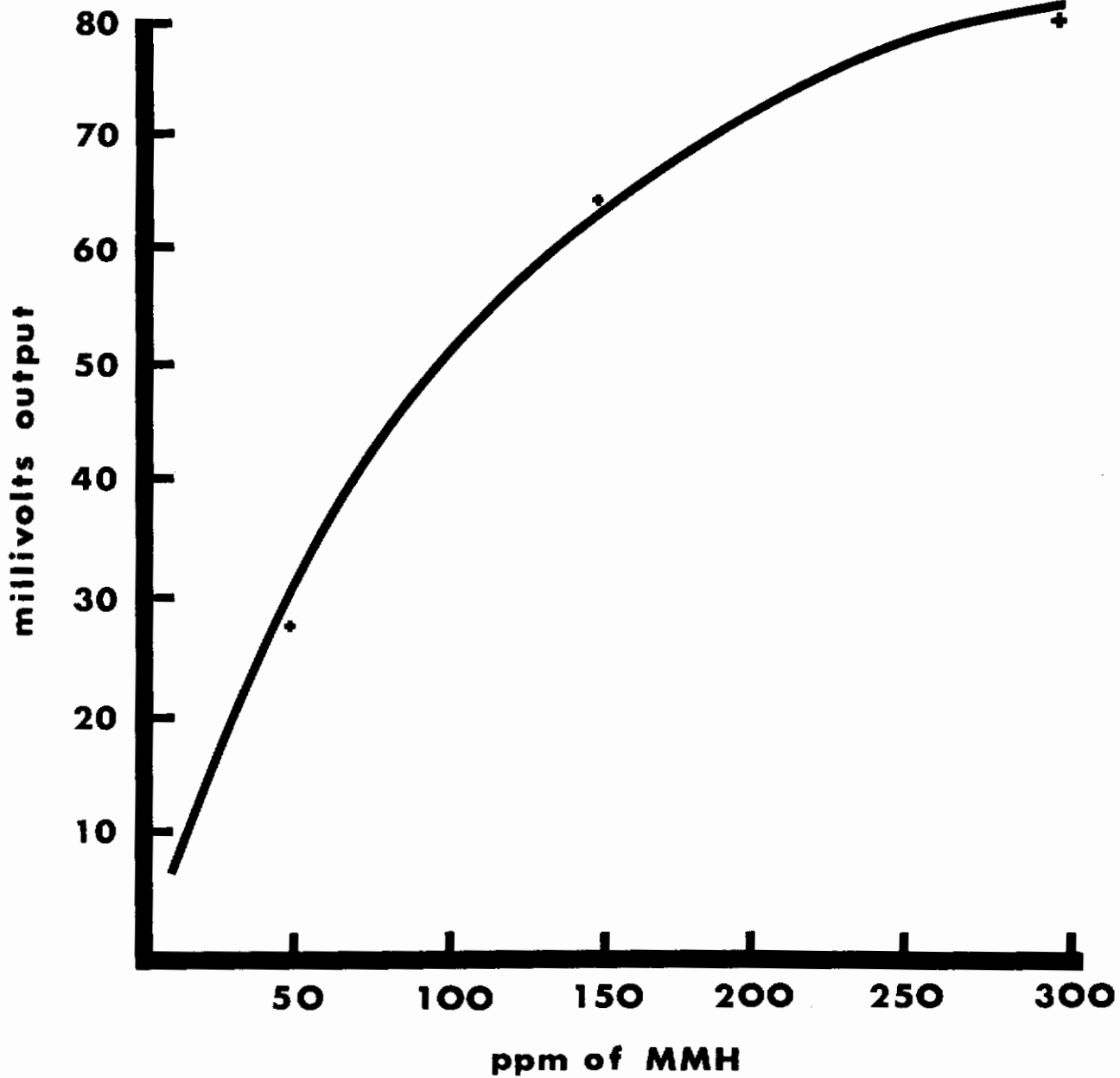
Figure 5. Monomethylhydrazine Standard Calibration Curve
