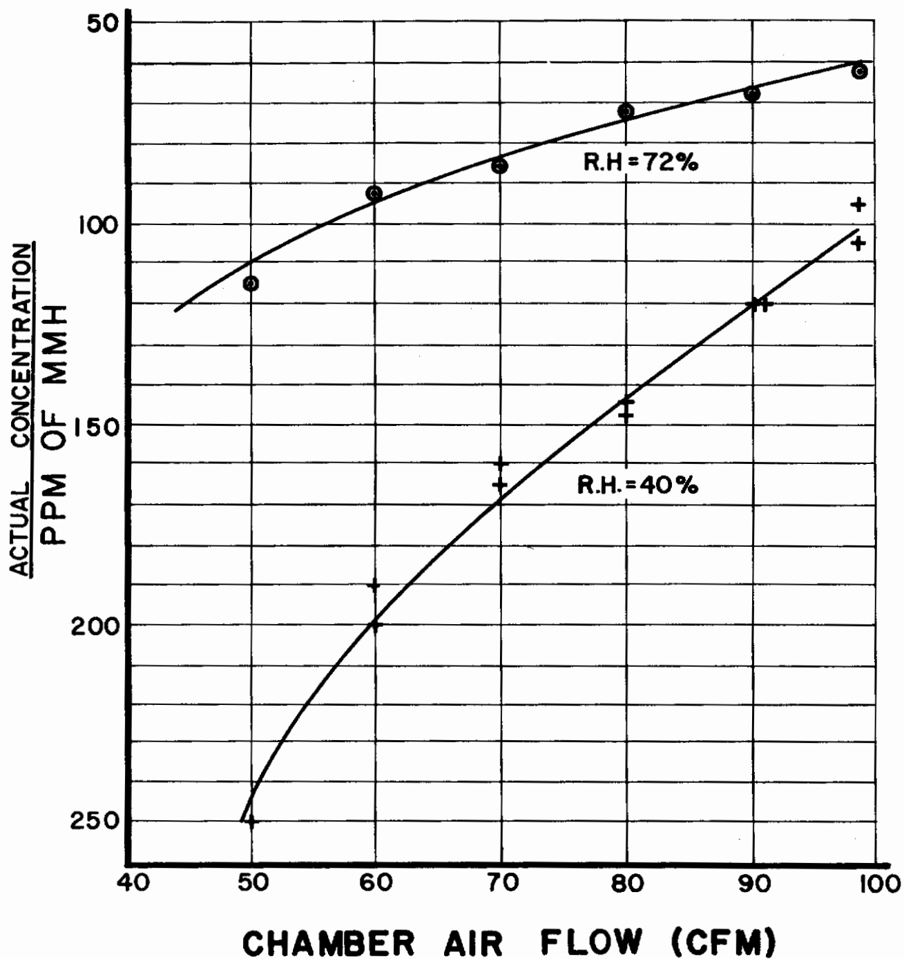
Figure 6. Effect of Relative Humidity on MMH Concentration
