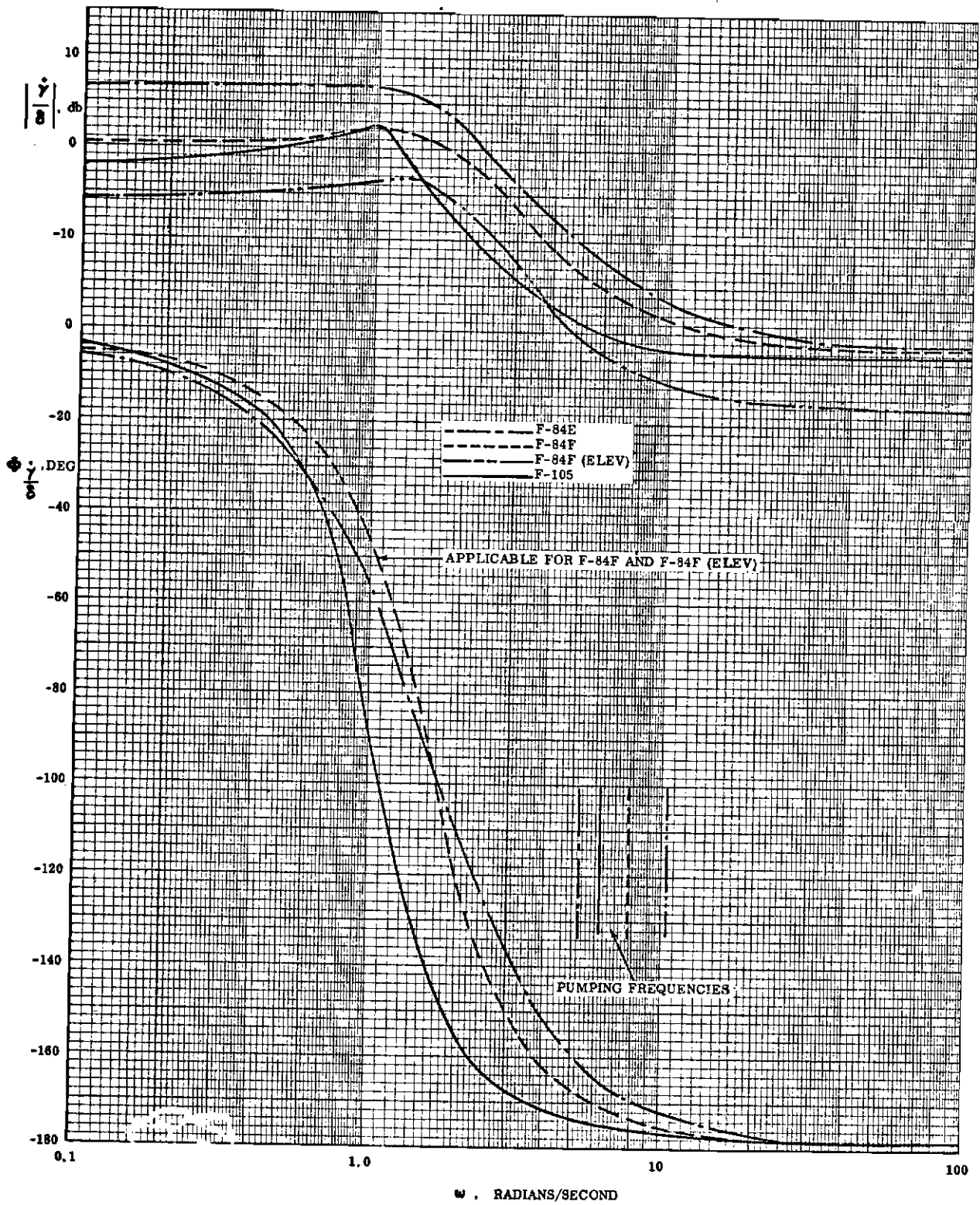
FIG. A-4 FREQUENCY RESPONSE IN RATE OF CHANGE OF FLIGHT PATH ANGLE FOR VARIOUS AIRCRAFT IN LANDING CONFIGURATION
