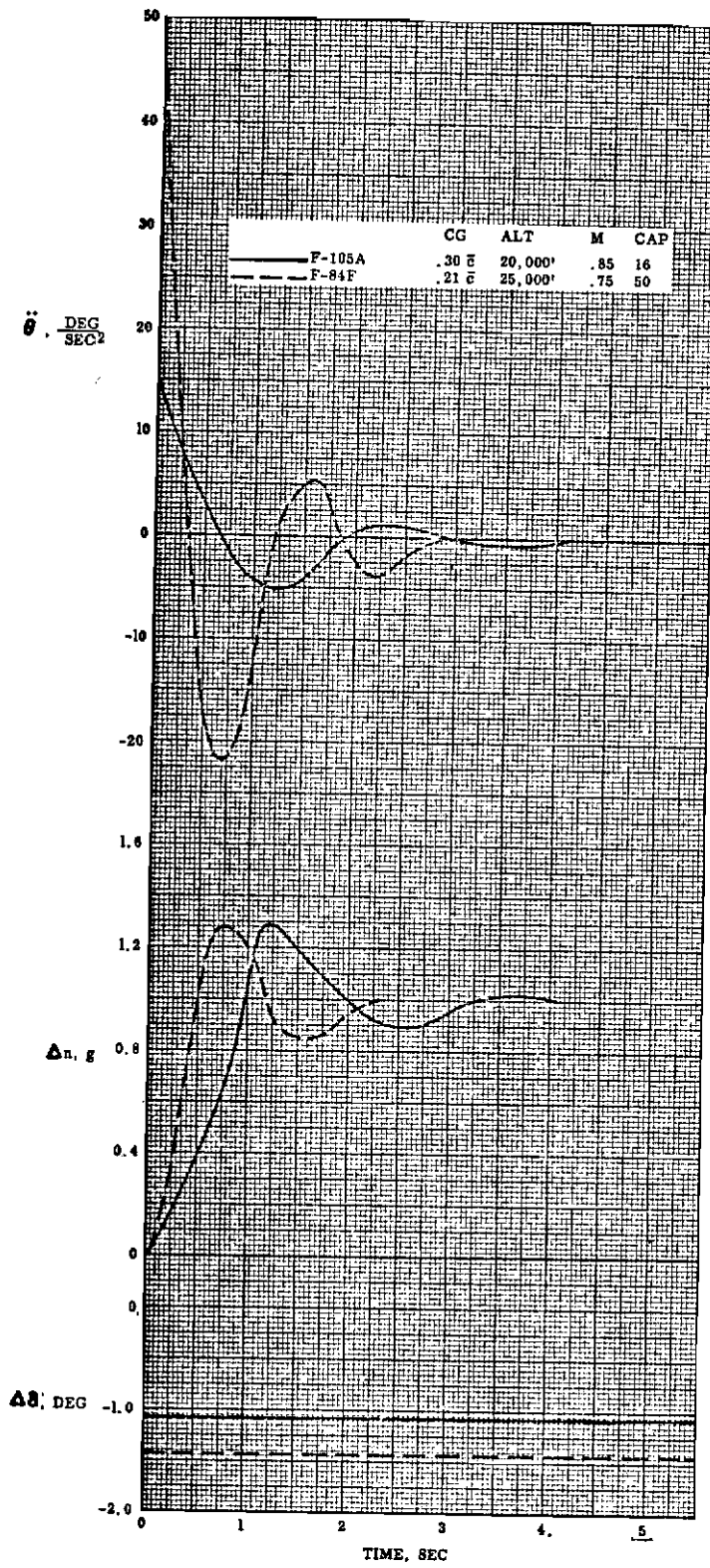
Fig. 1 A COMPARISON OF THE RESPONSE OF TWO AIRCRAFT
