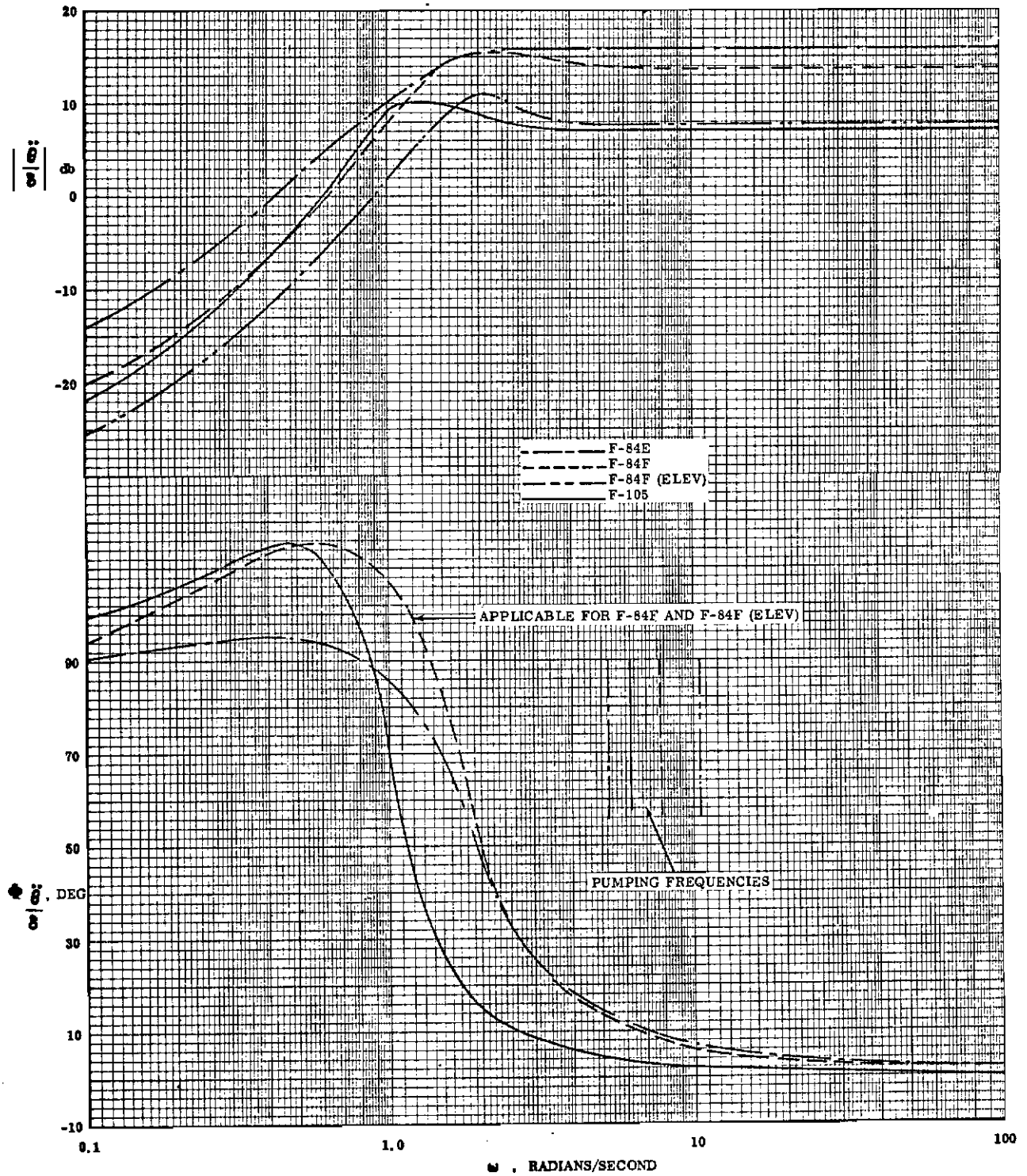
FIG. A-2 FREQUENCY RESPONSE IN ANGULAR ACCELERATION FOR VARIOUS AIRCRAFT IN THE LANDING CONFIGURATION
