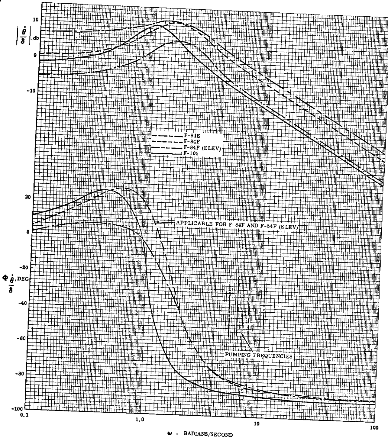
10. A-3 FREQUENCY RESPONSE IN ANGULAR VELOCITY FOR VARIOUS AIRCRAFT IN THE LANDING CONFIGURATION
