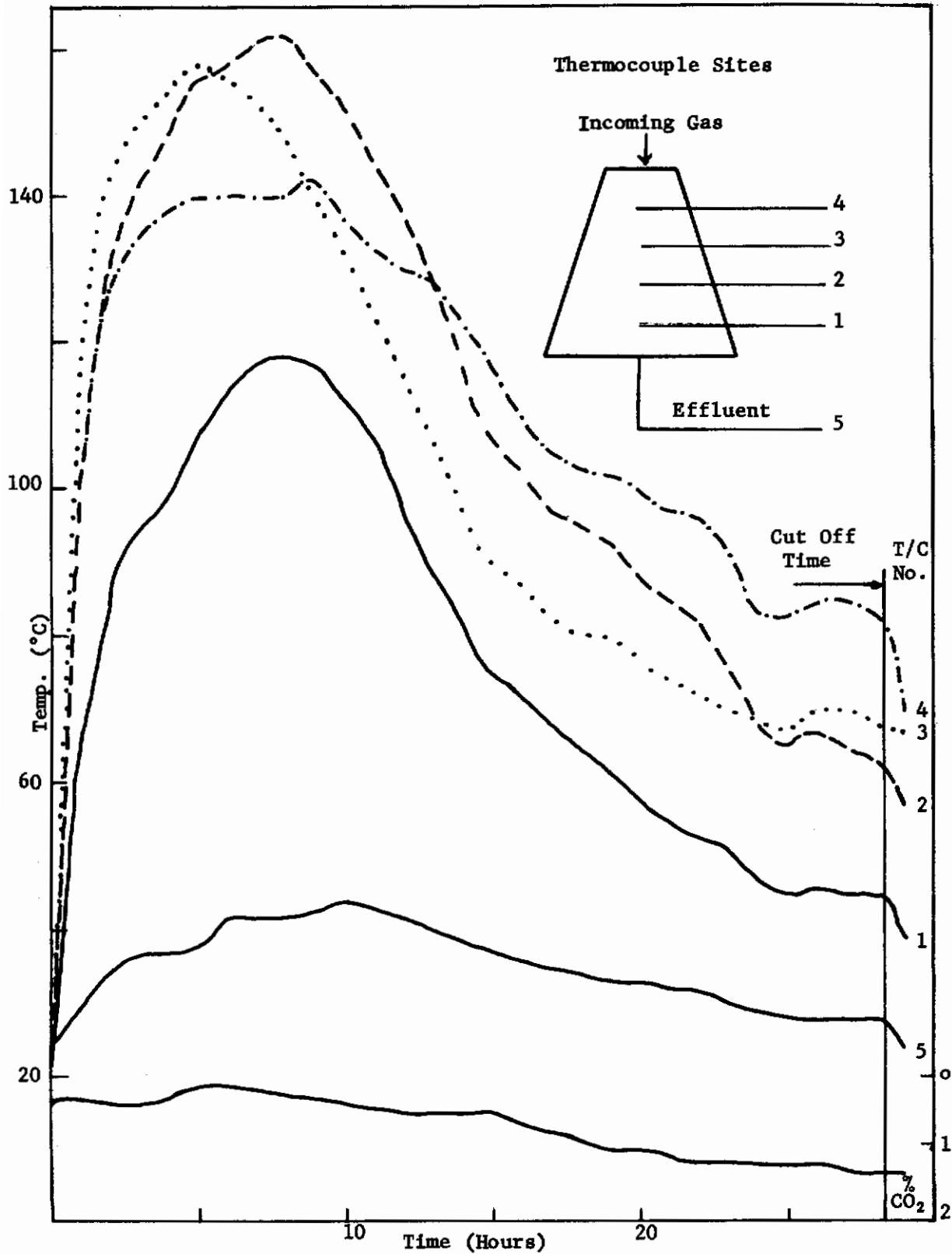
Figure 35 Profiles of Temperature and % CO 2 in Effluent in Test No. 2 of Prototype
