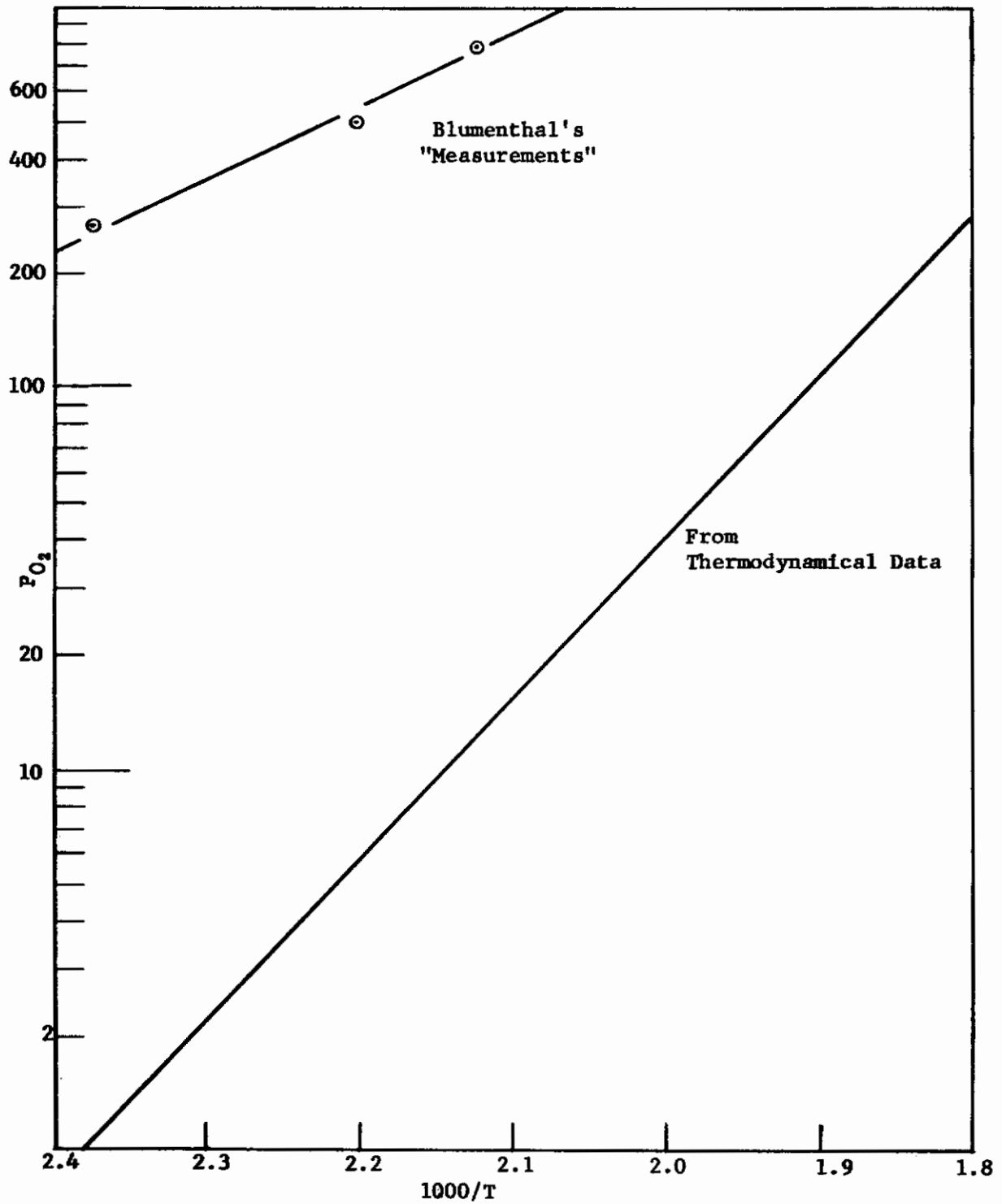
Figure 1 Oxygen Pressure of Lithium Peroxide
