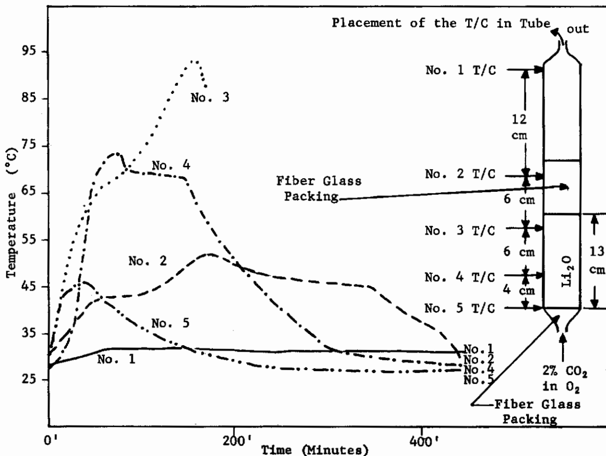
Figure No. 9 Temperature Profile of Test No. 4
