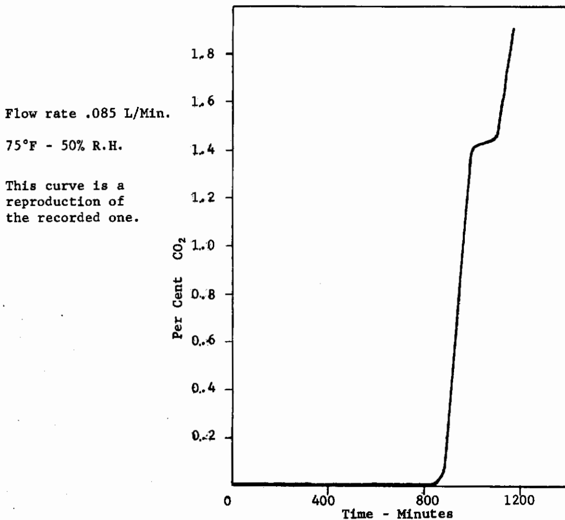
Figure 10 Absorption Curve of Run Number 12
