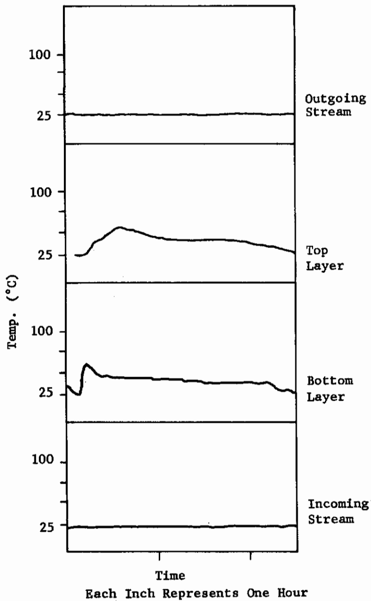
Figure 30 Temperature Profiles Taken At Different Sites During Test No. 45
