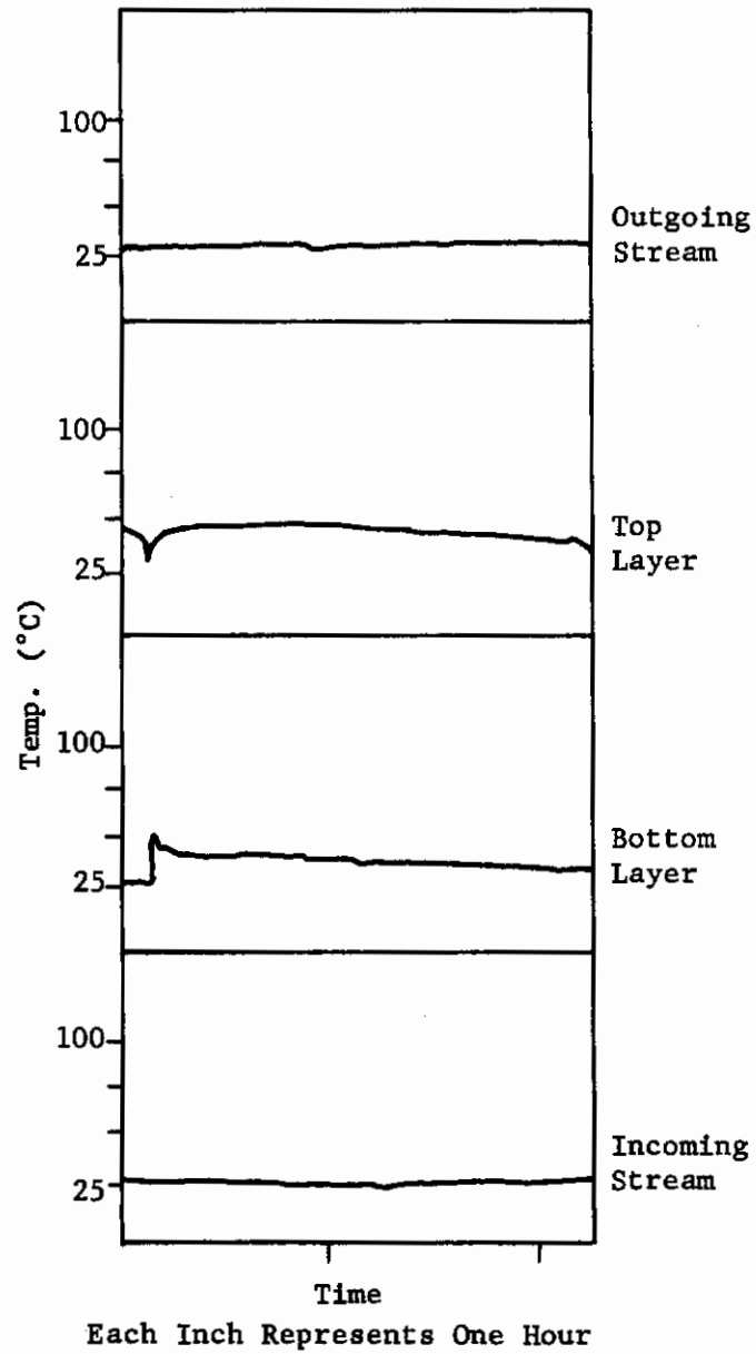
Figure 18 Temperature Profiles Taken at Different Sites During Test No. 32
