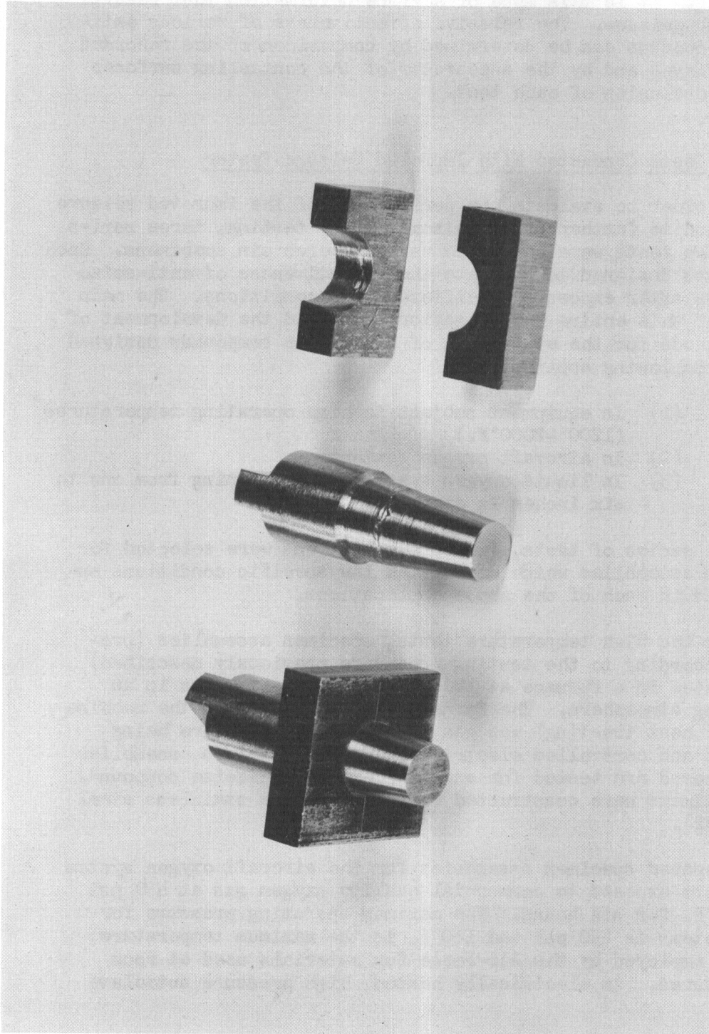
FIGURE 21. Galled Surfaces of Tapered Pin and Block Specimen after Seizure Test (Magnification 1.5X)
