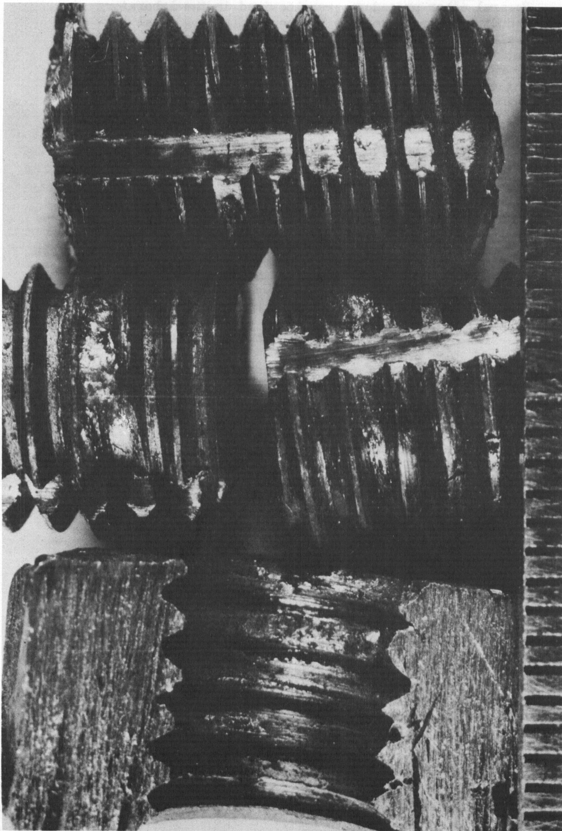
FIGURE 1. Damage to Threads Due to Metal Seizure (Magnification 11.5X)
