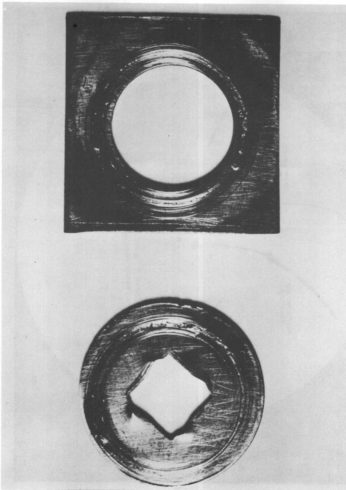
FIGURE 5. Galled Surface of Copper Sheet after Seizure Test (Magnification 5X)
