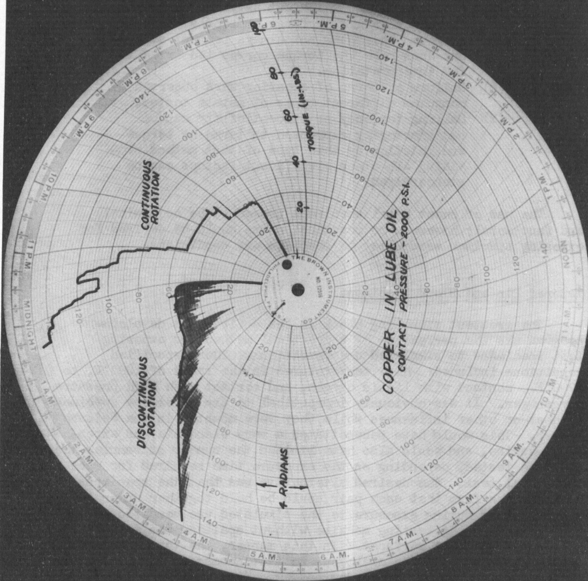
FIGURE 7. Typical Chart Record of Seizure Test
