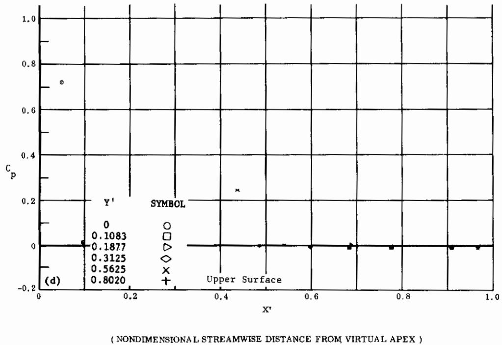
Fig. 13 Configuration I, \alpha = +50 , \delta_2 = \delta_3 = 0
