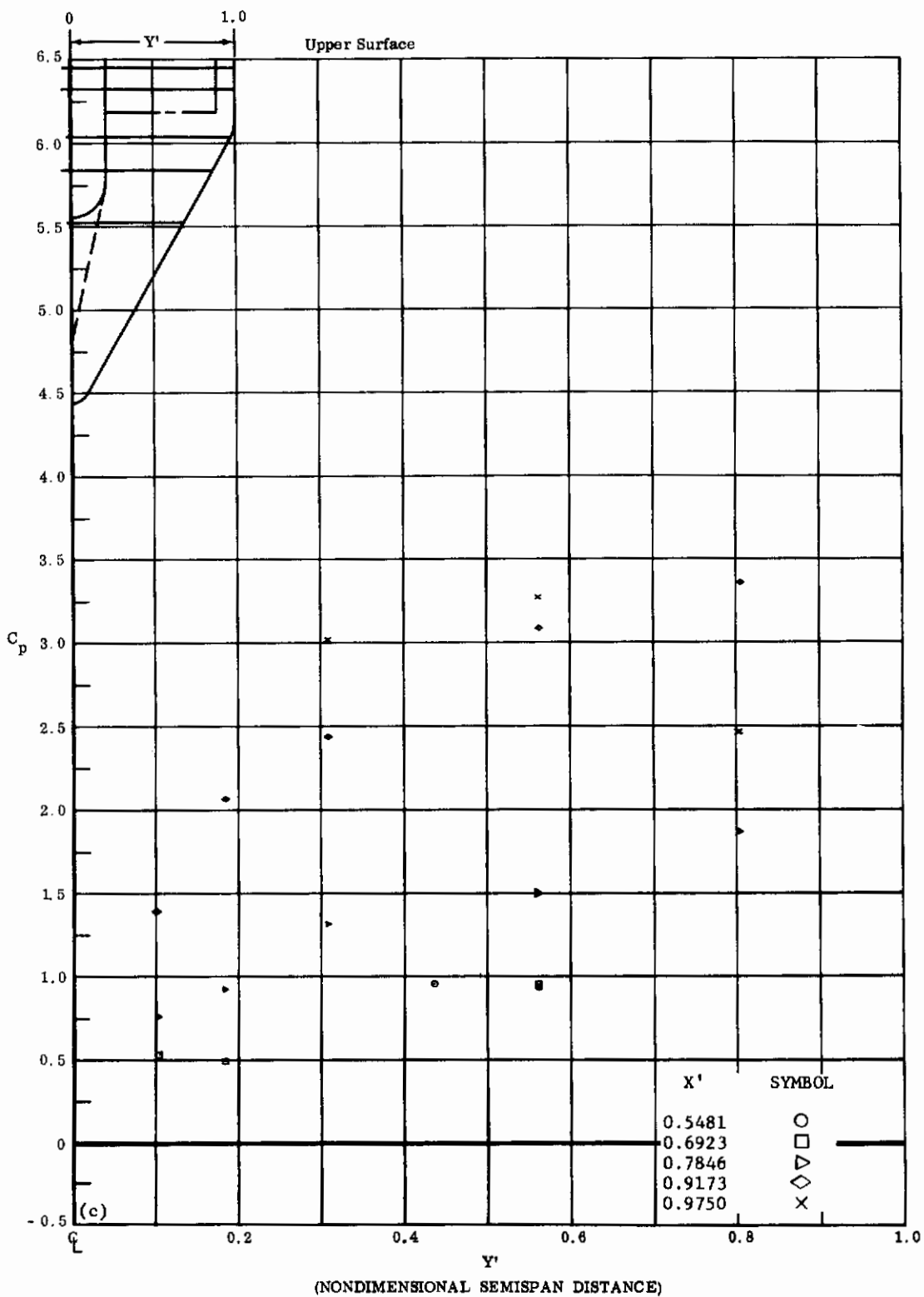
Fig. 24c Configuration I, \alpha = -35 , \delta_2 = \delta_3 = -30
