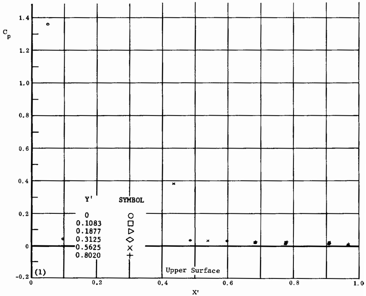
Fig. 9 Configuration I, \alpha = +30 , \delta_2 = \delta_3 = +20
