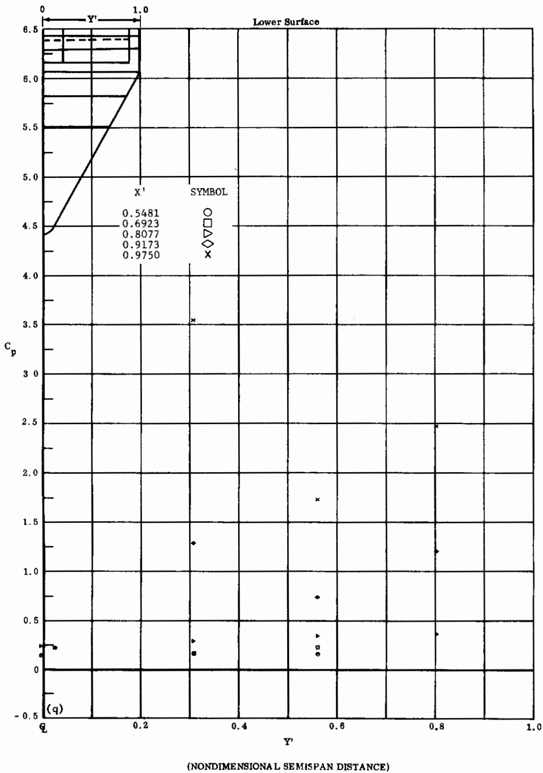
Fig. 5q Configuration I, \alpha = +10 , \delta_2 = \delta_3 = +39
