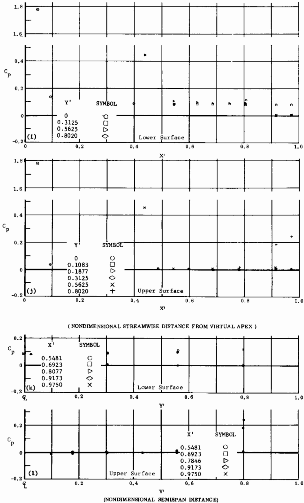
Fig. 6 Configuration I, \alpha = +10^\circ , \delta_2 = \delta_3 = -30^\circ
