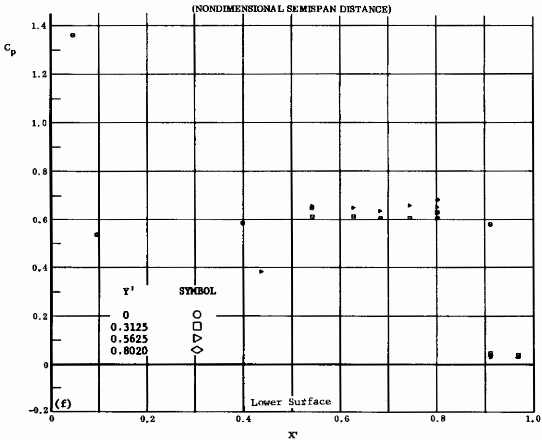
Fig. 10 Configuration I, \alpha = +30 , \delta_2 = \delta_3 = -39
