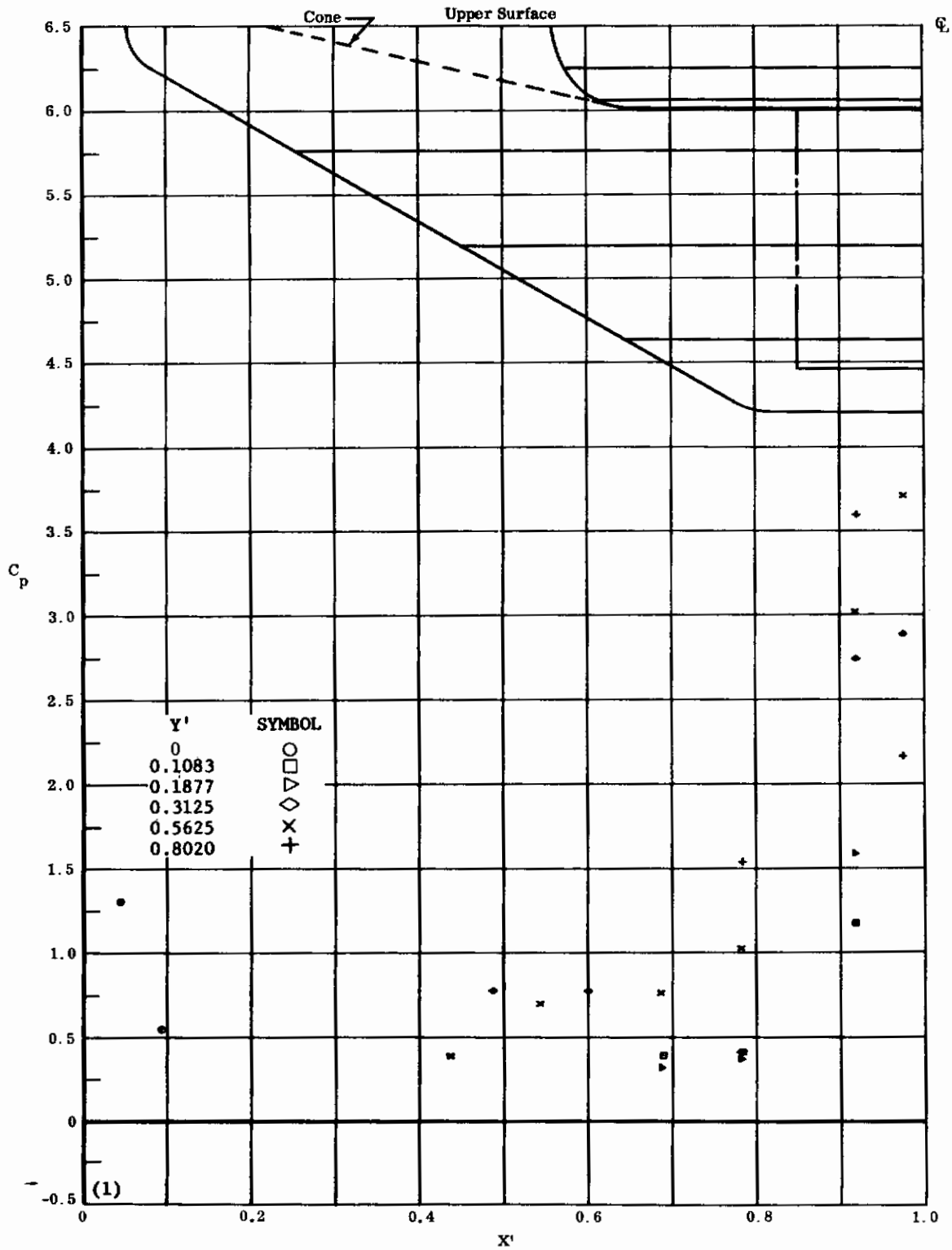
Fig. 231 Configuration I, \alpha = -30 , \delta_2 = \delta_3 = -30
