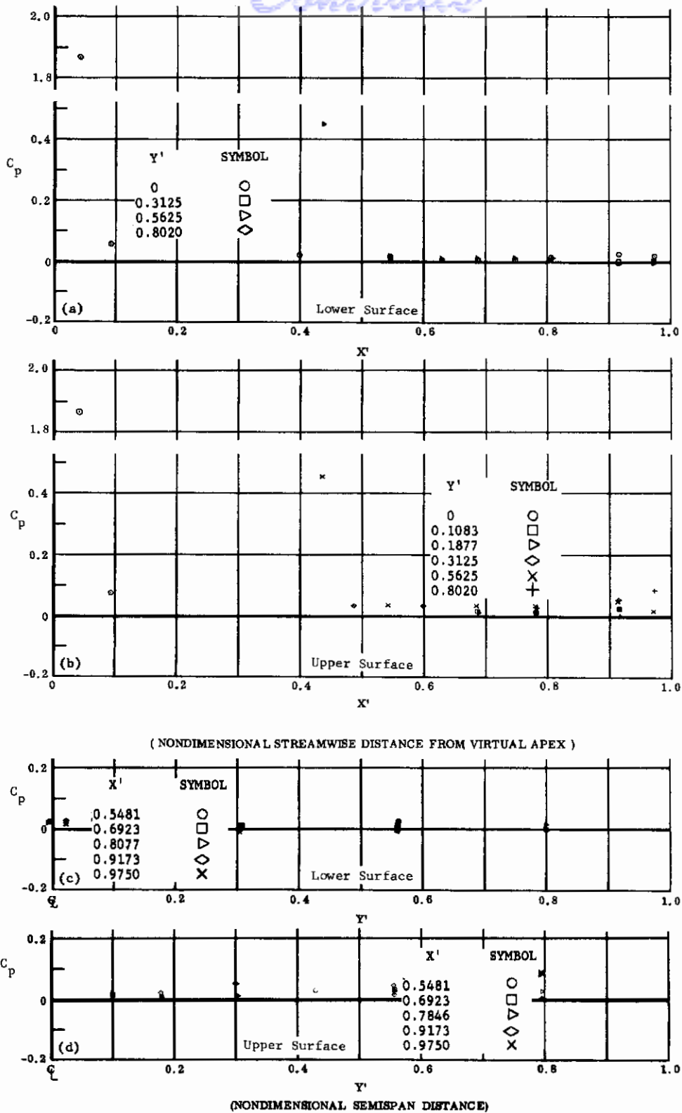
Fig. 4 Configuration I, \alpha = 0 , \delta_2 = \delta_3 = -10
