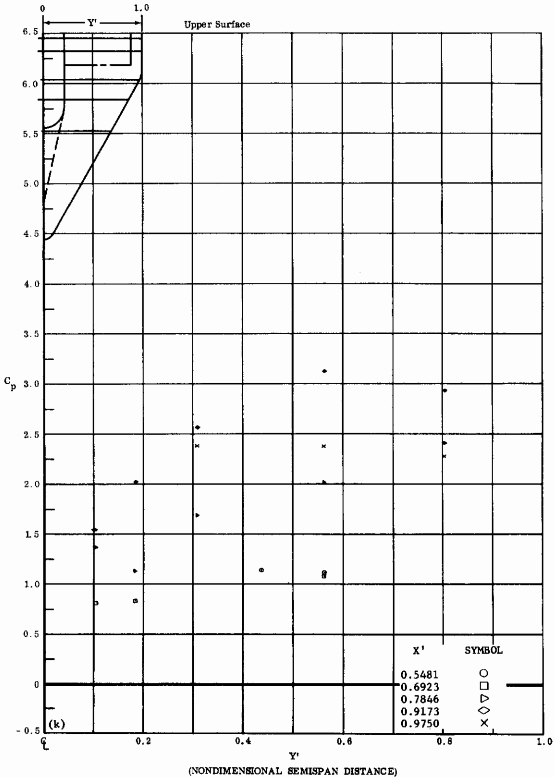
Fig. 47k Configuration IV, \alpha = -40 , \delta_2 = \delta_3 = -30
