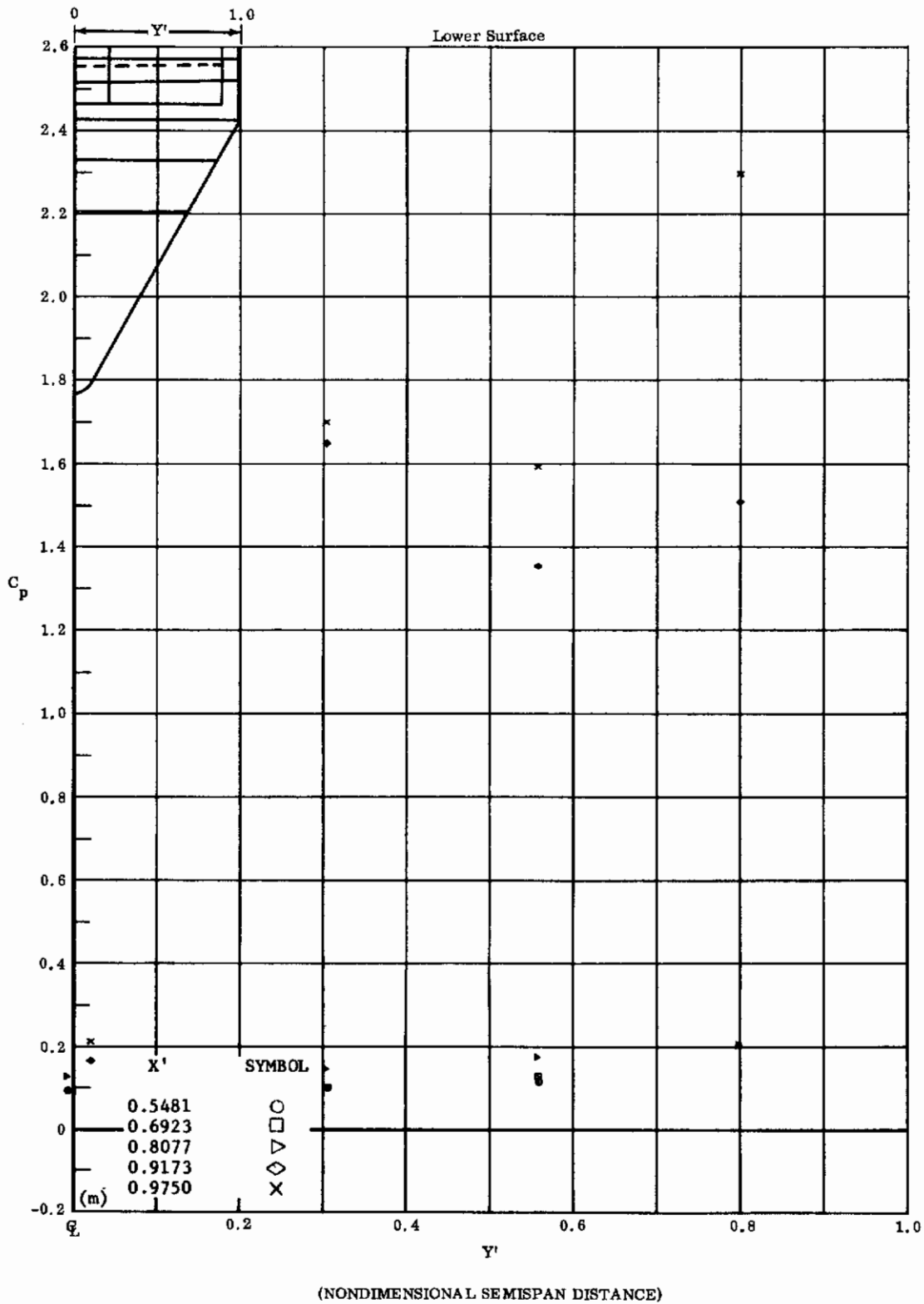
Fig. 31m Configuration IV, \alpha = +10 , \delta_2 = \delta_3 = +30 C_p vs. Y' , lower surface
