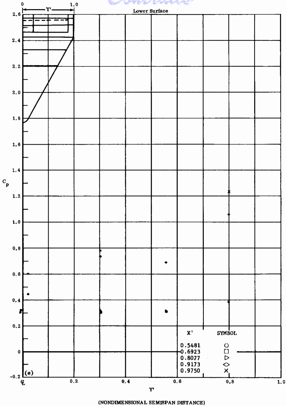
Fig. 33e Configuration IV, \alpha = +20 , \delta_2 = \delta_3 = +10 C_p vs. Y' , lower surface
