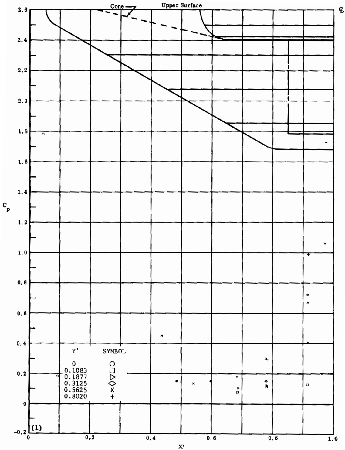
Fig. 411 Configuration IV, \alpha = -10 , \delta_2 = \delta_3 = -30
