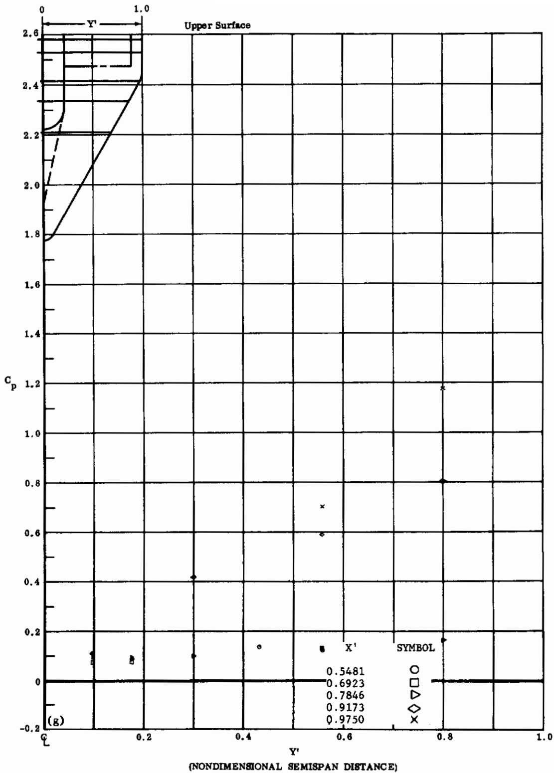
Fig. 41g Configuration IV, \alpha = -10 , \delta_2 = \delta_3 = -20
