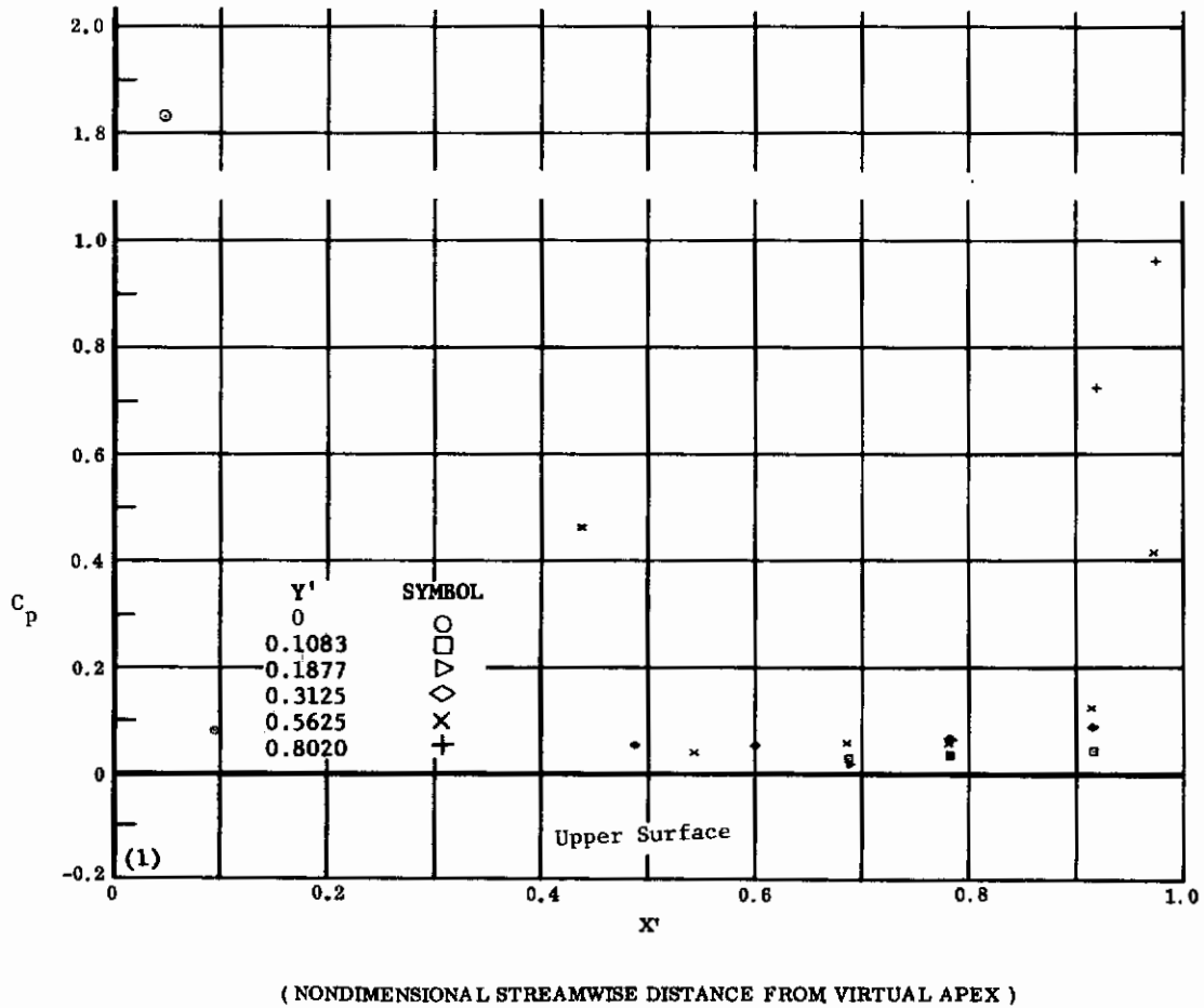
Fig. 30 Configuration IV, \alpha = 0 , \delta_2 = \delta_3 = -30
