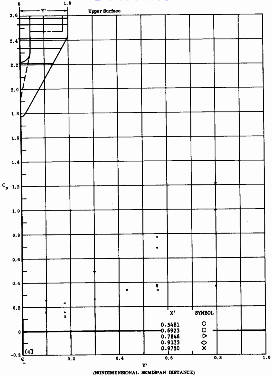
Fig. 43c Configuration IV, \alpha = -20 , \delta_2 = \delta_3 = -10
