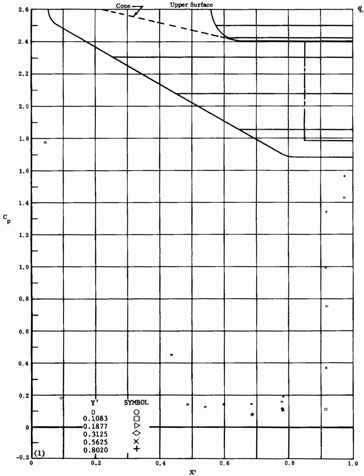
Fig. 171 Configuration I, \alpha = -10 , \delta_2 = \delta_3 = -30
