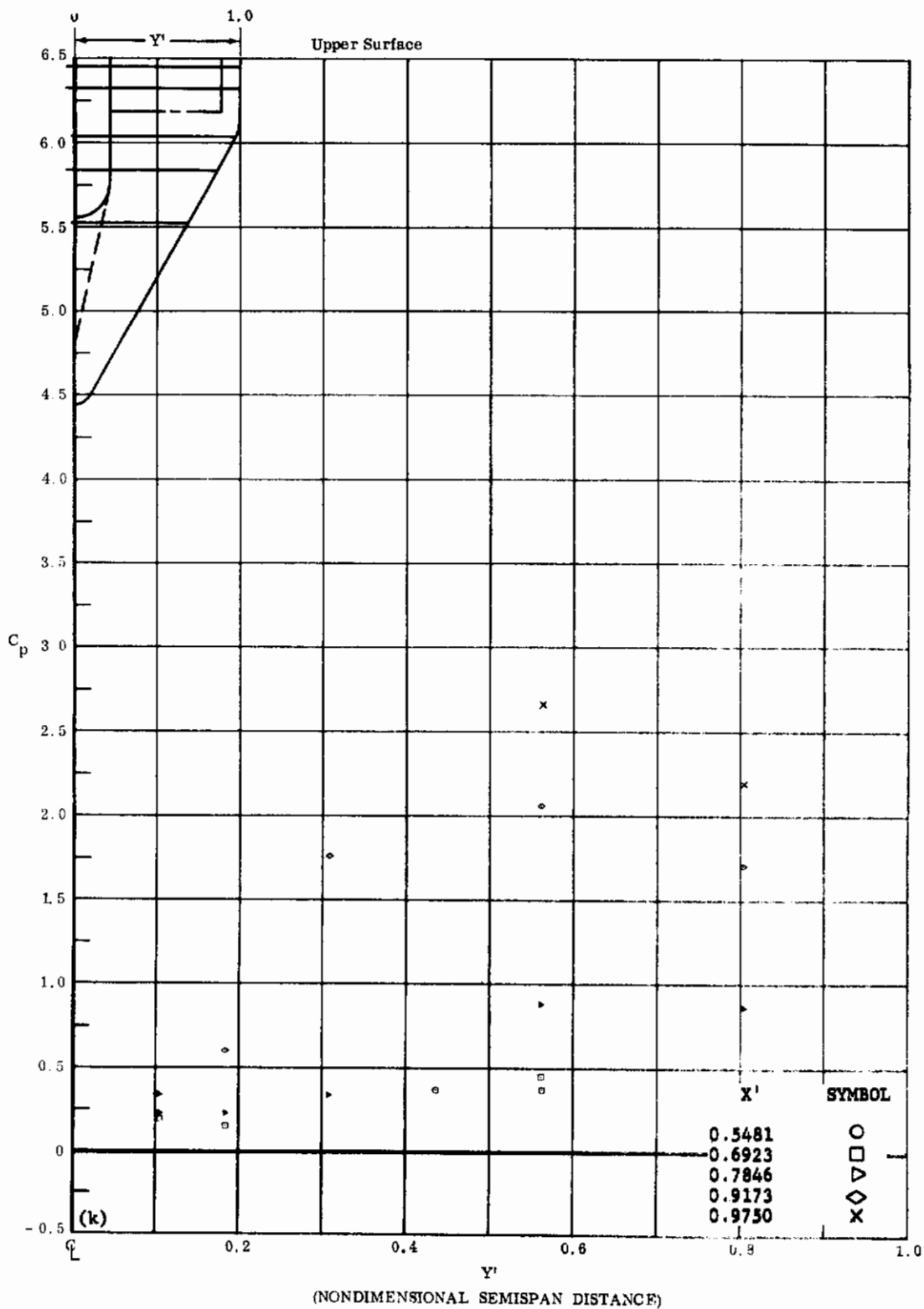
Fig. 43k Configuration IV, \alpha = -20 , \delta_2 = \delta_3 = -30
