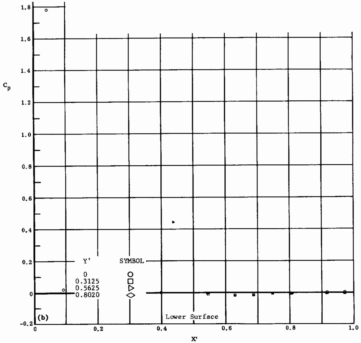
Fig. 17 Configuration I, \alpha = -10 , \delta_2 = \delta_3 = -10
