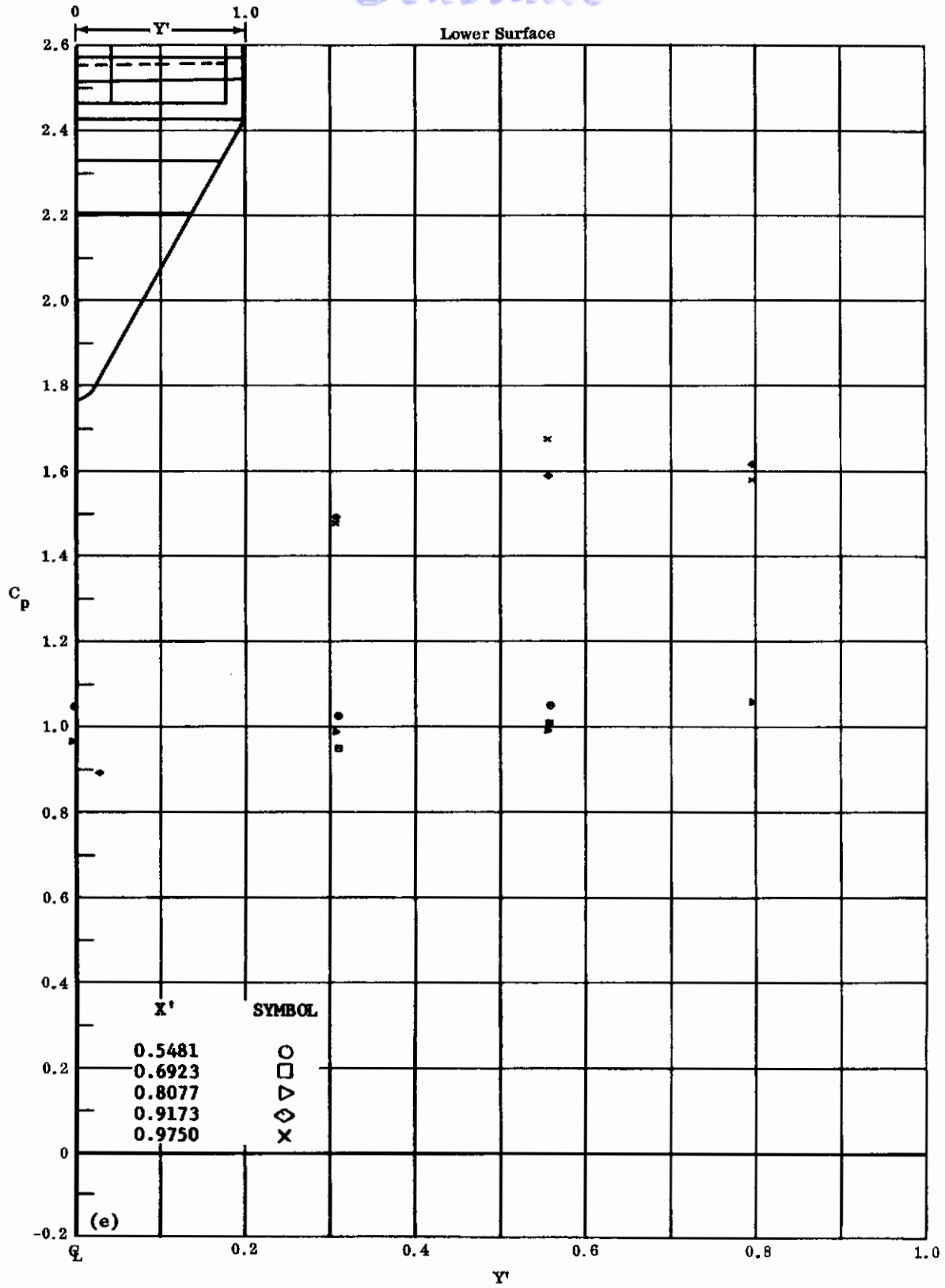
Fig. 11e Configuration I, \alpha = +40 , \delta_2 = \delta_3 = +10
