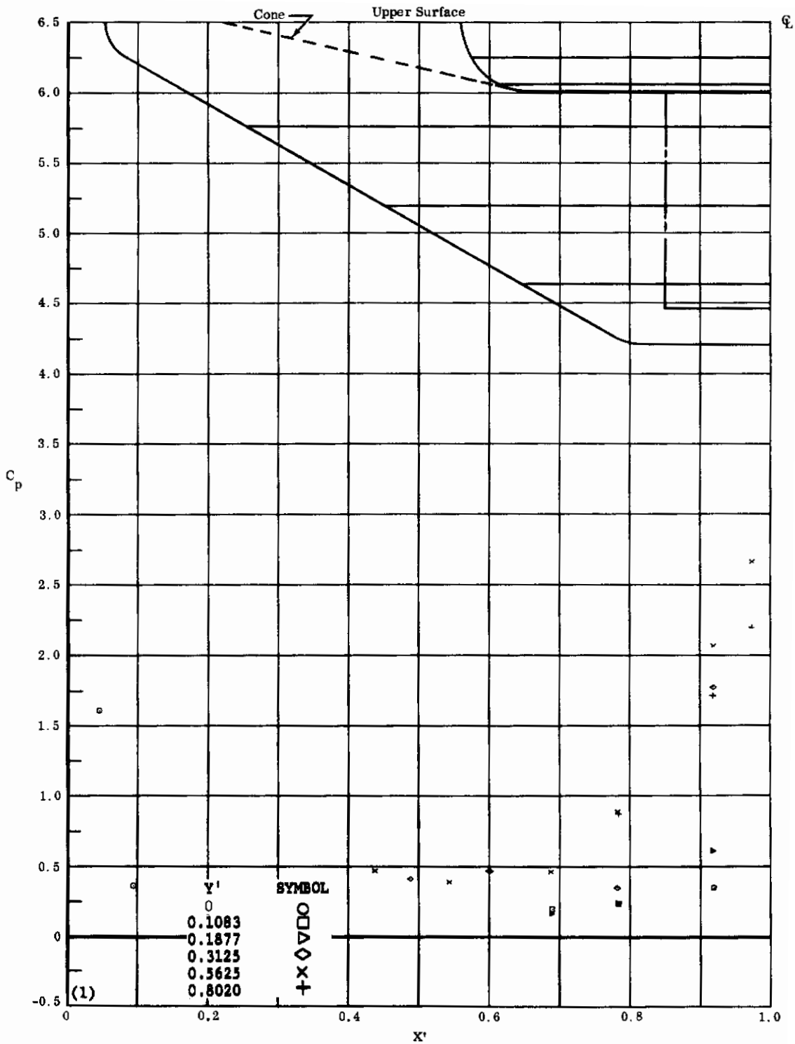
Fig. 431 Configuration IV, \alpha = -20 , \delta_2 = \delta_3 = -30
