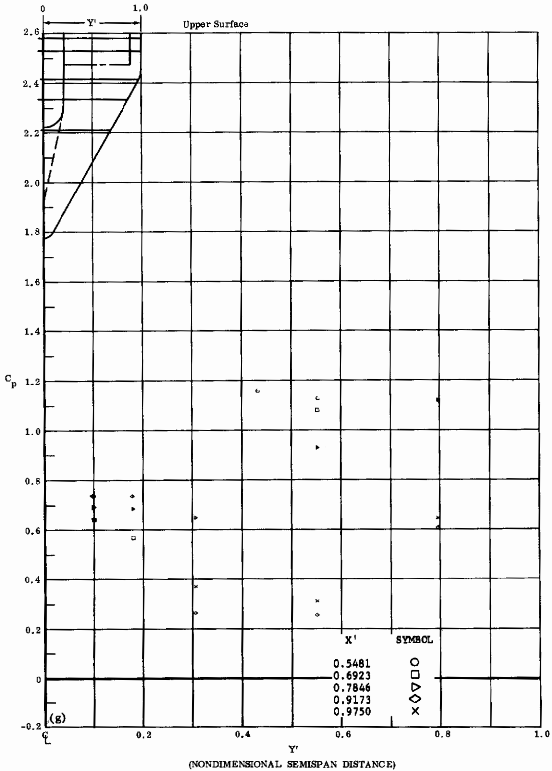
Fig. 46g Configuration IV, \alpha = -40 , \delta_2 = \delta_3 = +20 C_p vs. Y' , upper surface
