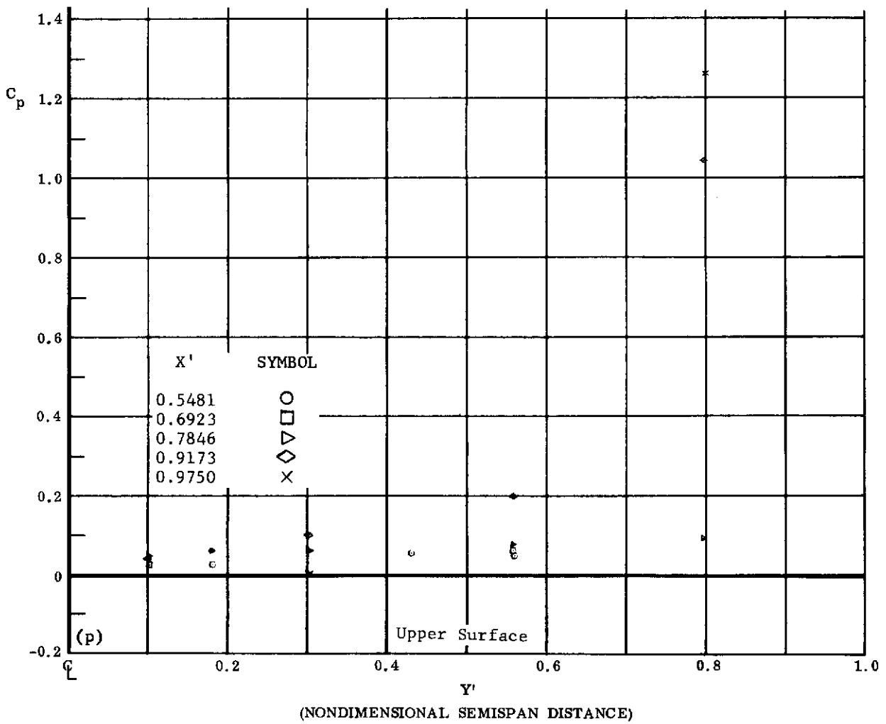
Fig. 4 Configuration I, \alpha = 0 , \delta_2 = \delta_3 = -39
