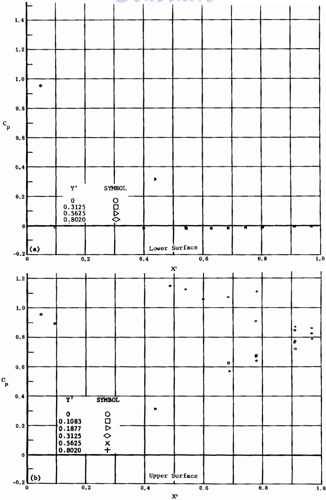
Fig. 25 Configuration I, \alpha = -40 , \delta_2 = \delta_3 = 0
