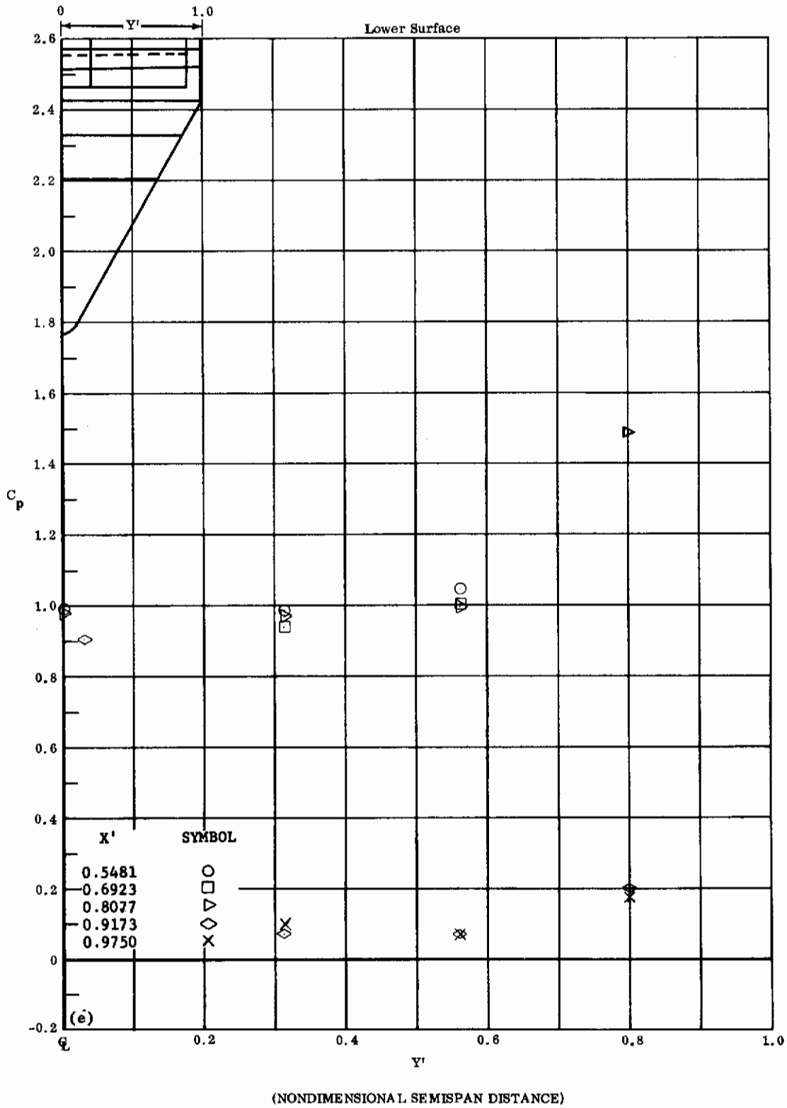
Fig. 38e Configuration IV, \alpha = +40 , \delta_2 = \delta_3 = -39 C_p vs. Y' , lower surface
