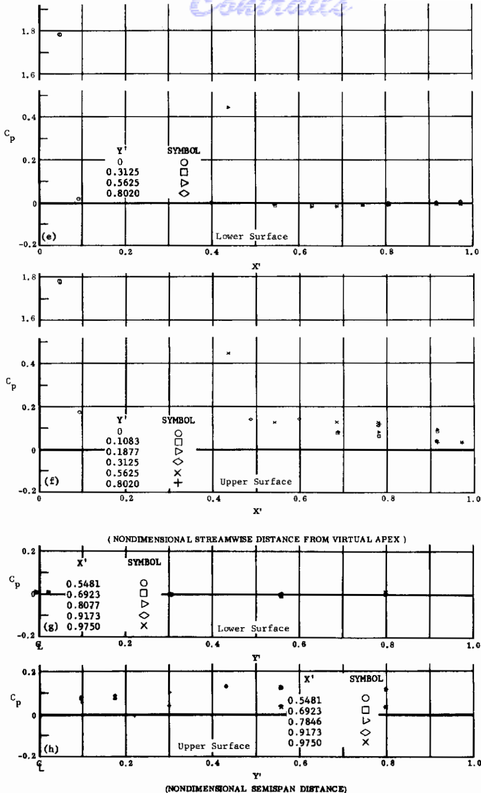
Fig. 16 Configuration I, \alpha = -10 , \delta_2 = \delta_3 = +10
