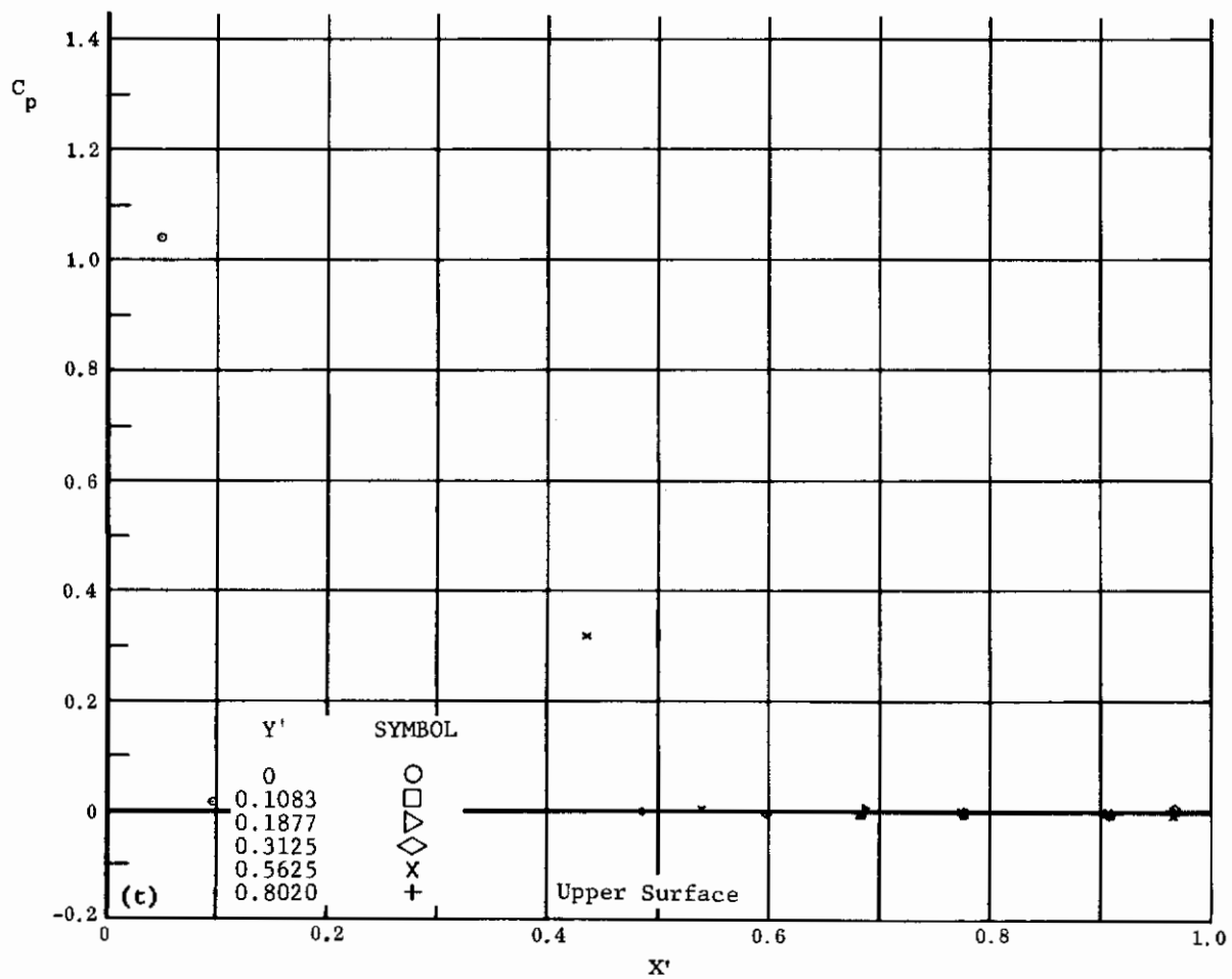
Fig. 11 Configuration I, \alpha = +40 , \delta_2 = \delta_3 = +39
