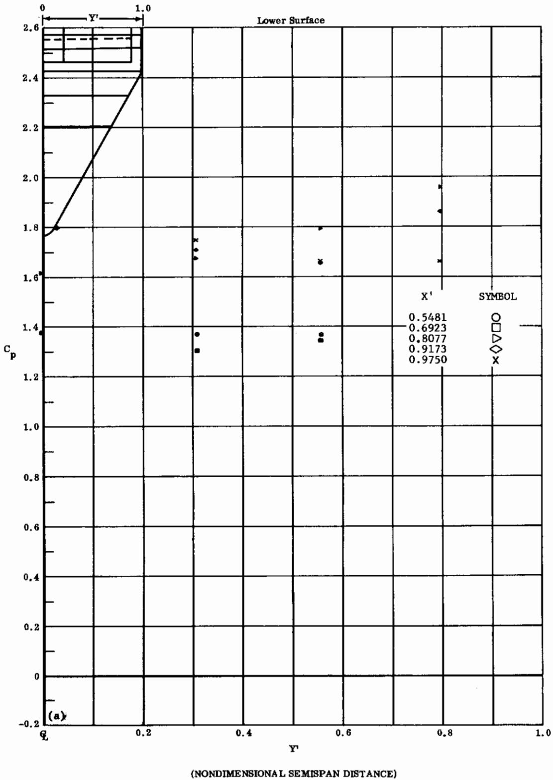
Fig. 39a Configuration IV, \alpha = +50 , \delta_2 = \delta_3 = 0 C_p vs. Y' , lower surface
