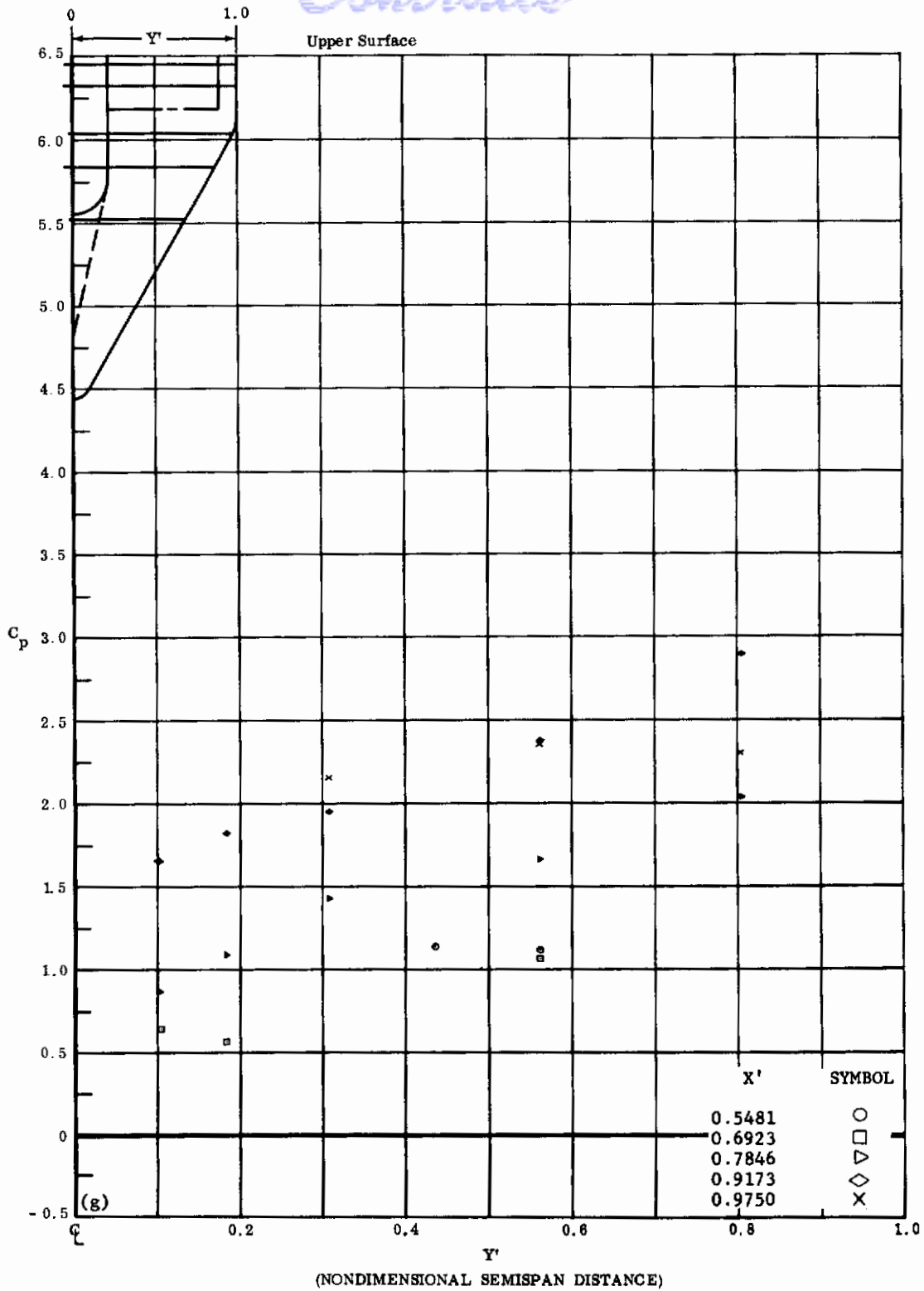
Fig. 47g Configuration IV, \alpha = -40 , \delta_2 = \delta_3 = -20
