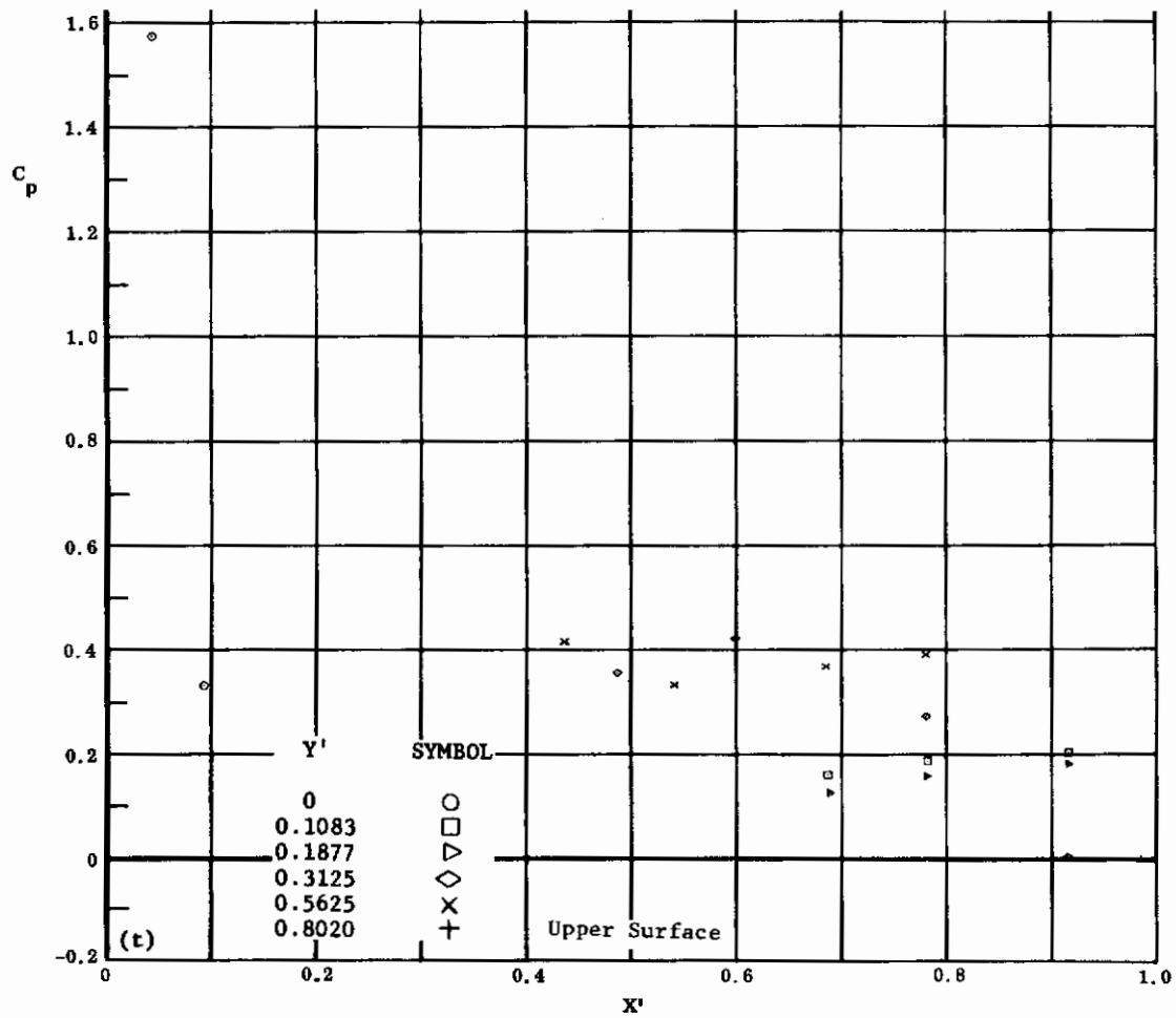
Fig. 19 Configuration I, \alpha = -20 , \delta_2 = \delta_3 = +39
