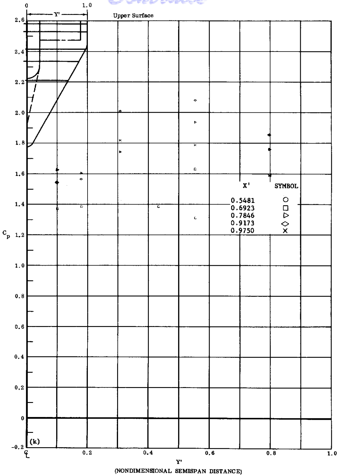
Fig. 28k Configuration I, \alpha = -50 , \delta_2 = \delta_3 = -30
