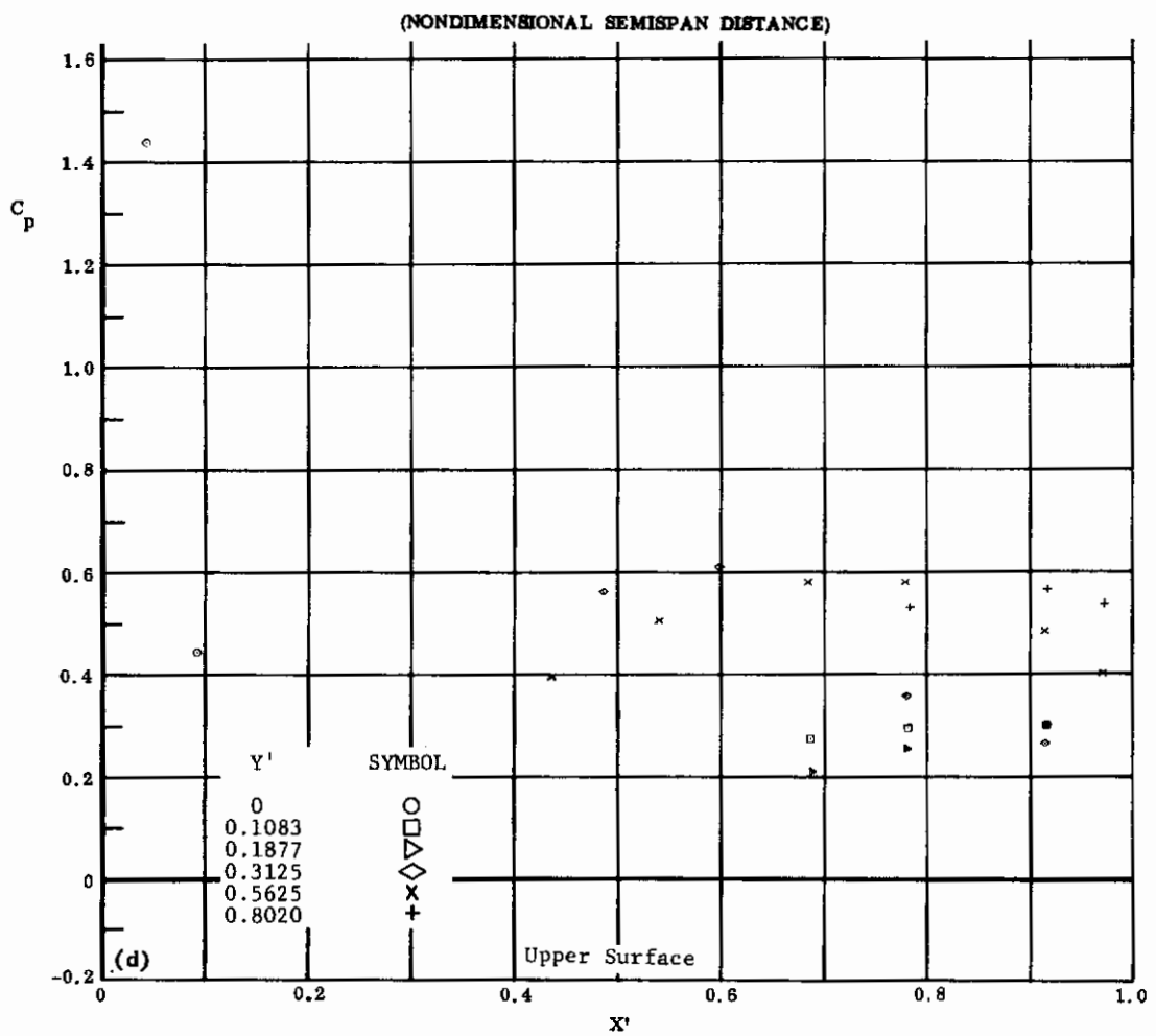
Fig. 21 Configuration I, \alpha = -25 , \delta_2 = \delta_3 = 0
