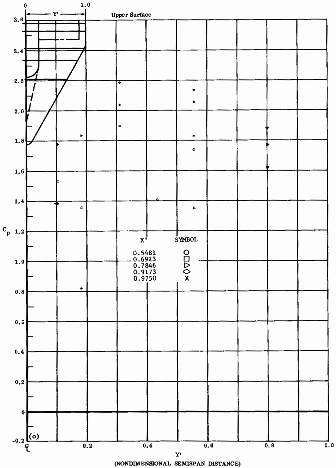
Fig. 28o Configuration I, \alpha = -50 , \delta_2 = \delta_3 = -39
