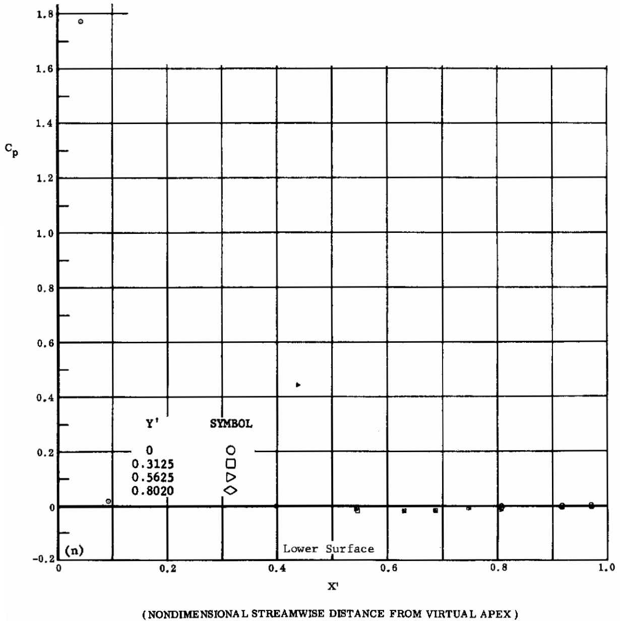
Fig. 17 Configuration I, \alpha = -10 , \delta_2 = \delta_3 = -39
