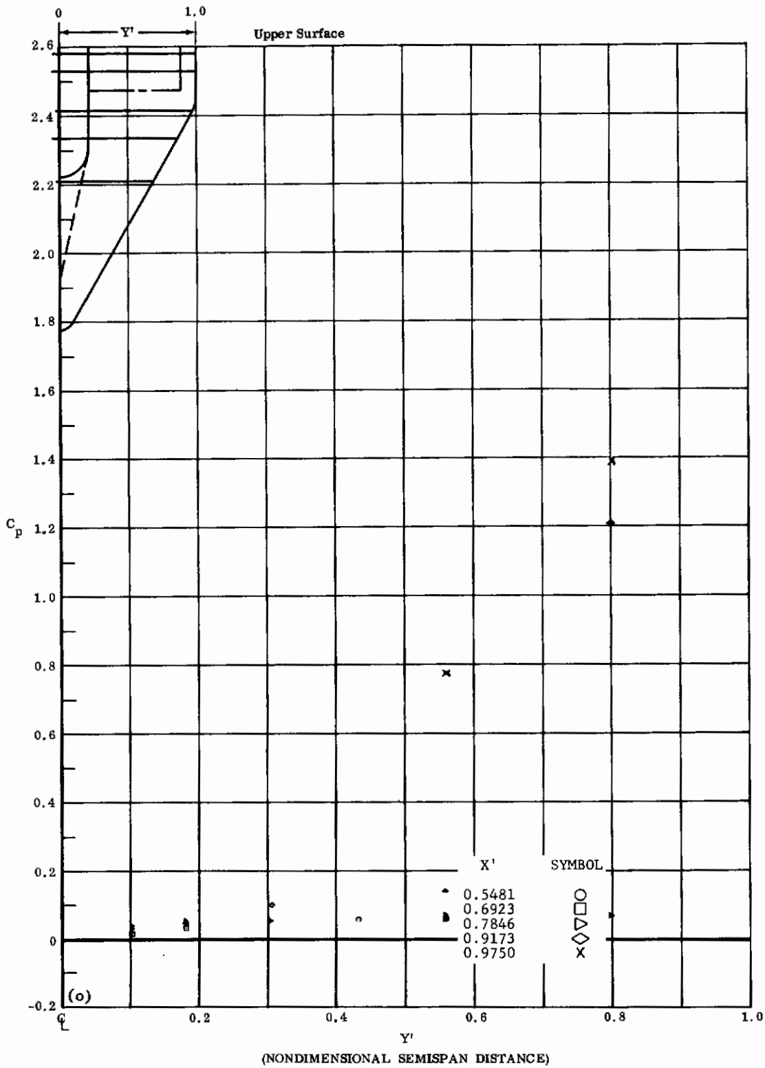
Fig. 30 Configuration IV, \alpha = 0 , \delta_2 = \delta_3 = -39^\circ
