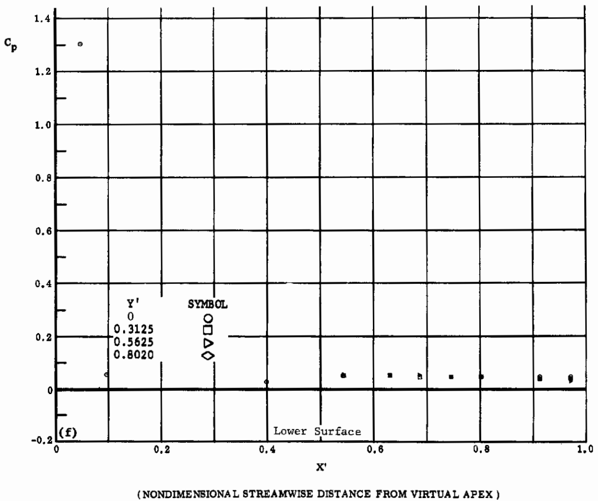
Fig. 45 Configuration IV, \alpha = -30 , \delta_2 = \delta_3 = -20
