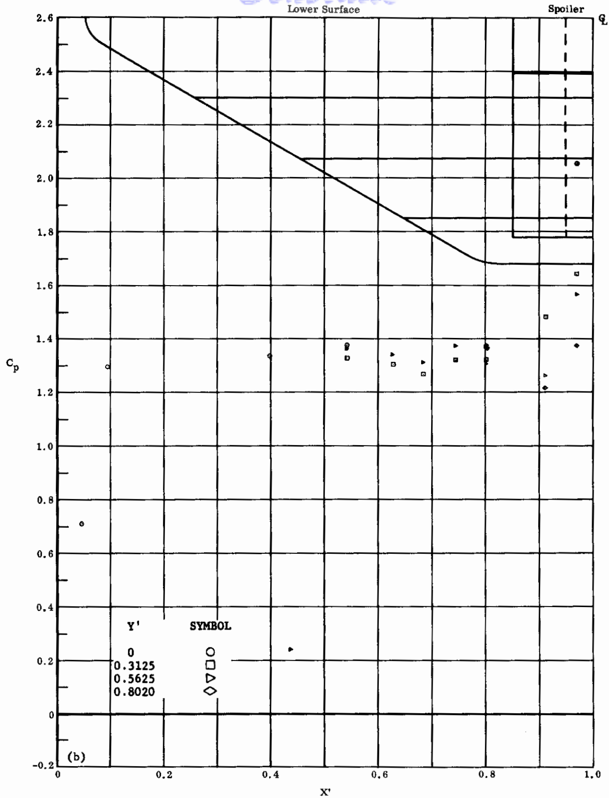
Fig. 13b Configuration I, \alpha = +50 , \delta_2 = \delta_3 = 0
