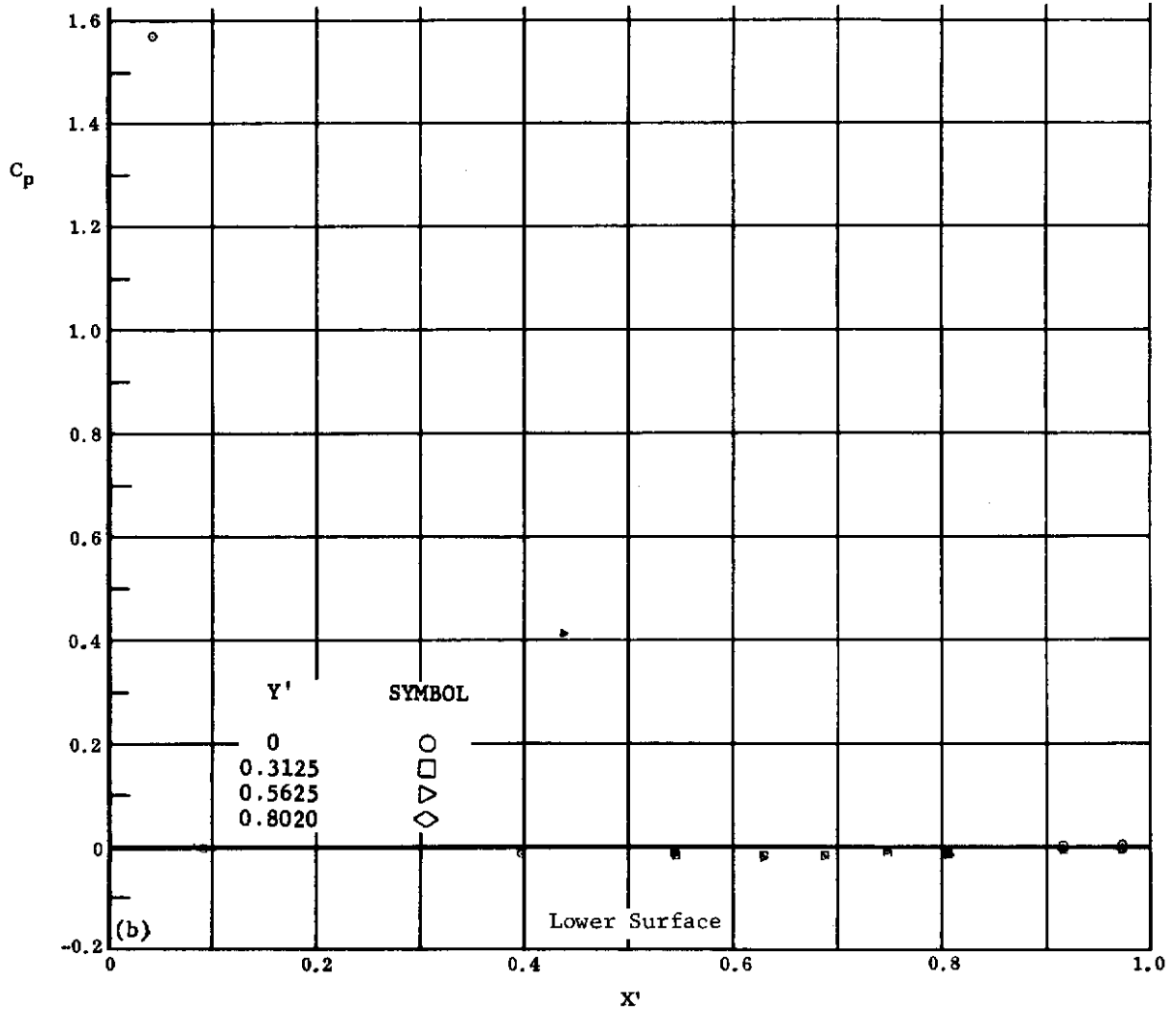
Fig. 19 Configuration I, \alpha = -20 , \delta_2 = \delta_3 = 0
