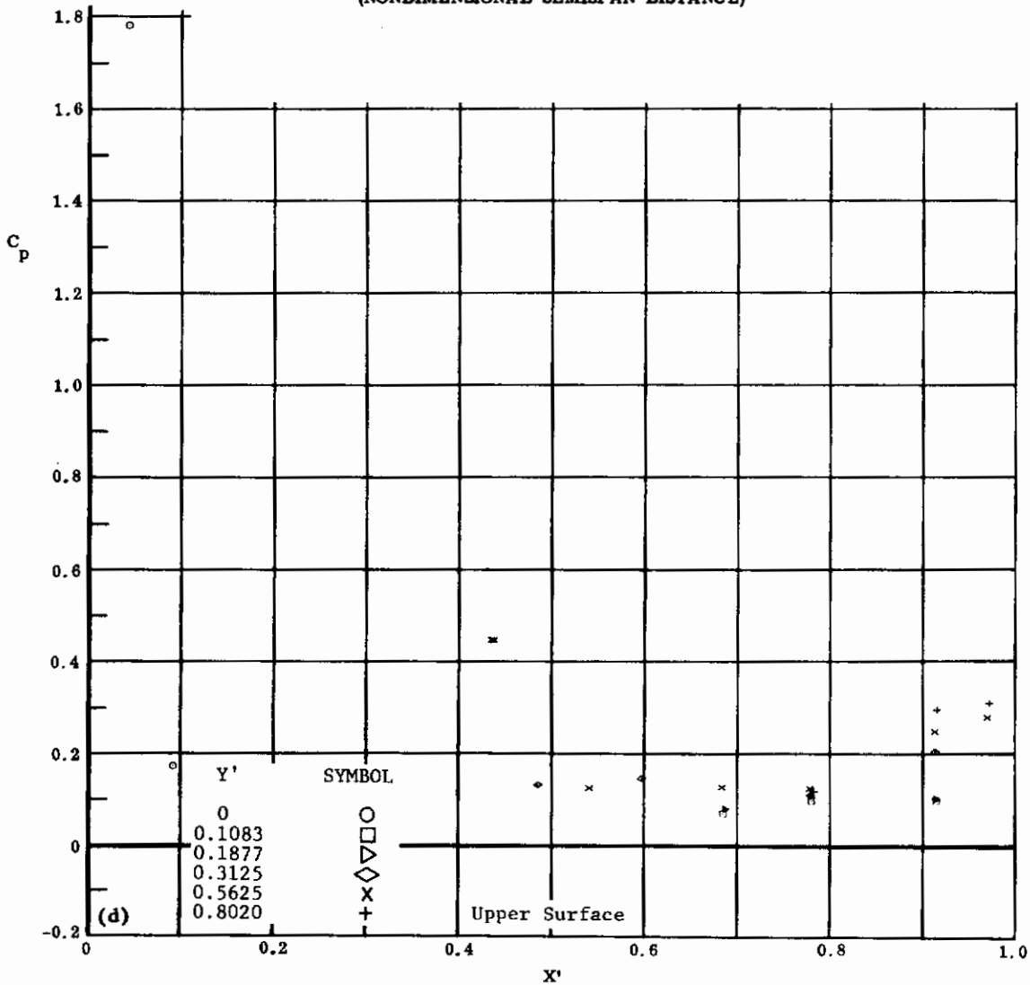
Fig. 17 Configuration I, \alpha = -10 , \delta_2 = \delta_3 = -10
