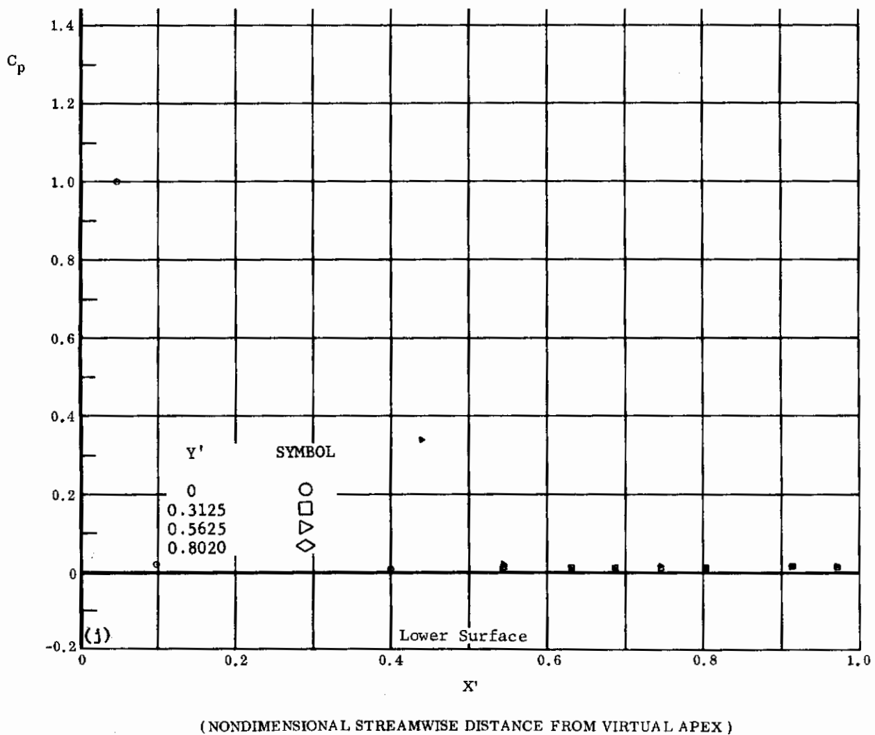
Fig. 46 Configuration IV, \alpha = -40 , \delta_2 = \delta_3 = +39
