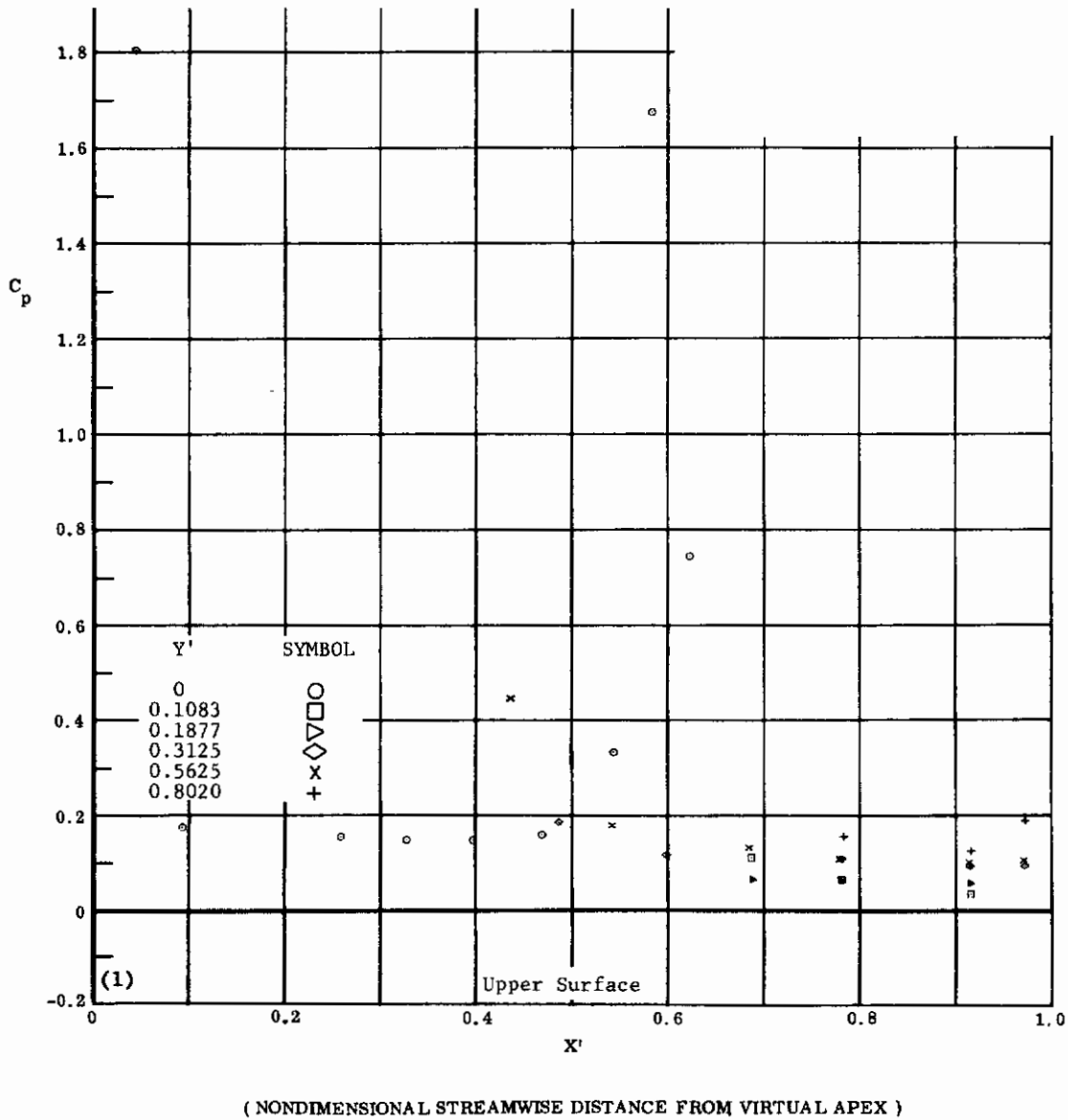
Fig. 51 Configuration VIII, Spoiler on, Re_{\infty}/ft \times 10^{-6} = 3.3
