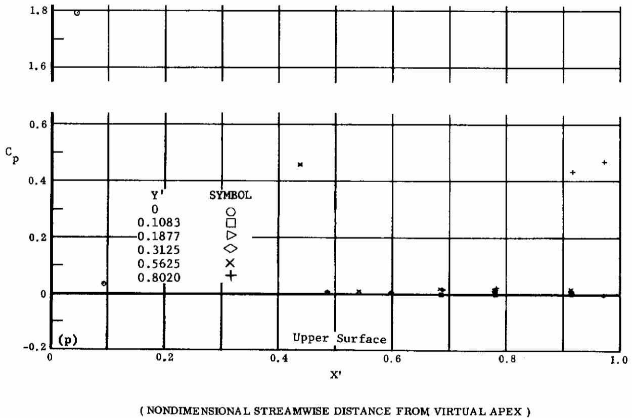
Fig. 6 Configuration I, \alpha = +10 , \delta_2 = \delta_3 = -39
