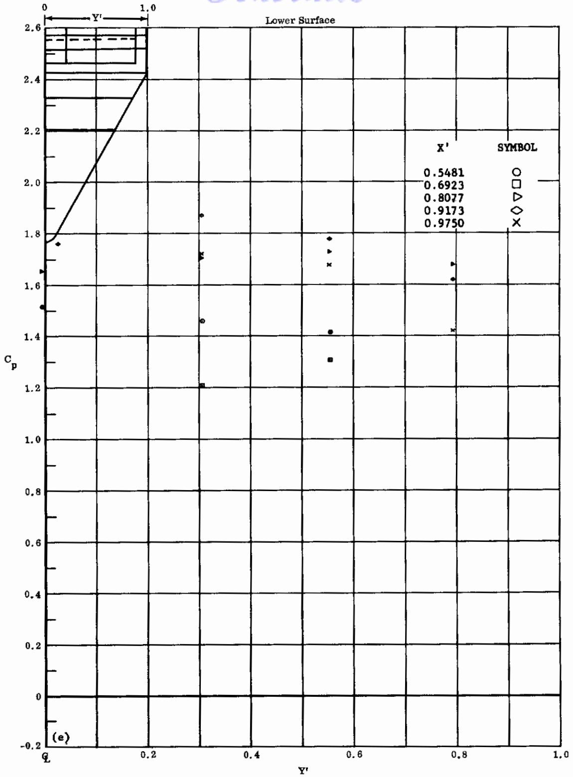
Fig. 13e Configuration I, \alpha = +50 , \delta_2 = \delta_3 = +10
