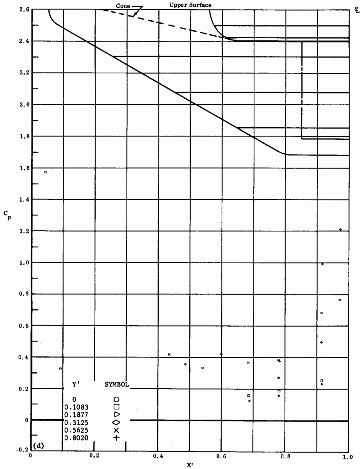
Fig. 43d Configuration IV, \alpha = -20 , \delta_2 = \delta_3 = -10
