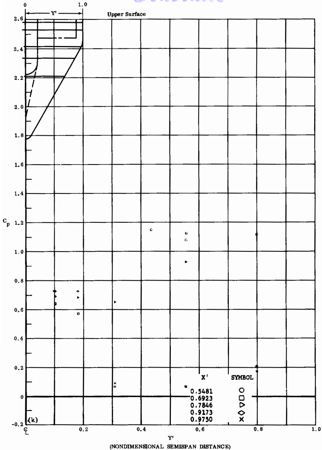
Fig. 46k Configuration IV, \alpha = -40 , \delta_2 = \delta_3 = +39
