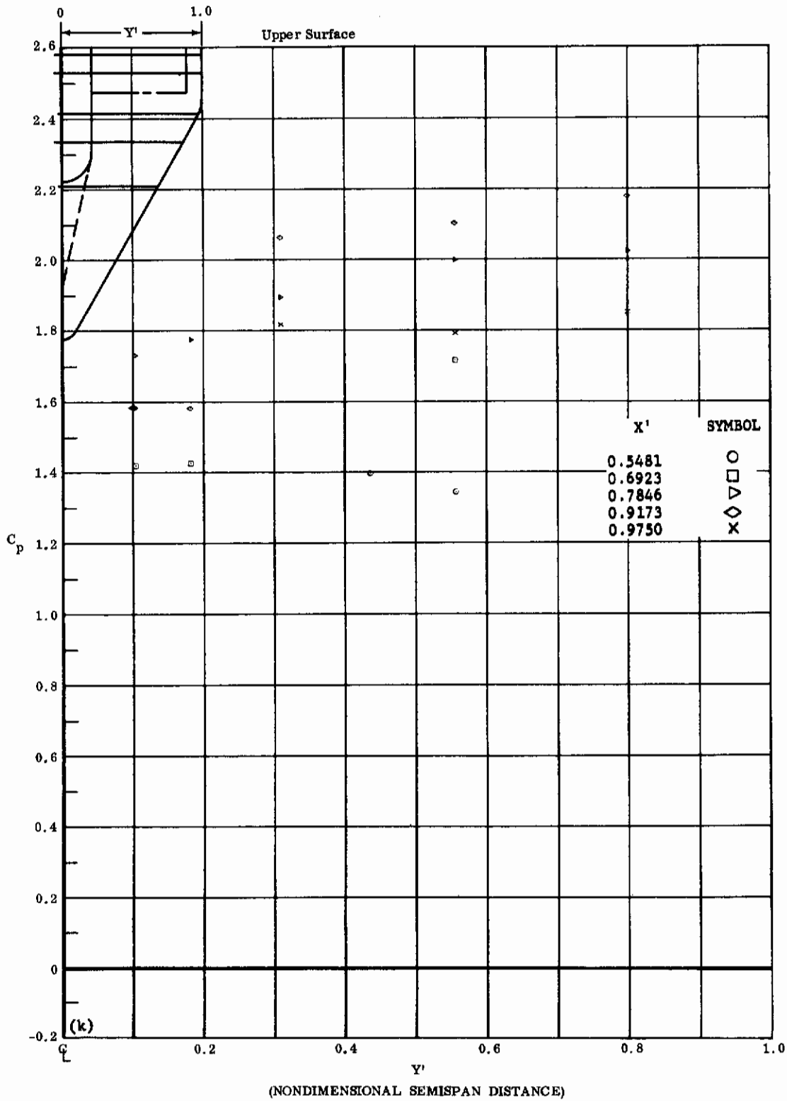
Fig. 49k Configuration IV, \alpha = -50 , \delta_2 = \delta_3 = -30
