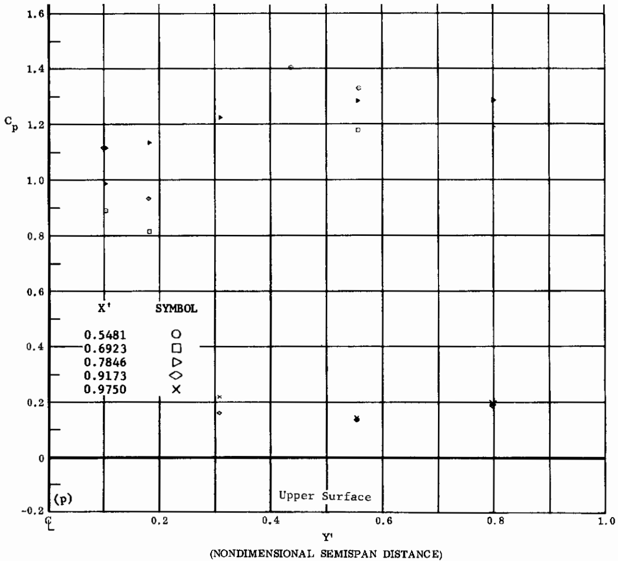
Fig. 27 Configuration I, \alpha = -50 , \delta_2 = \delta_3 = +39
