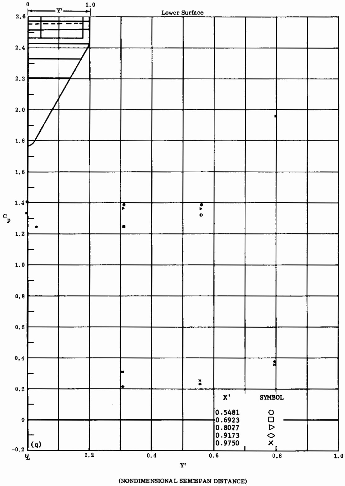
Fig. 39q Configuration IV, \alpha = +50 , \delta_2 = \delta_3 = -39
