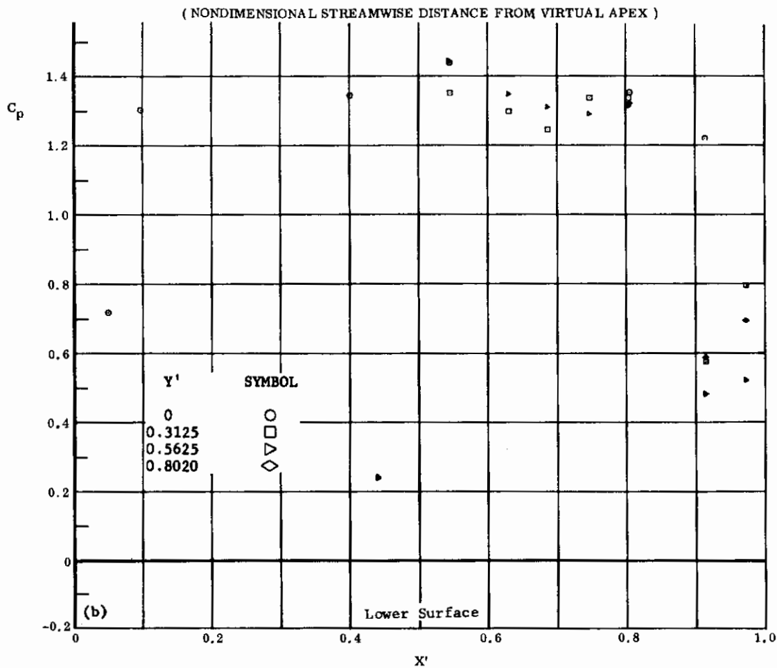
Fig. 14 Configuration I, \alpha = +50 , \delta_2 = \delta_3 = -20
