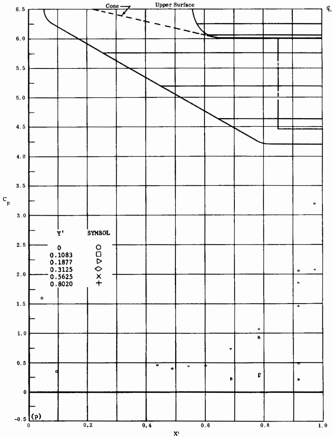
Fig. 43p Configuration IV, \alpha = -20 , \delta_2 = \delta_3 = -39
