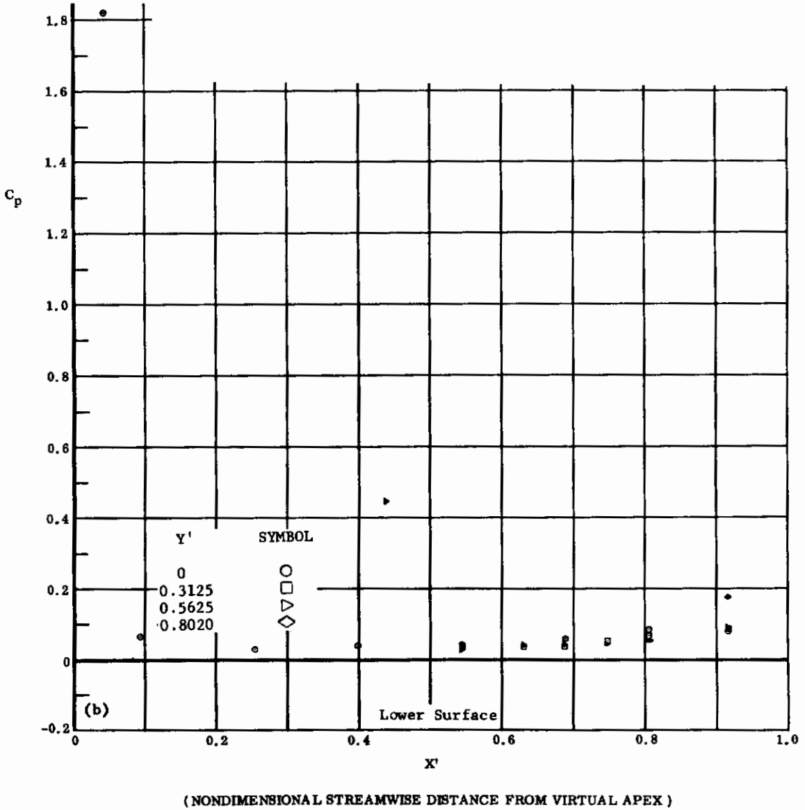
Fig. 51 Configuration VIII, Spoiler on, Re_{\infty}/ft \times 10^{-6} = 3.3
