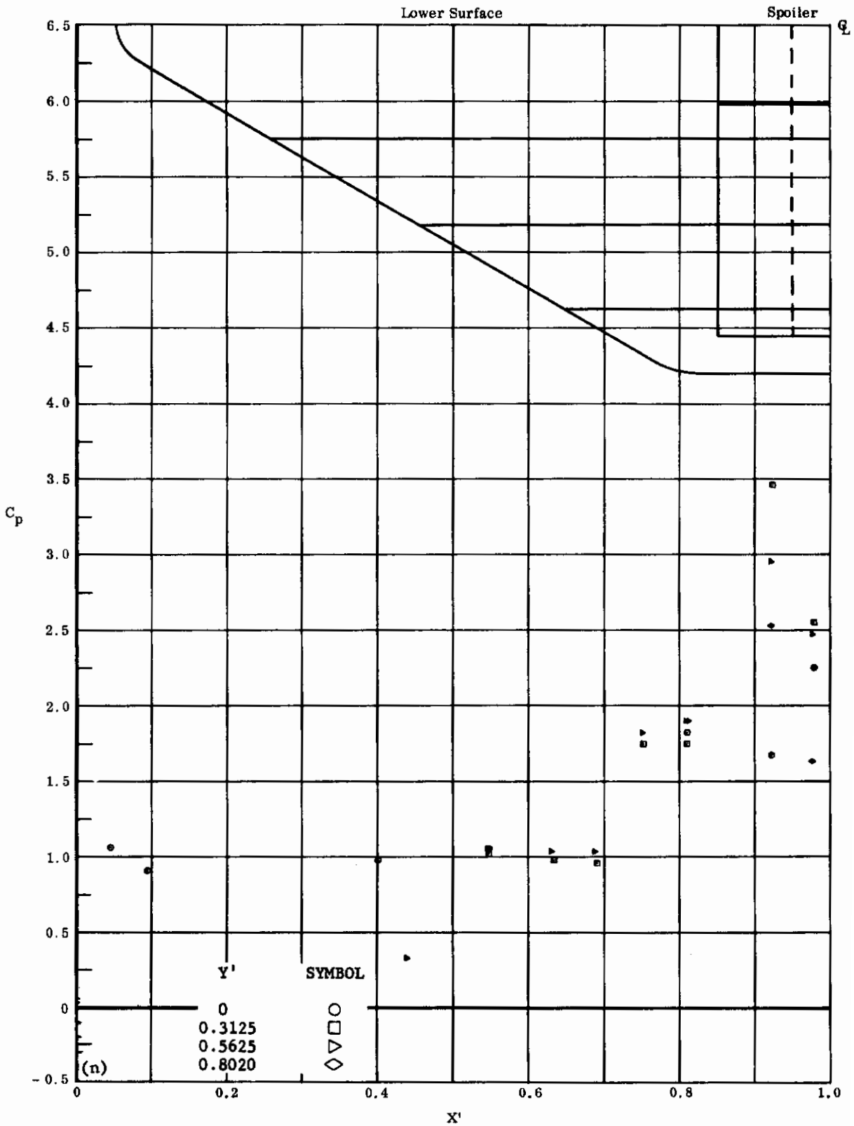
Fig. 11n Configuration I, \alpha = +40 , \delta_2 = \delta_3 = +30
