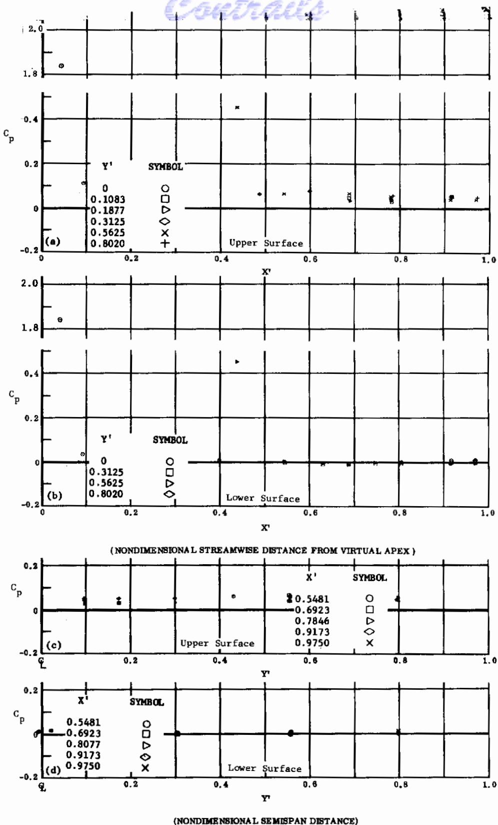
Fig. 15 Configuration I, \alpha = -5 , \delta_2 = \delta_3 = 0
