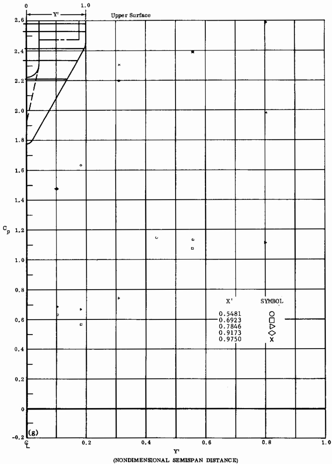
Fig. 26g Configuration I, \alpha = -40 , \delta_2 = \delta_3 = -20 C_p vs. Y' , upper surface
