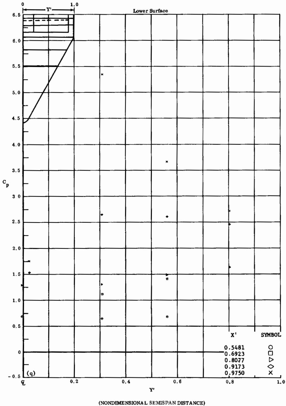
Fig. 35q Configuration IV, \alpha = +30 , \delta_2 = \delta_3 = +39
