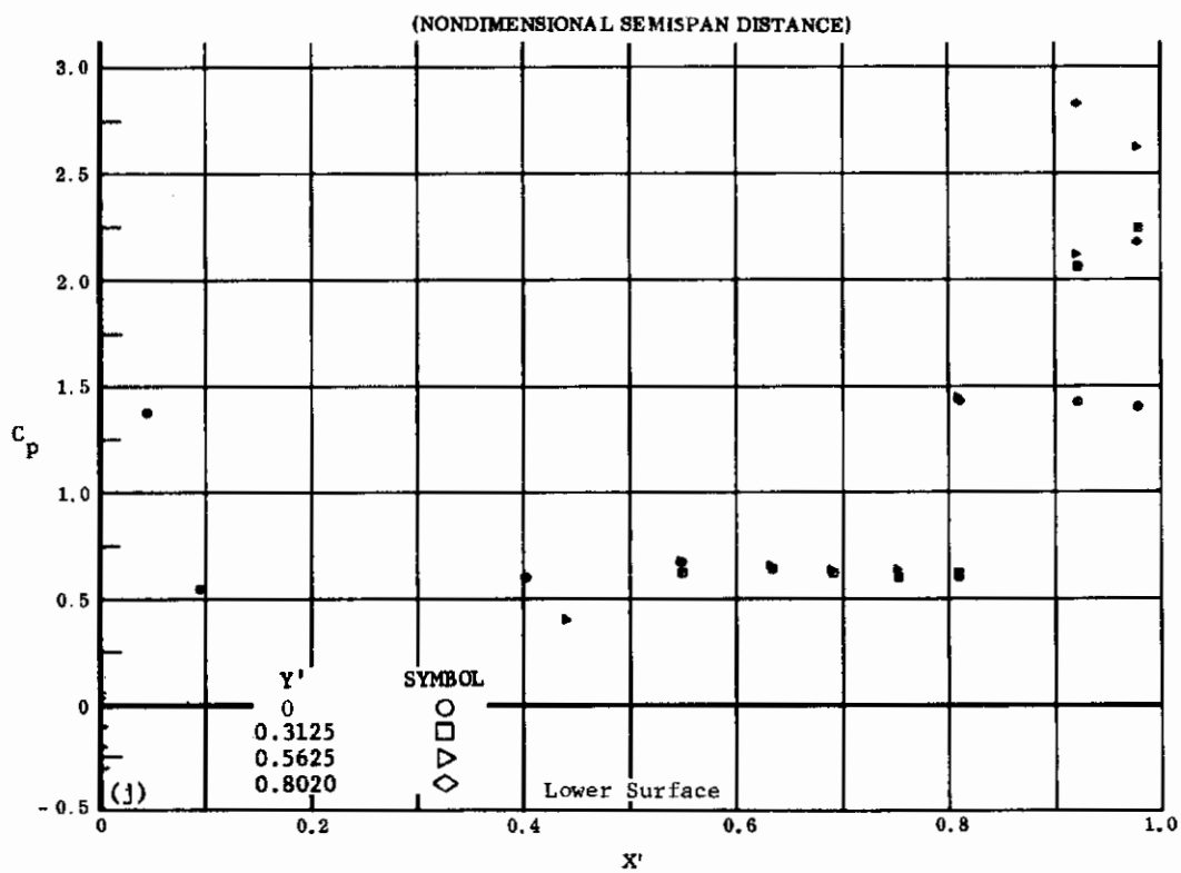
Fig. 35 Configuration IV, \alpha = +30 , \delta_2 = \delta_3 = +20
