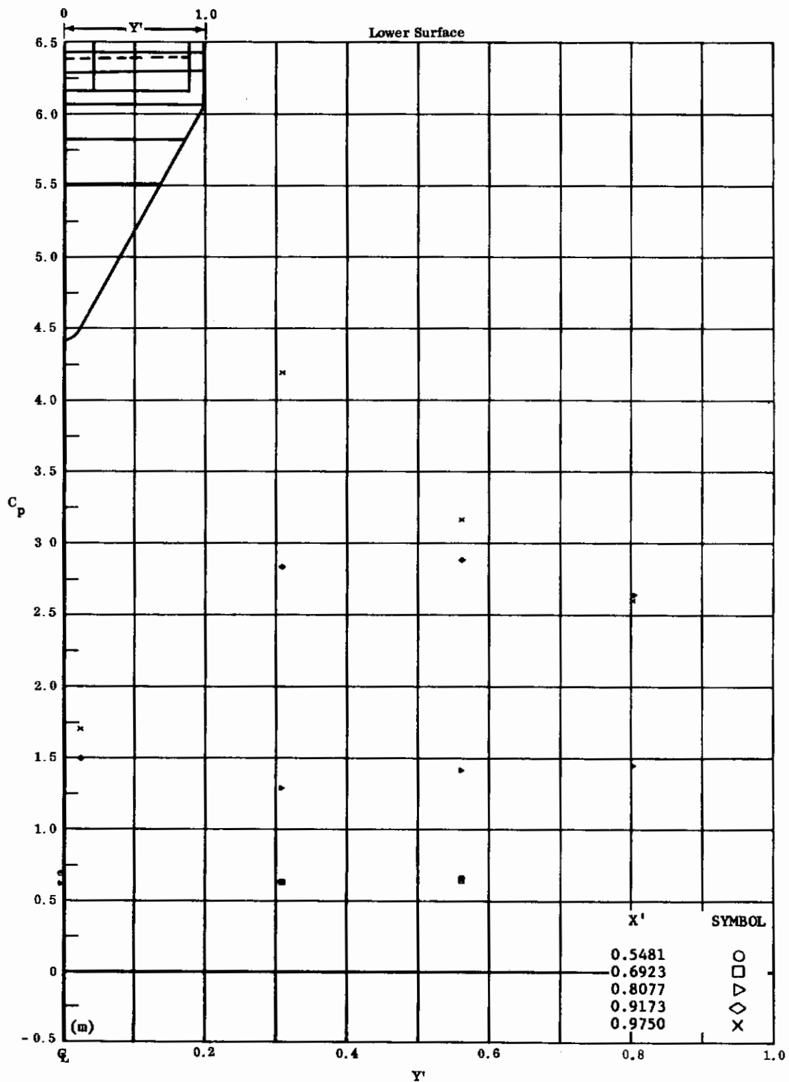
(NONDIMENSIONAL SEMISPAN DISTANCE) Fig. 9m Configuration I, \alpha = +30 , \delta_2 = \delta_3 = +30
