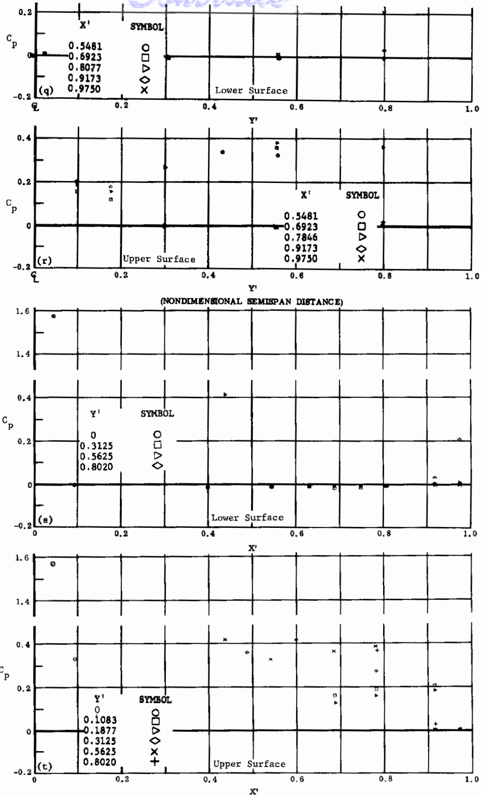
Fig. 42 Configuration IV, \alpha = -20 , \delta_2 = \delta_3 = +39
