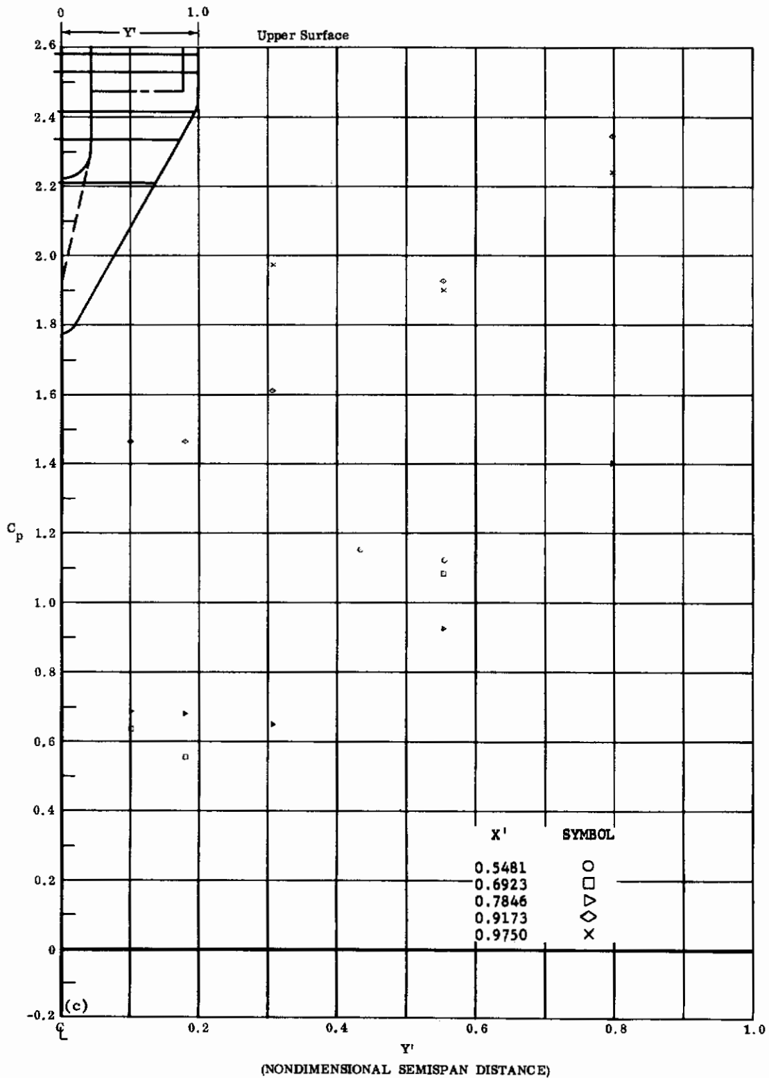
Fig. 47c Configuration IV, \alpha = -40 , \delta_2 = \delta_3 = -10
