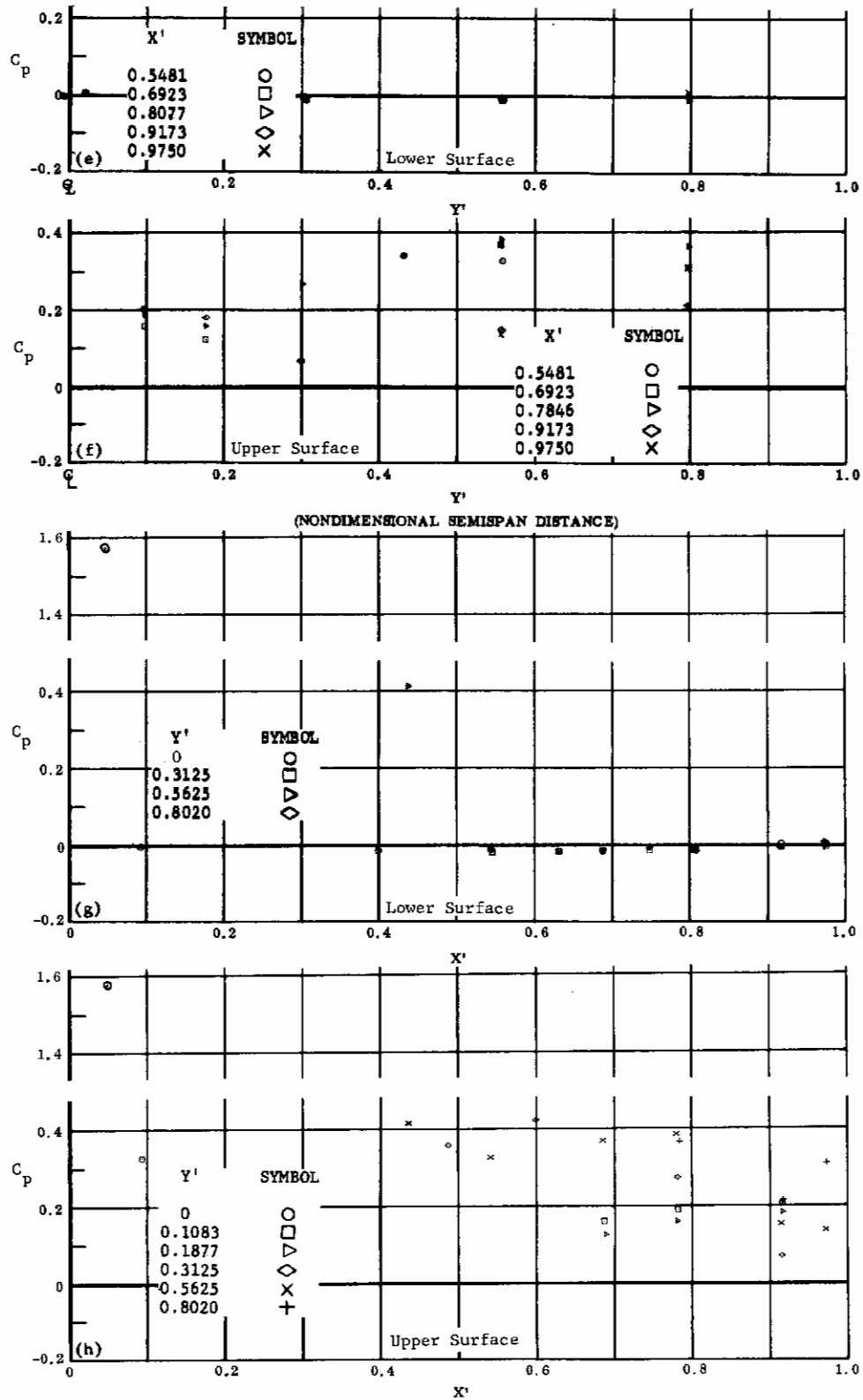
Fig. 42 Configuration IV, \alpha = -20 , \delta_2 = \delta_3 = +10
