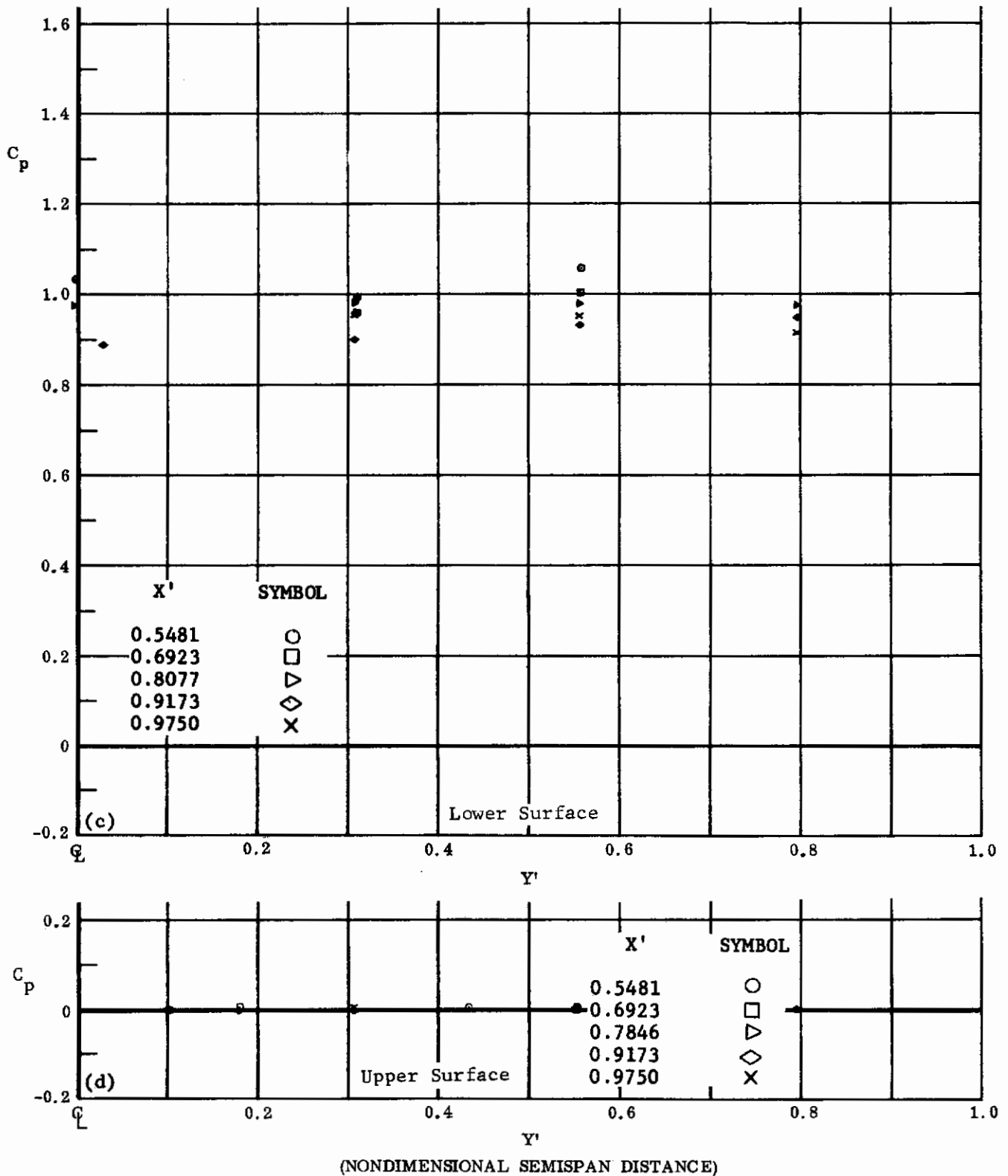
Fig. 11 Configuration I, \alpha = +40 , \delta_2 = \delta_3 = 0
