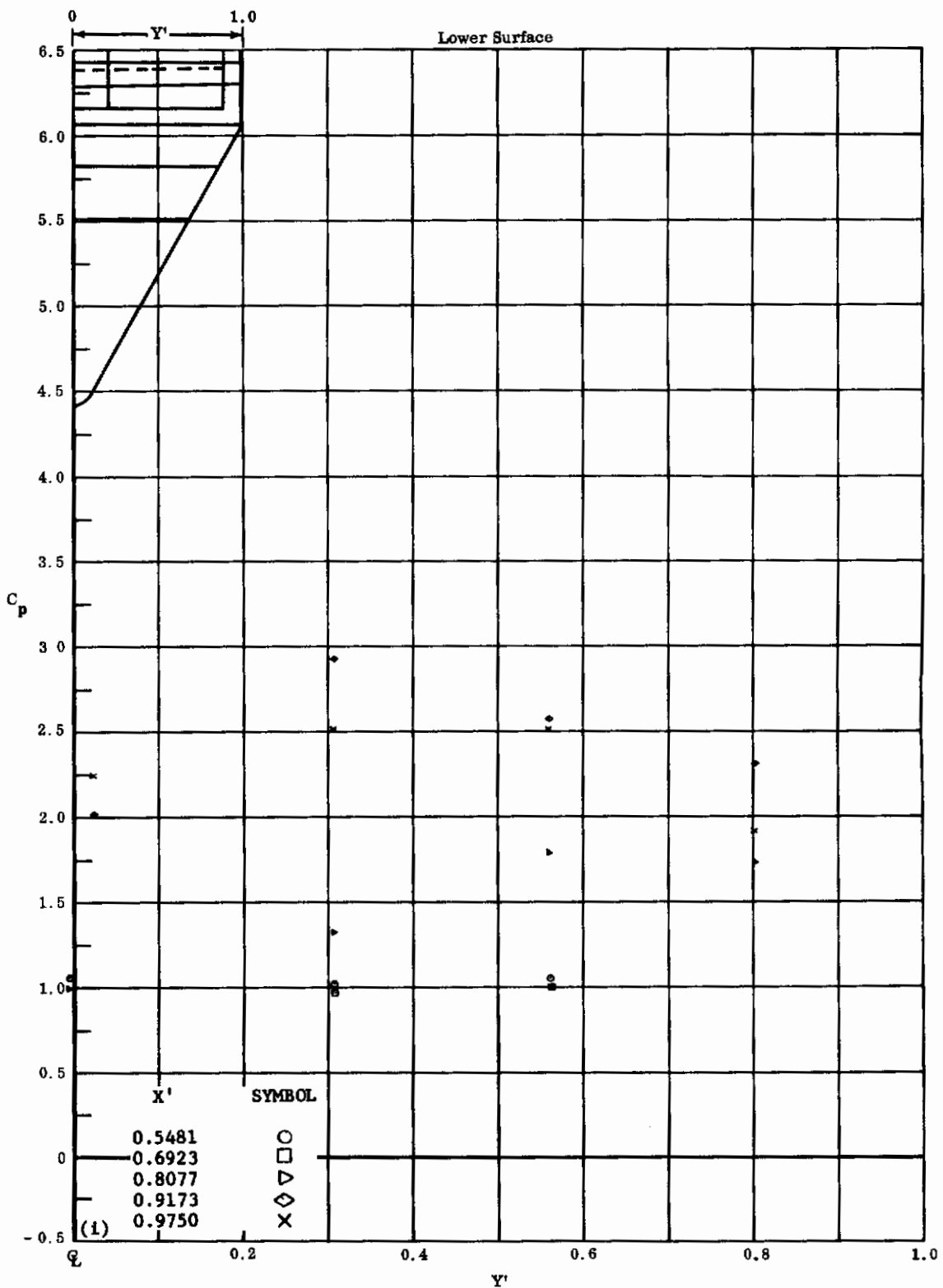
(NONDIMENSIONAL SEMISPAN DISTANCE) Fig. 111 Configuration I, \alpha = +40^\circ , \delta_2 = \delta_3 = +20 C_p vs. Y' , lower surface
