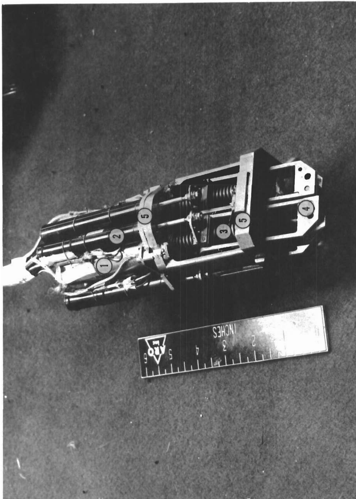
Figure 12 Photograph - Actuator Assembly (1) Electric Motors, (2) Potentiometers, (3) Lead Screws, (4) Control Rods (5) Water Cooled Bulkheads
