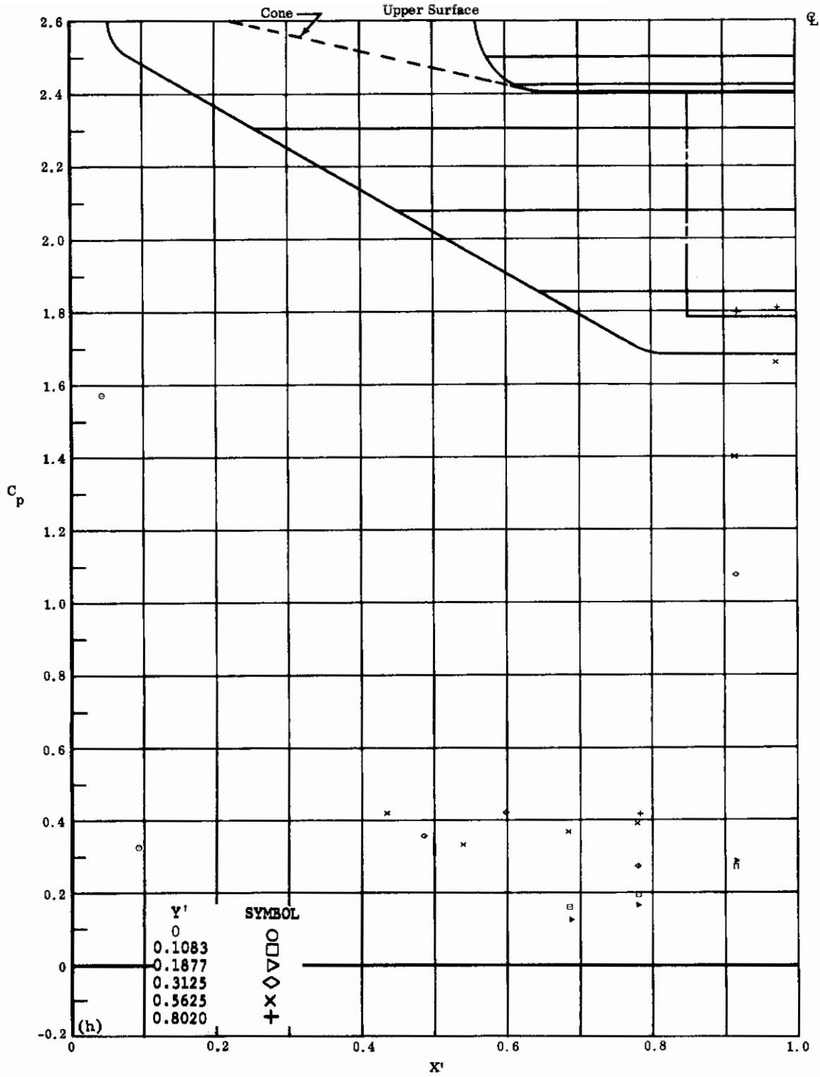
Fig. 43h Configuration IV, \alpha = -20 , \delta_2 = \delta_3 = -20
