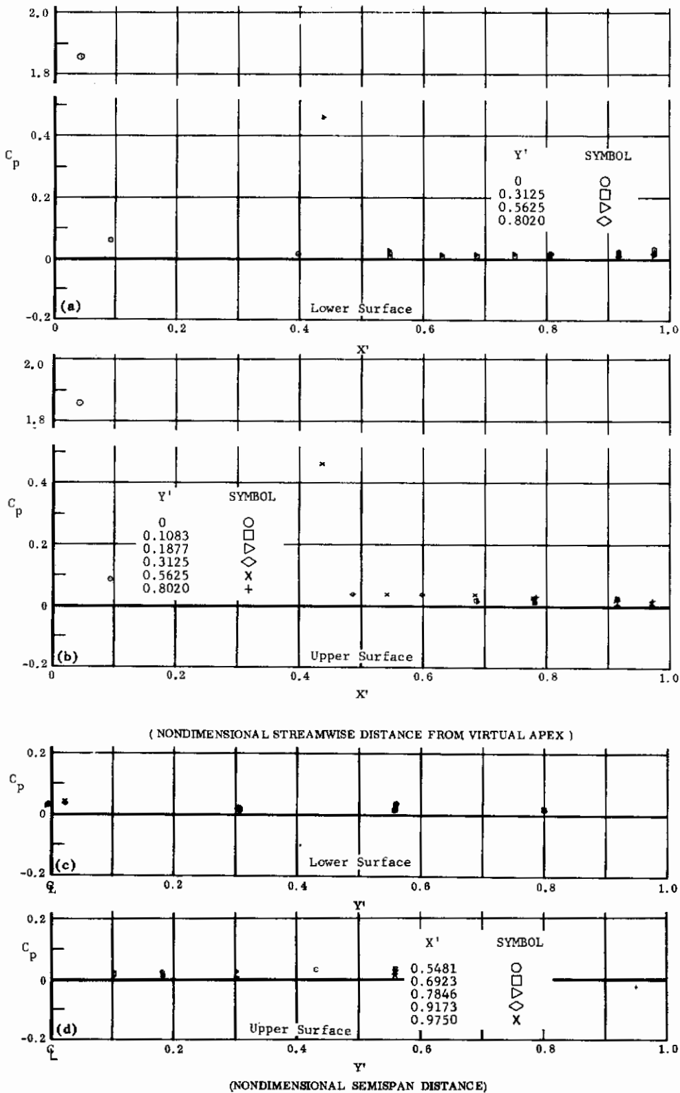
Fig. 3 Configuration I, \alpha = 0 , \delta_2 = \delta_3 = 0
