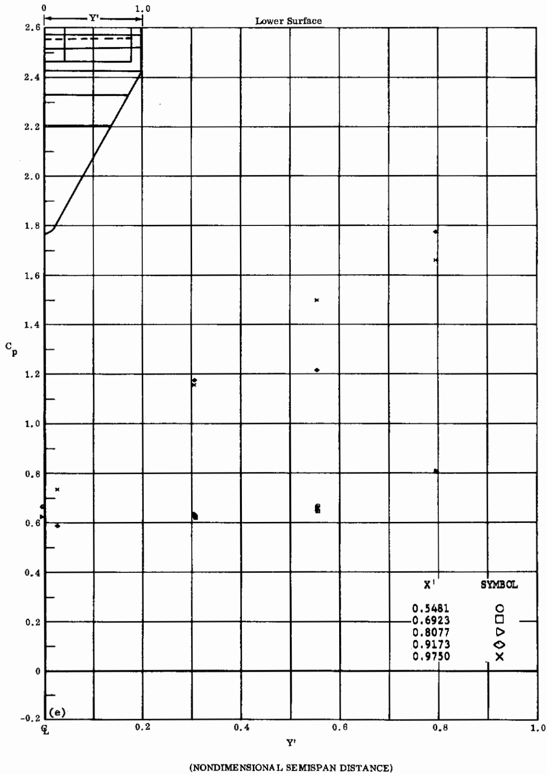
Fig. 35e Configuration IV, \alpha = +30 , \delta_2 = \delta_3 = +10
