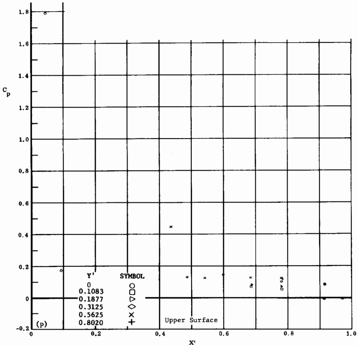
Fig. 16 Configuration I, \alpha = -10 , \delta_2 = \delta_3 = +30
