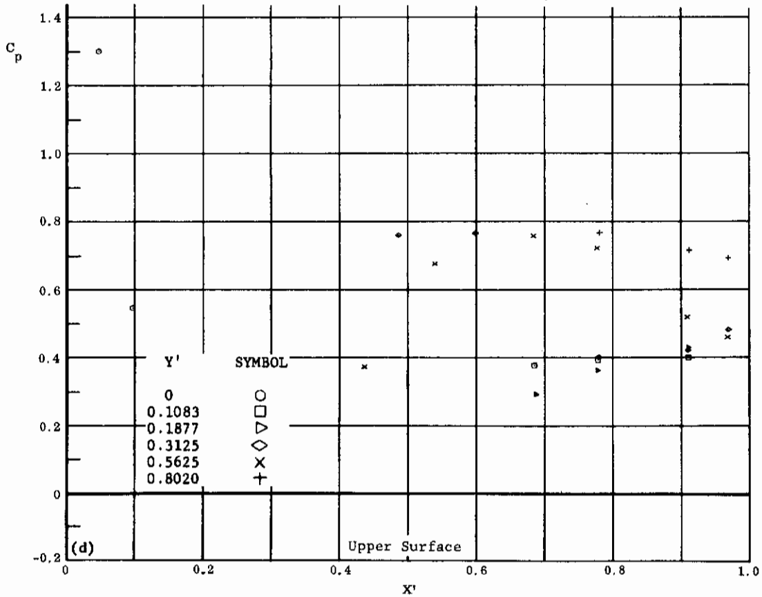
Fig. 22 Configuration I, \alpha = -30 , \delta_2 = \delta_3 = 0
