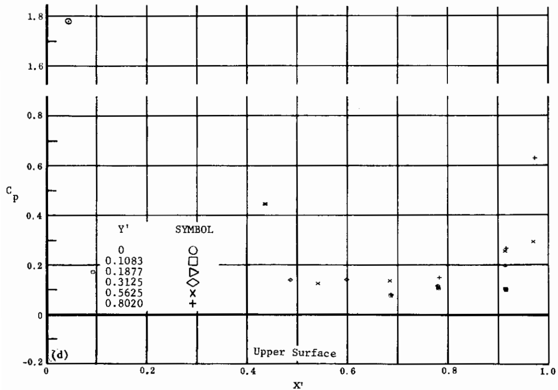
Fig. 41 Configuration IV, \alpha = -10 , \delta_2 = \delta_3 = -10
