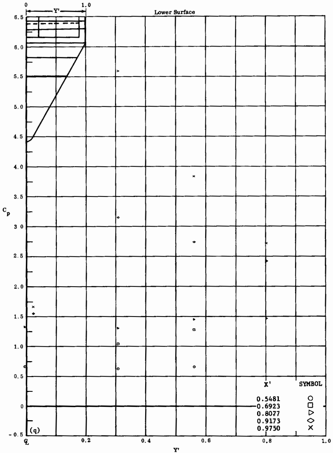
Fig. 9q Configuration I, \alpha = +30 , \delta_2 = \delta_3 = +39
