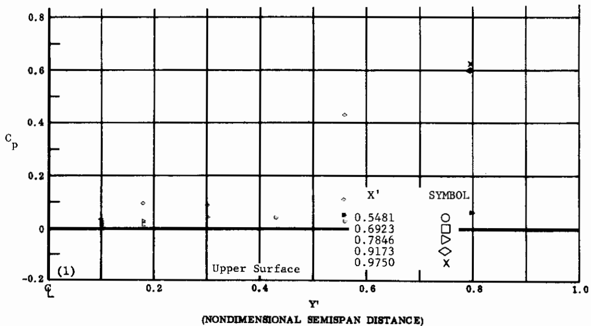
Fig. 4 Configuration I, \alpha = 0 , \delta_2 = \delta_3 = -30
