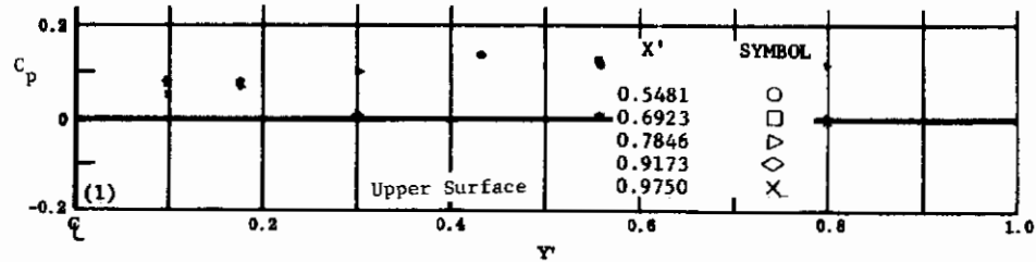
Fig. 16 Configuration I, \alpha = -10 , \delta_2 = \delta_3 = +20
