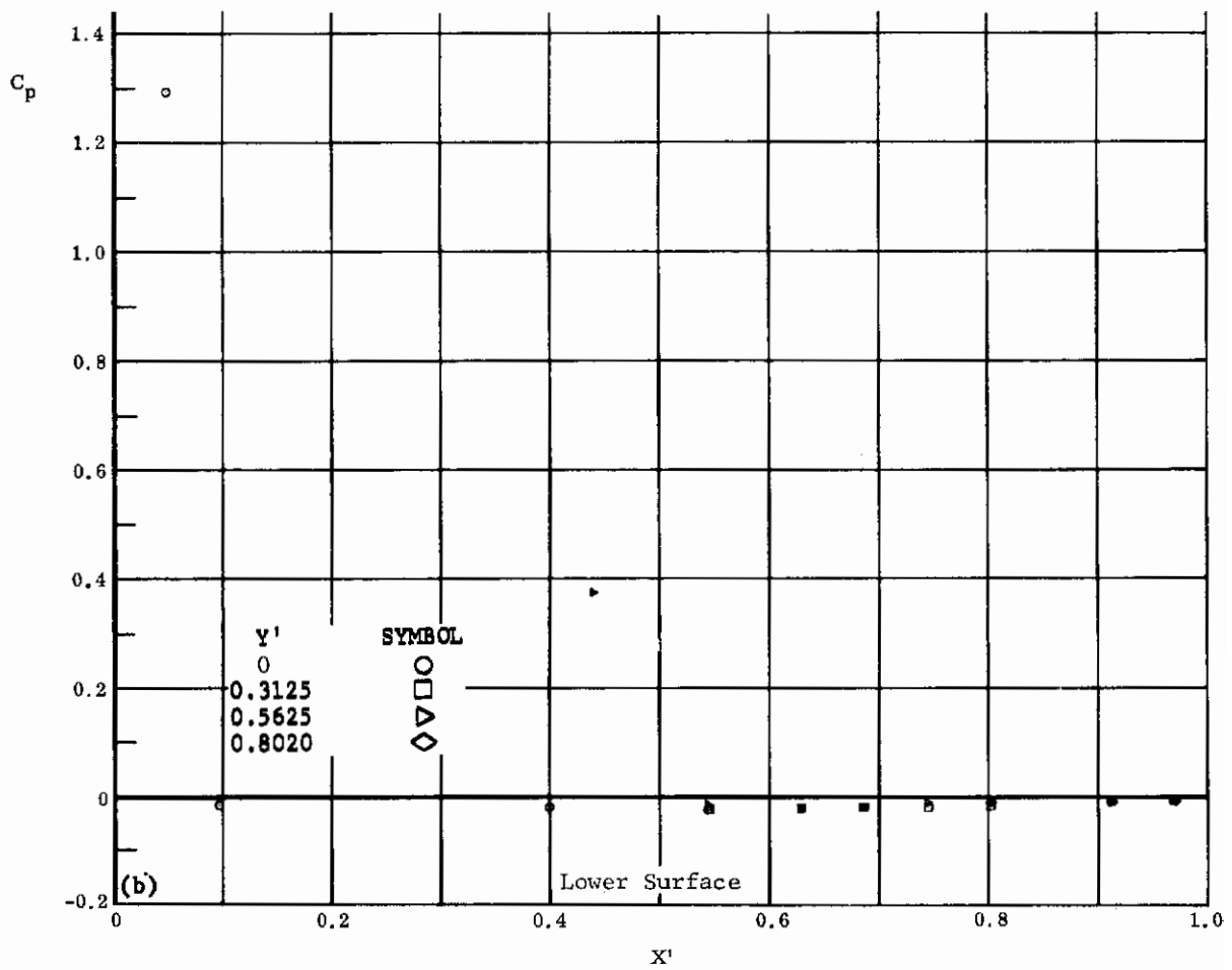
Fig. 44 Configuration IV, \alpha = -30 , \delta_2 = \delta_3 = 0
