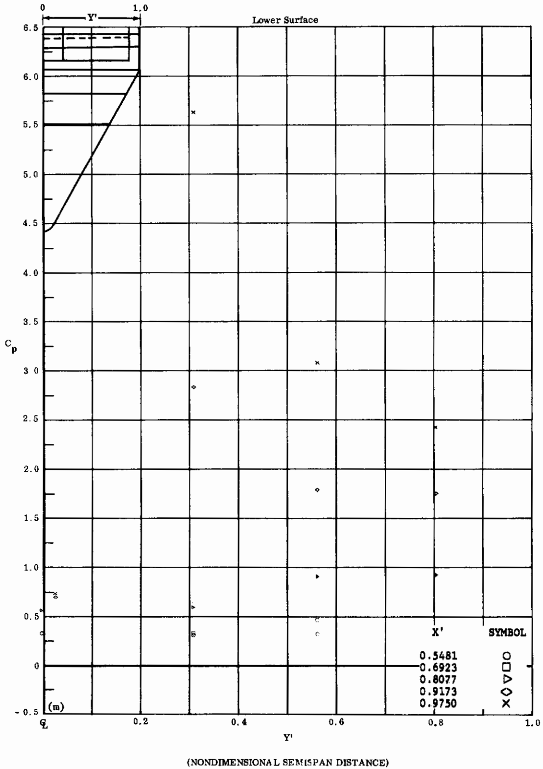
Fig. 33m Configuration IV, \alpha = +20 , \delta_2 = \delta_3 = +30
