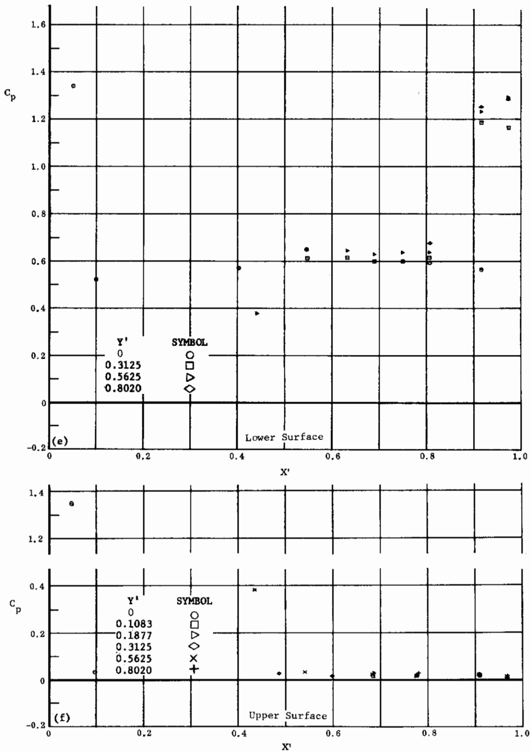
Fig. 9 Configuration I, \alpha = +30 , \delta_2 = \delta_3 = +10
