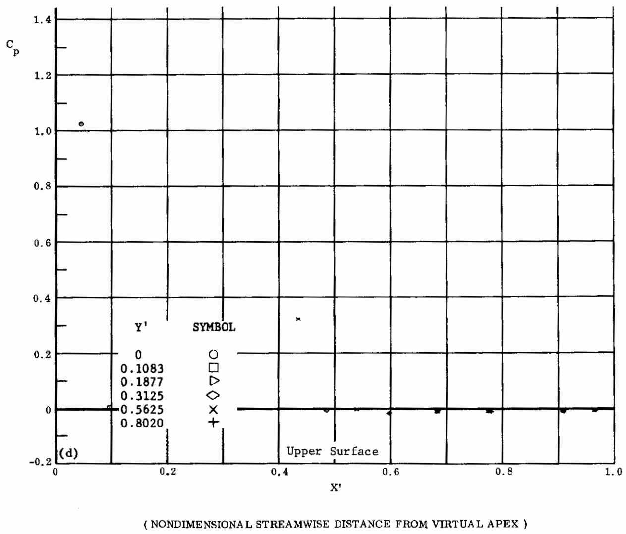
Fig. 37 Configuration IV, \alpha = +40 , \delta_2 = \delta_3 = 0
