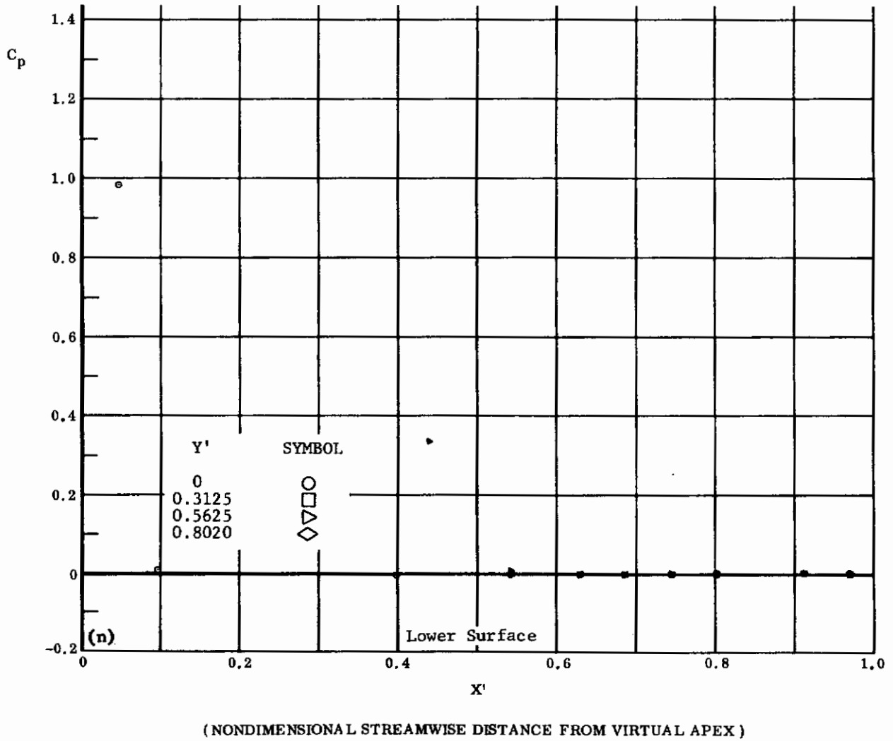
Fig. 47 Configuration IV, \alpha = -40 , \delta_2 = \delta_3 = -39
