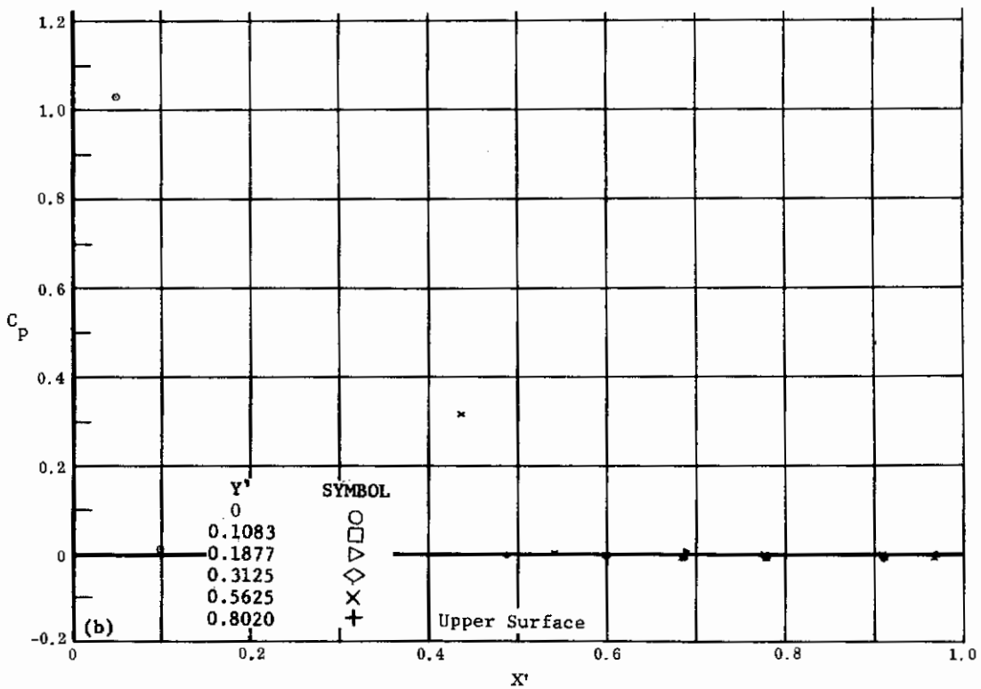
Fig. 11 Configuration I, \alpha = +40 , \delta_2 = \delta_3 = 0
