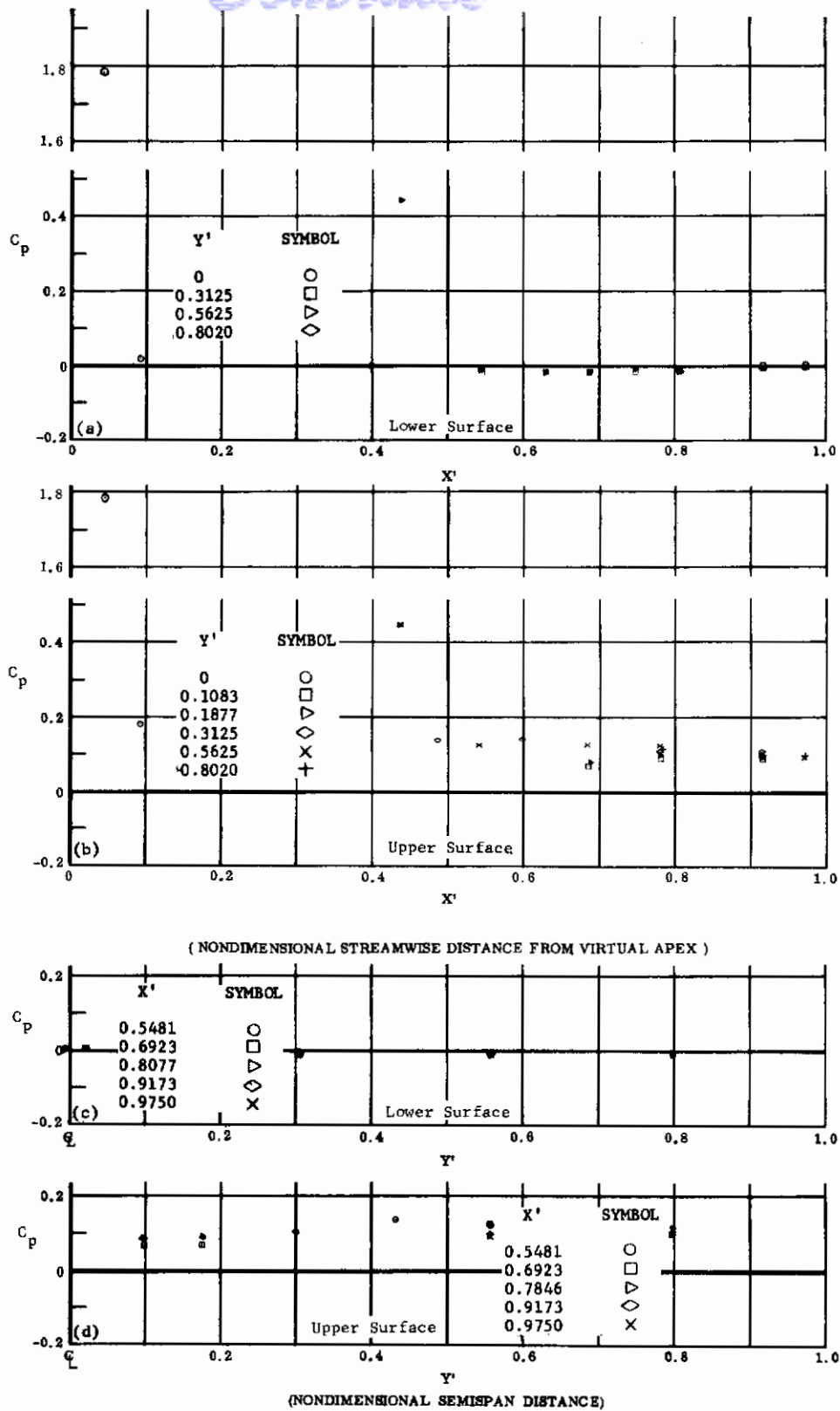
Fig. 16 Configuration I, \alpha = -10 , \delta_2 = \delta_3 = 0
