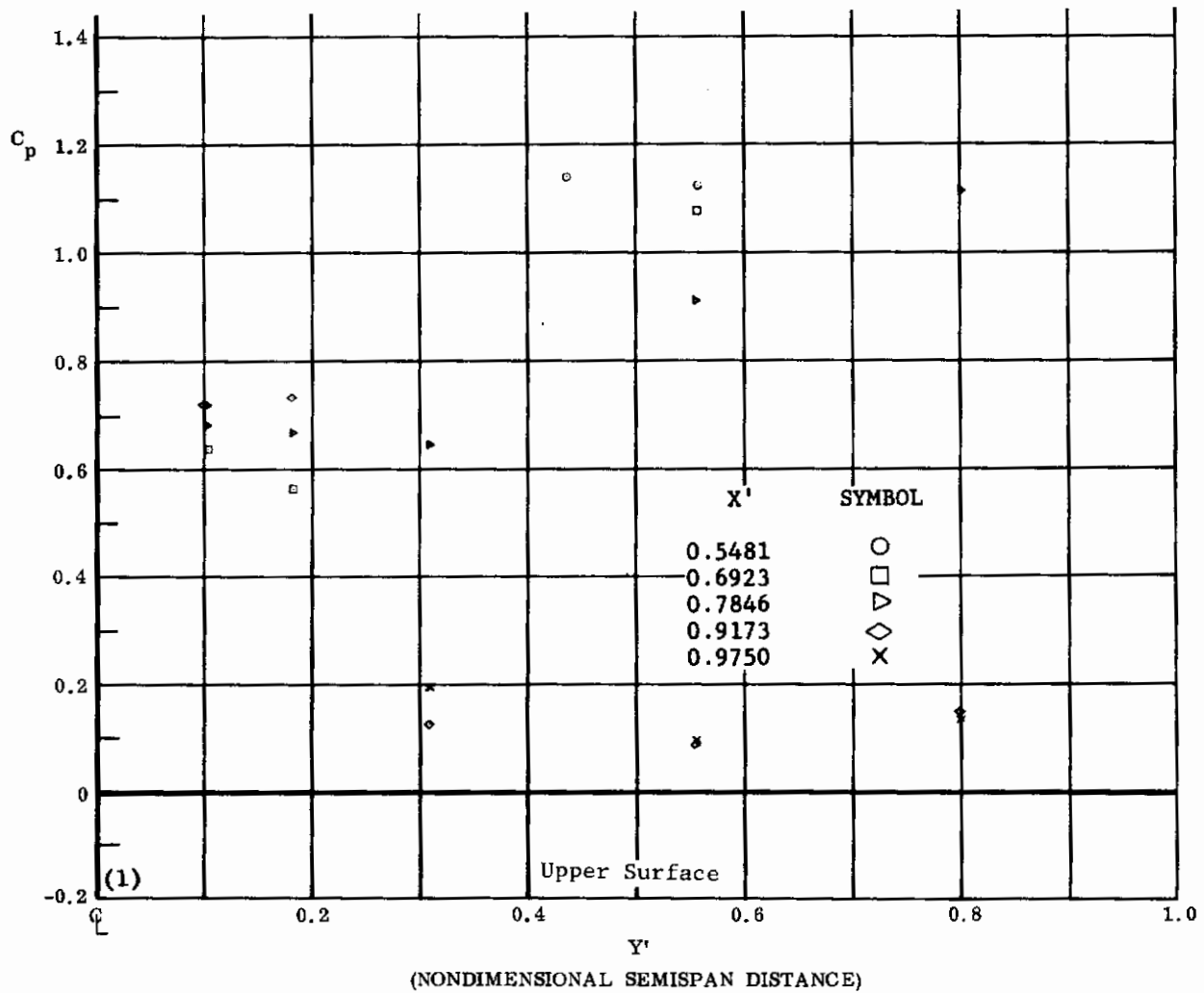
Fig. 25 Configuration I, \alpha = -40 , \delta_2 = \delta_3 = +30
