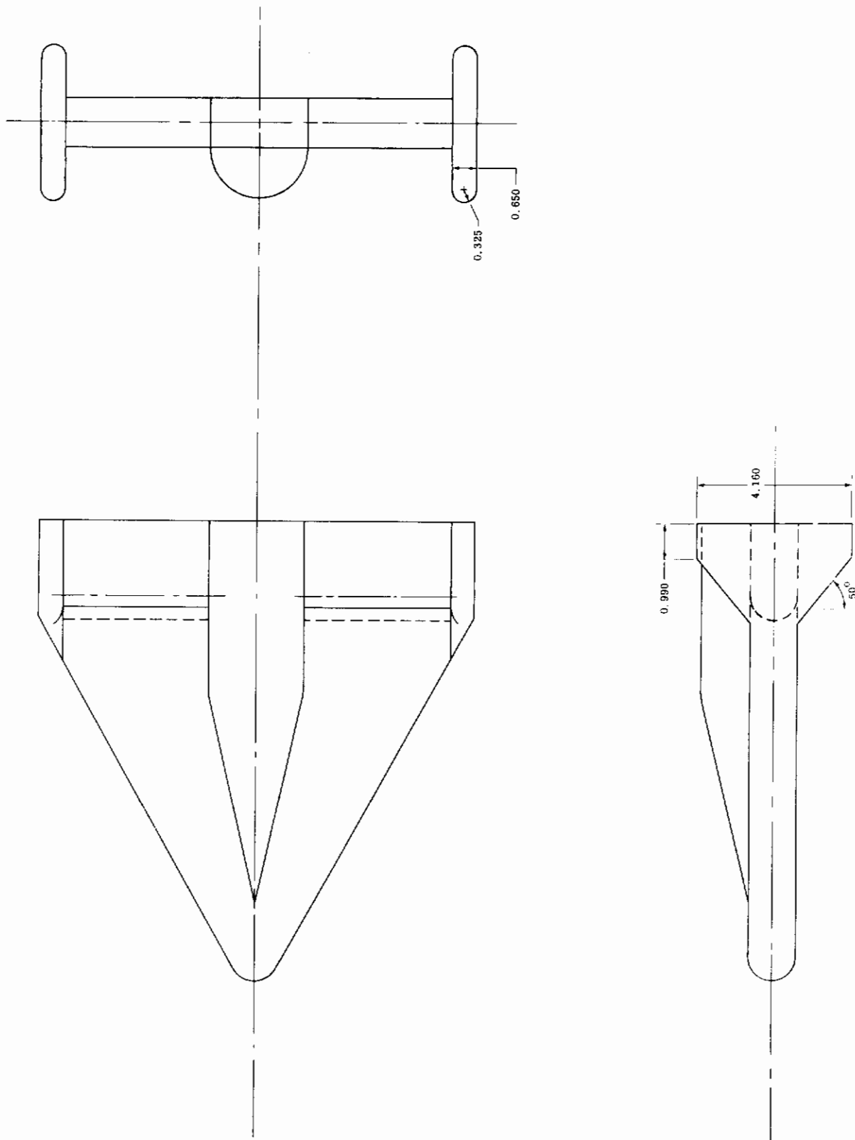
Fig. 1c Configuration IV - Basic Wing-Body + Tip Fins (for dimensions see Figure 1b)
