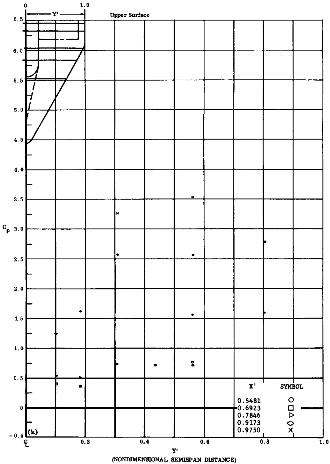
Fig. 45k Configuration IV, \alpha = -30 , \delta_2 = \delta_3 = -30
