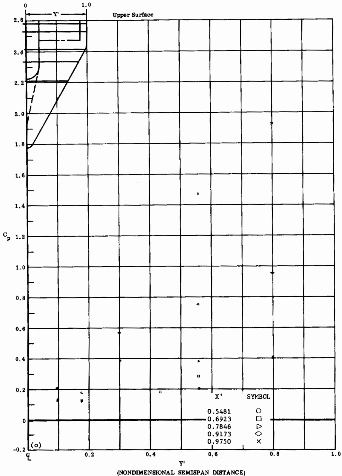
Fig. 170 Configuration I, \alpha = -10 , \delta_2 = \delta_3 = -39
