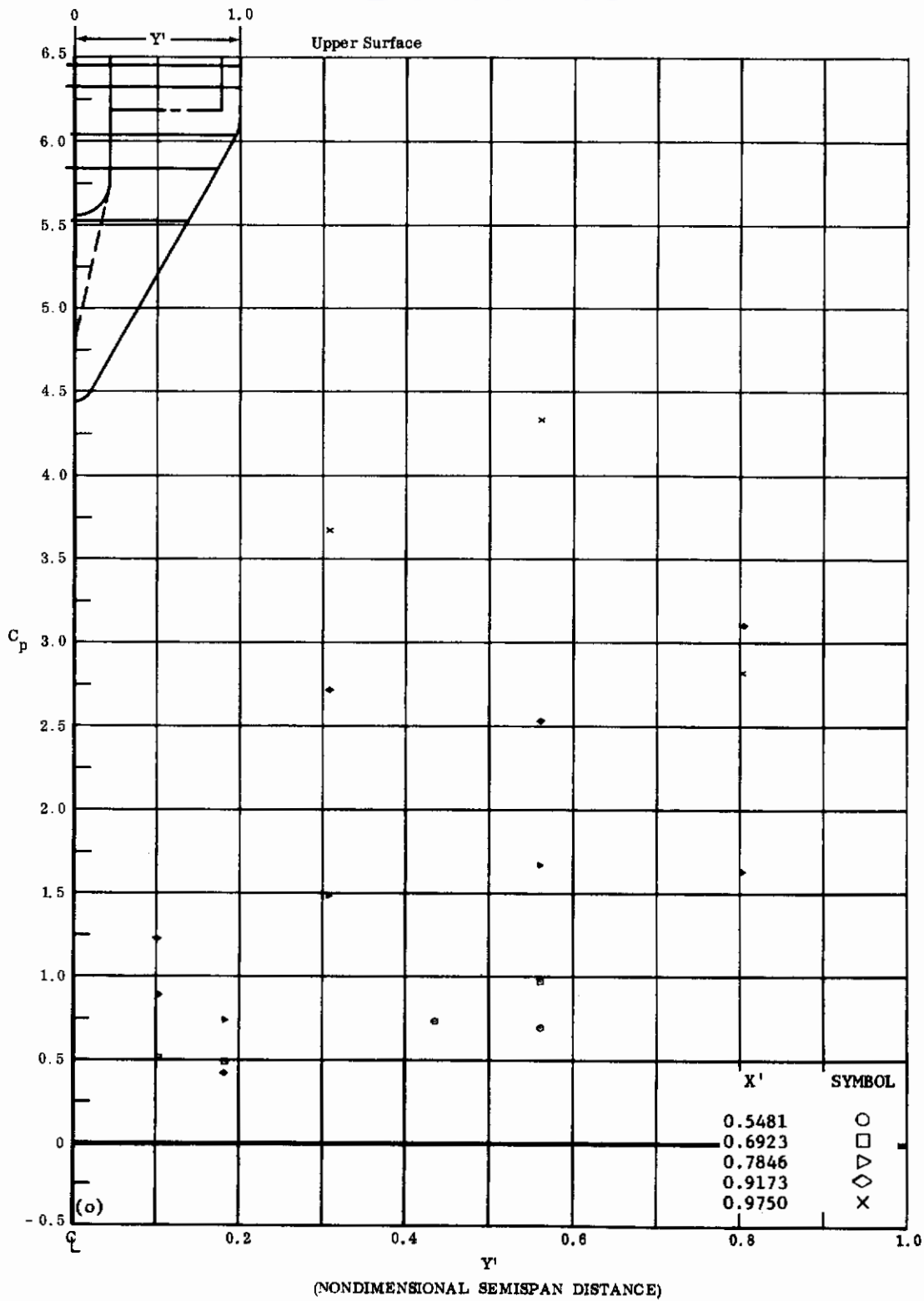
Fig. 23o Configuration I, \alpha = -30 , \delta_2 = \delta_3 = -39
