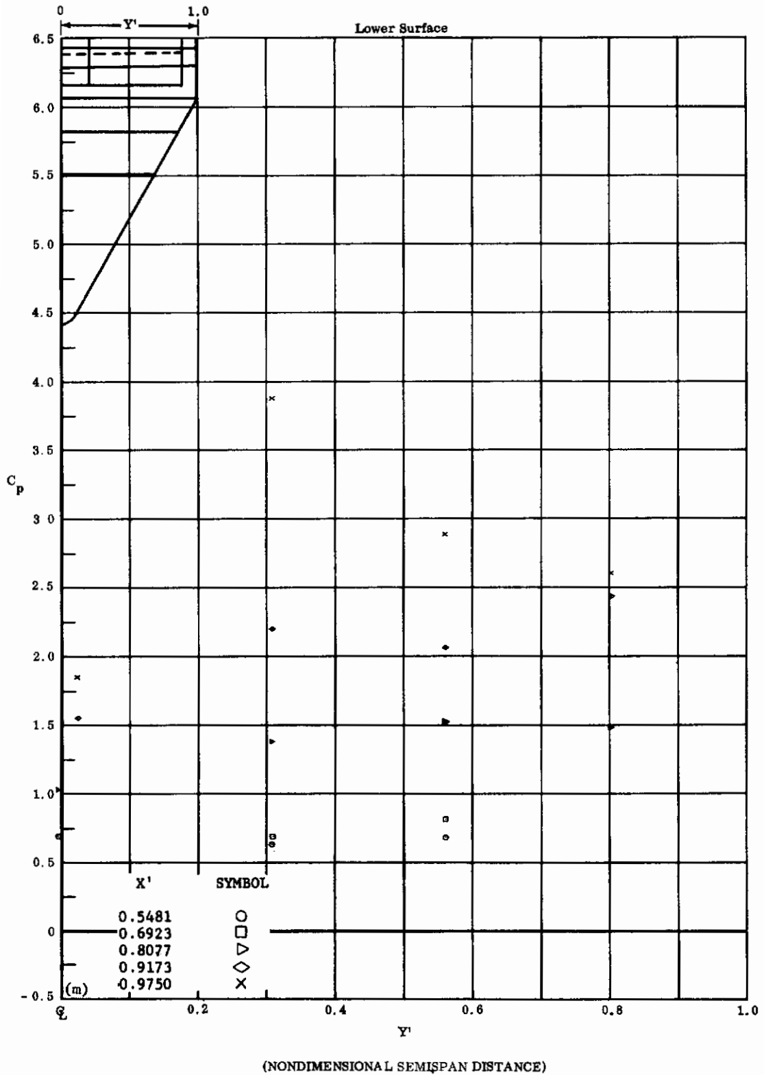
Fig. 35m Configuration IV, \alpha = +30 , \delta_2 = \delta_3 = +30 C_p vs. Y' , lower surface
