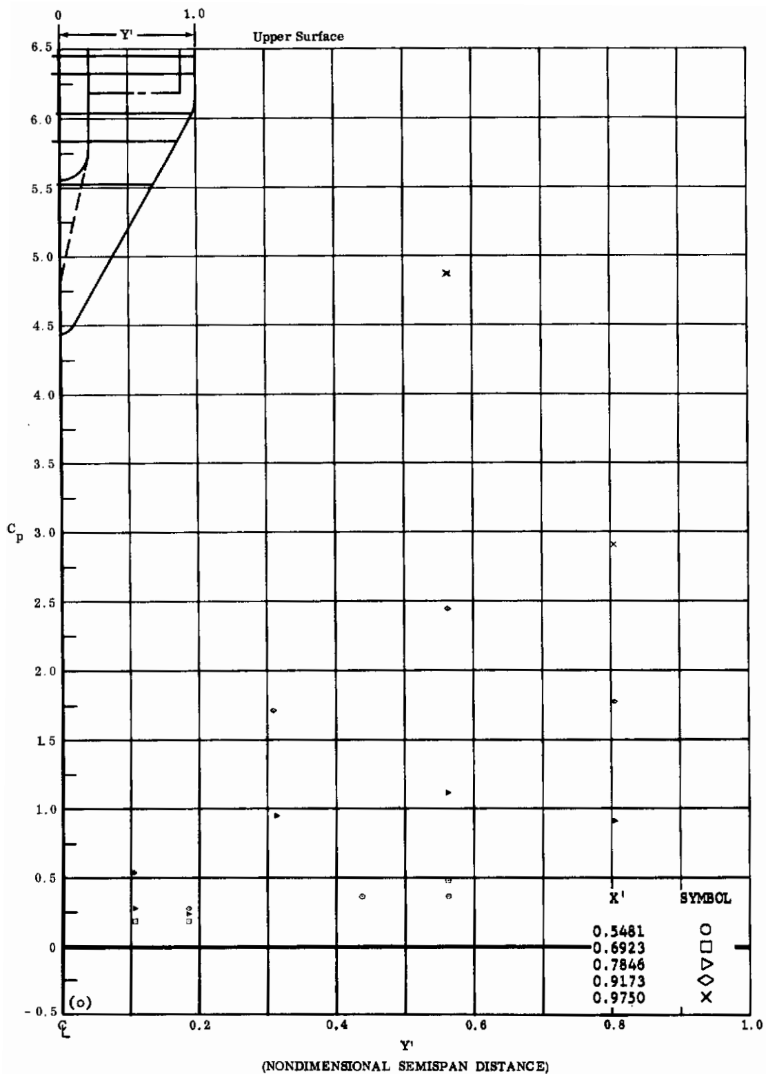
Fig. 20c Configuration I, \alpha = -20 , \delta_2 = \delta_3 = -39 C_p vs. Y' , upper surface
