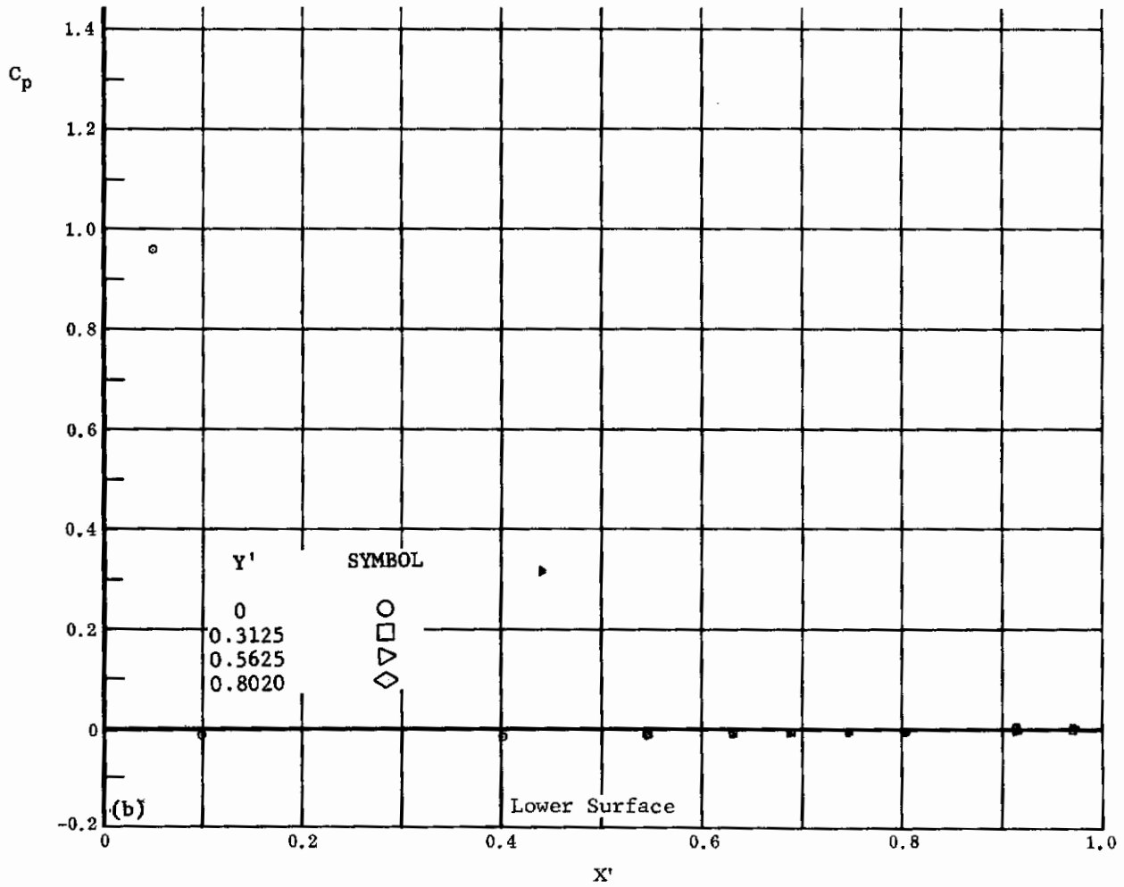
Fig. 46 Configuration IV, \alpha = -40 , \delta_2 = \delta_3 = 0
