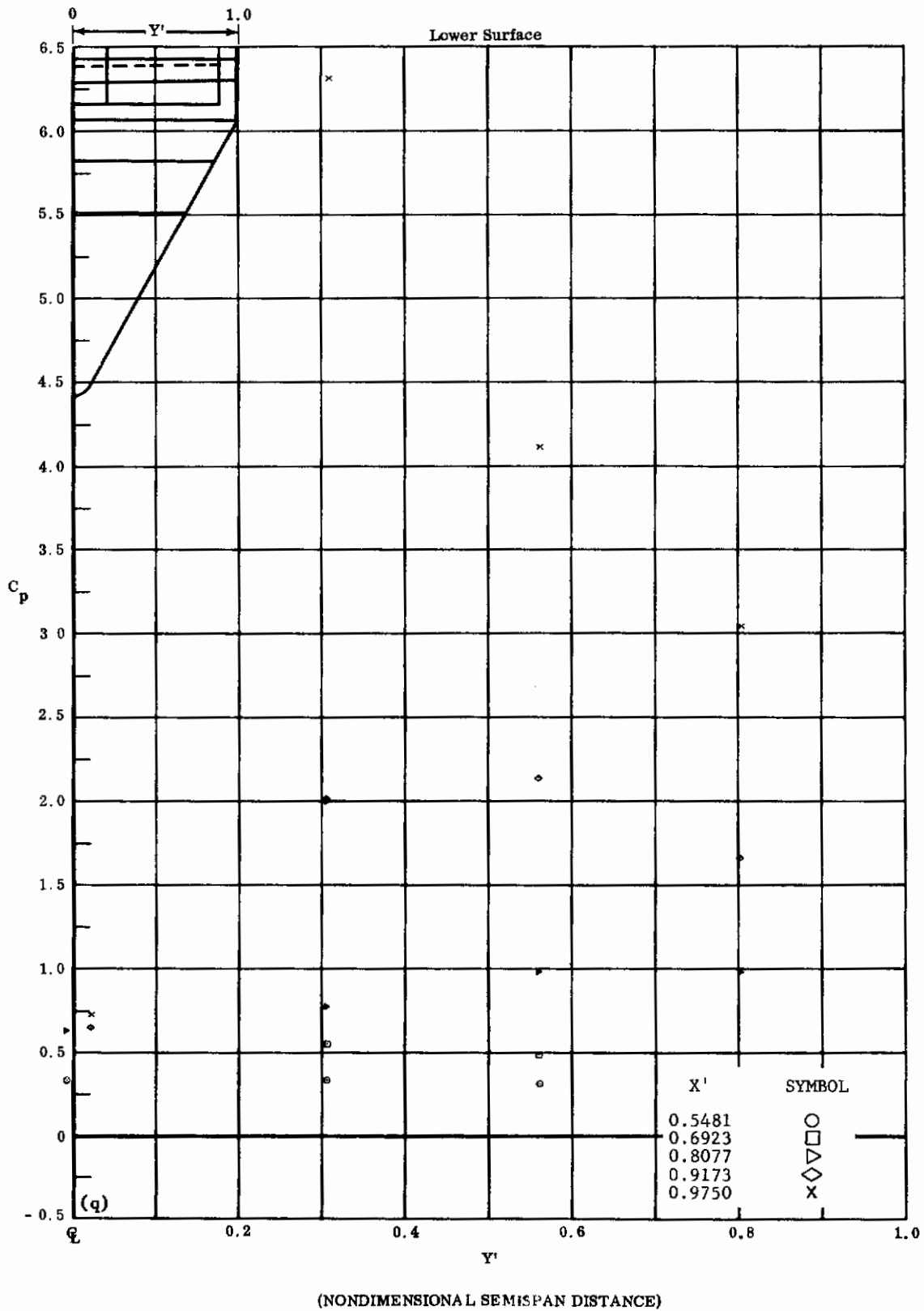
Fig. 7q Configuration I, \alpha = +20 , \delta_2 = \delta_3 = +39
