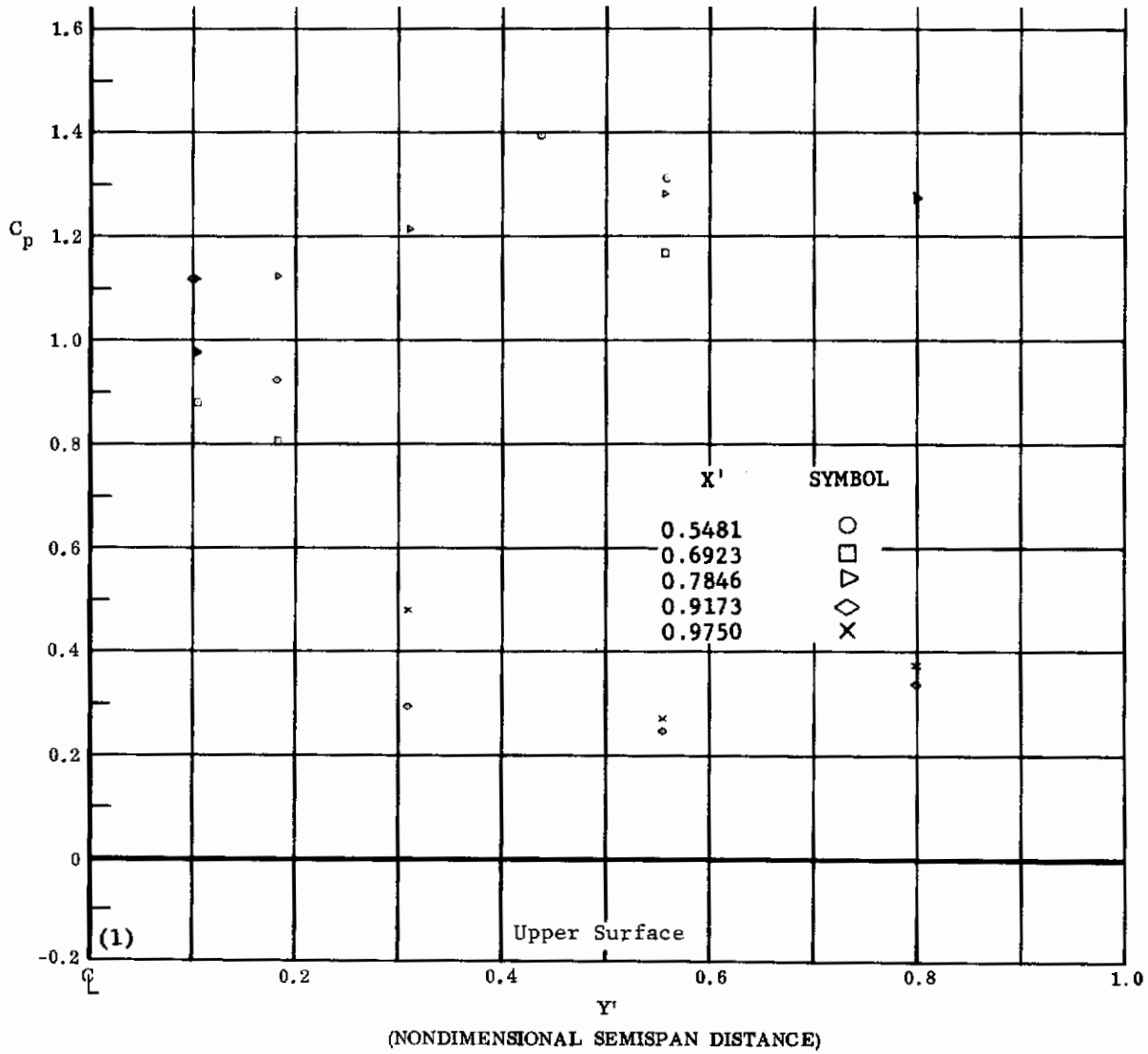
Fig. 27 Configuration I, \alpha = -50 , \delta_2 = \delta_3 = +30
