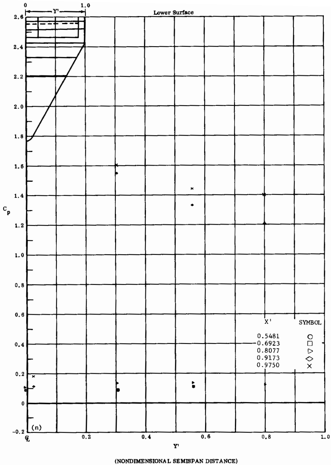
Fig. 5n Configuration I, \alpha = +10 , \delta_2 = \delta_3 = +30
