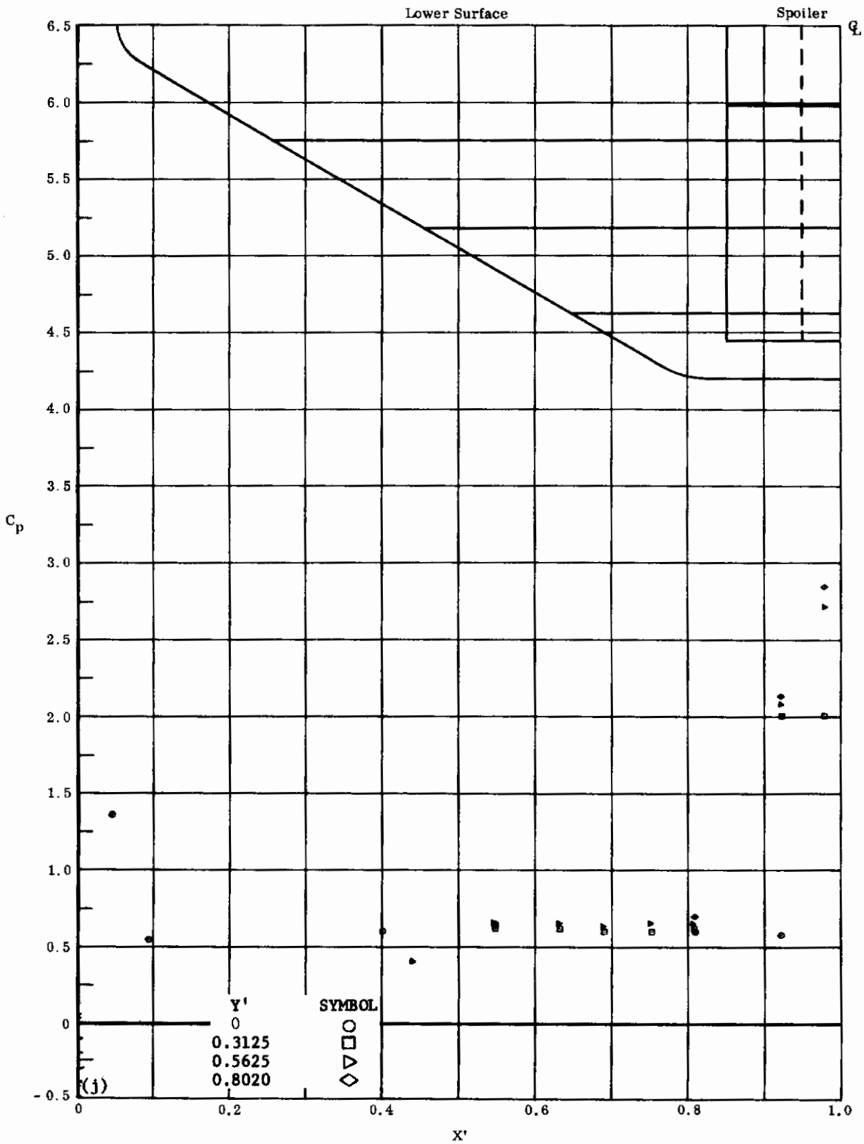
Fig. 9j Configuration I, \alpha = +30 , \delta_2 = \delta_3 = +20
