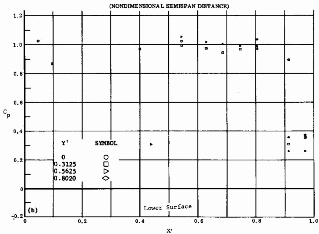
Fig. 12 Configuration I, \alpha = +40 , \delta_2 = \delta_3 = -20
