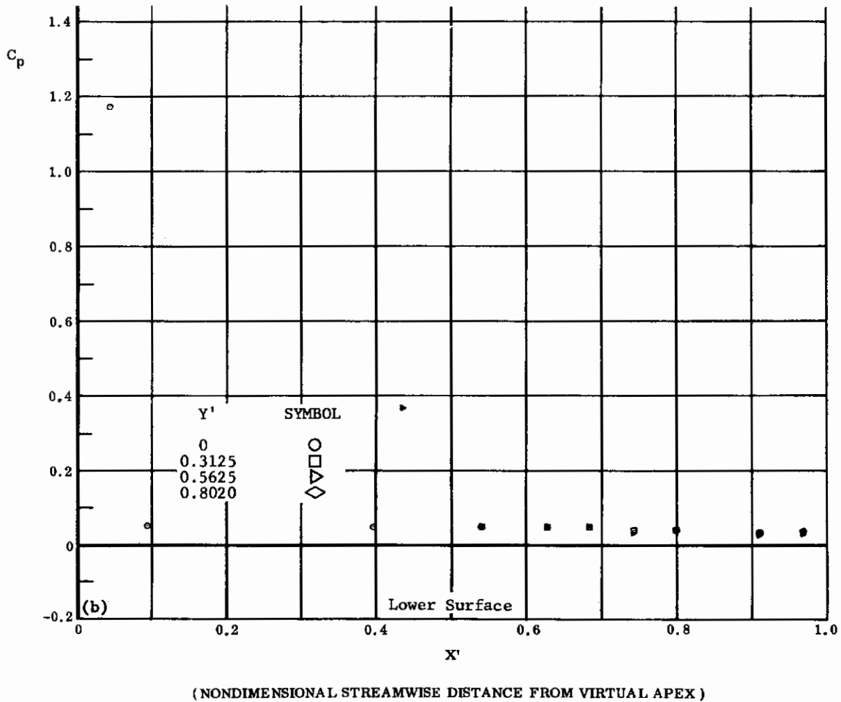
Fig. 24 Configuration I, \alpha = -35 , \delta_2 = \delta_3 = -30
