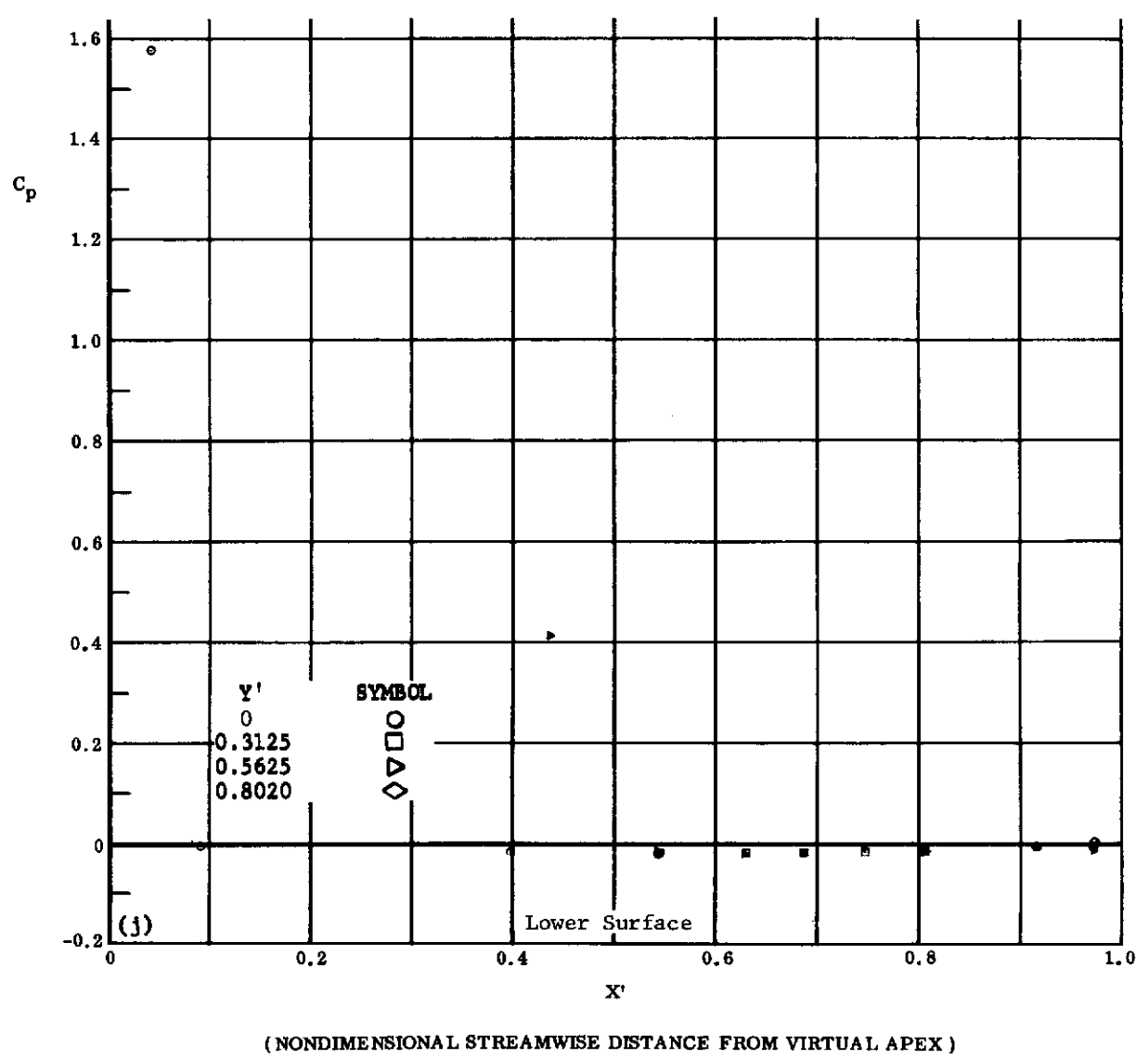
Fig. 43 Configuration IV, \alpha = -20 , \delta_2 = \delta_3 = -30
