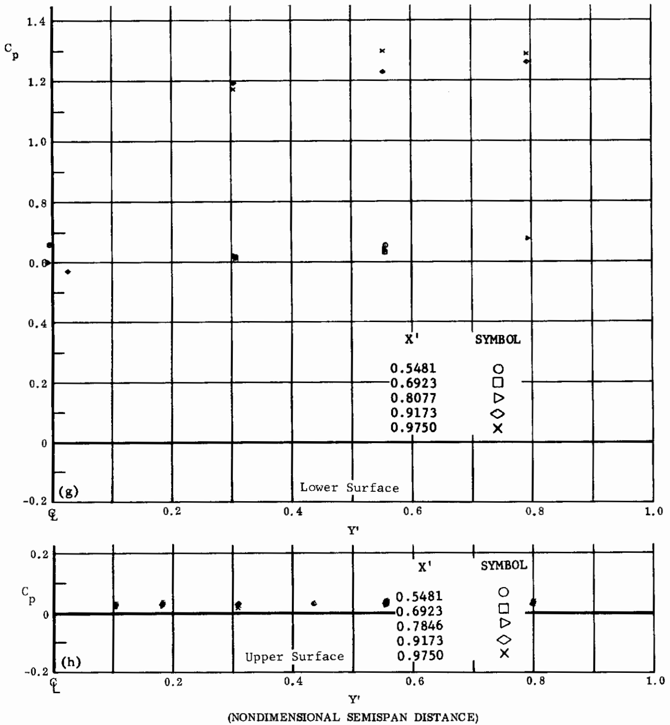
Fig. 9 Configuration I, \alpha = +30 , \delta_2 = \delta_3 = +10
