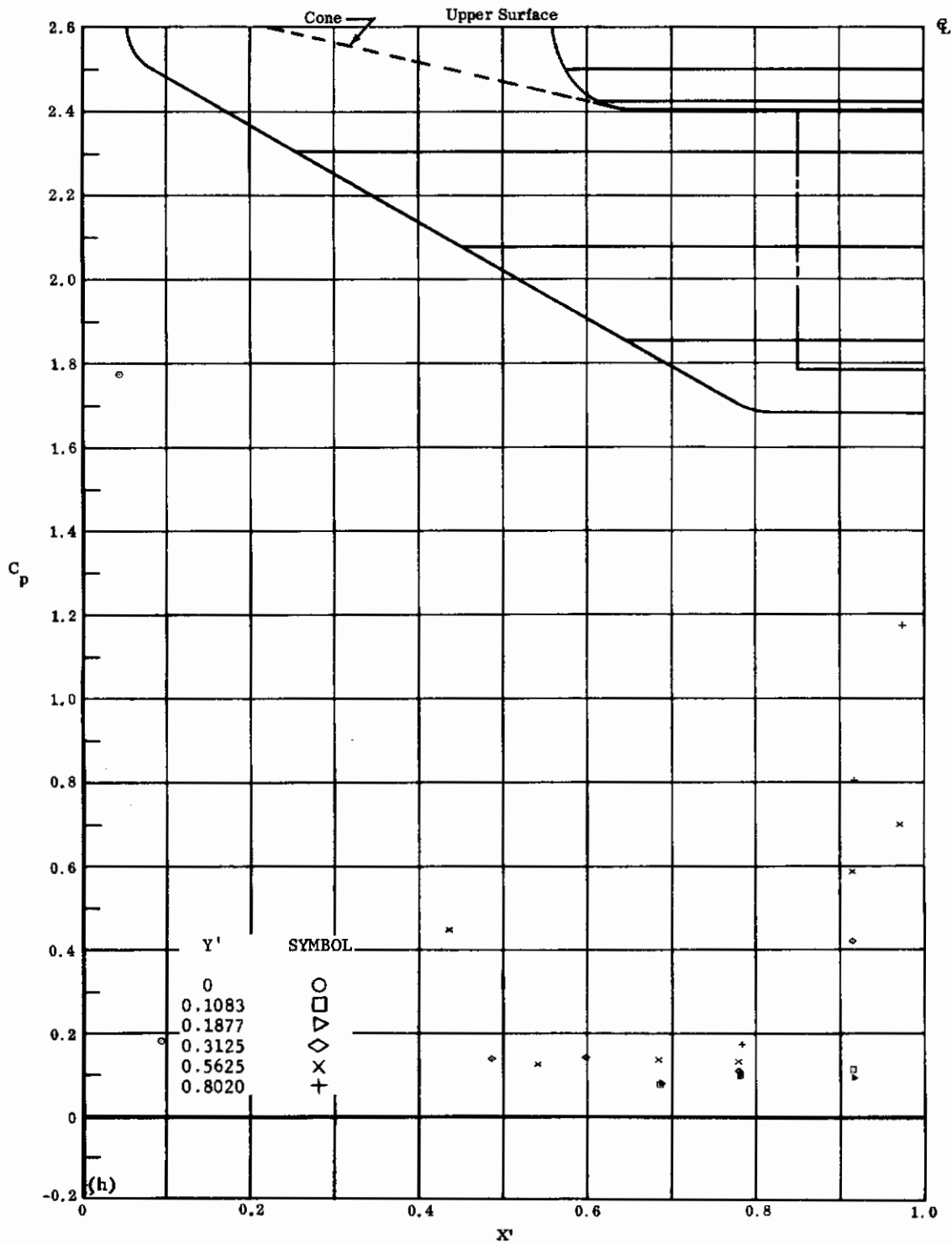
Fig. 4lh Configuration IV, \alpha = -10 , \delta_2 = \delta_3 = -20
