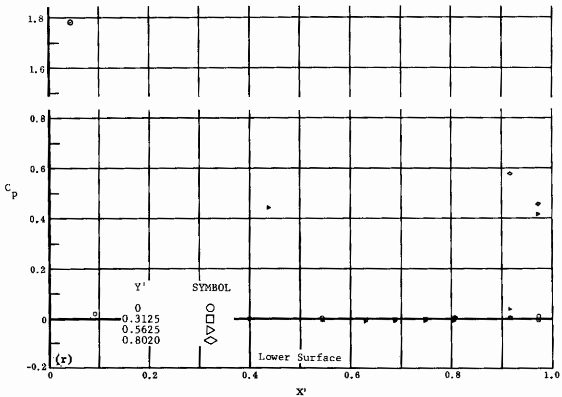
Fig. 16 Configuration I, \alpha = -10 , \delta_2 = \delta_3 = +39
