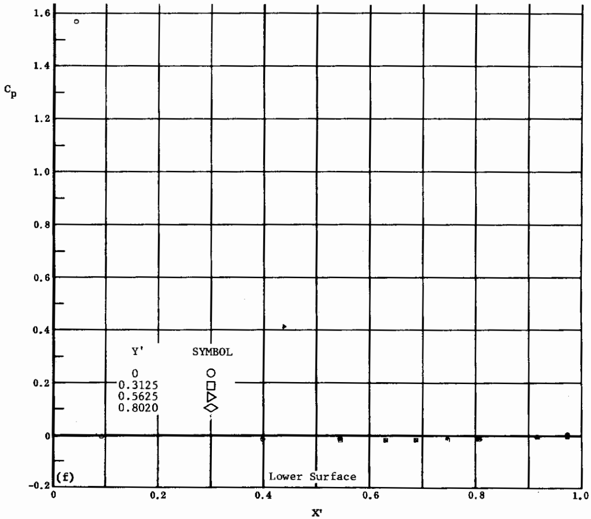
Fig. 19 Configuration I, \alpha = -20 , \delta_2 = \delta_3 = +10
