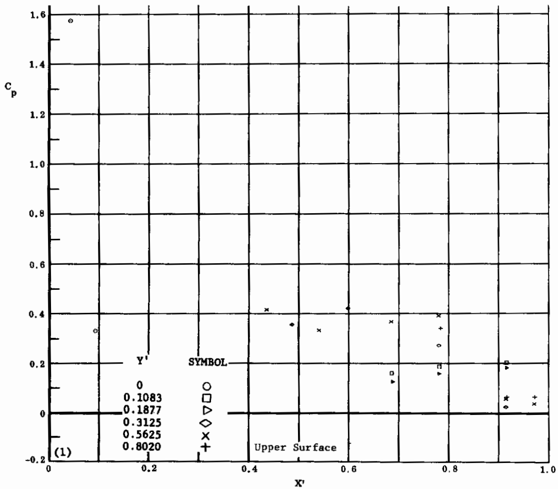
Fig. 19 Configuration I, \alpha = -20 , \delta_2 = \delta_3 = +20
