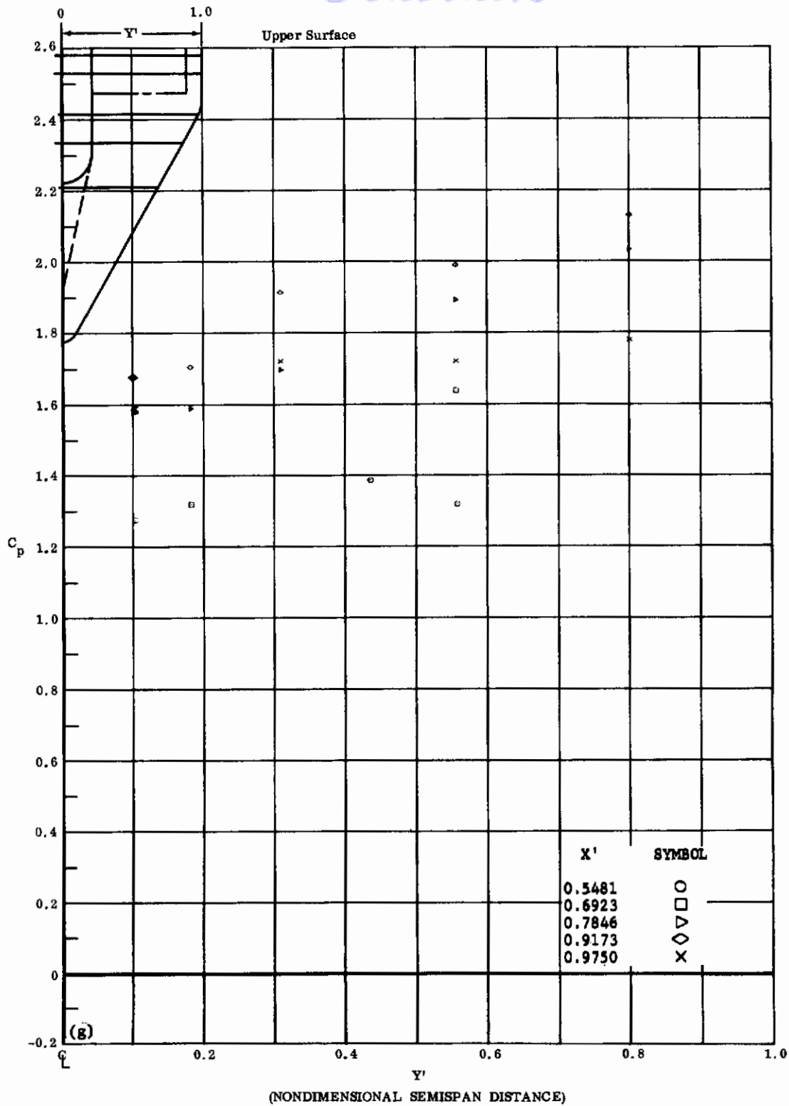
Fig. 49g Configuration IV, \alpha = -50 , \delta_2 = \delta_3 = -20
