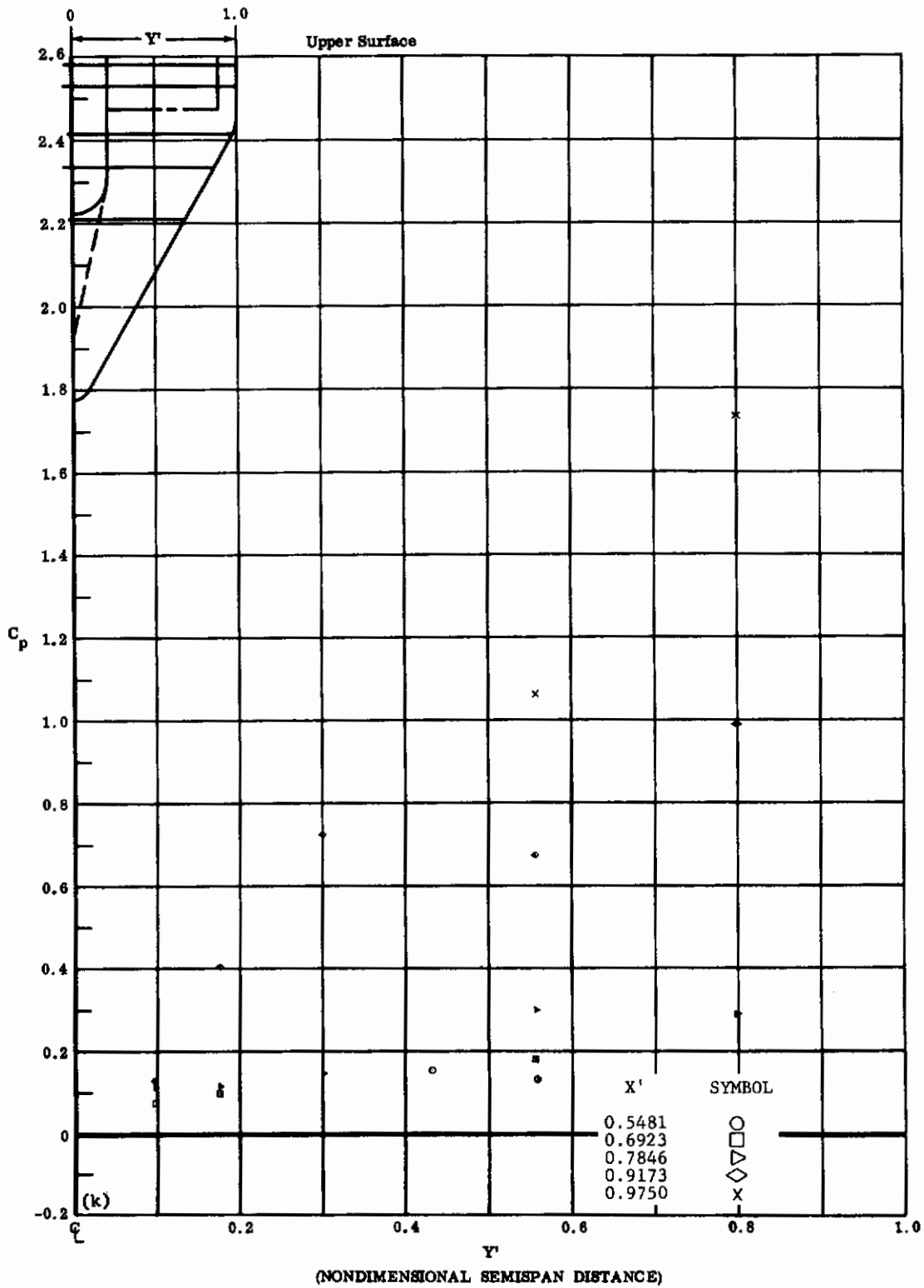
Fig. 41k Configuration IV, \alpha = -10 , \delta_2 = \delta_3 = -30
