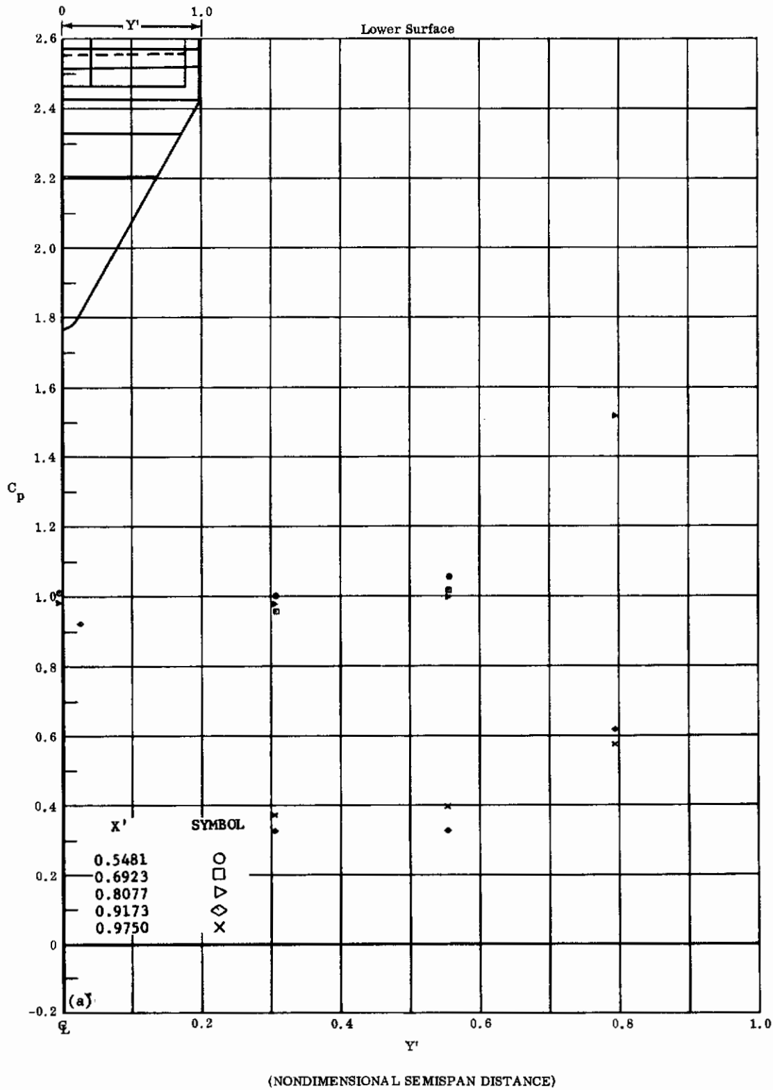
Fig. 38a Configuration IV, \alpha = +40 , \delta_2 = \delta_3 = -20 C_p vs. Y' , lower surface
