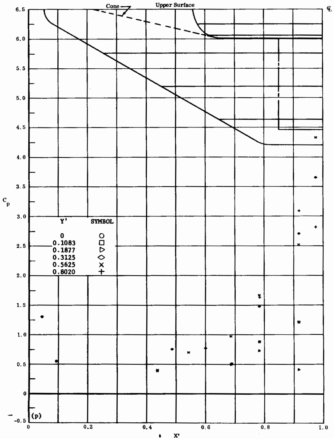
Fig. 23p Configuration I, \alpha = -30 , \delta_2 = \delta_3 = -39
