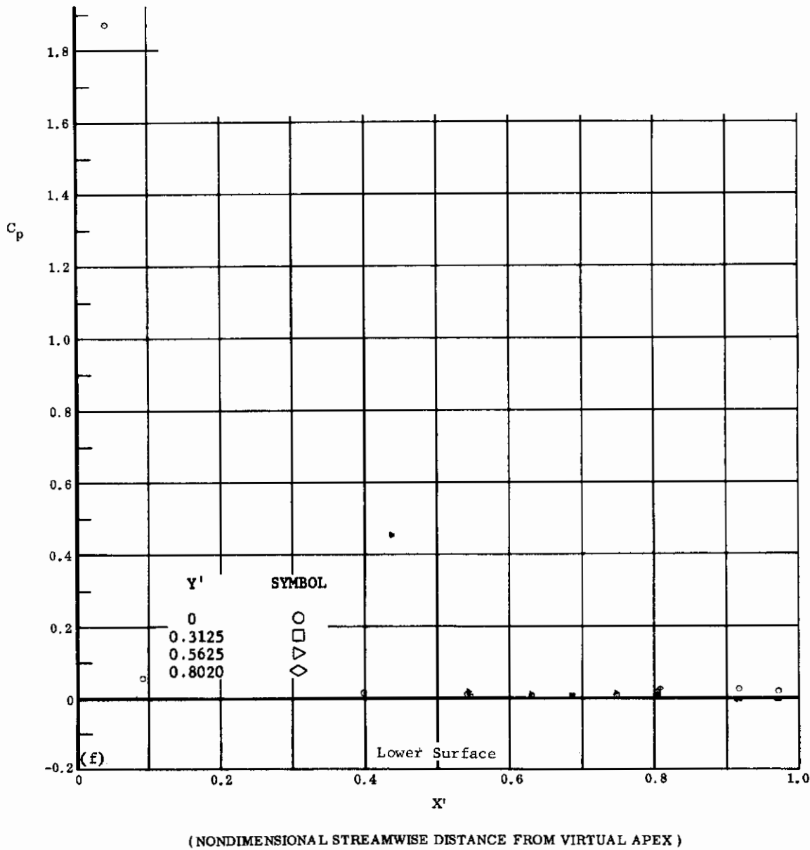
Fig. 30 Configuration IV, \alpha = 0 , \delta_2 = \delta_3 = -20
