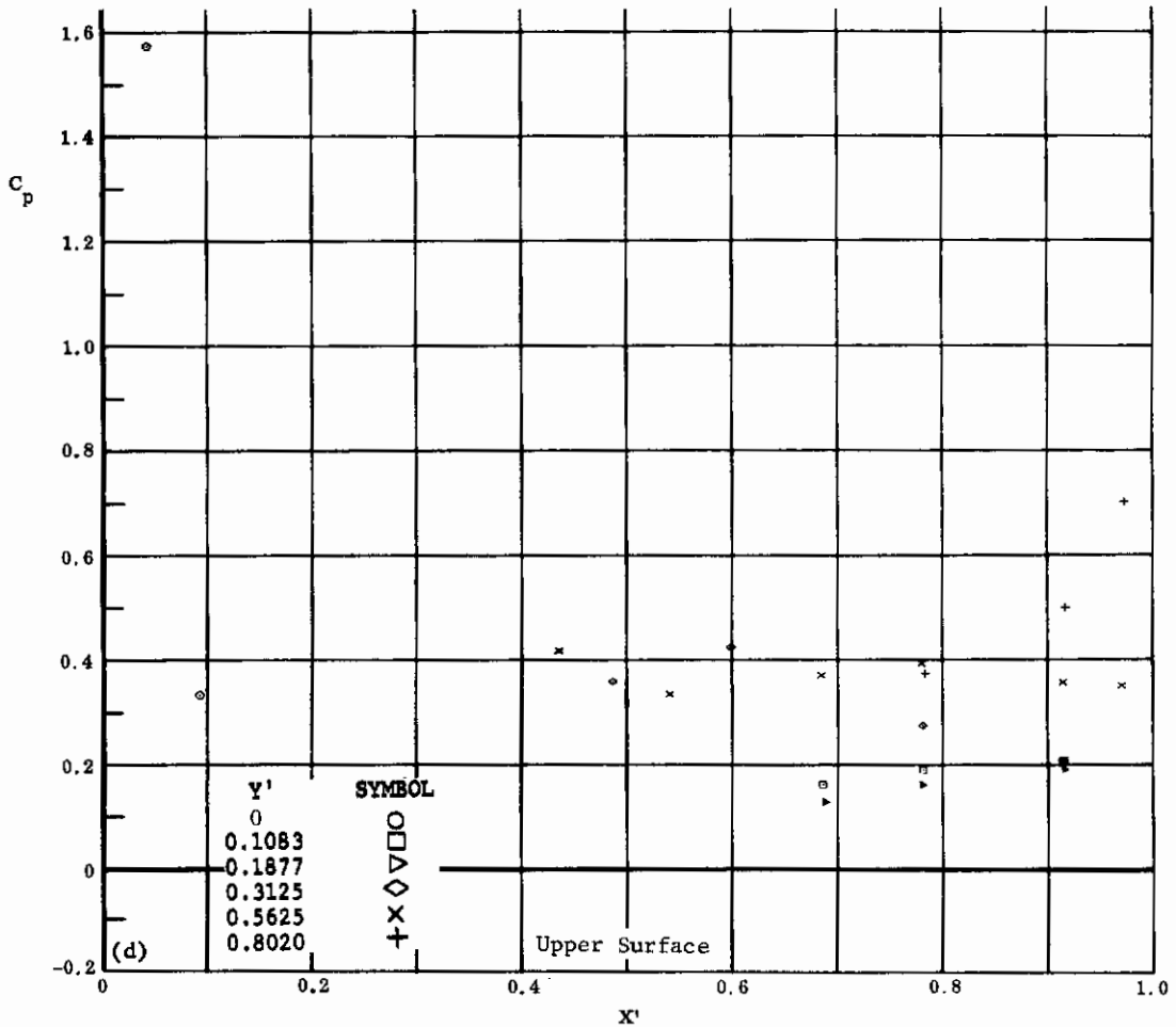
Fig. 42 Configuration IV, \alpha = -20 , \delta_2 = \delta_3 = 0
