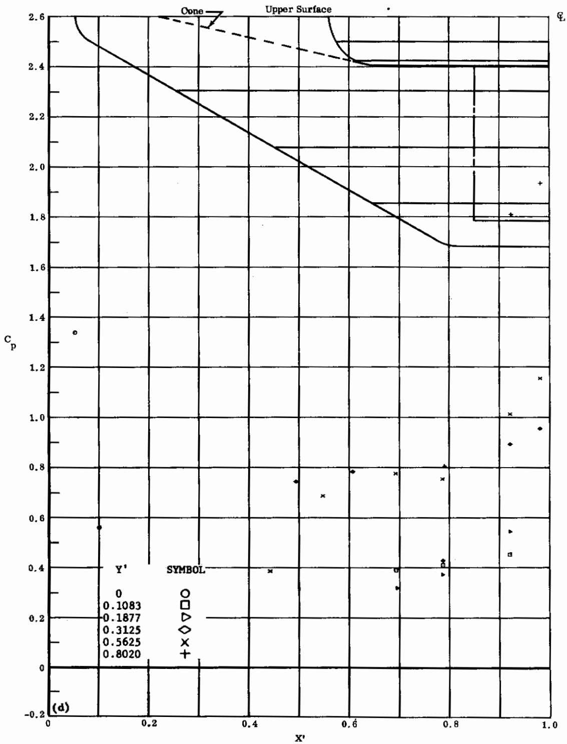
Fig. 45d Configuration IV, \alpha = -30 , \delta_2 = \delta_3 = -10
