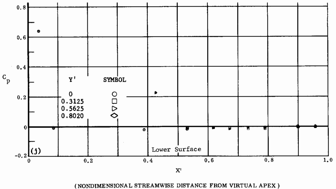
Fig. 49 Configuration IV, \alpha = -50 , \delta_2 = \delta_3 = -30
