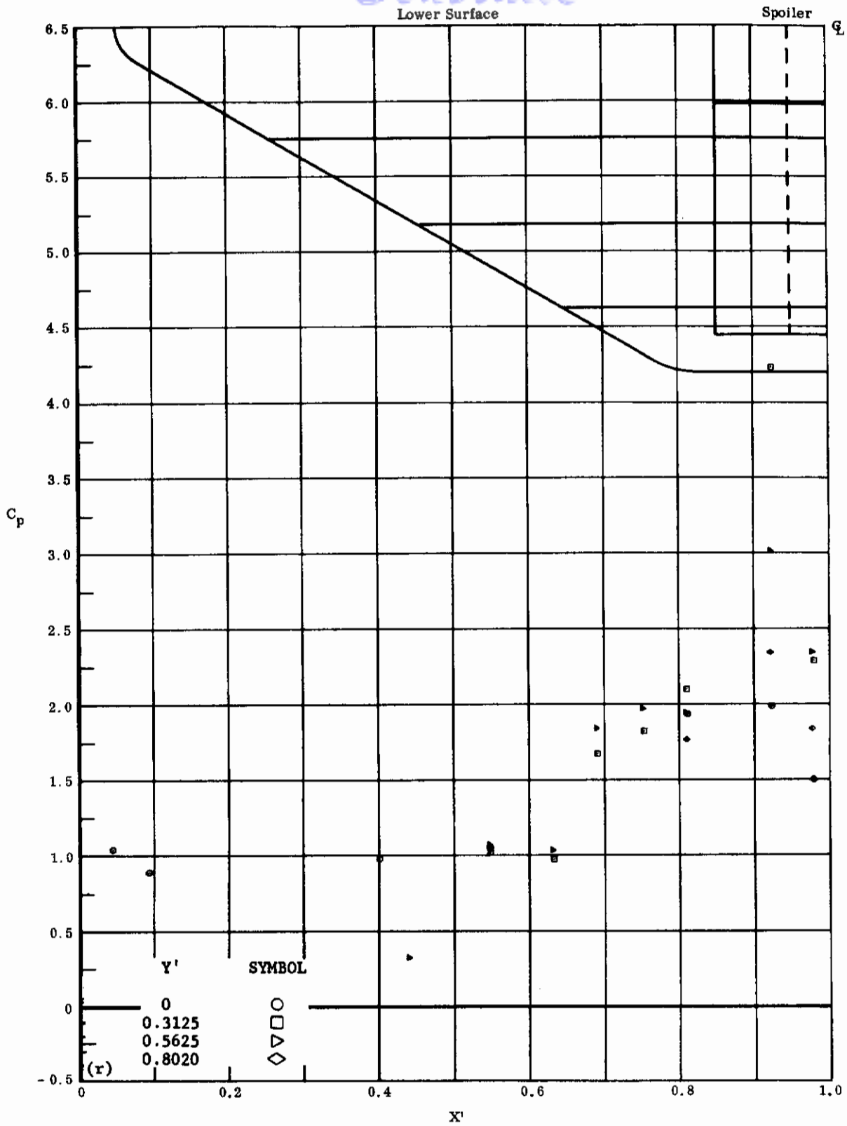
Fig. 11r Configuration I, \alpha = +40 , \delta_2 = \delta_3 = +39
