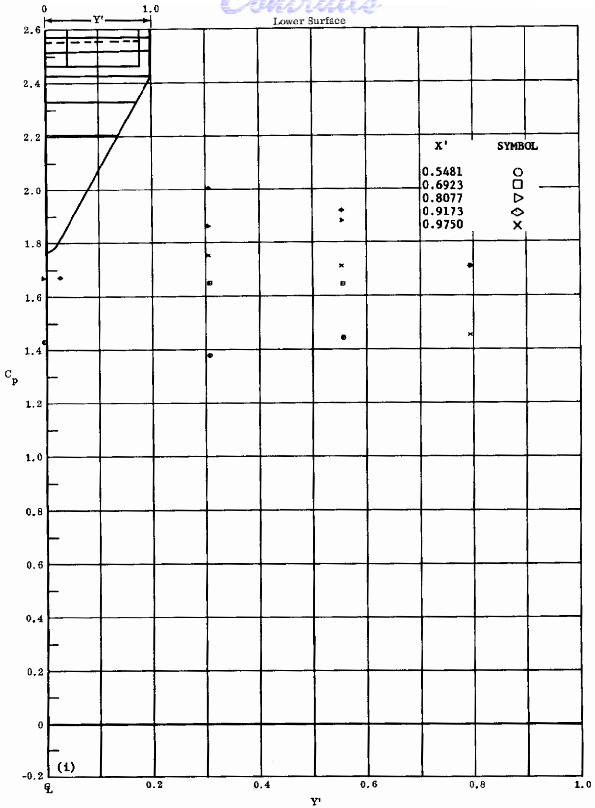
Fig. 13i Configuration I, \alpha = +50 , \delta_2 = \delta_3 = +20
