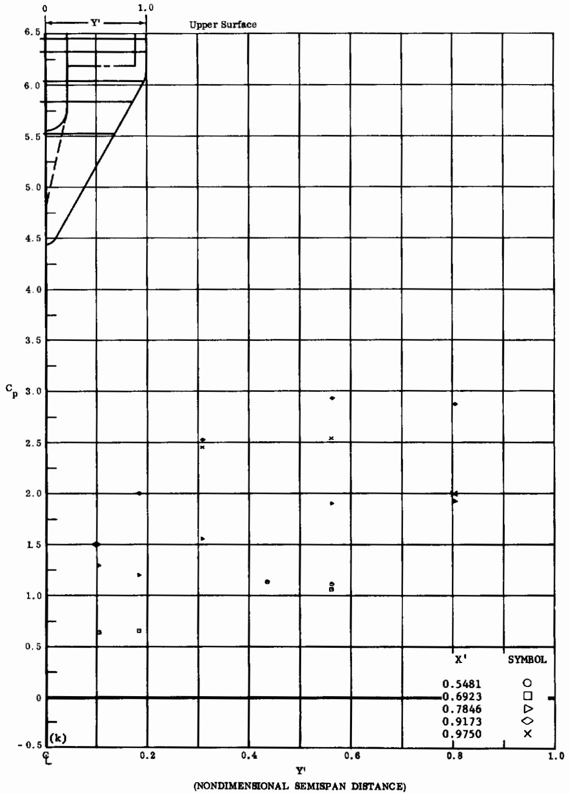
Fig. 26k Configuration I, \alpha = -40 , \delta_2 = \delta_3 = -30
