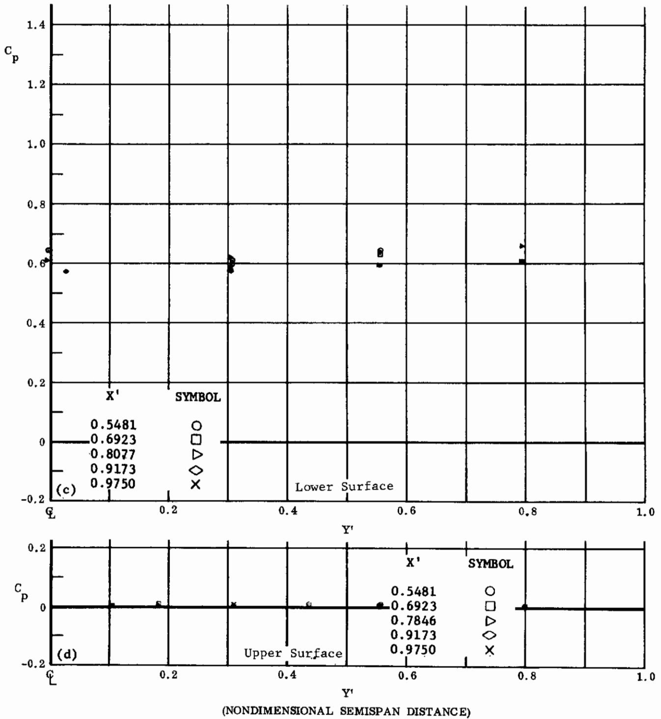
Fig. 9 Configuration I, \alpha = +30 , \delta_2 = \delta_3 = 0
