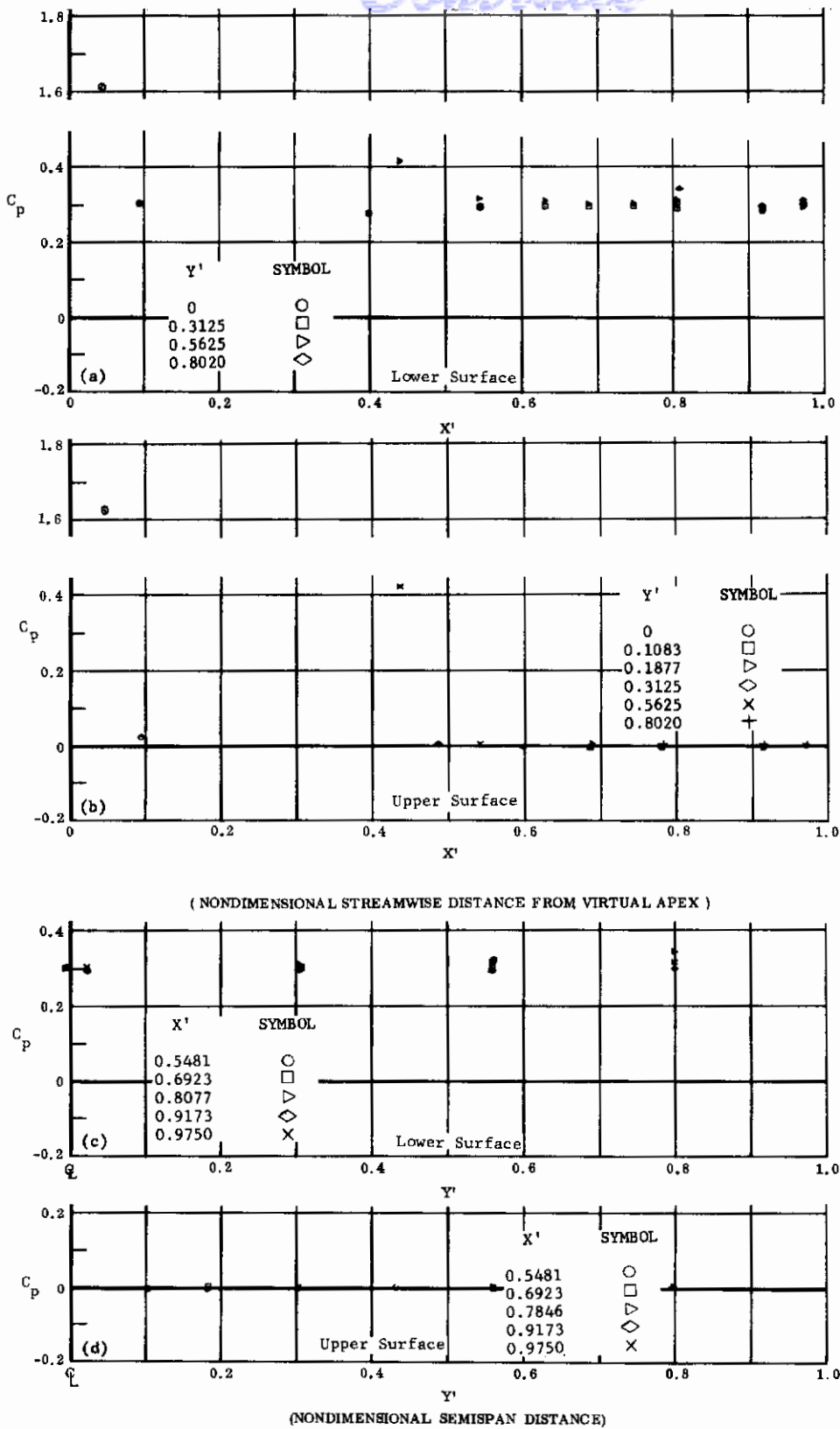
Fig. 7 Configuration I, \alpha = +20 , b_2 = b_3 = 0
