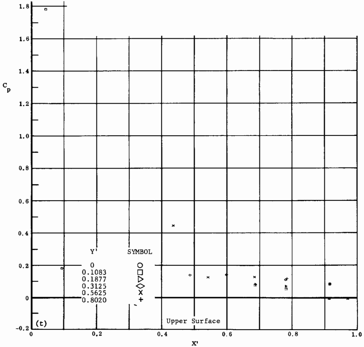
Fig. 16 Configuration I, \alpha = -10 , \delta_2 = \delta_3 = +39
