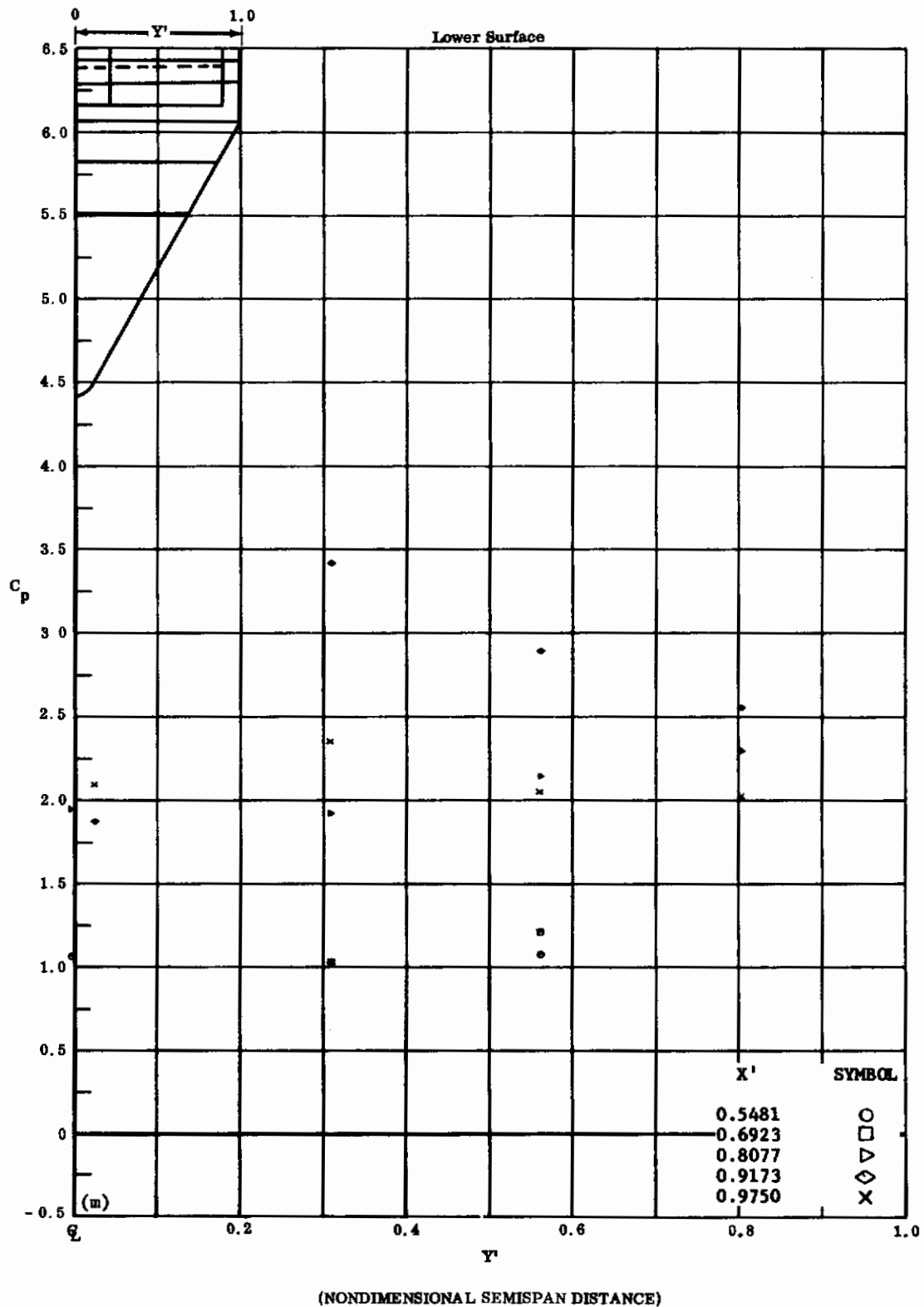
Fig. 37m Configuration IV, \alpha = +40 , \delta_2 = \delta_3 = +30 C_p vs. Y' , lower surface
