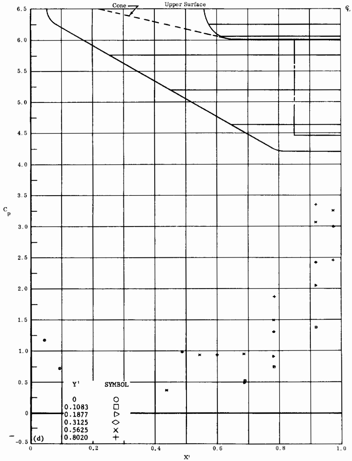
Fig. 24d Configuration I, \alpha = -35 , \delta_2 = \delta_3 = -30
