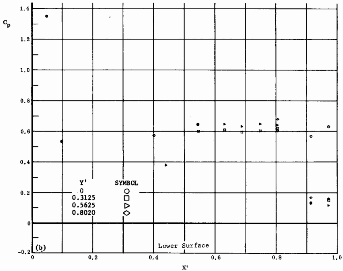
Fig. 10 Configuration I, \alpha = +30 , \delta_2 = \delta_3 = -20
