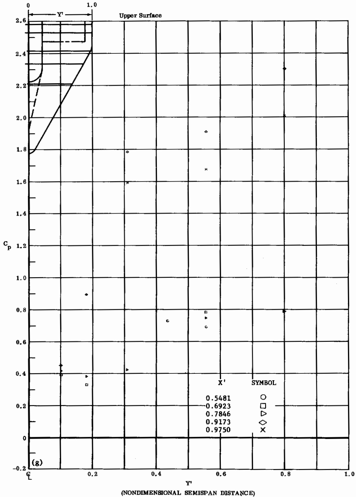
Fig. 23g Configuration I, \alpha = -30 , \delta_2 = \delta_3 = -20
