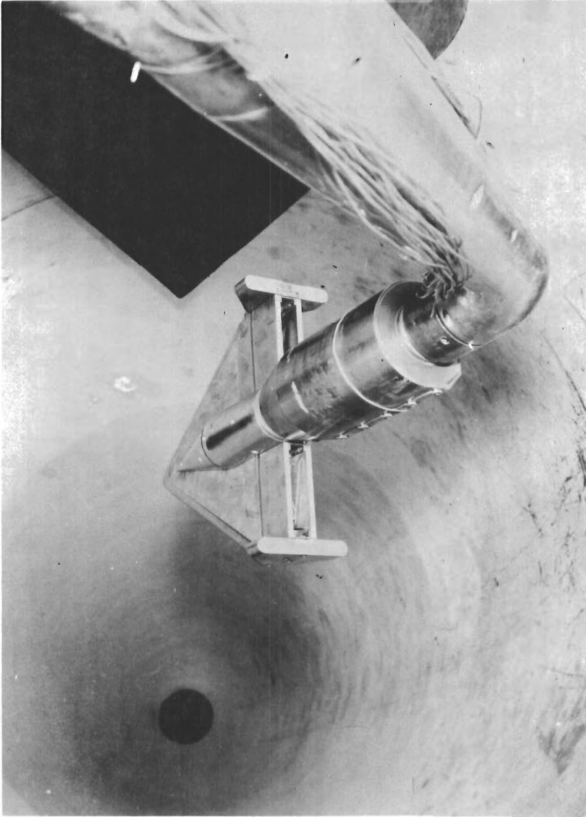
Figure 1j Photograph - Configuration IV, Mounted on Actuator Housing in the 50" Hypersonic Mach 8 Wind Tunnel
