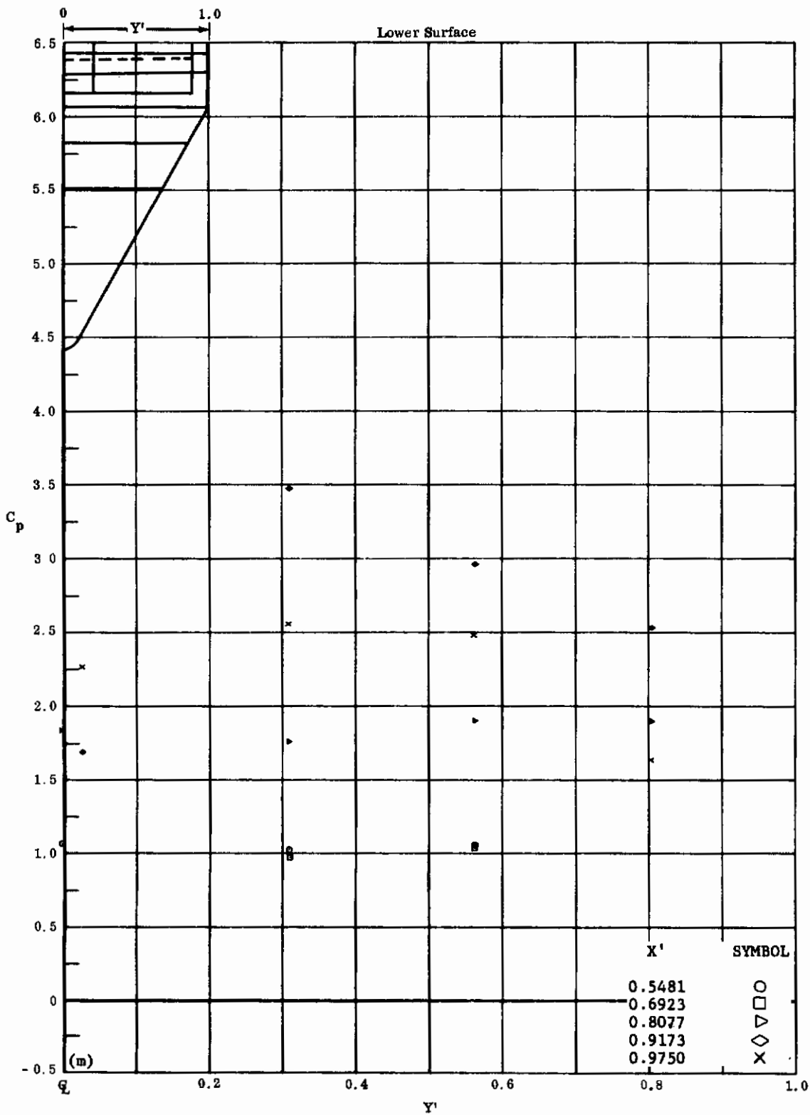
Fig. 11m Configuration I, \alpha = +40 , \delta_2 = \delta_3 = +30
