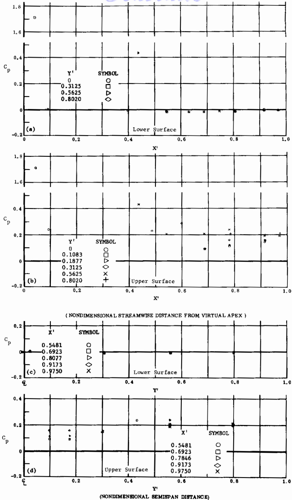
Fig. 18 Configuration I, \alpha = -15 , \delta_2 = \delta_3 = 0
