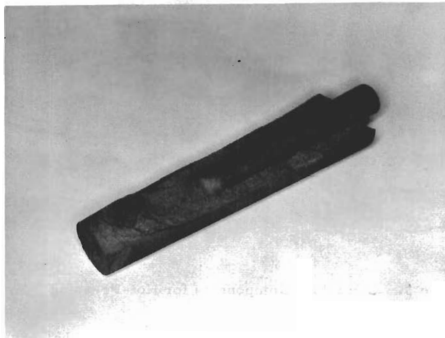
Figure 4. Graphite Die with Sample After Hot-Pressing
