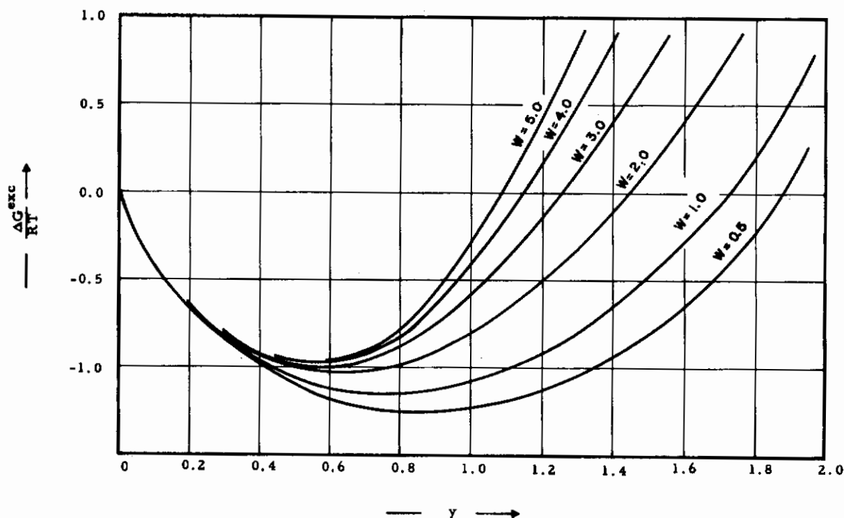
Figure 63. Model 2. Excess Free Energy due to Disorder in the Carbon Sublattice. Parameter: w = \frac{\Delta E}{RT} (Quantities per Mole Me_2C_y )
