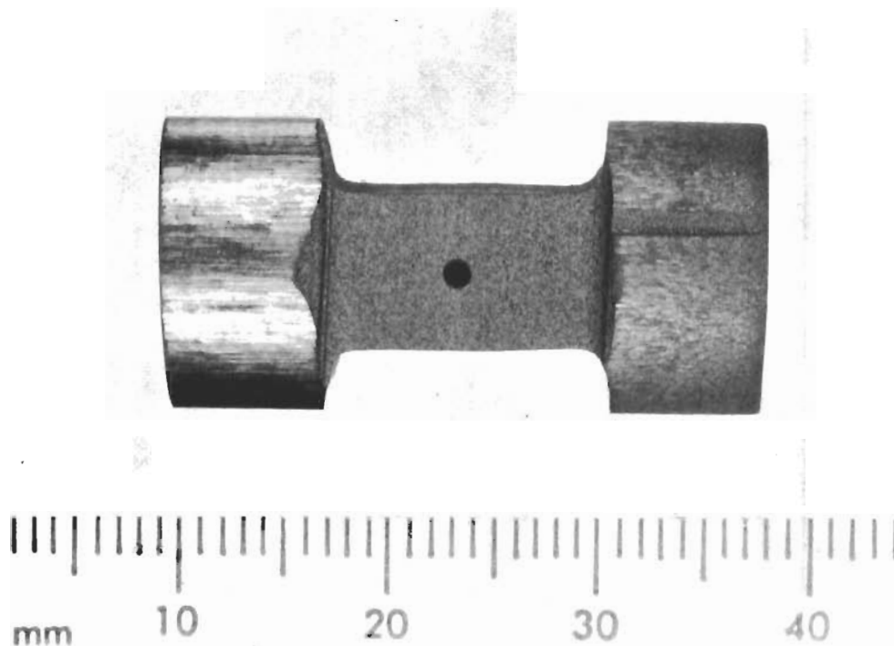
Figure 13. Pirani Melting Point Specimen, Hot Pressed and Ground
