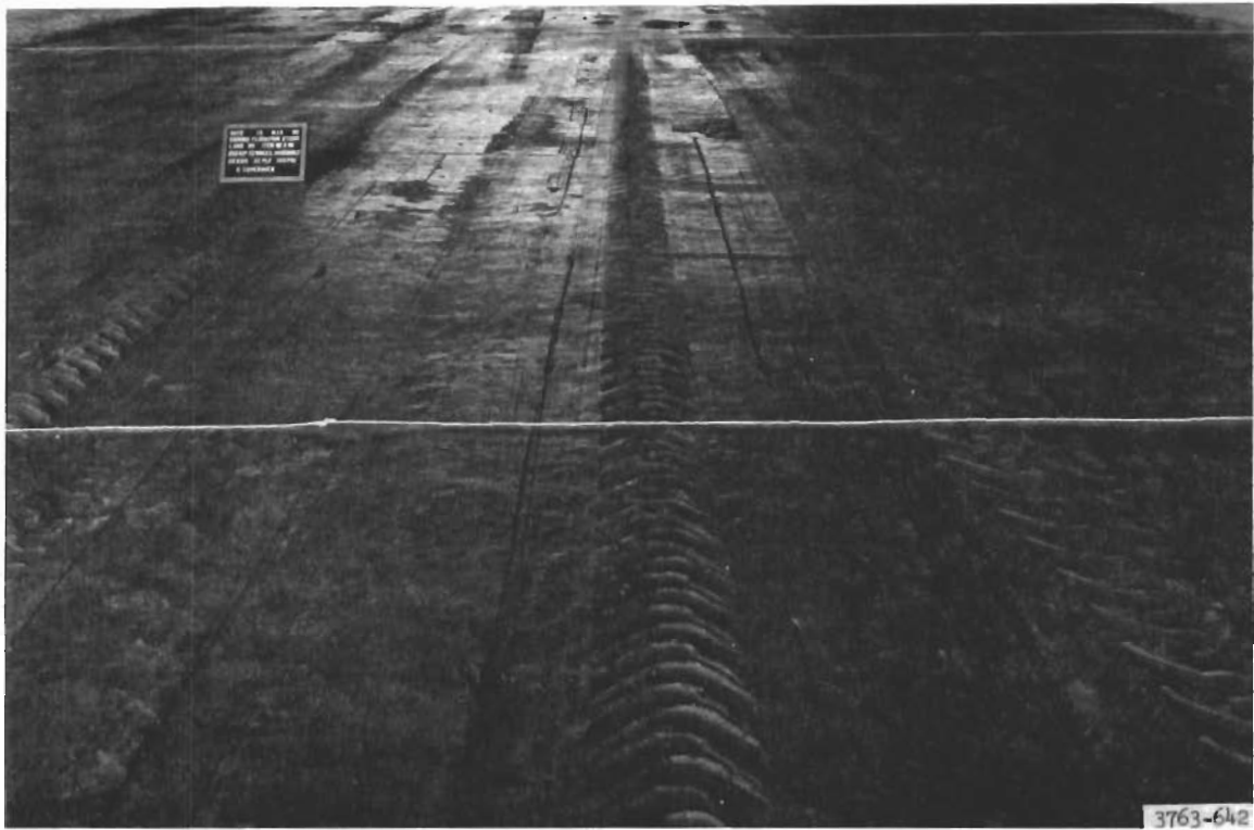
Figure 6. Lane 30, item 2, prior to traffic
