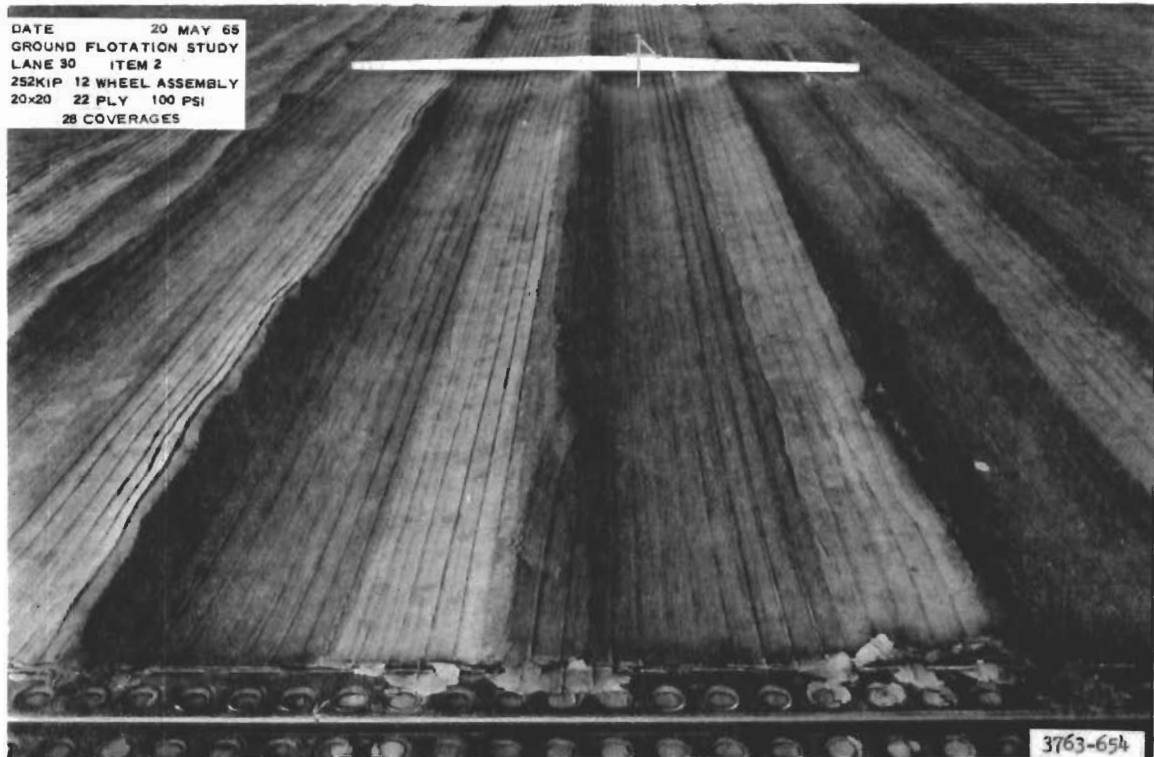
Figure 7. Lane 30, item 2. Transverse straightedge shows roughness at 28 coverages (failure)
