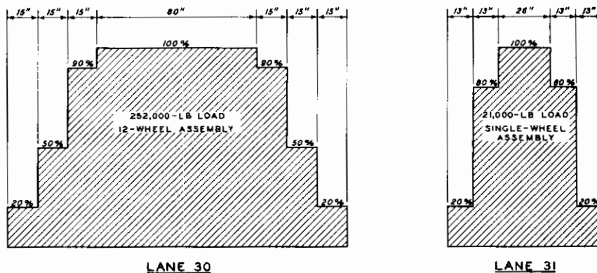
Figure 1. Traffic distribution patterns for Test Section 14
