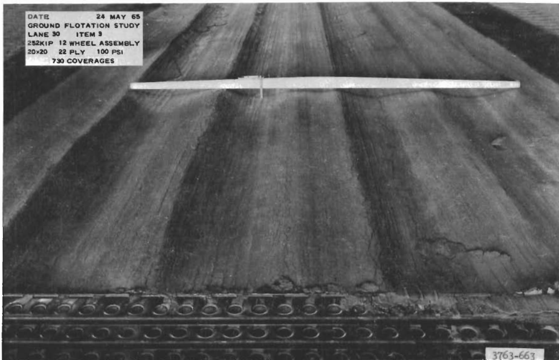
Figure 9. Lane 30, item 3. Transverse straightedge shows roughness at 730 coverages (failure)
