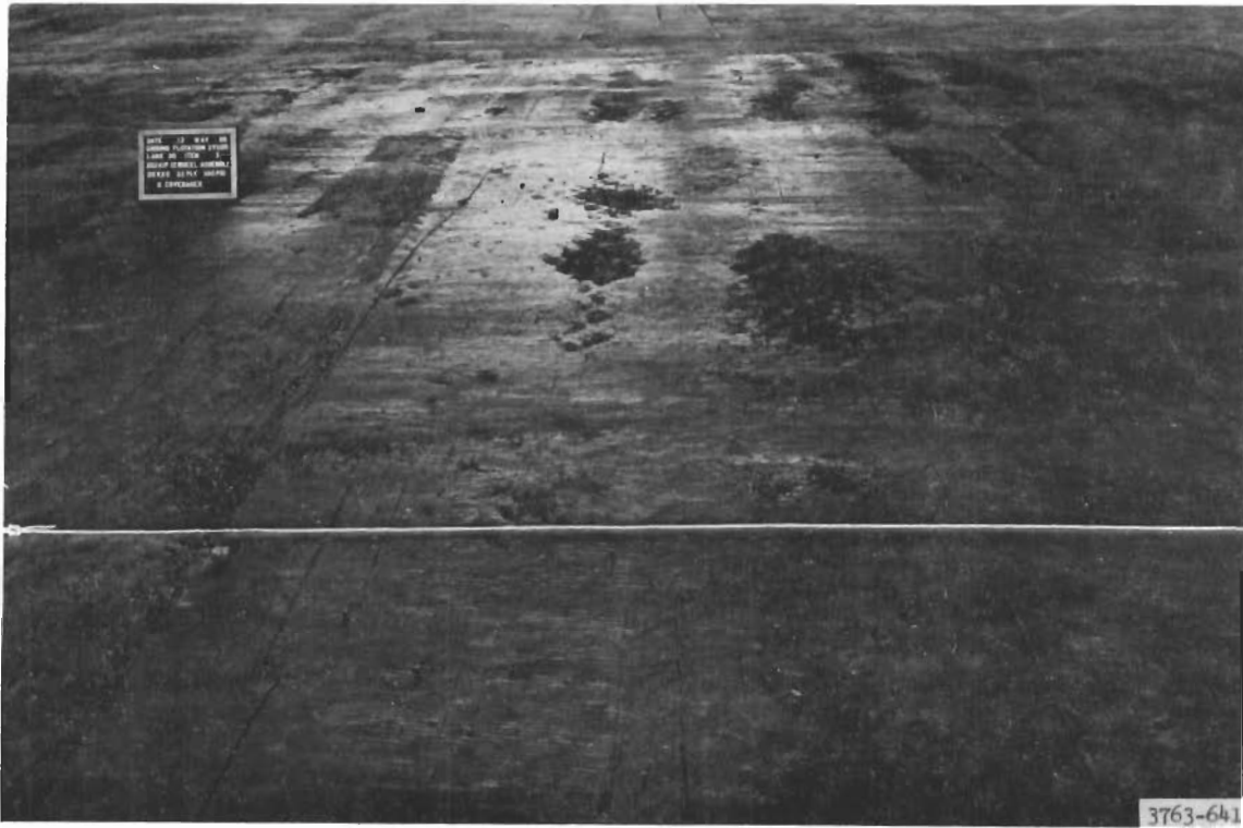
Figure 8. Lane 30, item 3, prior to traffic
