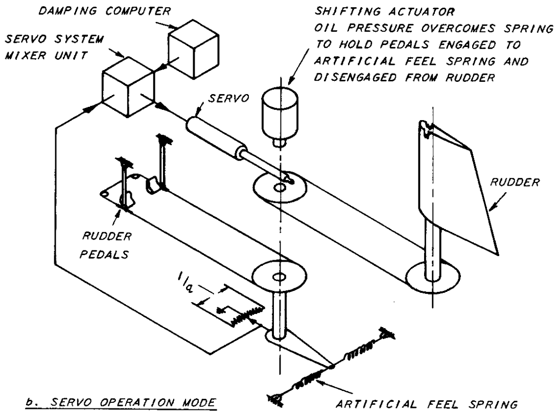
Fig. 1 SCHEMATIC DRAWING OF RUDDER SERVO INSTALLATION
