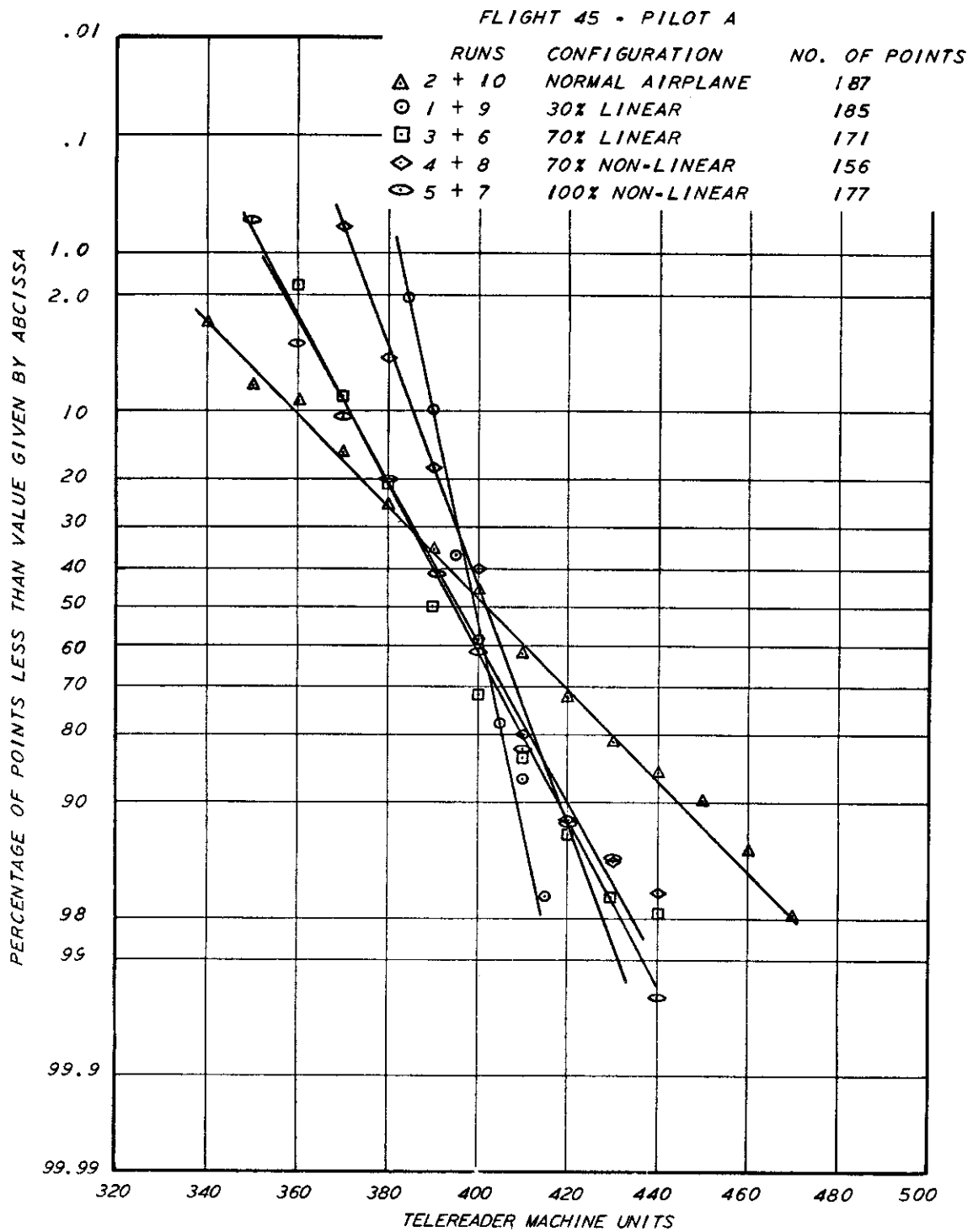
Fig. 12 DEMONSTRATION OF STATISTICAL NORMALITY OF TRACKING DATA
