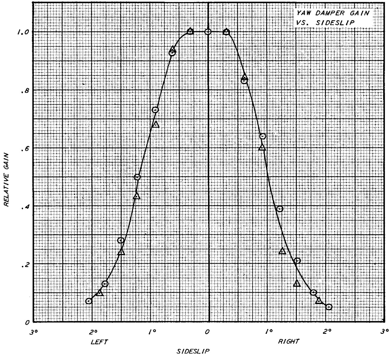
Fig. 3 MANNER IN WHICH YAW DAMPER GAIN WAS VARIED TO MAKE IT NON-LINEAR
