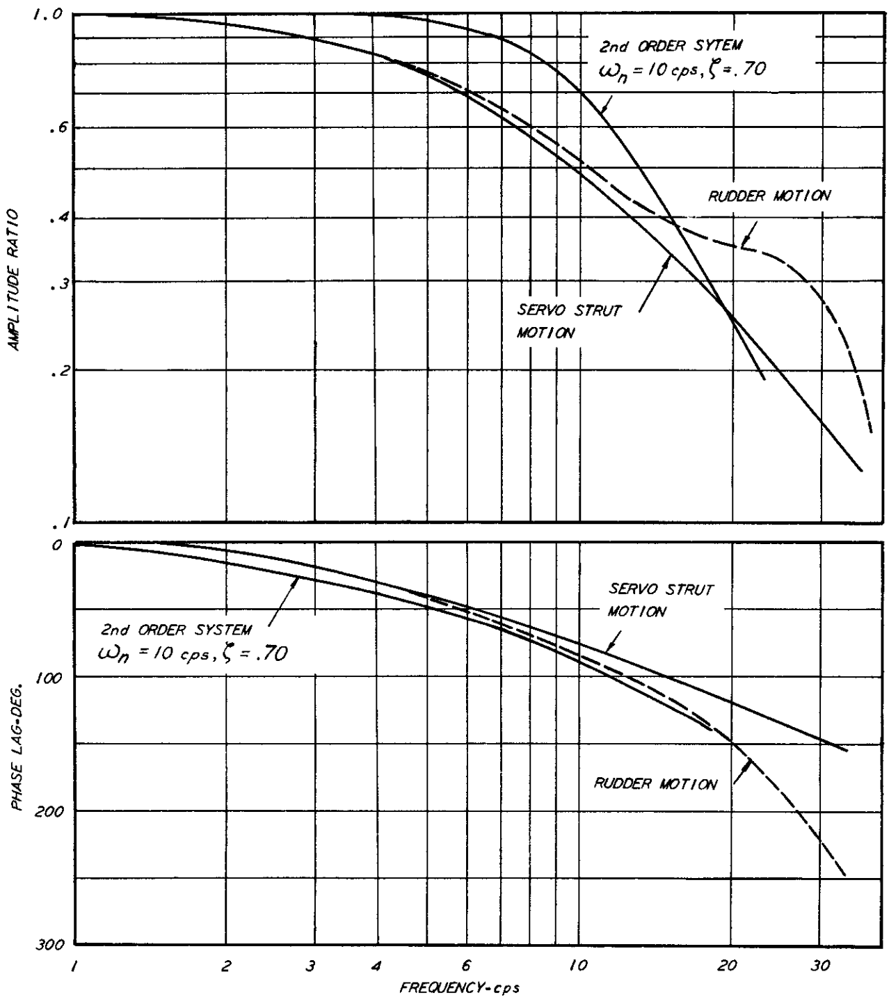
Fig. 6 FREQUENCY RESPONSE OF YAW DAMPER SERVO SYSTEM
