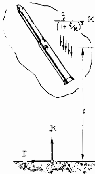
FIGURE 62 APPROXIMATIONS TO INVERSE SQUARE GRAVITY FIELD
