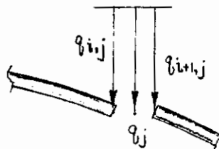
FIGURE 74 DISPLACEMENT CONTINUITY AT A JOINT BETWEEN ELEMENTS OF A MEMBER
