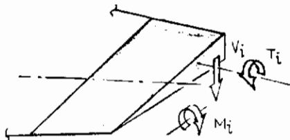
FIGURE 86 LOADS AT THE END OF AN ELEMENT
