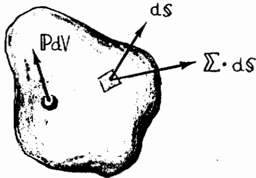
FIGURE 3 SURFACE AND BODY FORCES
