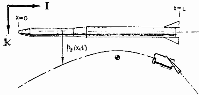
FIGURE 22 SLENDER CONTROLLED VEHICLE
