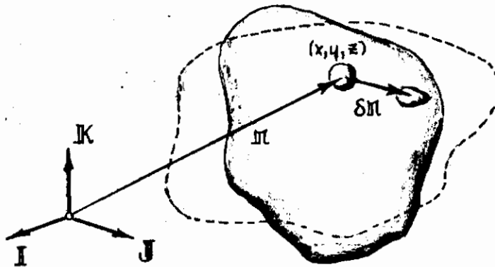
FIGURE 4 A VIRTUAL DISPLACEMENT OF THE SYSTEM
