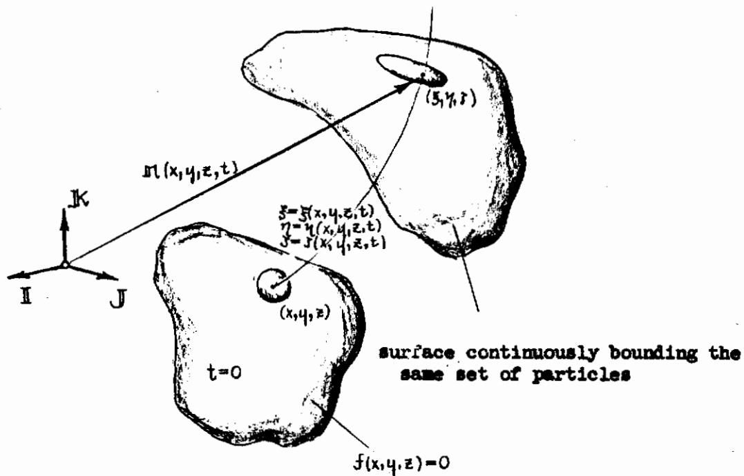
FIGURE 2 EULERIAN AND LAGRANGIAN COORDINATES
