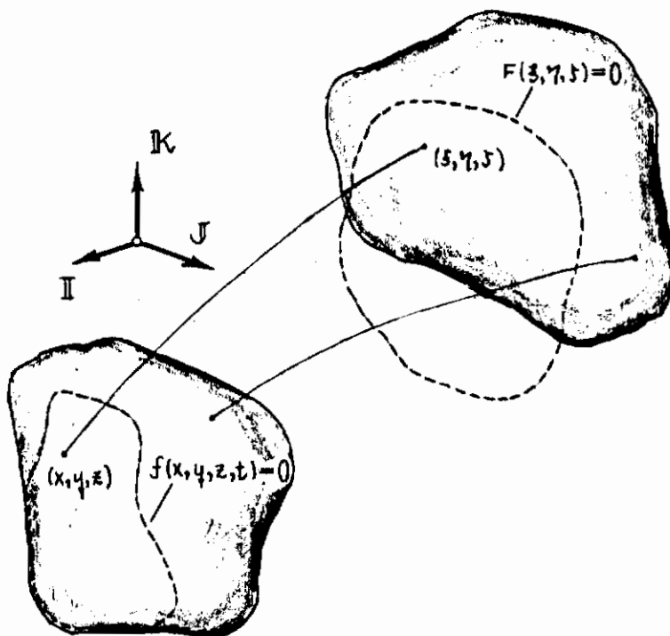
FIGURE 5 ILLUSTRATING THE REGION OF INTEGRATION
