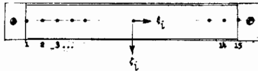
FIGURE 136 COLLOCATION POINTS
