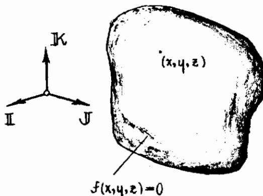
FIGURE 1 A PORTION OF THE CONTINUUM
