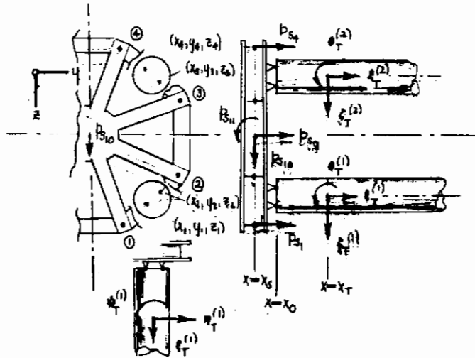
FIGURE 142 SPIDER BEAM - OUTER LOX TANK COMPATIBILITY
