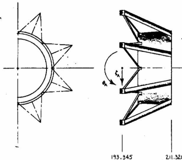
FIGURE 121 DEGREES-OF-FREEDOM FOR ADAPTER
