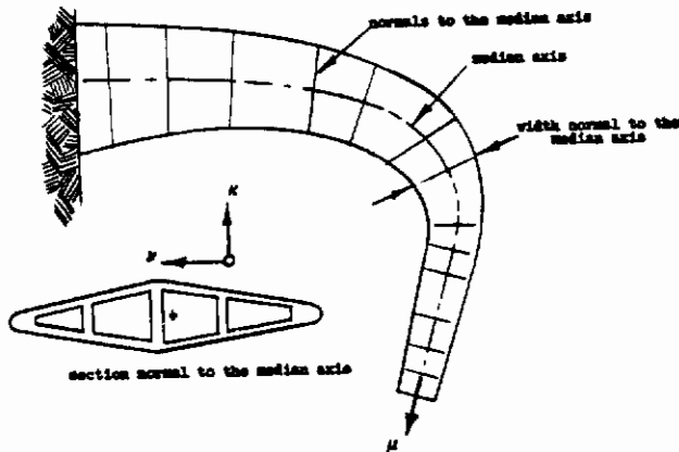
FIGURE 78 GEOMETRY OF A BEAM
