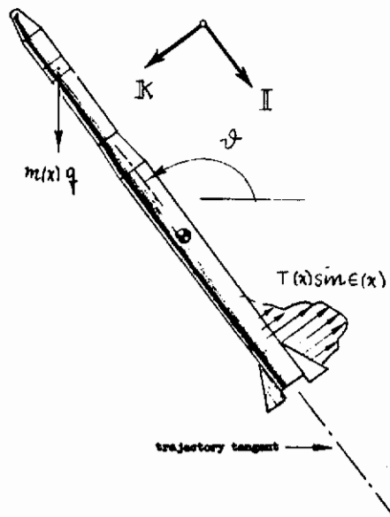
FIGURE 35 DISTRIBUTED LATERAL FORCES
