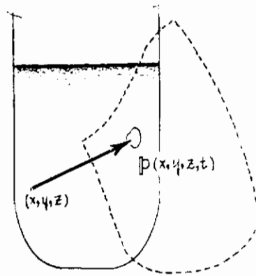
FIGURE 49 DISPLACEMENTS OF SLOSHING FUEL
