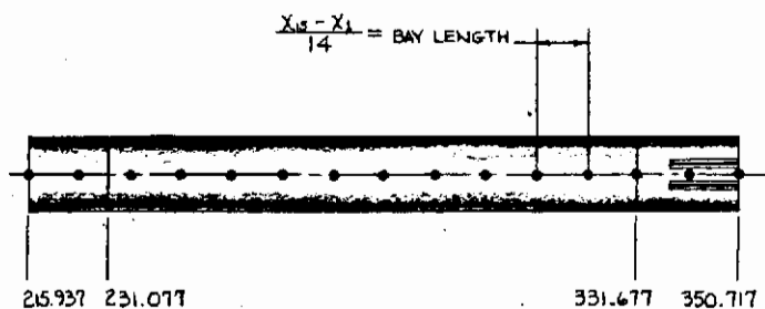
FIGURE 127 COLLOCATION POINT GEOMETRY FOR FUEL TANK
