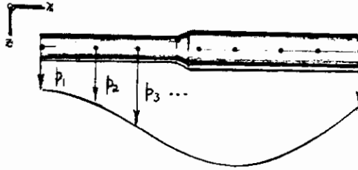
FIGURE 90 GENERALIZED COORDINATES FOR A ONE-DIMENSIONAL COMPONENT
