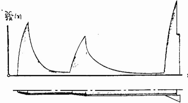
FIGURE 26 RUNNING AIR LOAD DISTRIBUTION FOR A SLENDER LAUNCH VEHICLE
