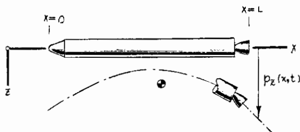
FIGURE 46 SLENDER LAUNCH VEHICLE WITH GIMBALED ENGINE
