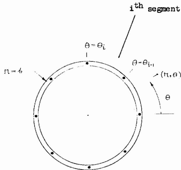
FIGURE 19 COLLOCATION POINTS
