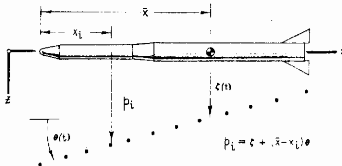
FIGURE 28 COLLOCATION POINT DISPLACEMENTS FOR THE RIGID MISSILE
