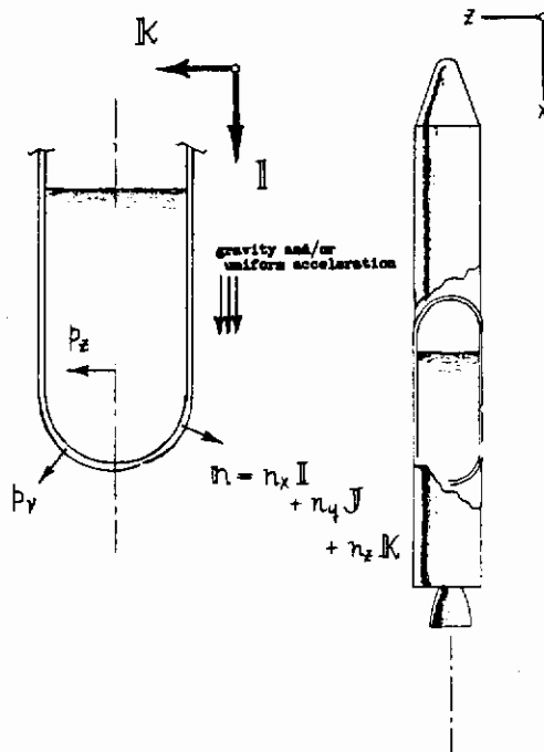
FIGURE 48 LIQUID FUEL TANK AND LAUNCH VEHICLE
