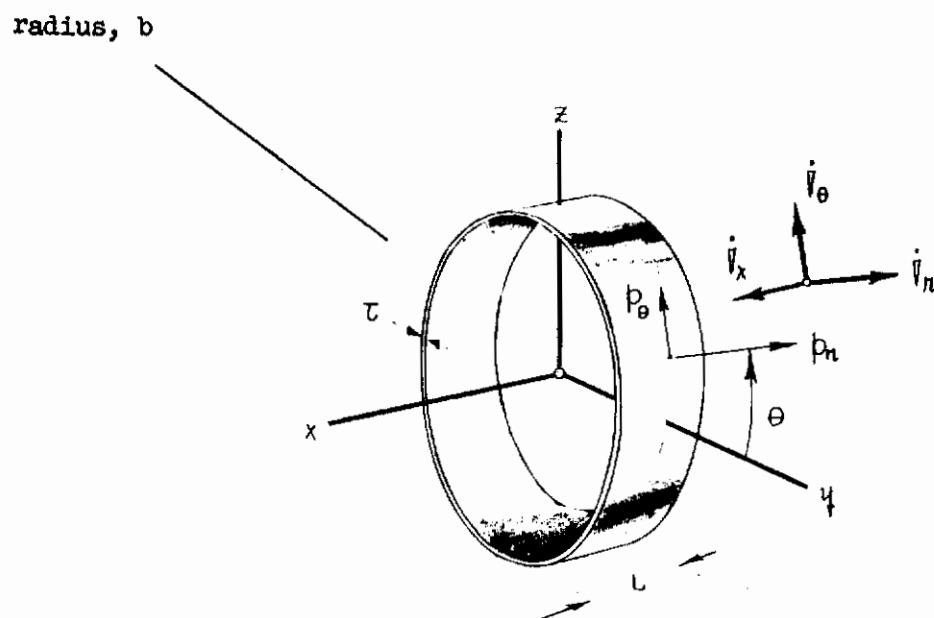
FIGURE 18 UNIFORM THIN RING
