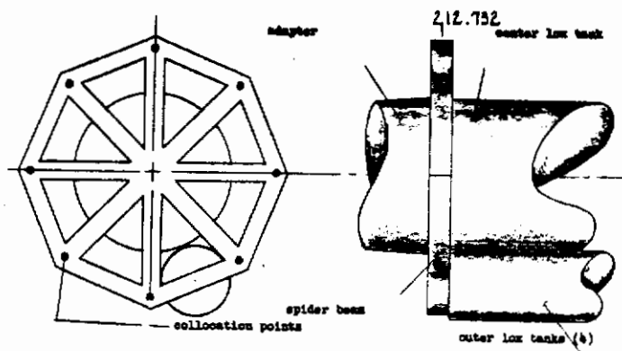
FIGURE 123 COLLOCATION POINT GEOMETRY FOR SPIDER BEAM
