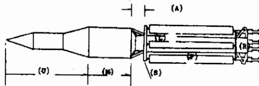
FIGURE 130 VEHICLE WITHOUT OUTER LOX TANKS
