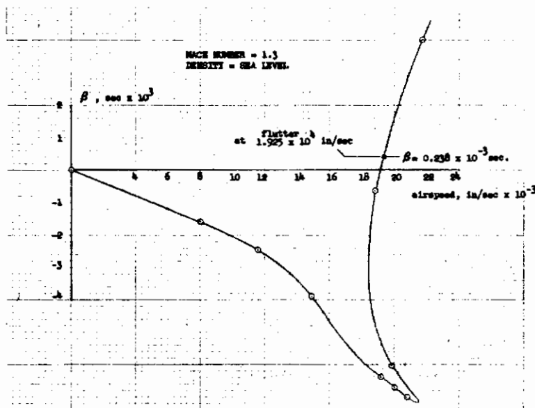
FIGURE 51 GRAPHICAL REPRESENTATION OF SOLUTION OF FLUTTER DETERMINANT
