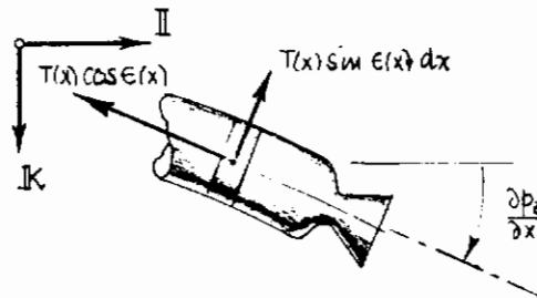
FIGURE 36 DISTRIBUTED THRUST FORCE ON THE FLEXIBLE MISSILE
