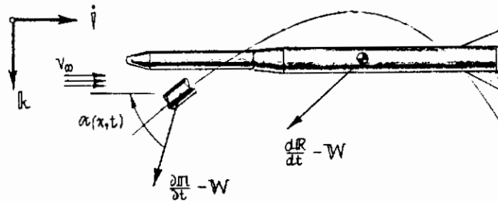
FIGURE 59 AERODYNAMIC ASSUMPTIONS
