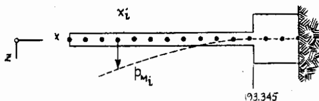
FIGURE 120 EQUIVALENT BEAM
