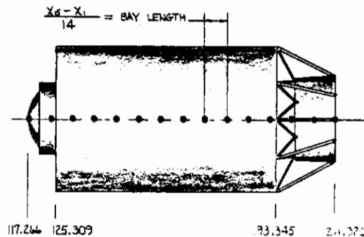
FIGURE 119 COLLOCATION POINT GEOMETRY FOR MIDDLE STAGE
