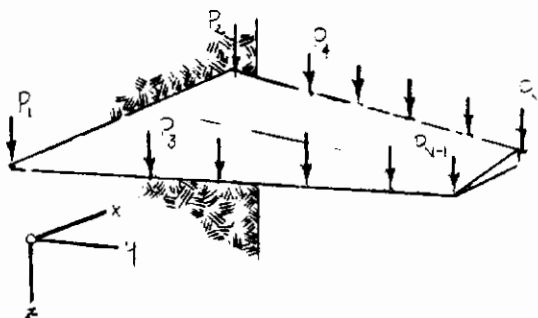
FIGURE 84 LOADED BEAM
