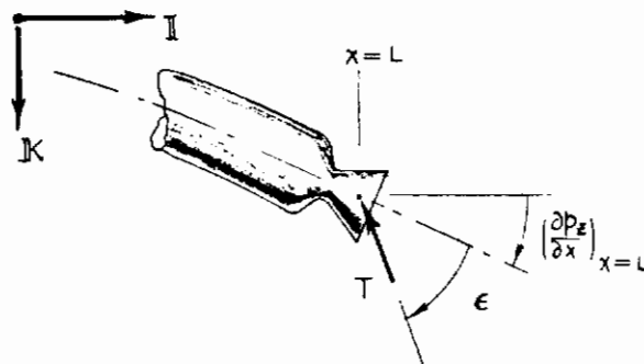
FIGURE 37 CONCENTRATED THRUST FORCE MISALIGNED AT AN ANGLE, \epsilon
