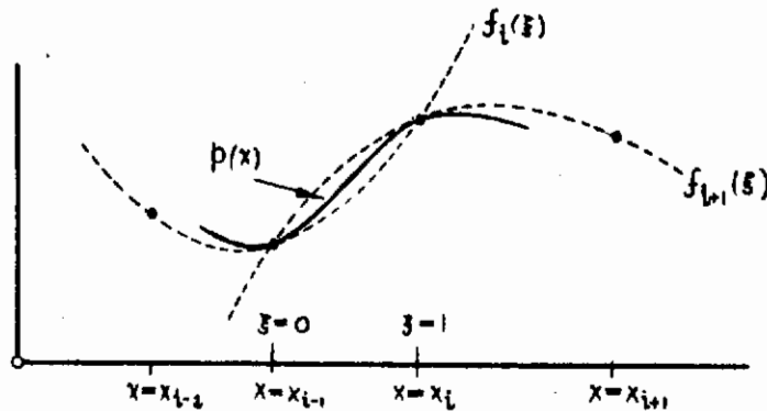
FIGURE 10 DIPARABOLIC INTERPOLATION
