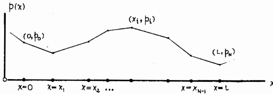
FIGURE 9 TRAPEZOIDAL INTERPOLATION
