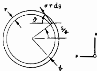
FIGURE 83 SHEAR STRESS ON A THIN-WALL CYLINDER
