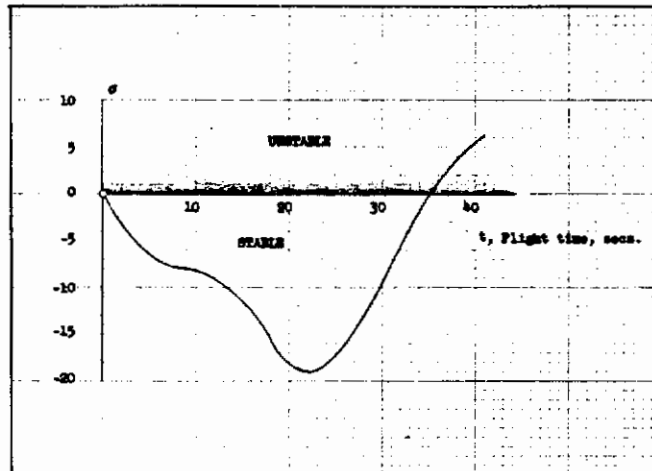
FIGURE 53 DAMPING VERSUS FLIGHT TIME
