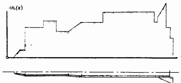
FIGURE 23 MASS DISTRIBUTION FOR A SLENDER LAUNCH VEHICLE
