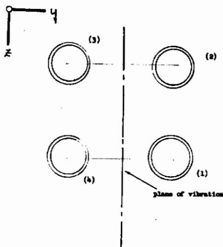
FIGURE 140 ARRANGEMENT OF FOUR OUTER LOX TANKS
