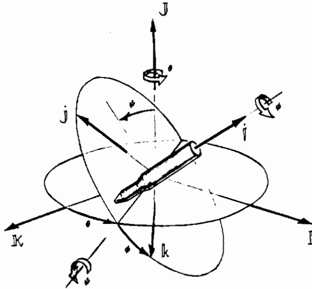
FIGURE 67 EULER ANGLES
