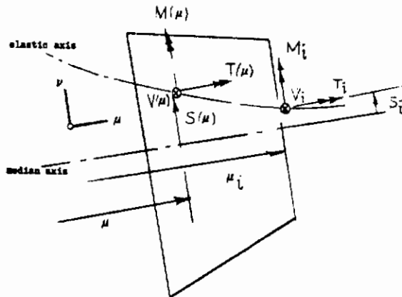
FIGURE 87 FREE BODY OF AN ELEMENT
