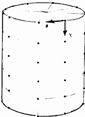
FIGURE 104 COLLOCATION POINTS FOR A CYLINDRICAL SHELL
