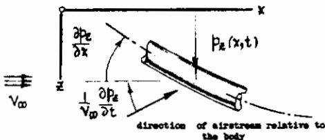
FIGURE 25 LOCAL ANGLE-OF-ATTACK
