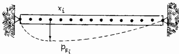
FIGURE 128 EQUIVALENT BEAM FOR FUEL TANK
