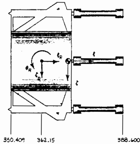
FIGURE 129 OUTRIGGER DEGREES-OF-FREEDOM
