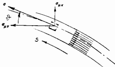
FIGURE 82 SHEARING STRESSES
