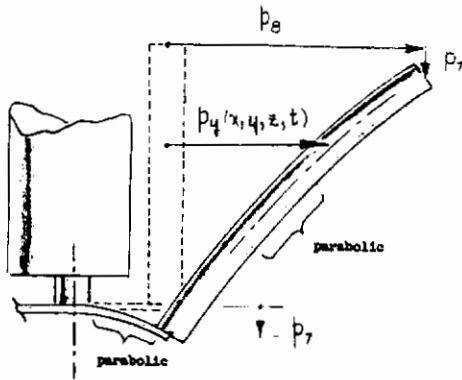
FIGURE 113 DEFLECTIONS IN THE SYMMETRIC PLANE
