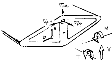
FIGURE 79 STRESS RESULTANTS ON A SECTION
