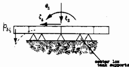
FIGURE 124 GENERALIZED COORDINATES FOR SPIDER BEAM
