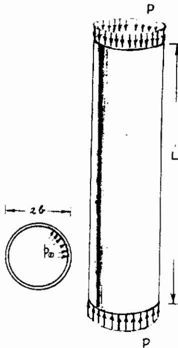
FIGURE 107 SLENDER CYLINDRICAL SHELL
