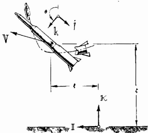
FIGURE 58 INERTIAL AND BODY REFERENCE SYSTEMS
