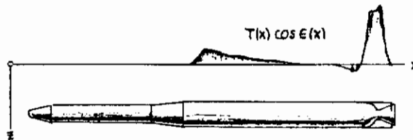
FIGURE 32 DISTRIBUTION OF AXIAL COMPONENT OF THRUST
