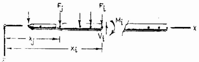
FIGURE 29 INTERNAL LOADS AT THE COLLOCATION POINTS
