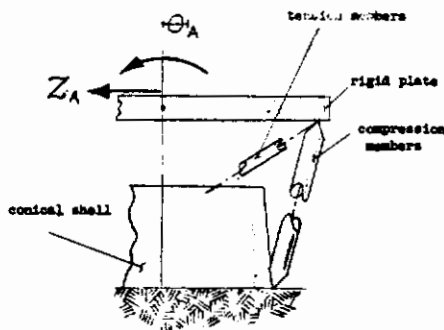
FIGURE 122 GENERALIZED ADAPTER LOADS
