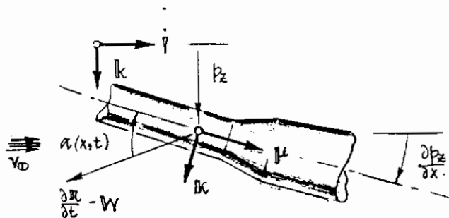
FIGURE 60 LOCAL ANGLE-OF-ATTACK
