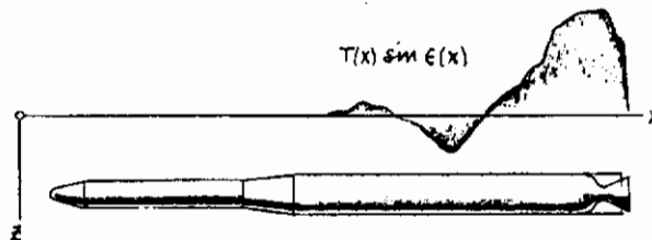
FIGURE 33 DISTRIBUTION OF LATERAL COMPONENT OF THRUST
