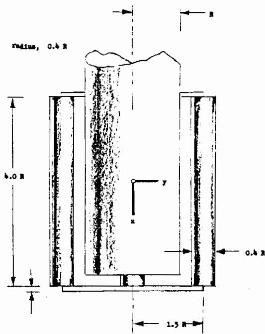
FIGURE 111 MODEL DIMENSIONS
