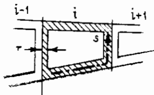
FIGURE 81 A SINGLE CELL
