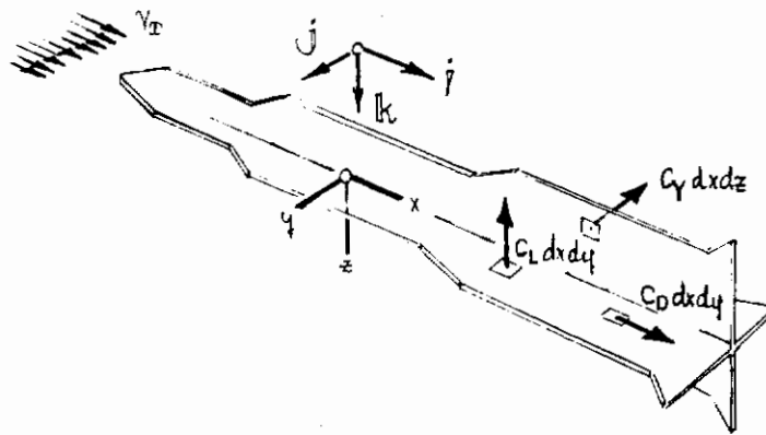
FIGURE 69 IDEALIZED DISTRIBUTION OF AERODYNAMICS FORCES
