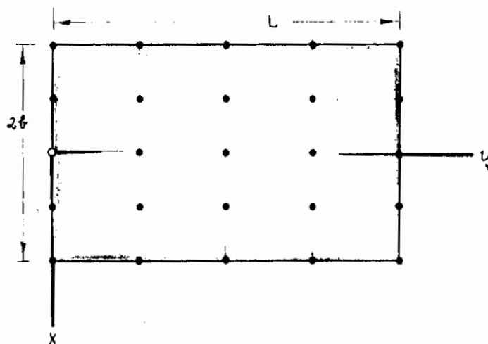
FIGURE 15 COLLOCATION POINTS ON THE PLATE
