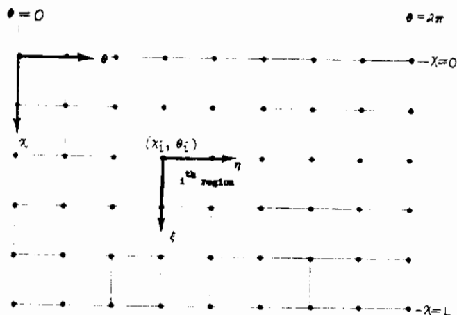
FIGURE 105 INSIDE OF DEVELOPED SHELL SHOWING TYPICAL REGION
