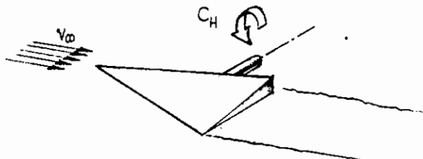
FIGURE 30 SIGN CONVENTION FOR CONTROL "HINGE" MOMENTS
