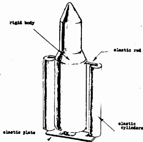
FIGURE 110 EXAMPLE VEHICLE
