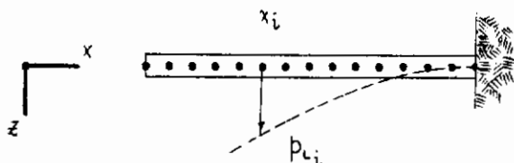
FIGURE 126 EQUIVALENT BEAM
