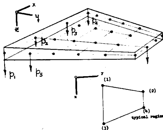
FIGURE 91 GENERALIZED COORDINATES FOR A TWO-DIMENSIONAL COMPONENT
