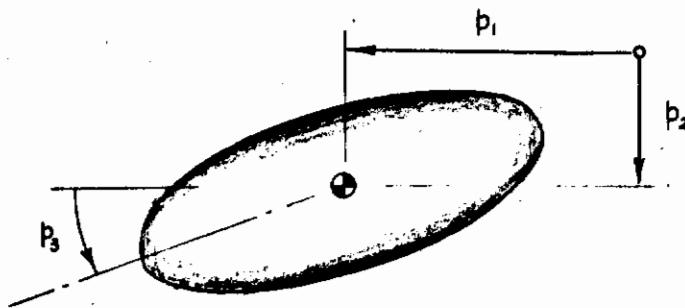
FIGURE 6 RIGID BODY IN PLANE MOTION
