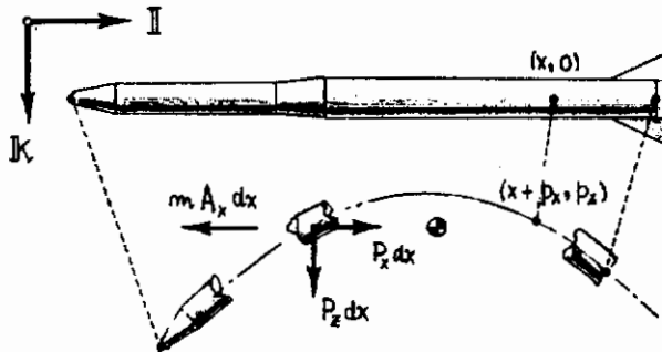
FIGURE 31 AXIALLY LOADED LAUNCH VEHICLE
