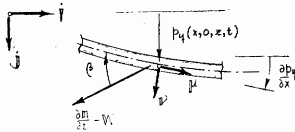
FIGURE 71 THE LOCAL ANGLE OF SIDESLIP
