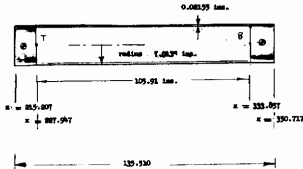
FIGURE 135 GEOMETRY OF OUTER LOX TANK
