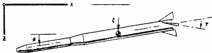
FIGURE 27 GENERALIZED COORDINATES FOR THE RIGID MISSILE
