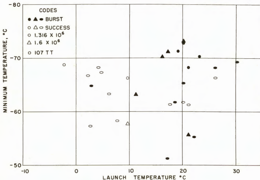
Figure 2. Balloon Performance Versus Launch Temperature and Minimum Ascent Temperature
