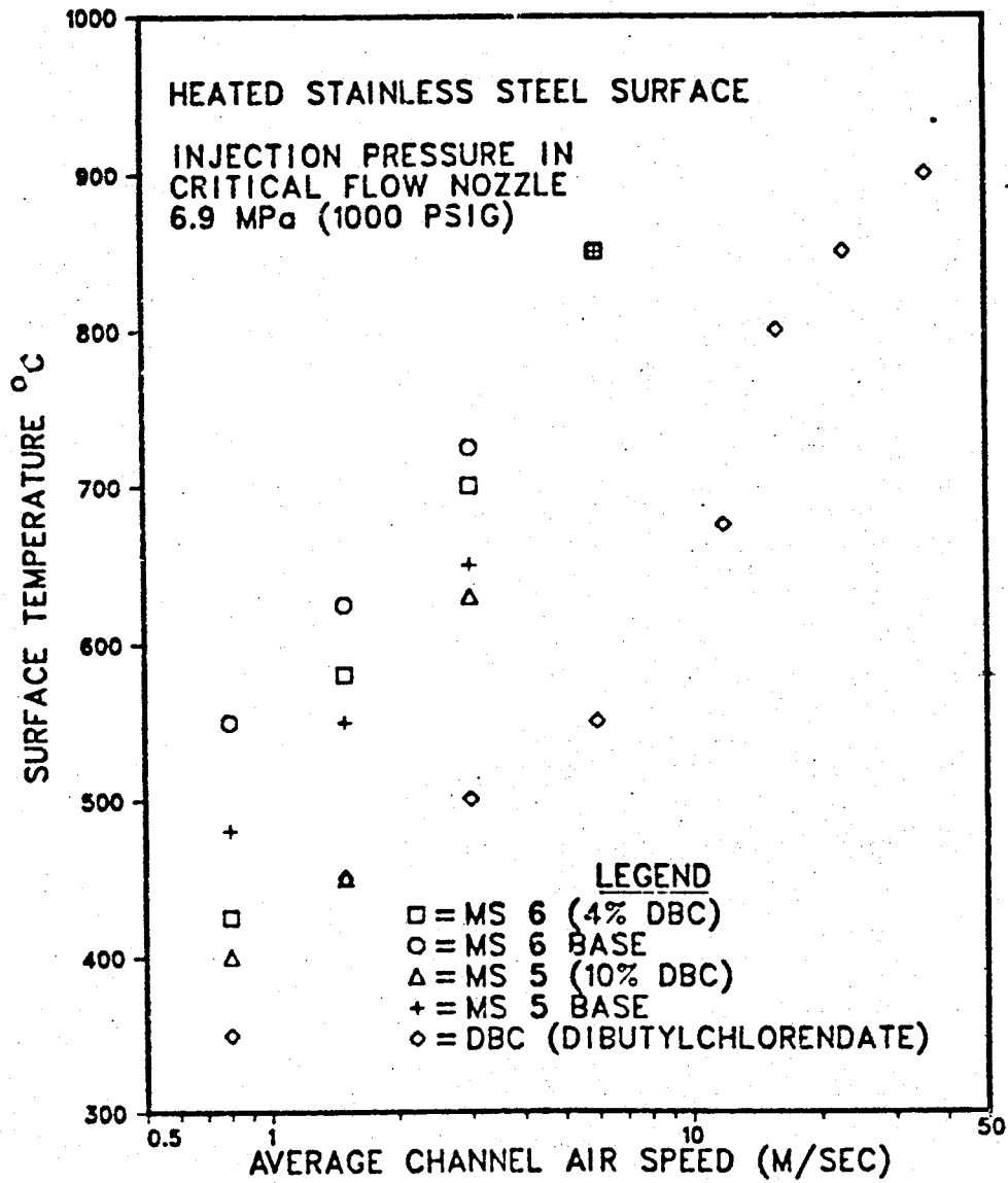
FIGURE 12 AIR SPEED EFFECTS ON HOT SURFACE IGNITION TEMPERATURE OF SILICONE BASE FLUIDS AND ADDITIVES
