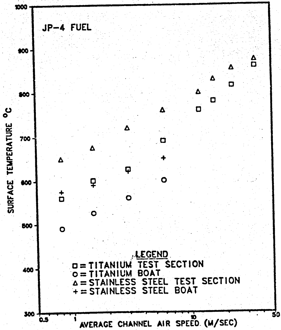
FIGURE A-2 AIR SPEED AND SURFACE MATERIAL EFFECTS ON HOT SURFACE IGNITION TEMPERATURE OF AIRCRAFT FUELS
