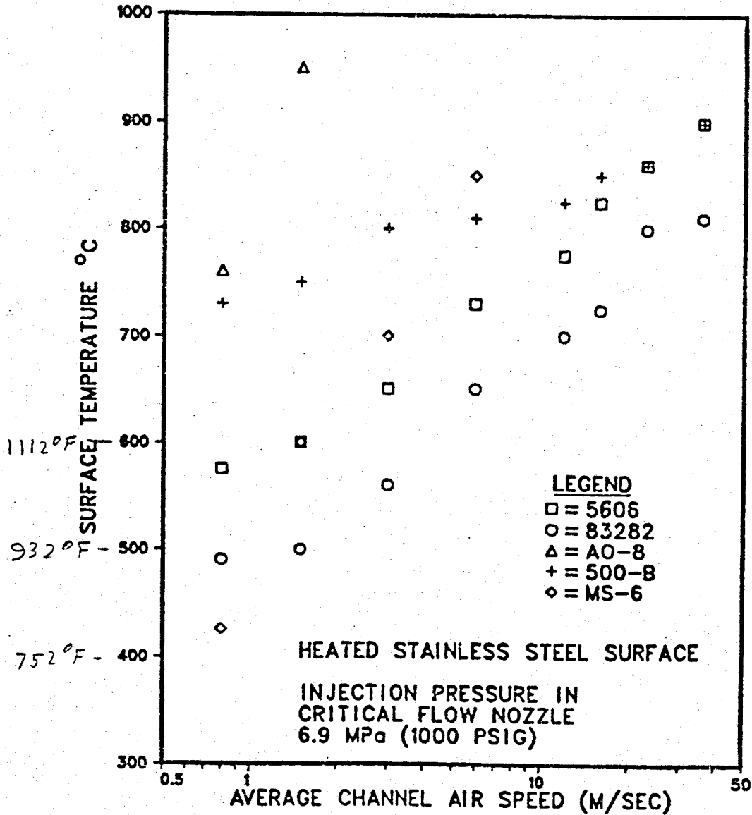
FIGURE 10 AIR SPEED AND SURFACE MATERIAL EFFECTS ON HOT SURFACE IGNITION TEMPERATURE OF AIRCRAFT HYDRAULIC FLUIDS
