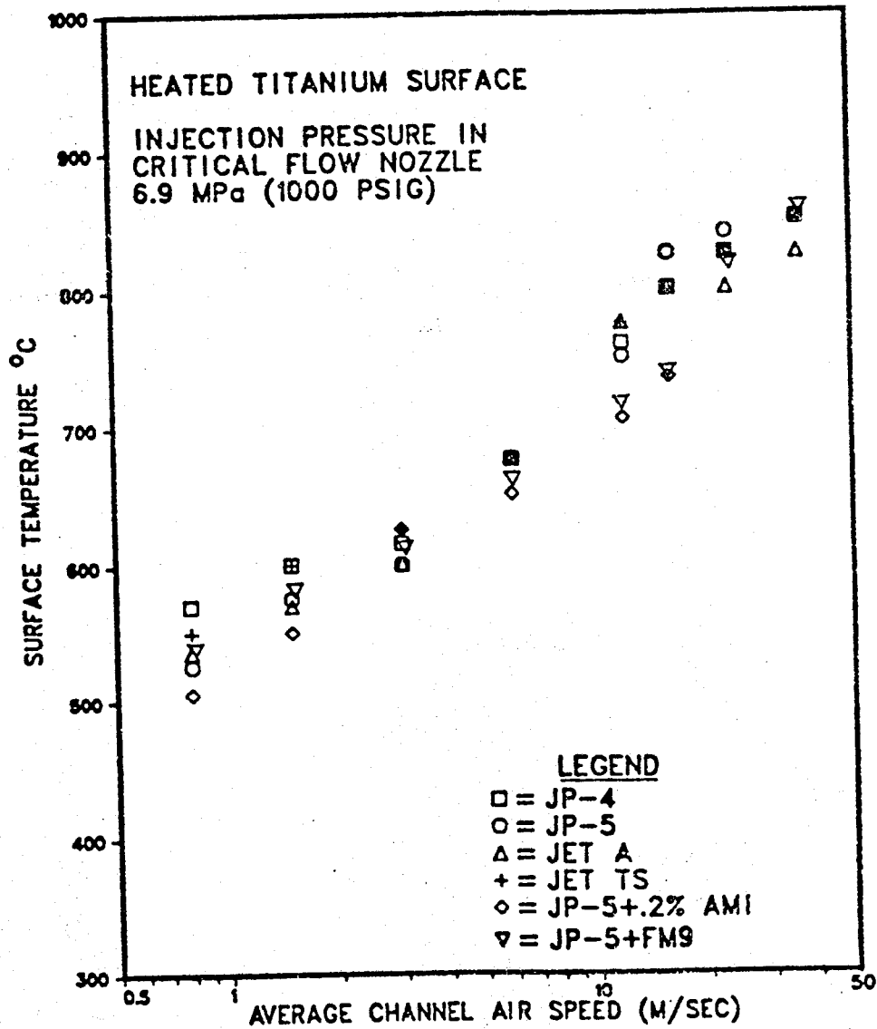
FIGURE 8 AIR SPEED AND SURFACE MATERIAL EFFECTS ON HOT SURFACE IGNITION TEMPERATURE OF AIRCRAFT FUELS
