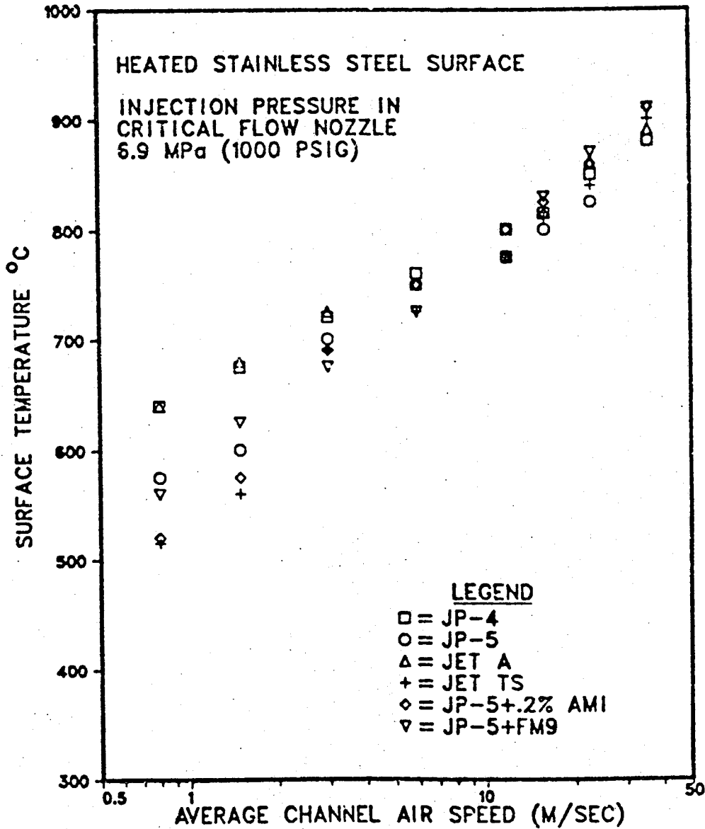
FIGURE 7 AIR SPEED AND SURFACE MATERIAL EFFECTS ON HOT SURFACE IGNITION TEMPERATURE OF AIRCRAFT FUELS
