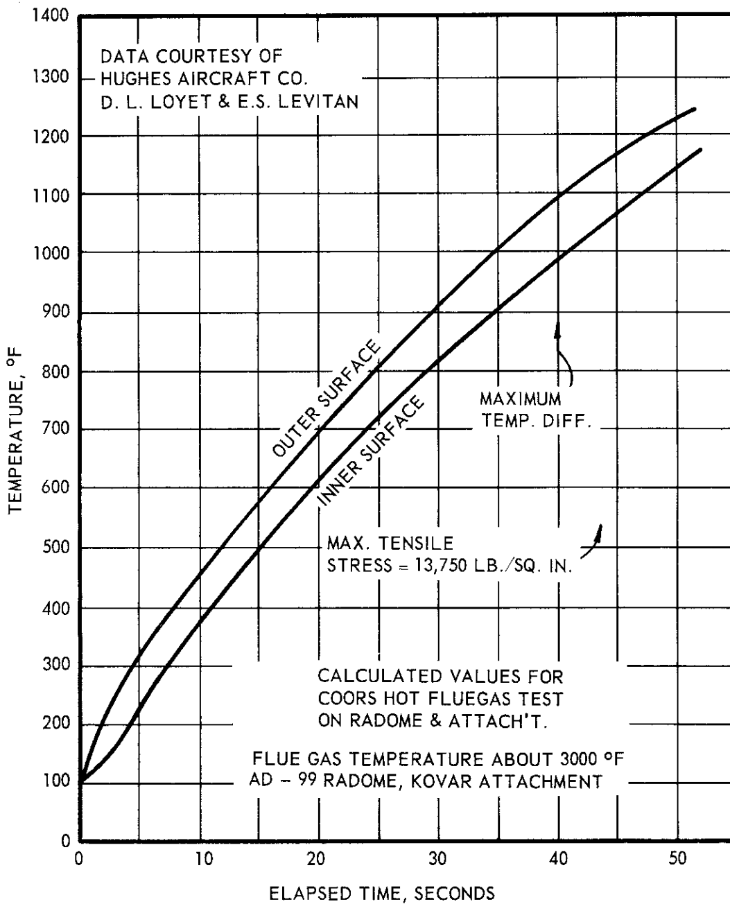
Figure 7. Thermal Gradient in the Wall of Radome Injected into Hot Gas Stream.
