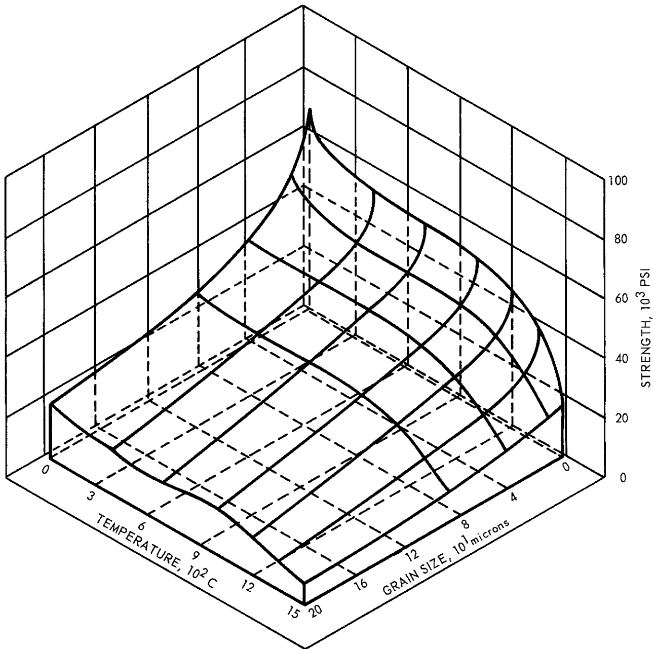
Figure 1. Strength-Temperature-Grain-Size Surface for Dense Pure Hot-Pressed Alumina.
