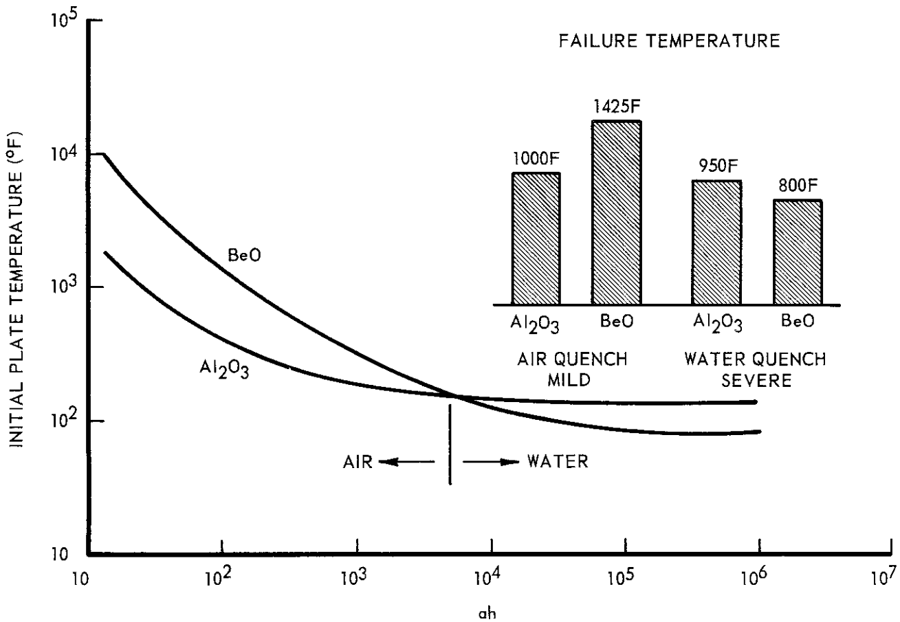
Figure 3. Relative Thermal Shock Resistance of Al 2 O 3 and BeO as Function of Thermal Shock Environment (ah).
