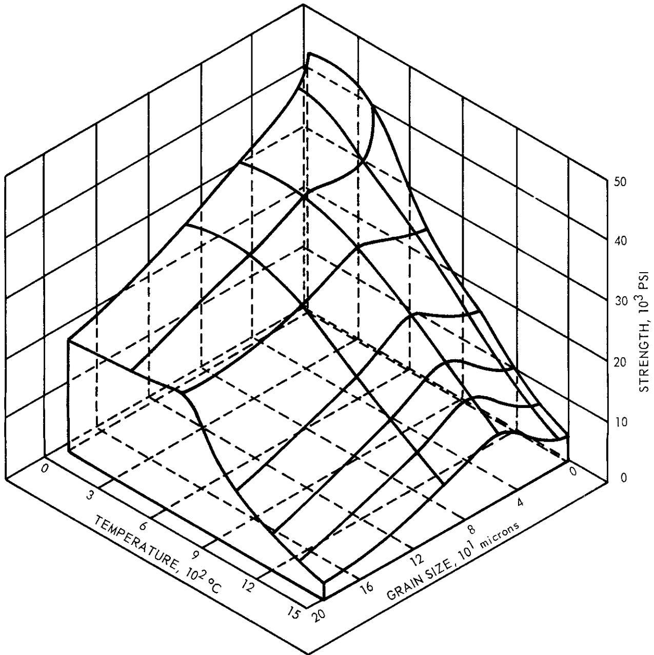
Figure 2. Strength-Temperature-Grain-Size Surface for Dense Pure Hot-Pressed Magnesia.
