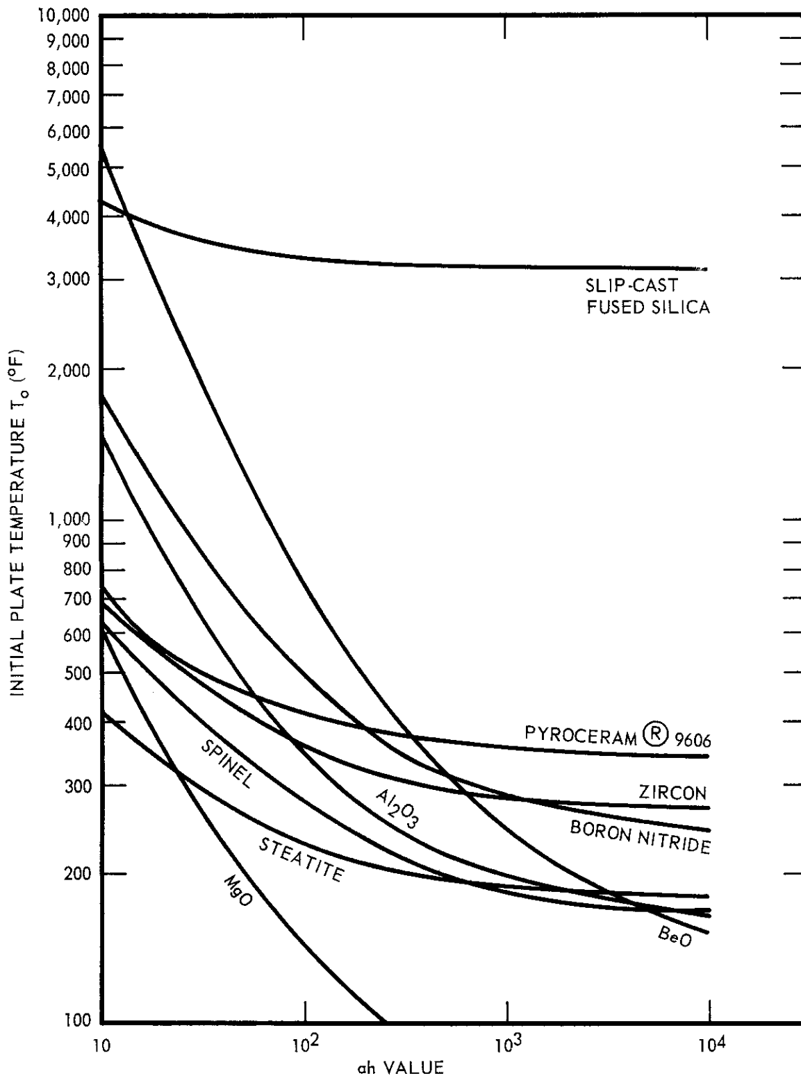
Figure 4. Relative Thermal Shock Resistance of Candidate Reentry Radome Materials as a Function of Thermal Shock Environment ( ah ).
