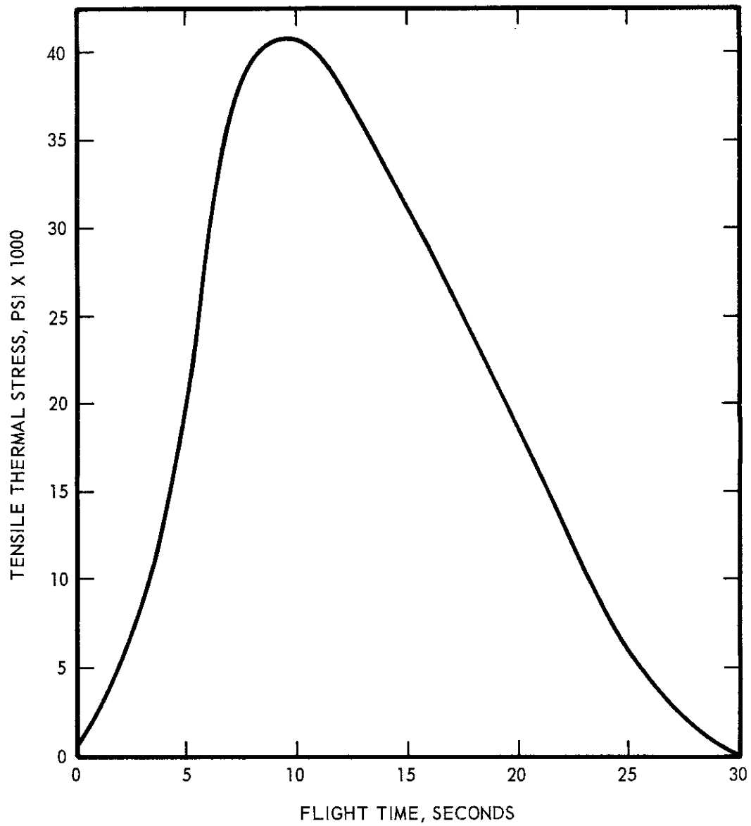
Figure 14. Tensile Thermal Stress at Stagnation Point Versus Flight Time for Alumina Radome.
