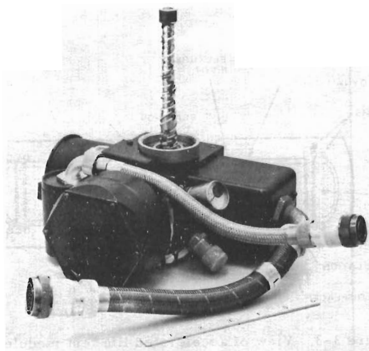
Figure 3-1. 77°K airborne VM refrigerator (71-7232)
