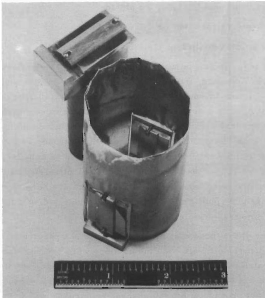
Figure 9. Aluminum foil test sleeve with sputtered \text{Cr}_3\text{Si}_2 (incomplete inside coverage)
