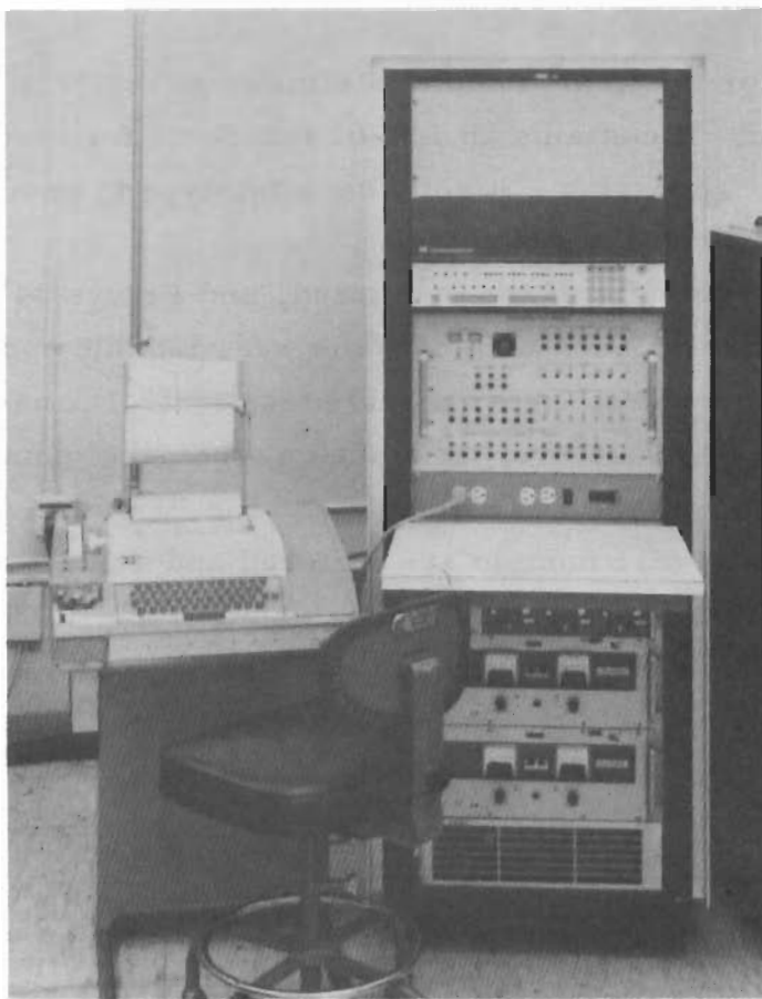
Figure 34. Wear module test console (76-50429)
