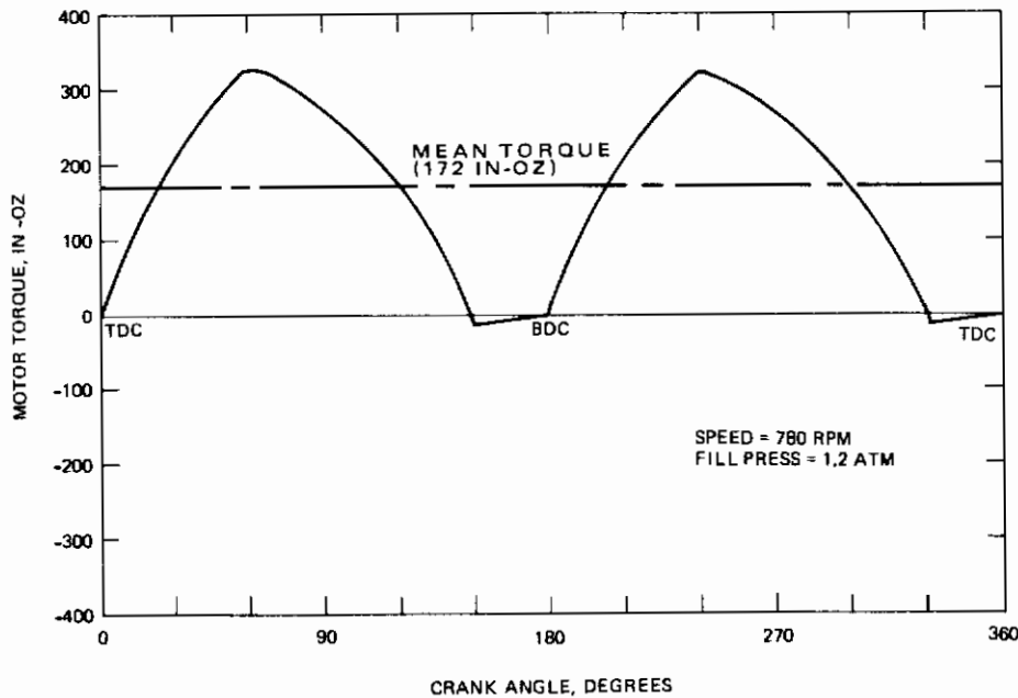
Figure 20. Motor torque as a function of crank angle
