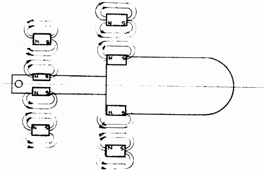
Figure 42. Schematic representation of magnetically supported displacer
