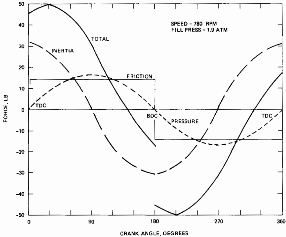
Figure 19. Summation of wrist pin forces as a function of crank angle
