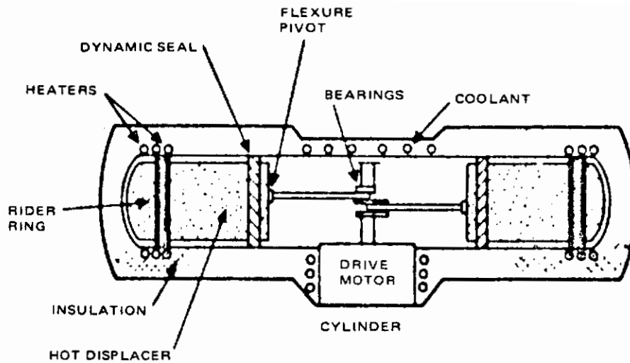
Figure 3-3. View of accelerated life test module
