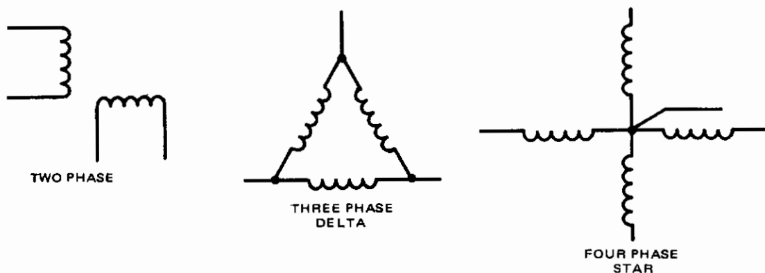
Figure 51. Three common winding configurations
