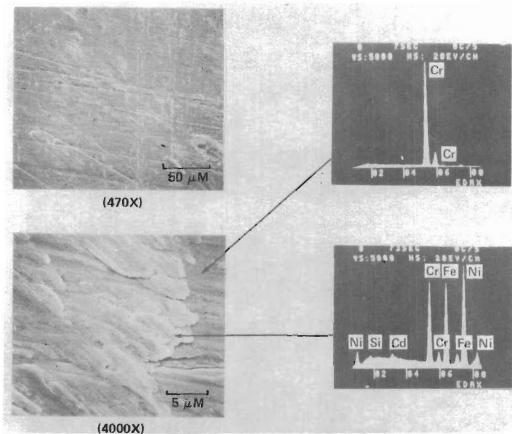
Figure 15. Ion plated \text{Cr}_{23}\text{C}_6 (lot 5); steel tip scratch
