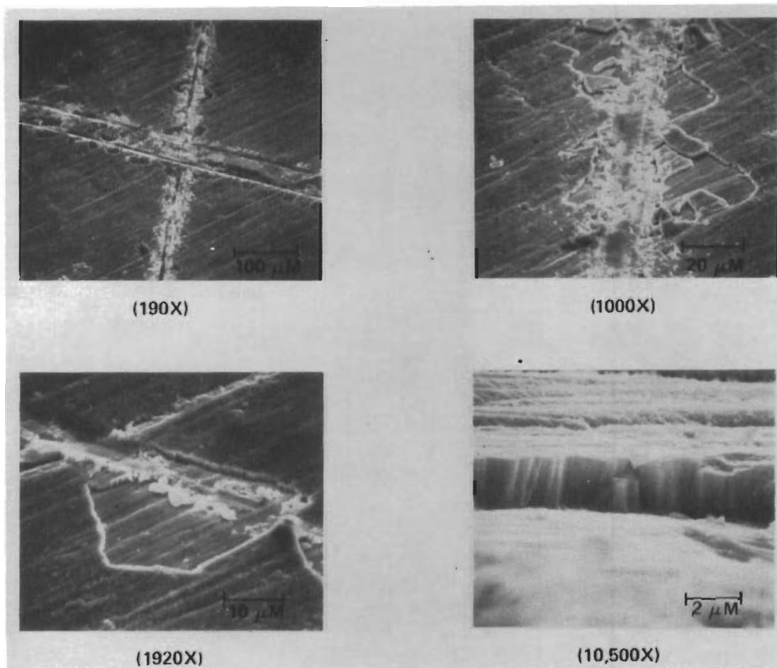
Figure 12. Sputtered \text{Cr}_3\text{Si}_2 (lot 1); carbide tip scratch
