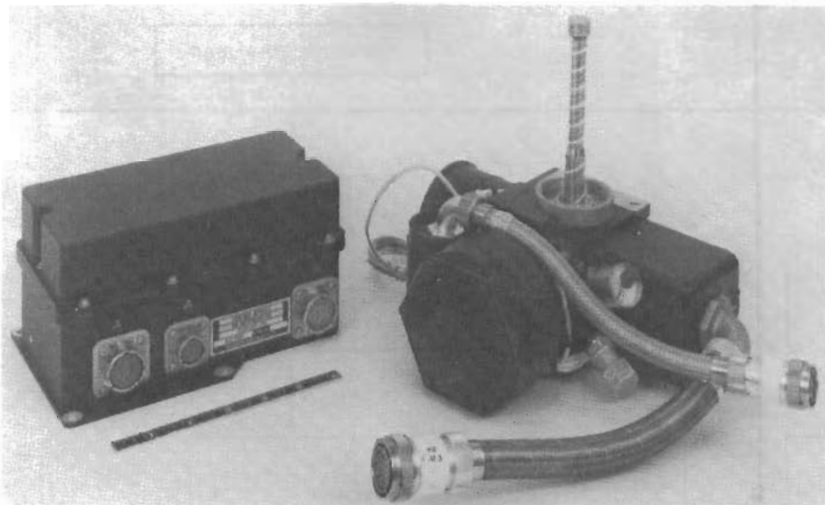
Figure 2. Airborne VM refrigerator manufactured by Hughes Aircraft Company (4R18086)
