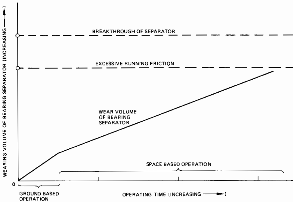
Figure 8. Wear characteristics of bearing separator
