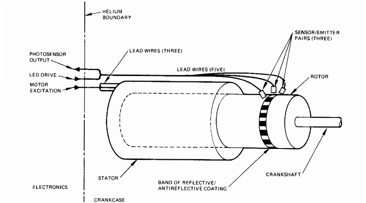
Figure 55. Mechanical schematic for recommended commutation scheme
