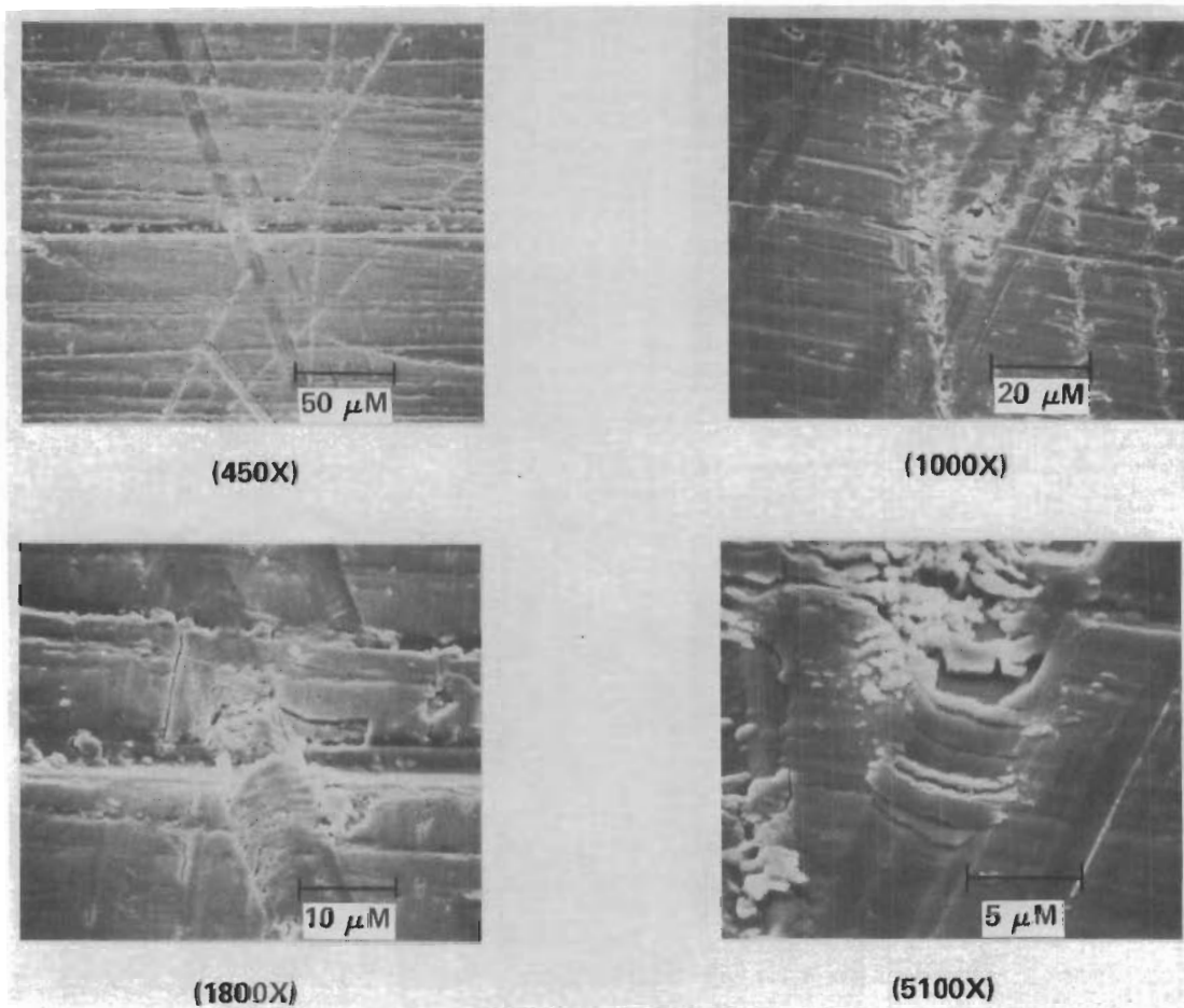
Figure 13. Ion plated \text{Cr}_{23}\text{C}_6 (lot 5); carbide tip scratch
