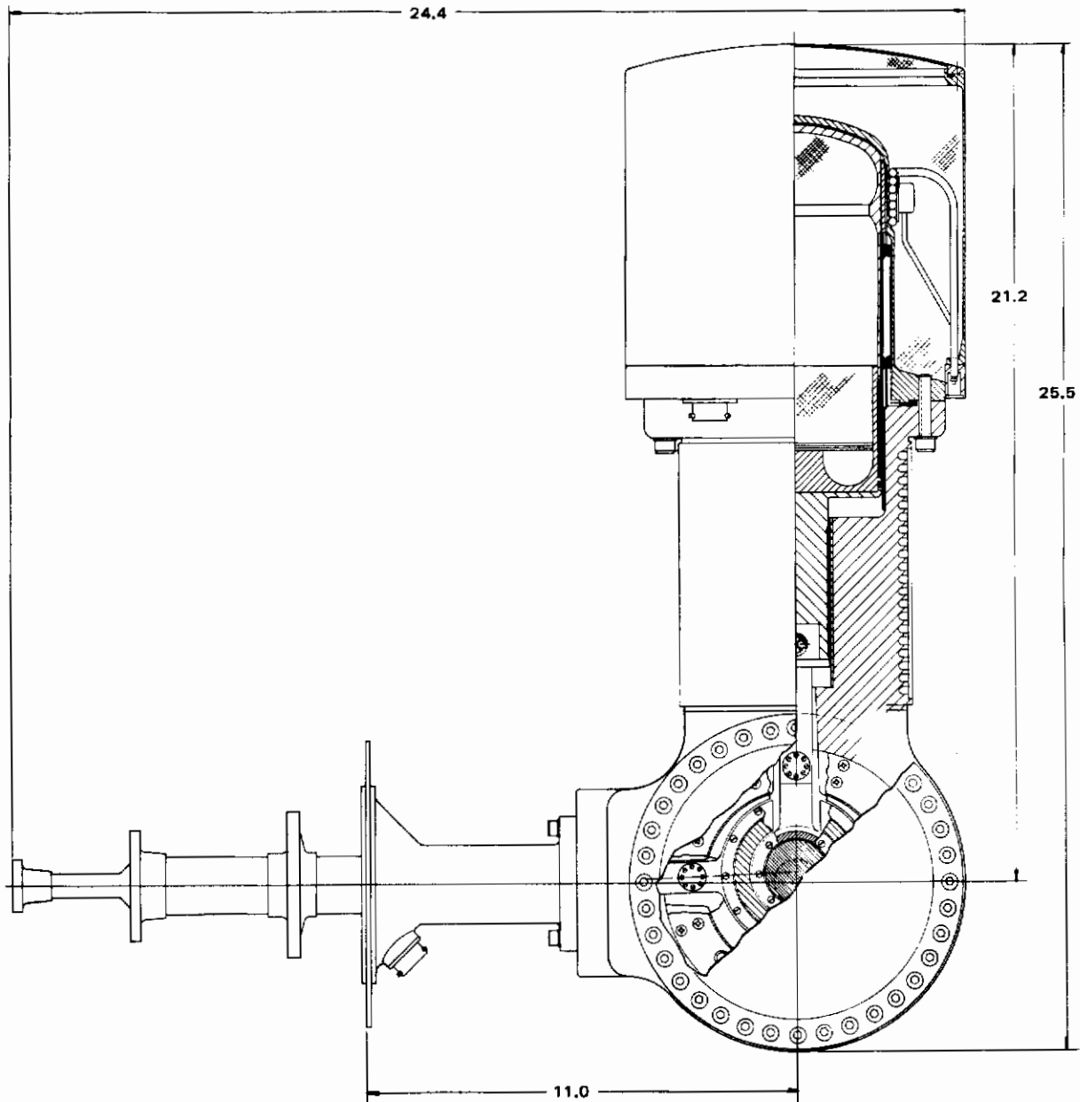
Figure 46. Crosshead support
