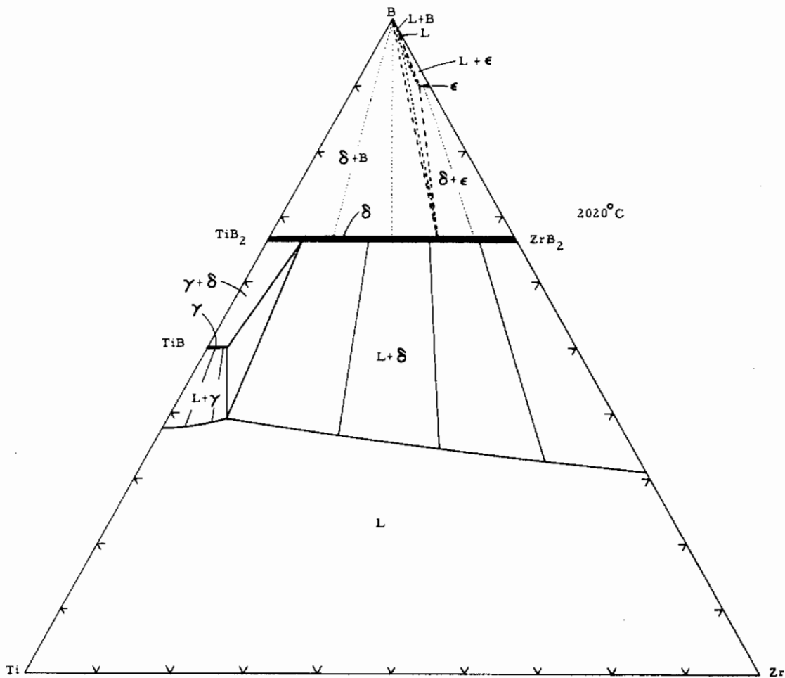
Figure 36. Isothermal section at 2020°C. [Four-Phase Reaction ( L + \delta \rightleftharpoons \epsilon + B )], Estimated.
