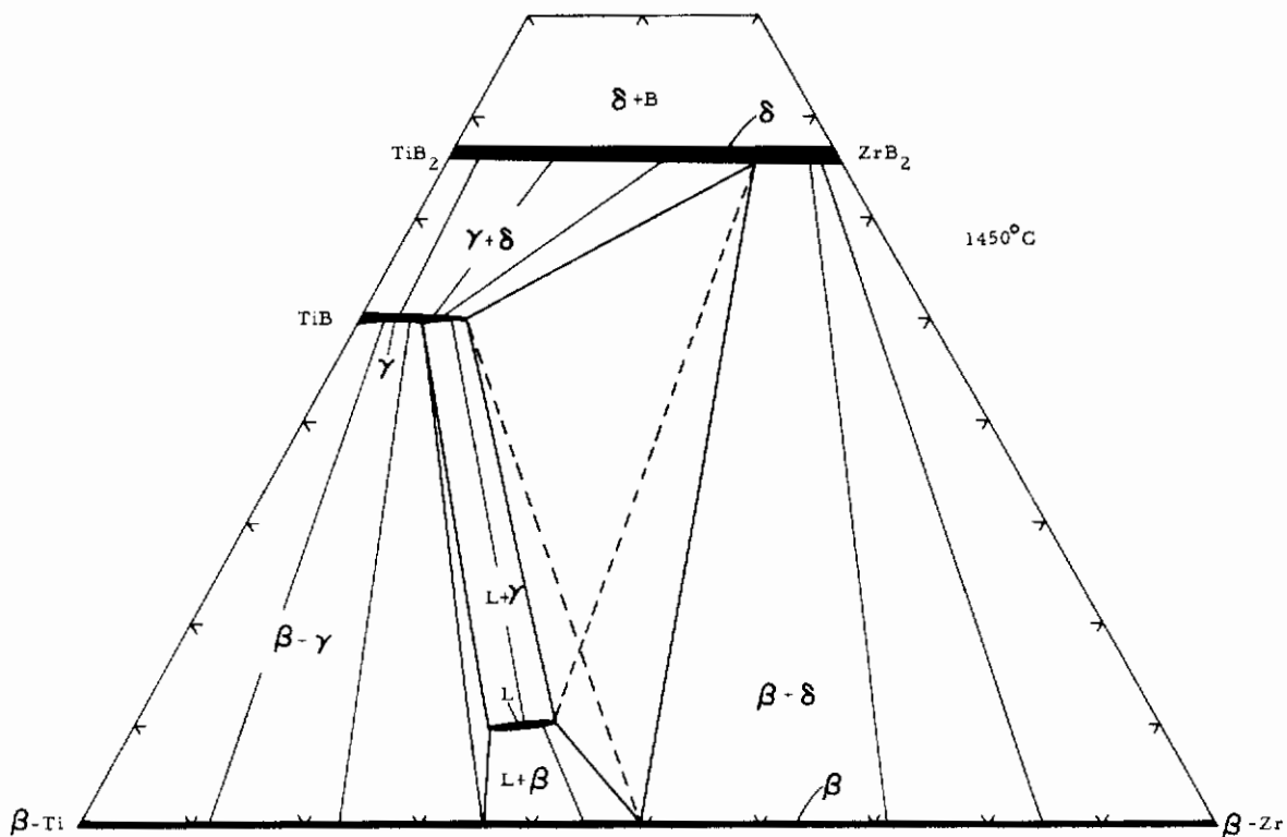
Figure 29. Isothermal Section at 1450°C. [Four-Phase Reaction ( L + \delta = \beta + \gamma )]
