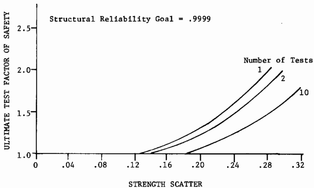
Figure 19. Ultimate Design and Test Factor of Safety for a Given Structural Reliability Goal Versus Strength Scatter (Reference 29)
