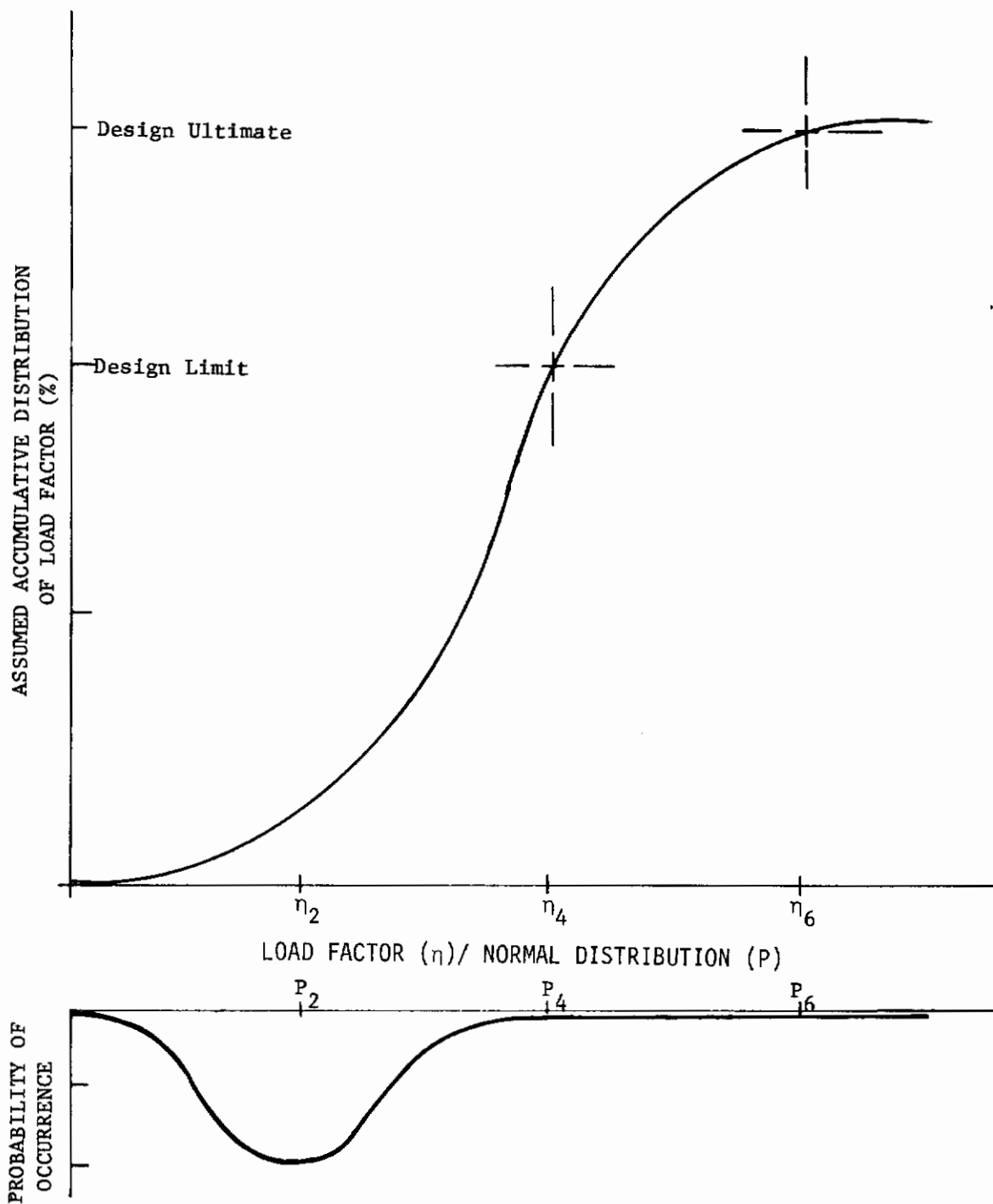
Figure 14. Statistical Representation of the Factor of Safety Design Concept
