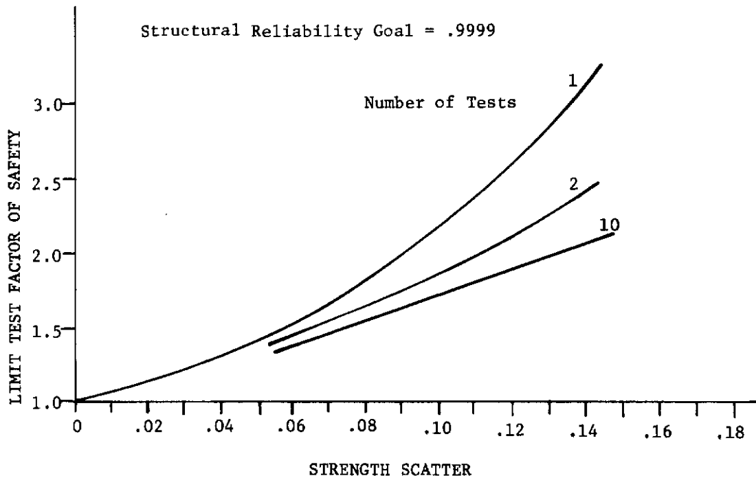
Figure 18. Limit Design and Test Factor of Safety for a Given Structural Reliability Goal Versus Strength Scatter (Reference 29)
