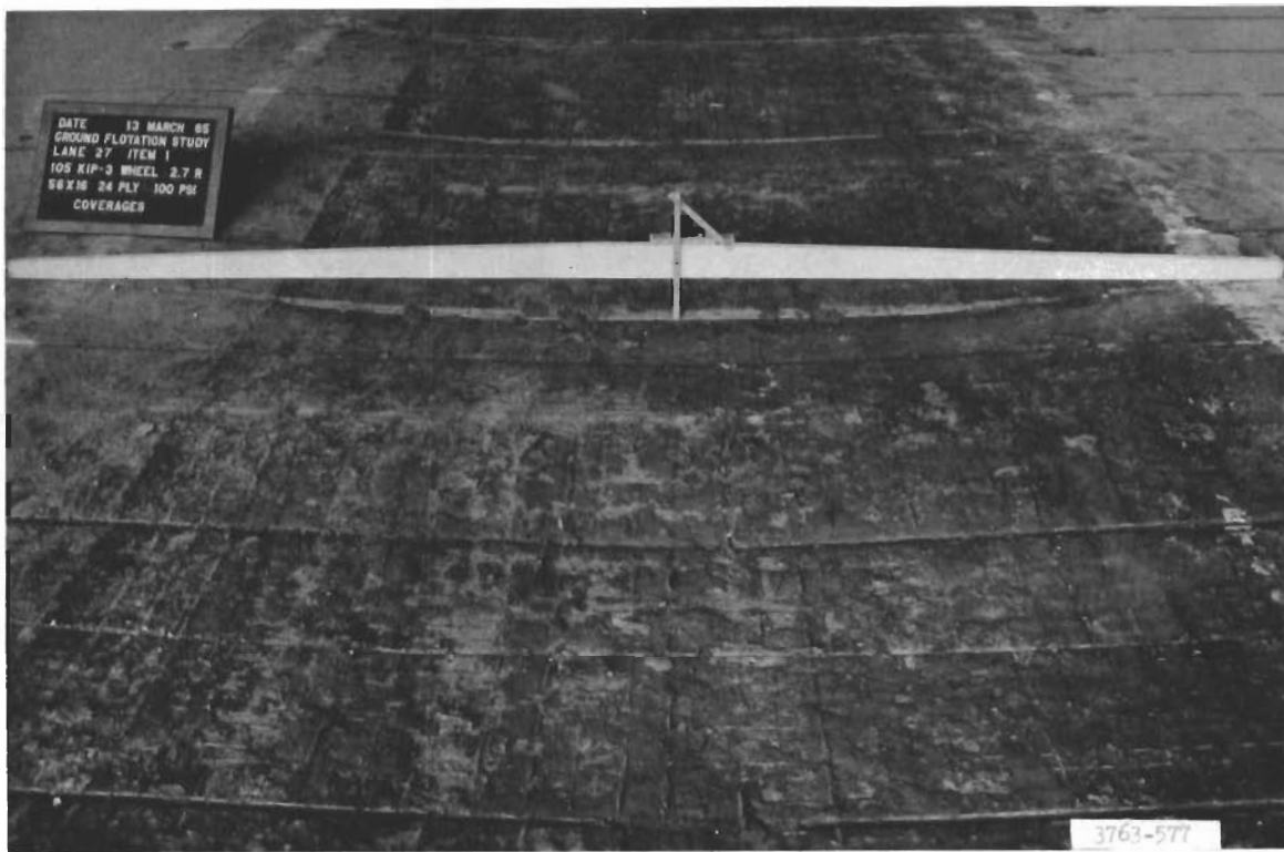
Figure 10. Lane 27, item 1. Transverse straightedge shows roughness at 68 coverages (failure)
