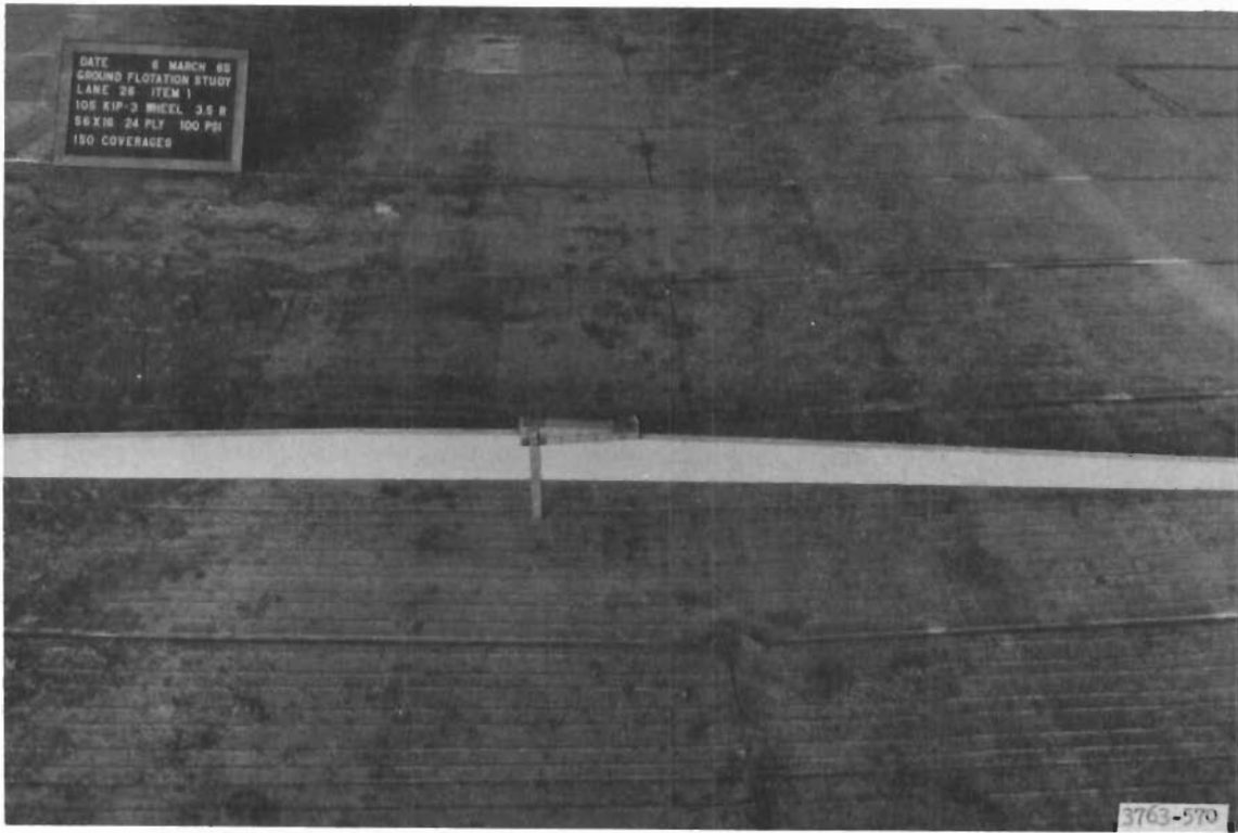
Figure 4. Lane 26, item 1. Transverse straightedge shows roughness at 150 coverages (failure)
