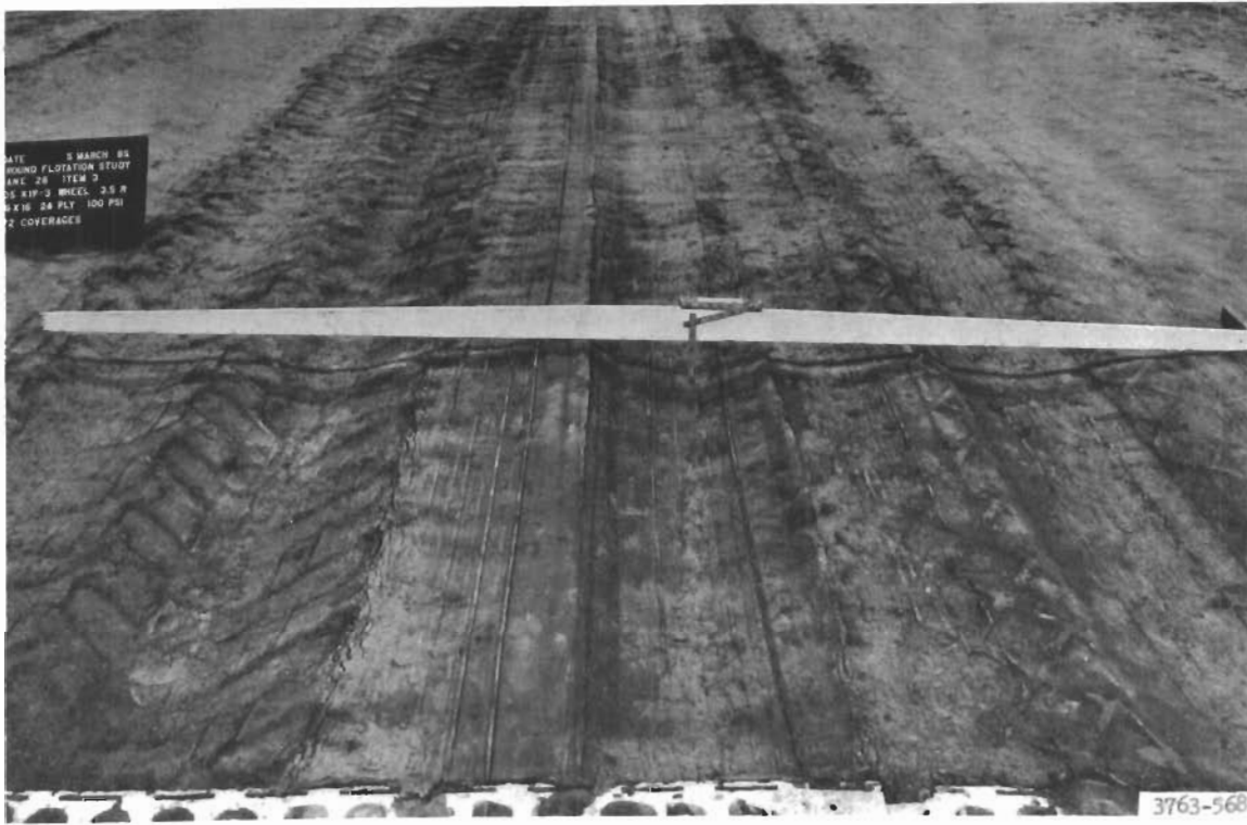
Figure 8. Lane 26, item 3. Transverse straightedge shows roughness at 72 coverages (failure)
