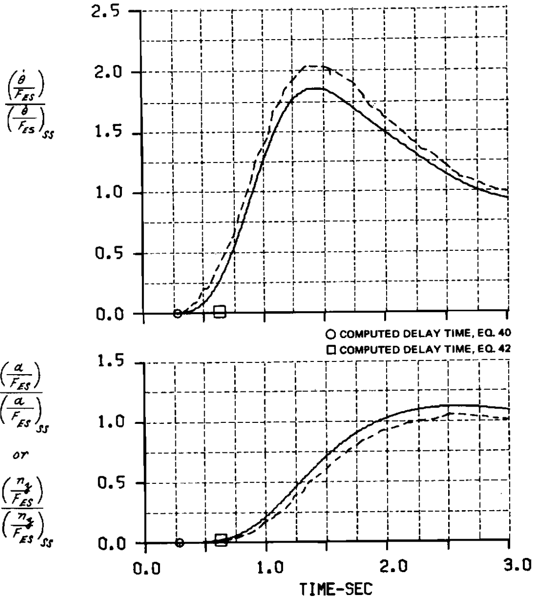
Figure A-33 COMPUTED AND MEASURED LONGITUDINAL SHORT PERIOD RESPONSES FOR A STEP ELEVATOR STICK FORCE INPUT CONF. LA(F)-5(1)
