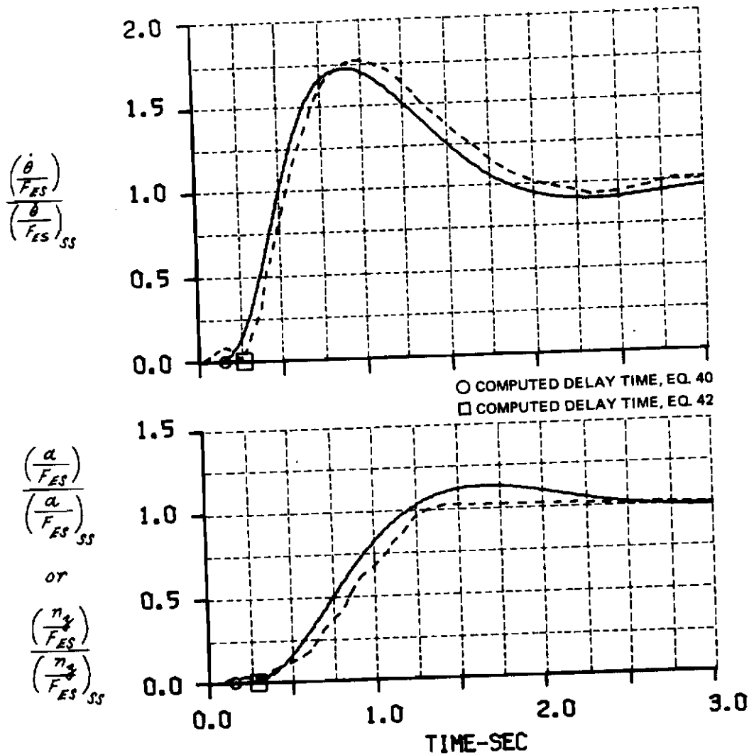
Figure A-8 COMPUTED AND MEASURED LONGITUDINAL SHORT PERIOD RESPONSES FOR A STEP ELEVATOR STICK FORCE INPUT CONF. A(M)-2(2.5)
