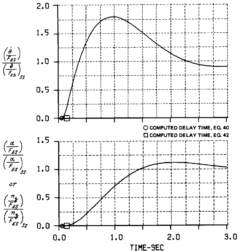
Figure A-28 COMPUTED AND MEASURED LONGITUDINAL SHORT PERIOD RESPONSES FOR A STEP ELEVATOR STICK FORCE INPUT CONF. LA(F)-2(10)
