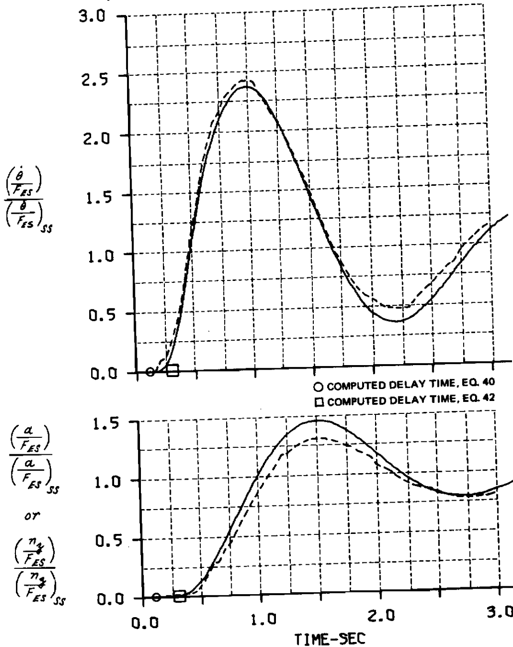
Figure A-17 COMPUTED AND MEASURED LONGITUDINAL SHORT PERIOD RESPONSES FOR A STEP ELEVATOR STICK FORCE INPUT CONF. 8(F)-5(2.5)
