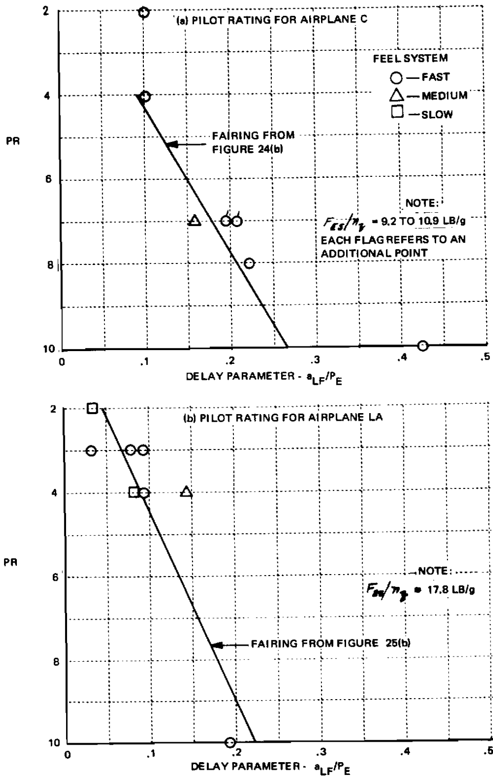
Figure 27 VARIATION OF PILOT RATING WITH DELAY PARAMETER (PILOT B - AIRPLANE CONF. C AND LA)
