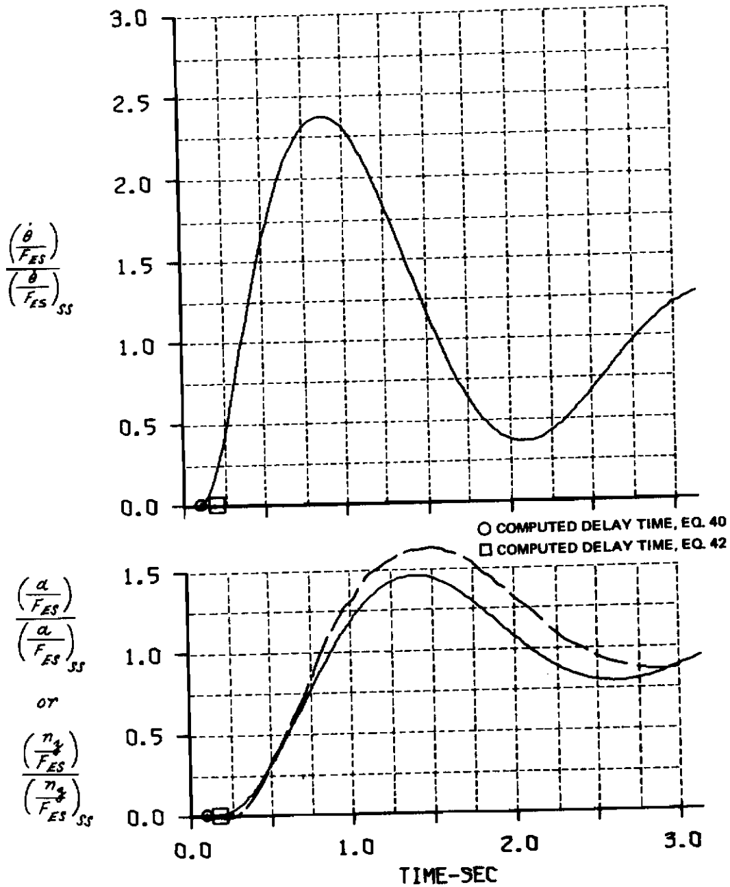
Figure A-14 COMPUTED AND MEASURED LONGITUDINAL SHORT PERIOD RESPONSES FOR A STEP ELEVATOR STICK FORCE INPUT CONF. B(F)-2(2.5)
