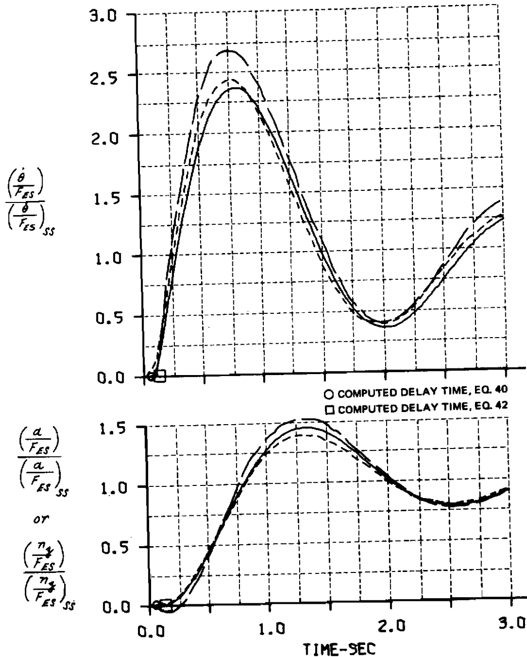
Figure A-13 COMPUTED AND MEASURED LONGITUDINAL SHORT PERIOD RESPONSES FOR A STEP ELEVATOR STICK FORCE INPUT CONF. B(F)-2(10)
