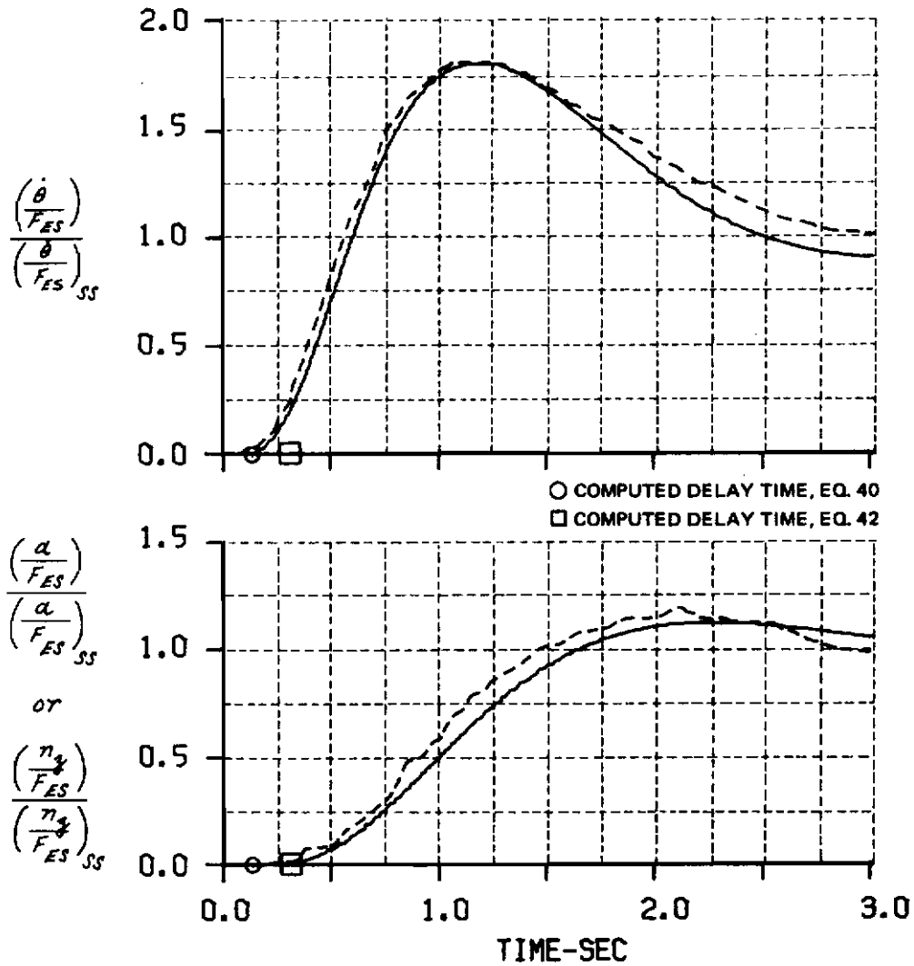
Figure A-30 COMPUTED AND MEASURED LONGITUDINAL SHORT PERIOD RESPONSES FOR A STEP ELEVATOR STICK FORCE INPUT CONF. LA(F)-2(1)
