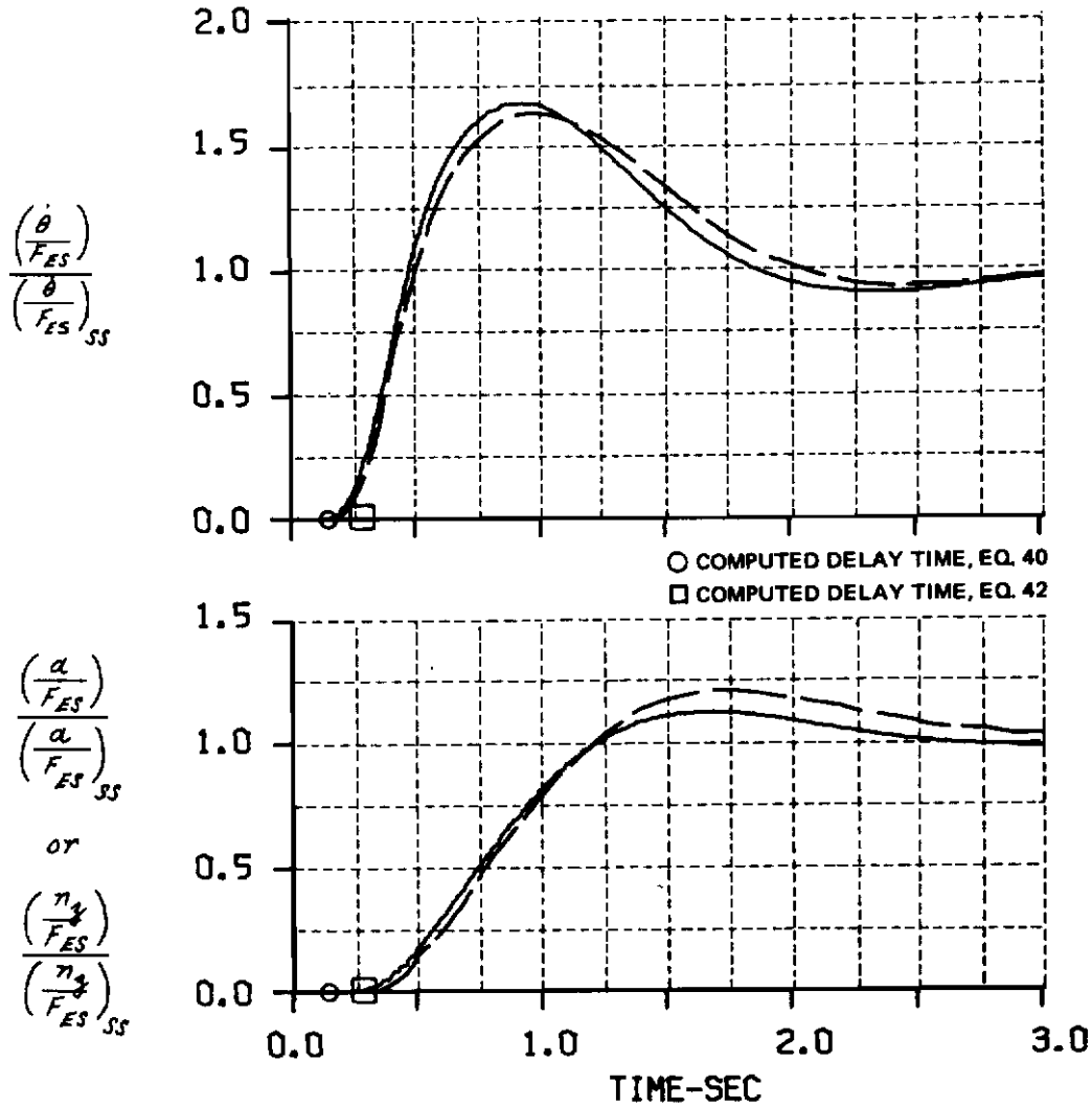
Figure A-4 COMPUTED AND MEASURED LONGITUDINAL SHORT PERIOD RESPONSES FOR A STEP ELEVATOR STICK FORCE INPUT CONF. A(F)-4(2.5)
