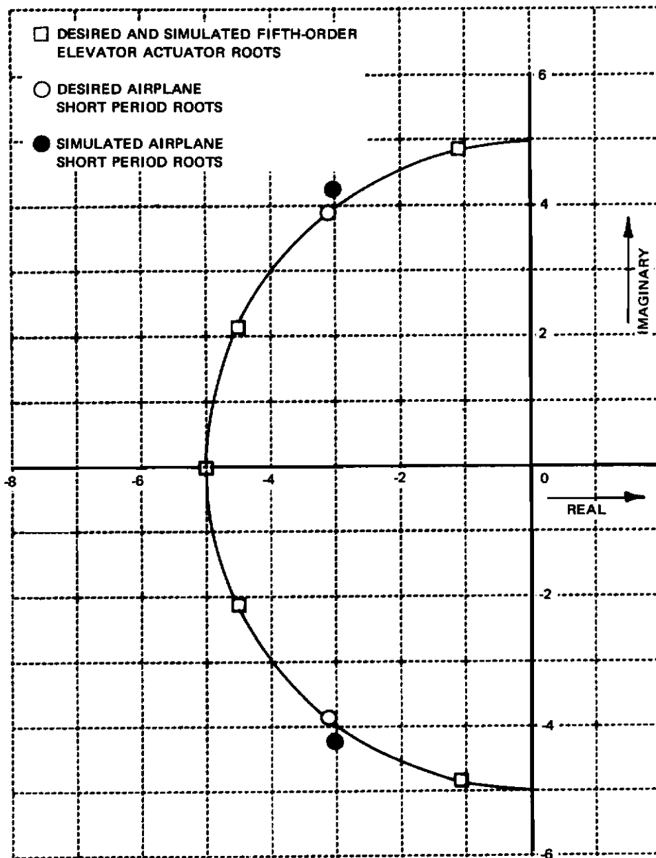
Figure 7 BUTTERWORTH DISTRIBUTION OF ACTUATOR AND AIRPLANE LONGITUDINAL SHORT PERIOD ROOTS FOR CONFIGURATION C_1(F)-5(.796)
