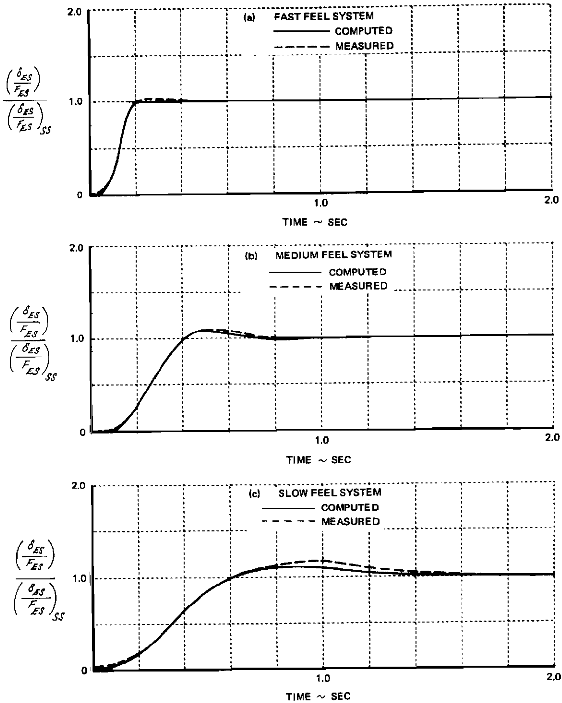
Figure 3 RESPONSE CHARACTERISTICS OF THE FEEL SYSTEM TO A STEP STICK FORCE INPUT (SECOND-ORDER FEEL SYSTEM WITH NOTCH FILTER)
