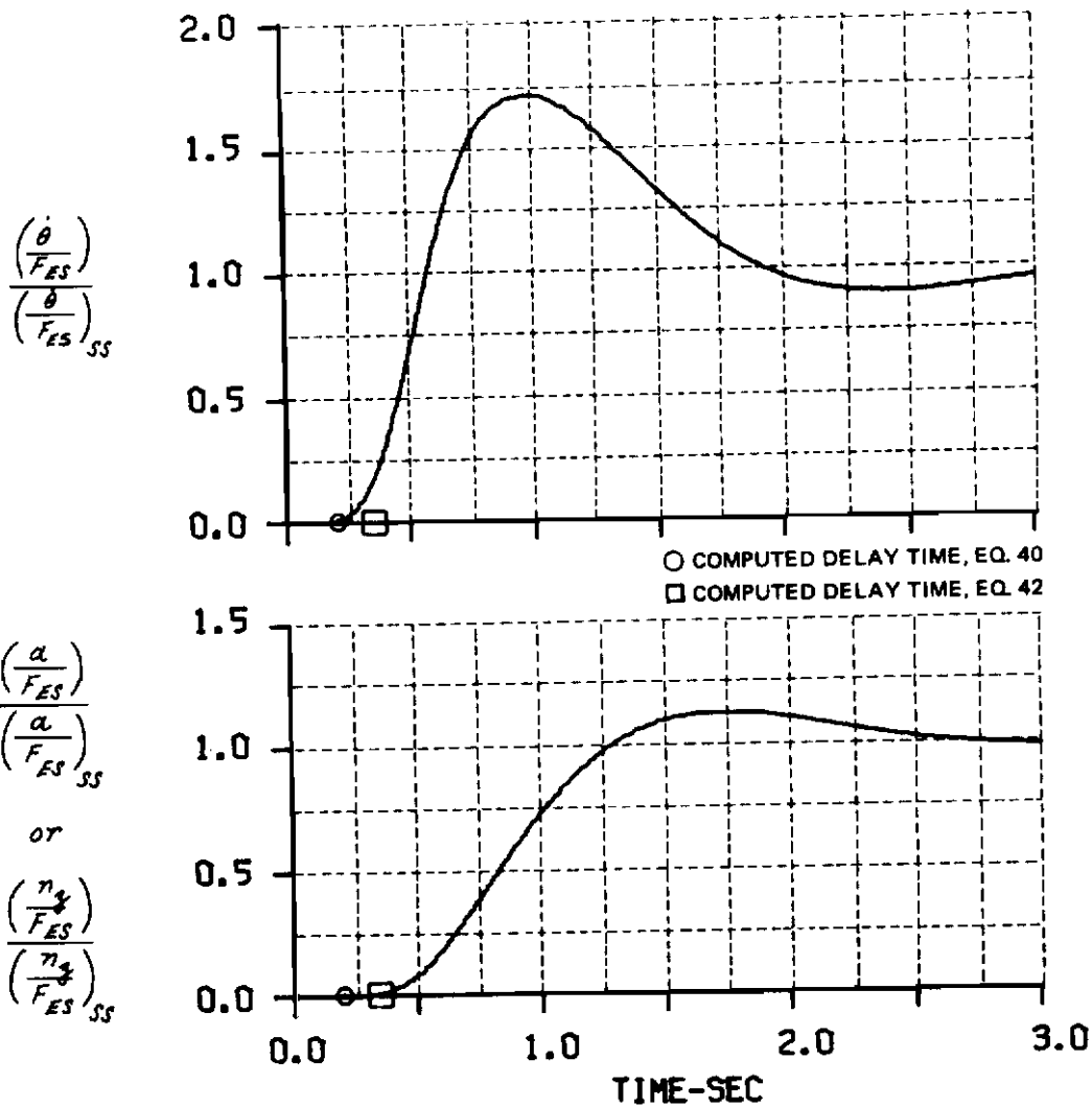
Figure A-9 COMPUTED AND MEASURED LONGITUDINAL SHORT PERIOD RESPONSES FOR A STEP ELEVATOR STICK FORCE INPUT CONF. A(M)-4(2.5)
