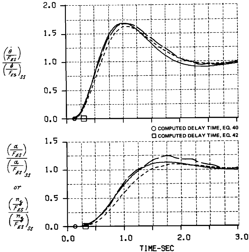
Figure A-3 COMPUTED AND MEASURED LONGITUDINAL SHORT PERIOD RESPONSES FOR A STEP ELEVATOR STICK FORCE INPUT CONF. A(F)-2(1)
