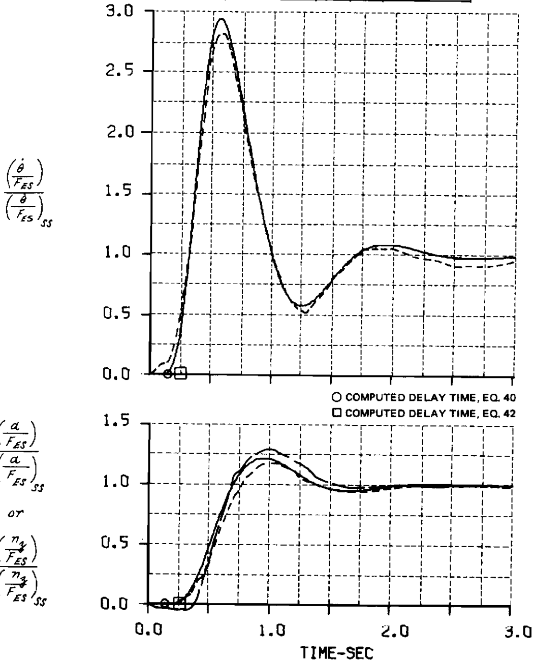
Figure A-22 COMPUTED AND MEASURED LONGITUDINAL SHORT PERIOD RESPONSES FOR A STEP ELEVATOR STICK FORCE INPUT CONF. C(F)-4(2.5)
