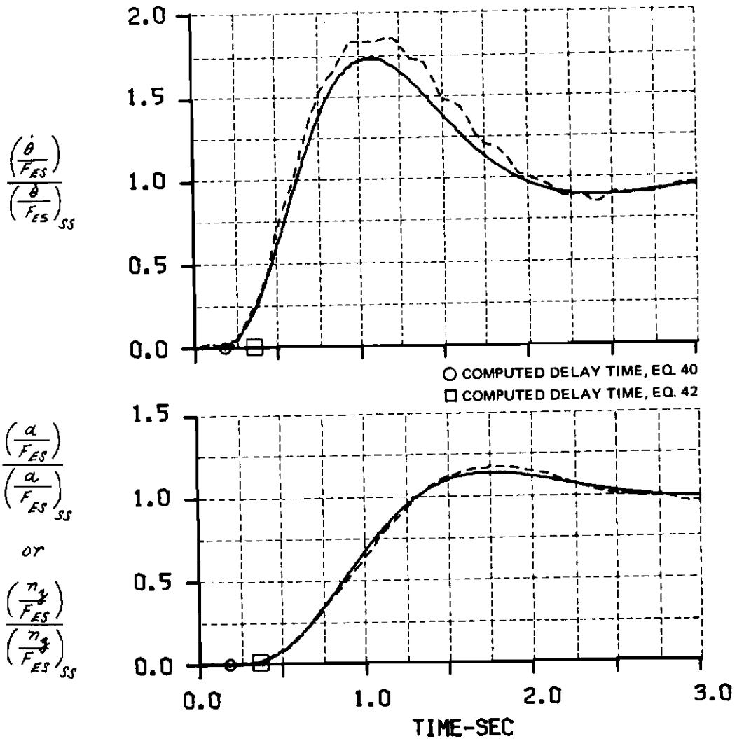
Figure A-11' COMPUTED AND MEASURED LONGITUDINAL SHORT PERIOD RESPONSES FOR A STEP ELEVATOR STICK FORCE INPUT CONF. A(S)-2(2.5)
