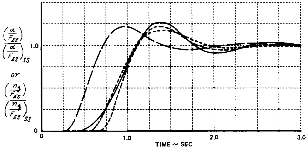
Figure 19 COMPARISON OF HIGHER-ORDER LONGITUDINAL RESPONSES WITH SECOND-ORDER RESPONSES WITH TIME DELAY FOLLOWING A STEP STICK FORCE INPUT - CONF. C(F)-5(1)
