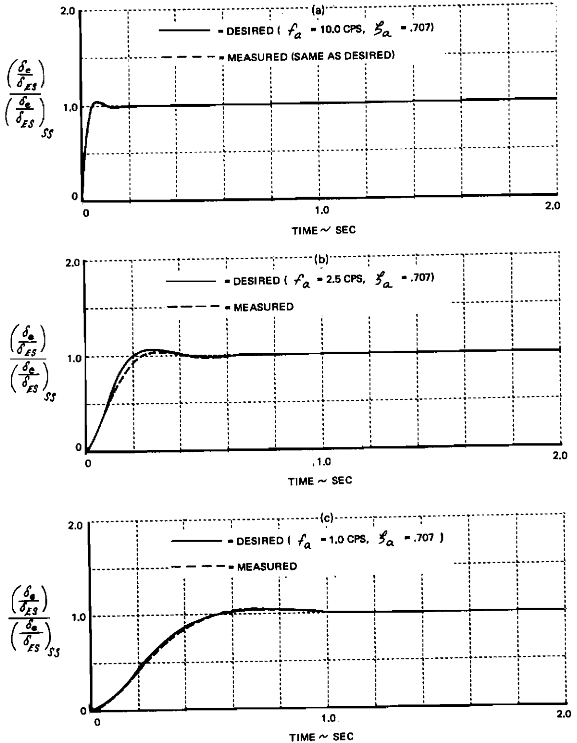
Figure 4 ELEVATOR RESPONSE TO STEP STICK INPUTS FOR VARIOUS ACTUATORS SIMULATED (SECOND-ORDER ACTUATORS)
