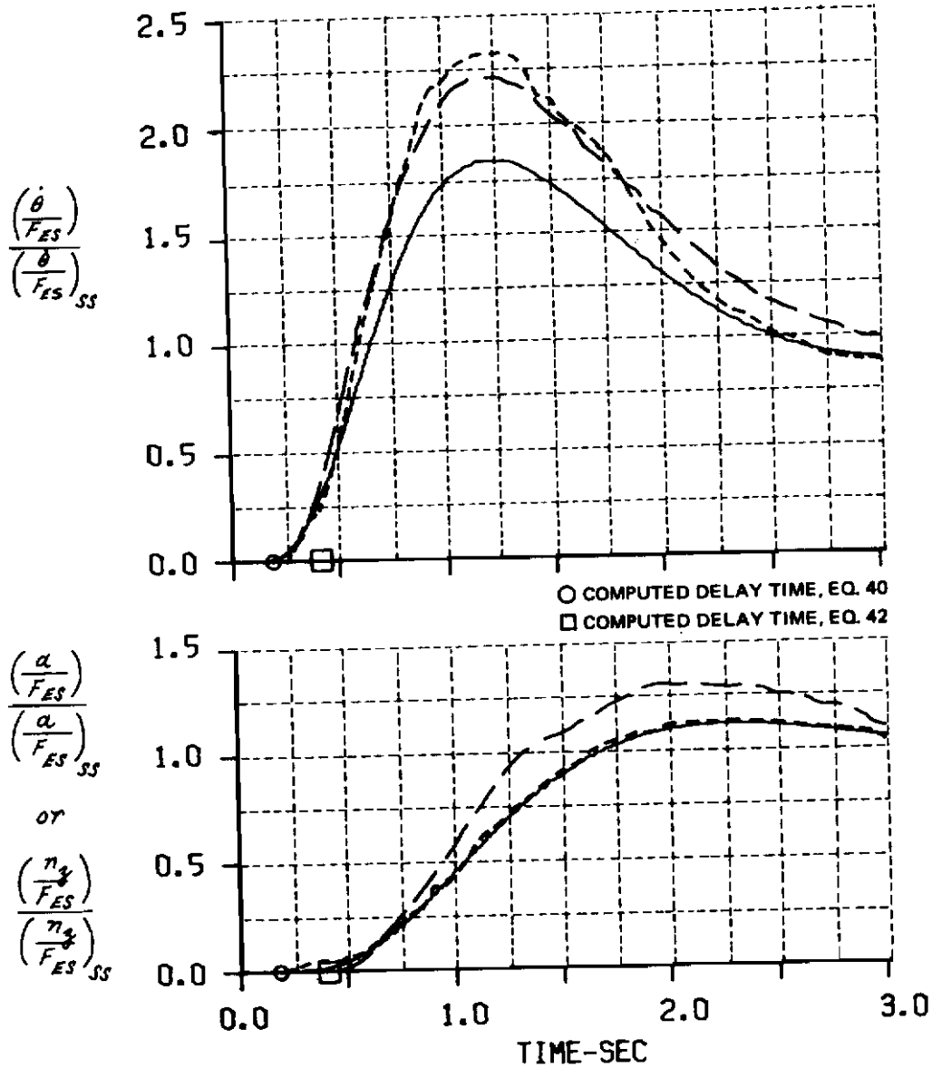
Figure A-37 COMPUTED AND MEASURED LONGITUDINAL SHORT PERIOD RESPONSES FOR A STEP ELEVATOR STICK FORCE INPUT CONF. LA(S)-2(2.5)
