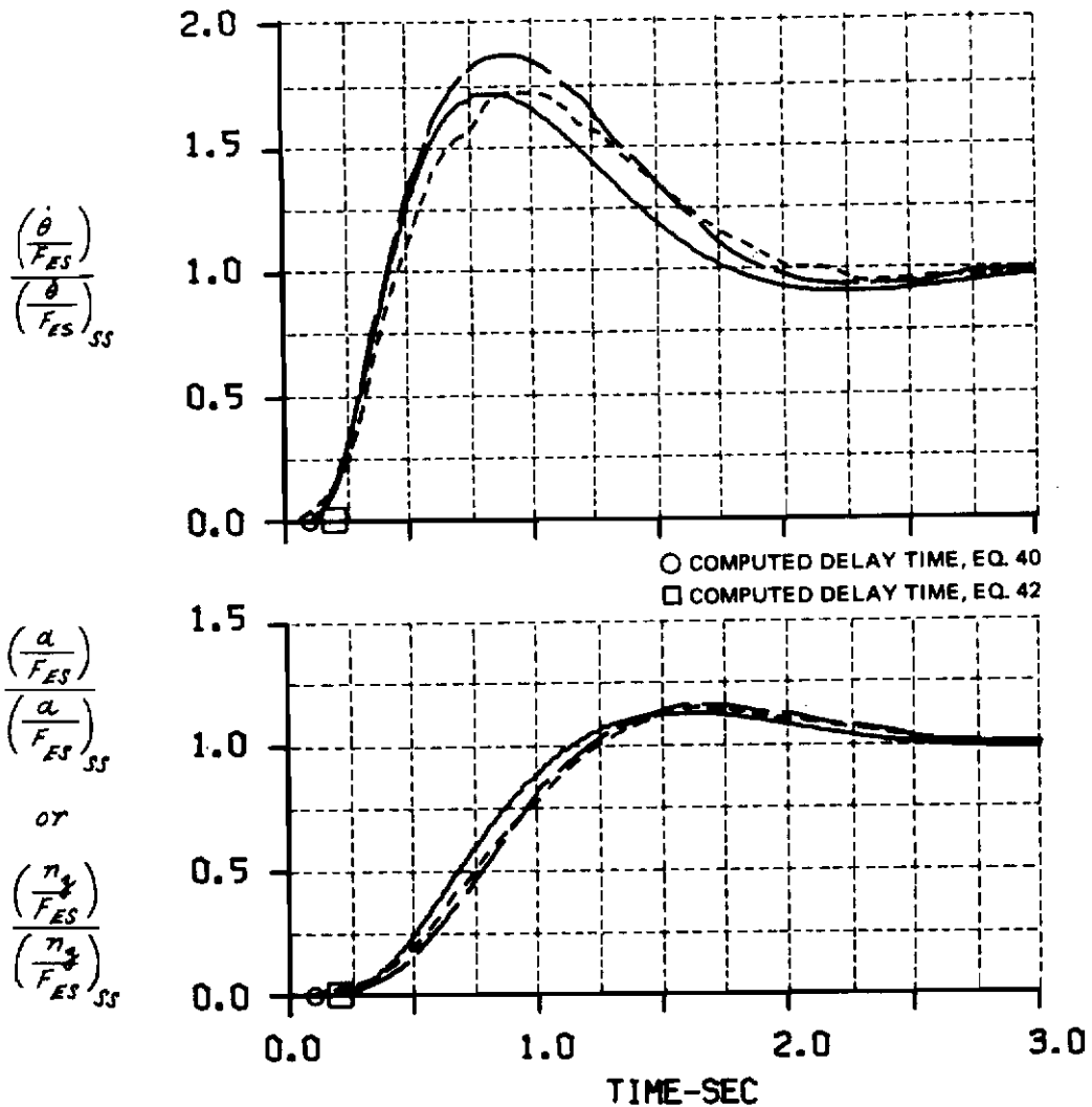
Figure A-7 COMPUTED AND MEASURED LONGITUDINAL SHORT PERIOD RESPONSES FOR A STEP ELEVATOR STICK FORCE INPUT CONF. A(M)-2(10)
