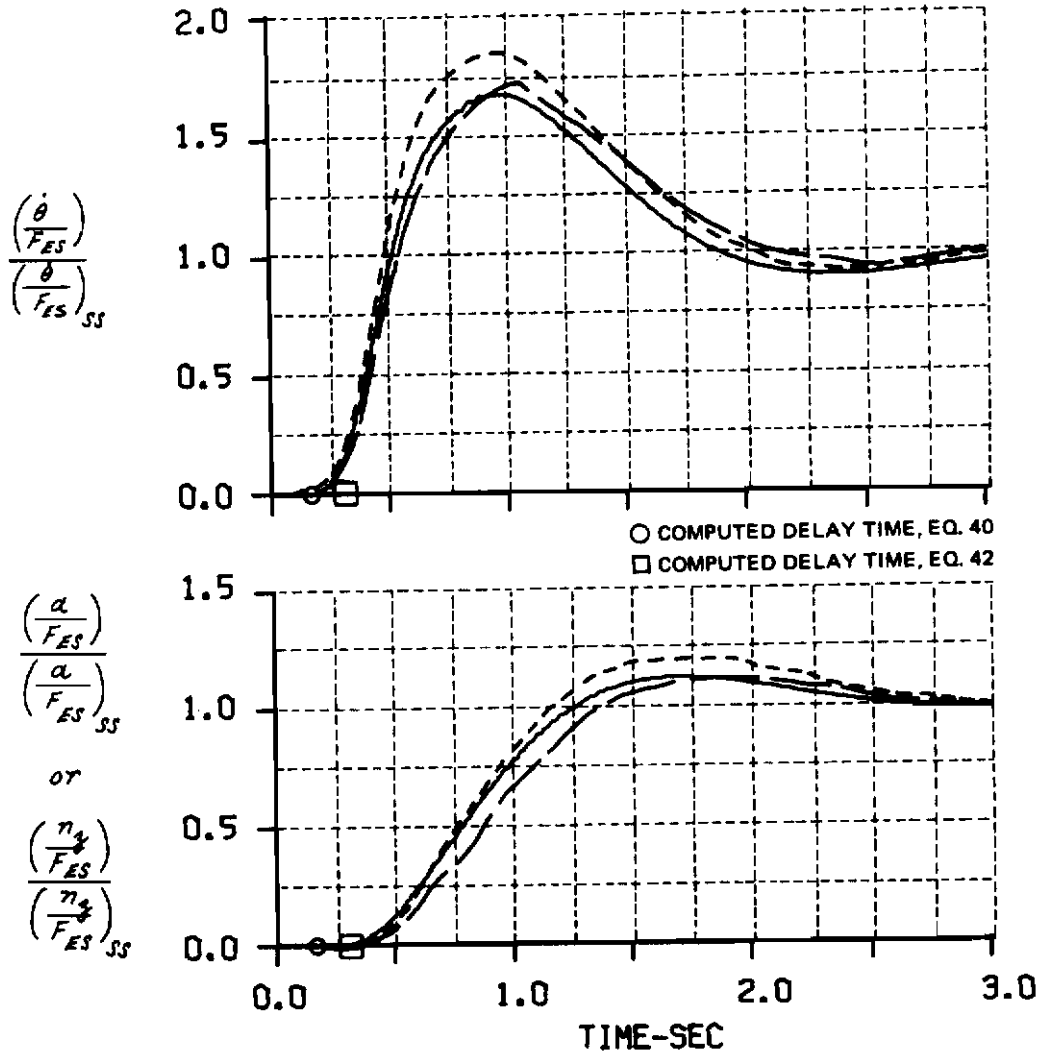
Figure A-5 COMPUTED AND MEASURED LONGITUDINAL SHORT PERIOD RESPONSES FOR A STEP ELEVATOR STICK FORCE INPUT CONF. A(F)-5(2.5)
