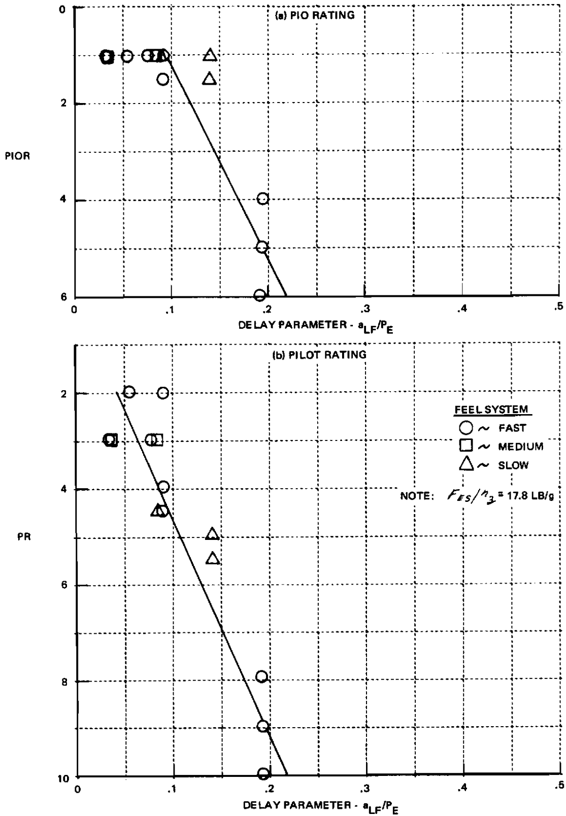
Figure 25 VARIATION OF PILOT RATING AND PIO RATING WITH DELAY PARAMETER (PILOT H - AIRPLANE CONF. LA)
