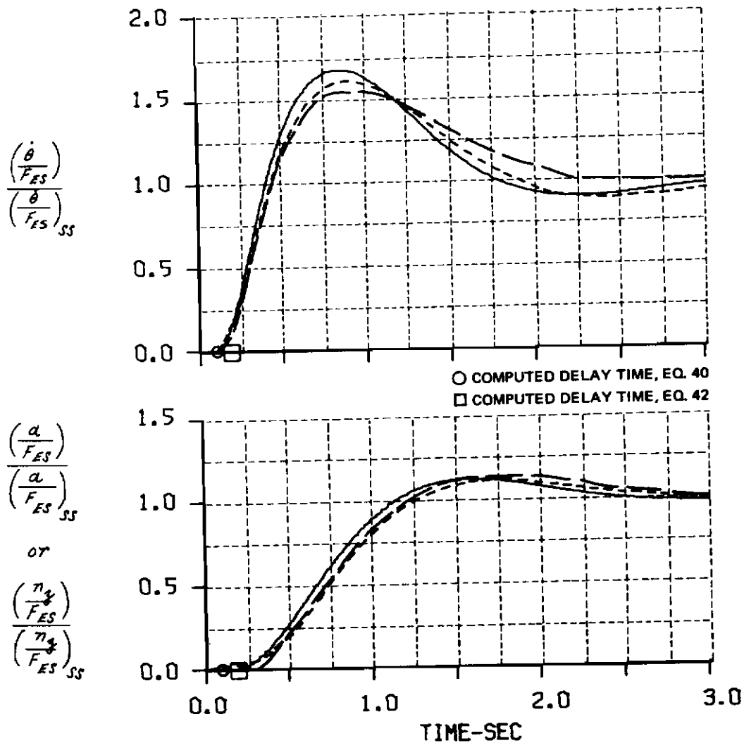
Figure A-2 COMPUTED AND MEASURED LONGITUDINAL SHORT PERIOD RESPONSES FOR A STEP ELEVATOR STICK FORCE INPUT CONF. A(F)-2(2.5)
