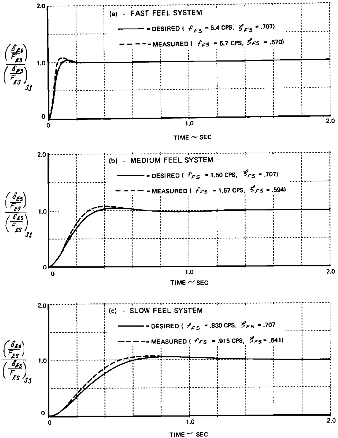
Figure 2 RESPONSE CHARACTERISTICS OF THE FEEL SYSTEM TO A STEP STICK FORCE INPUT (SECOND-ORDER FEEL SYSTEMS—NO NOTCH FILTER)
