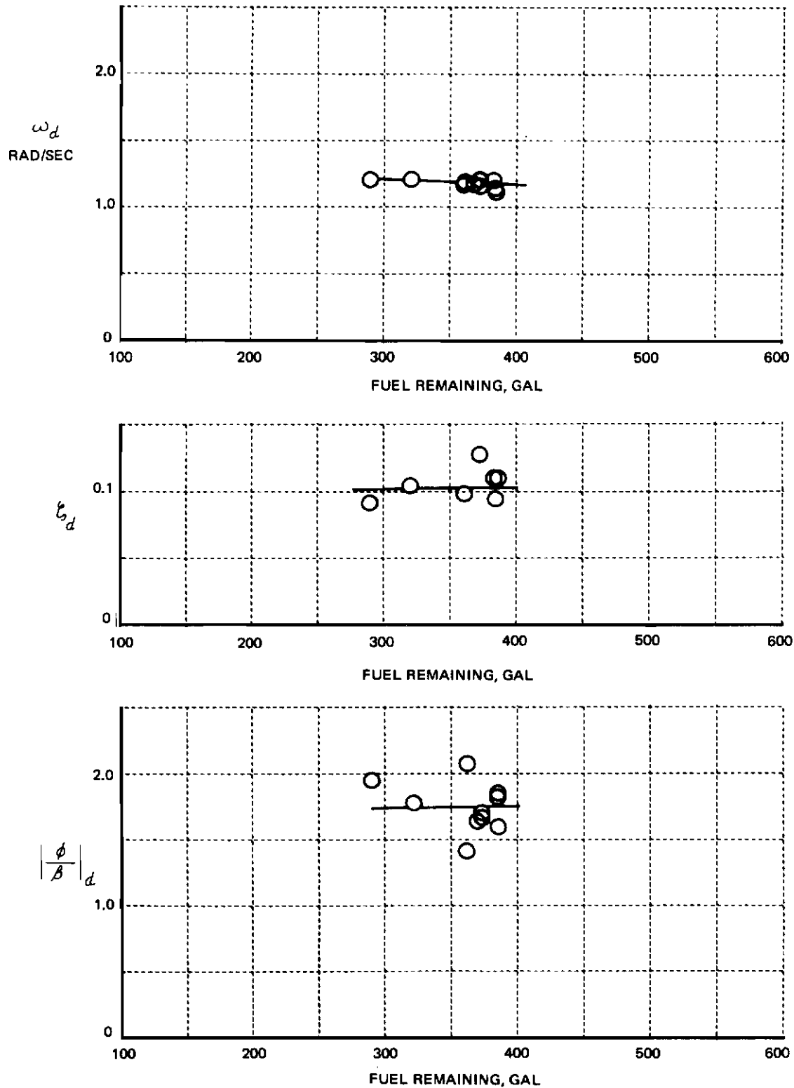
Figure 9 IN-FLIGHT MEASUREMENTS OF LATERAL-DIRECTIONAL MODE CHARACTERISTICS SIMULATED (LANDING APPROACH FLIGHT CONDITION)
