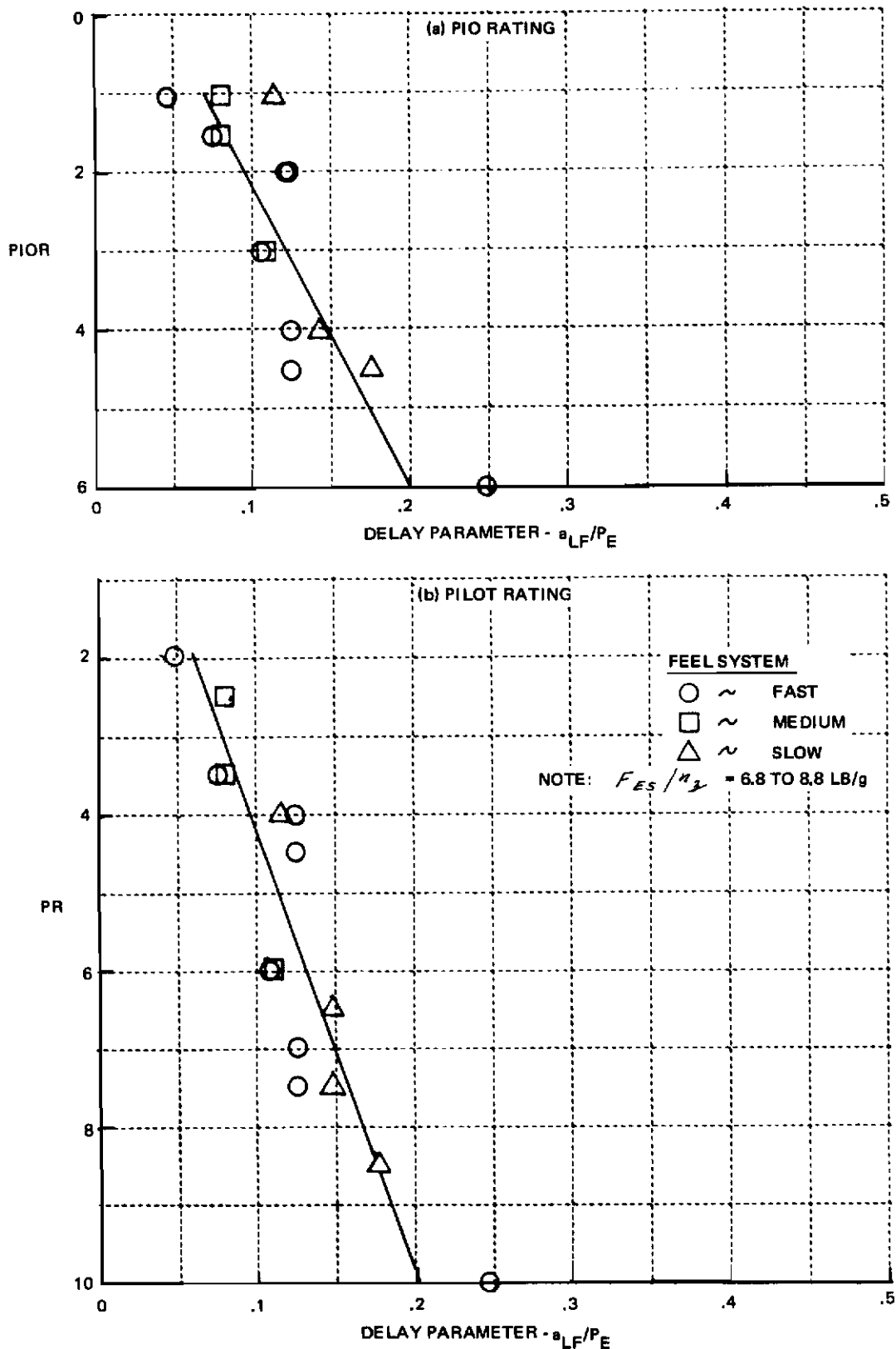
Figure 22 VARIATION OF PILOT RATING AND PIO RATING WITH DELAY PARAMETER (PILOT H - AIRPLANE CONF. A)
