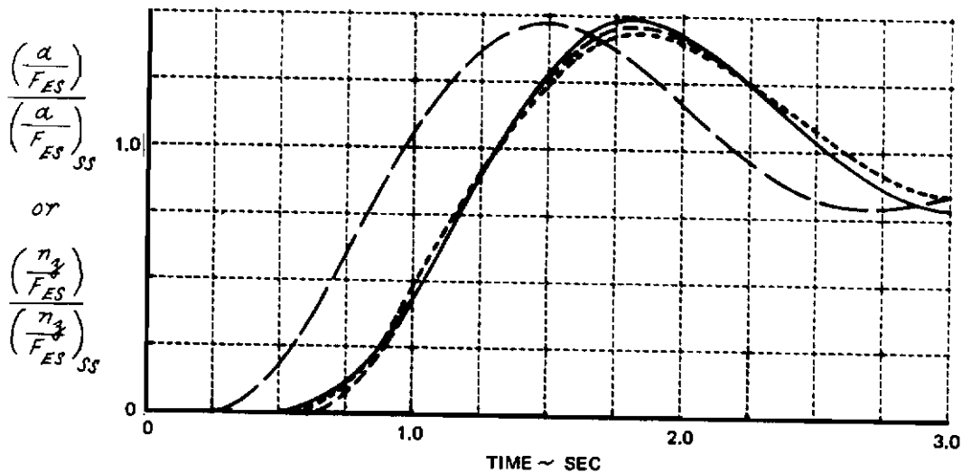
Figure 18 COMPARISON OF HIGHER-ORDER LONGITUDINAL RESPONSES WITH SECOND-ORDER RESPONSES WITH TIME DELAY FOLLOWING A STEP STICK FORCE INPUT - CONF. B(F)-5(1)
