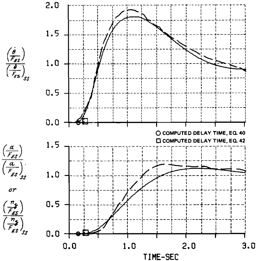
Figure A-35 COMPUTED AND MEASURED LONGITUDINAL SHORT PERIOD RESPONSES FOR A STEP ELEVATOR STICK FORCE INPUT CONF. LA(M)-2(2.5)
