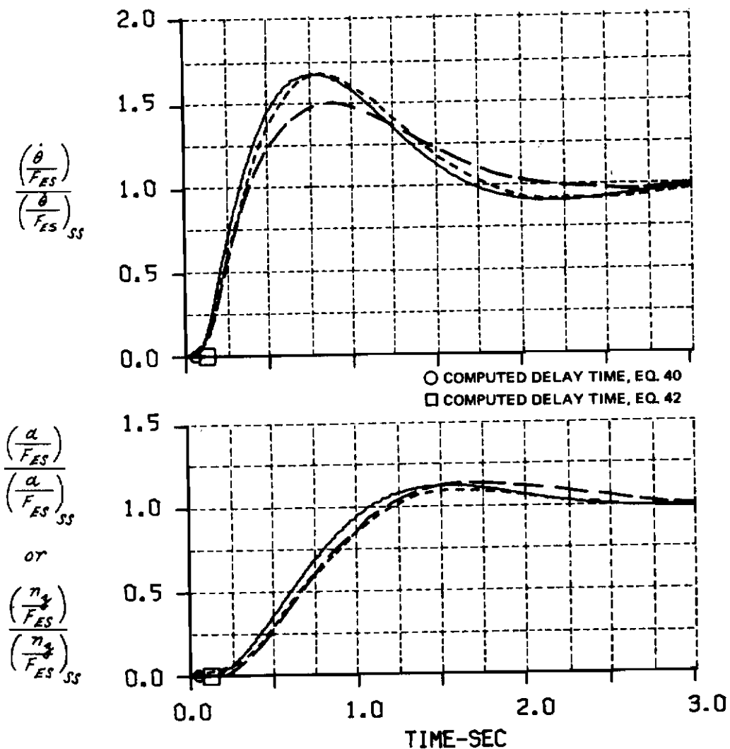
Figure A-1 COMPUTED AND MEASURED LONGITUDINAL SHORT PERIOD RESPONSES FOR A STEP ELEVATOR STICK FORCE INPUT CONF. A(F)-2(10)
