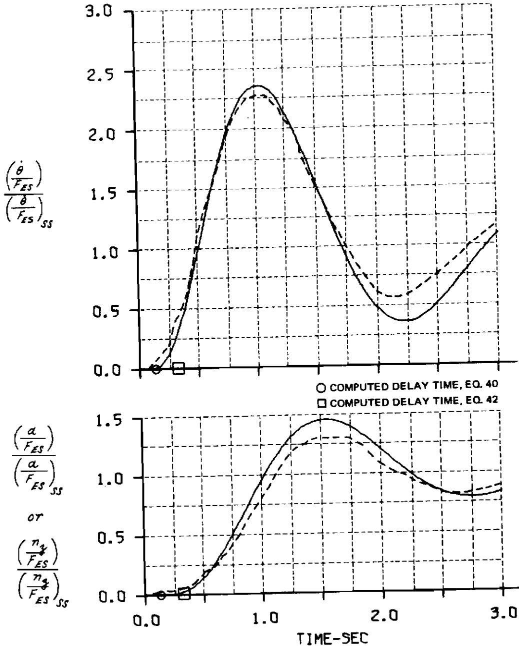
Figure A-15 COMPUTED AND MEASURED LONGITUDINAL SHORT PERIOD RESPONSES FOR A STEP ELEVATOR STICK FORCE INPUT CONF. B(F)-2(1)
