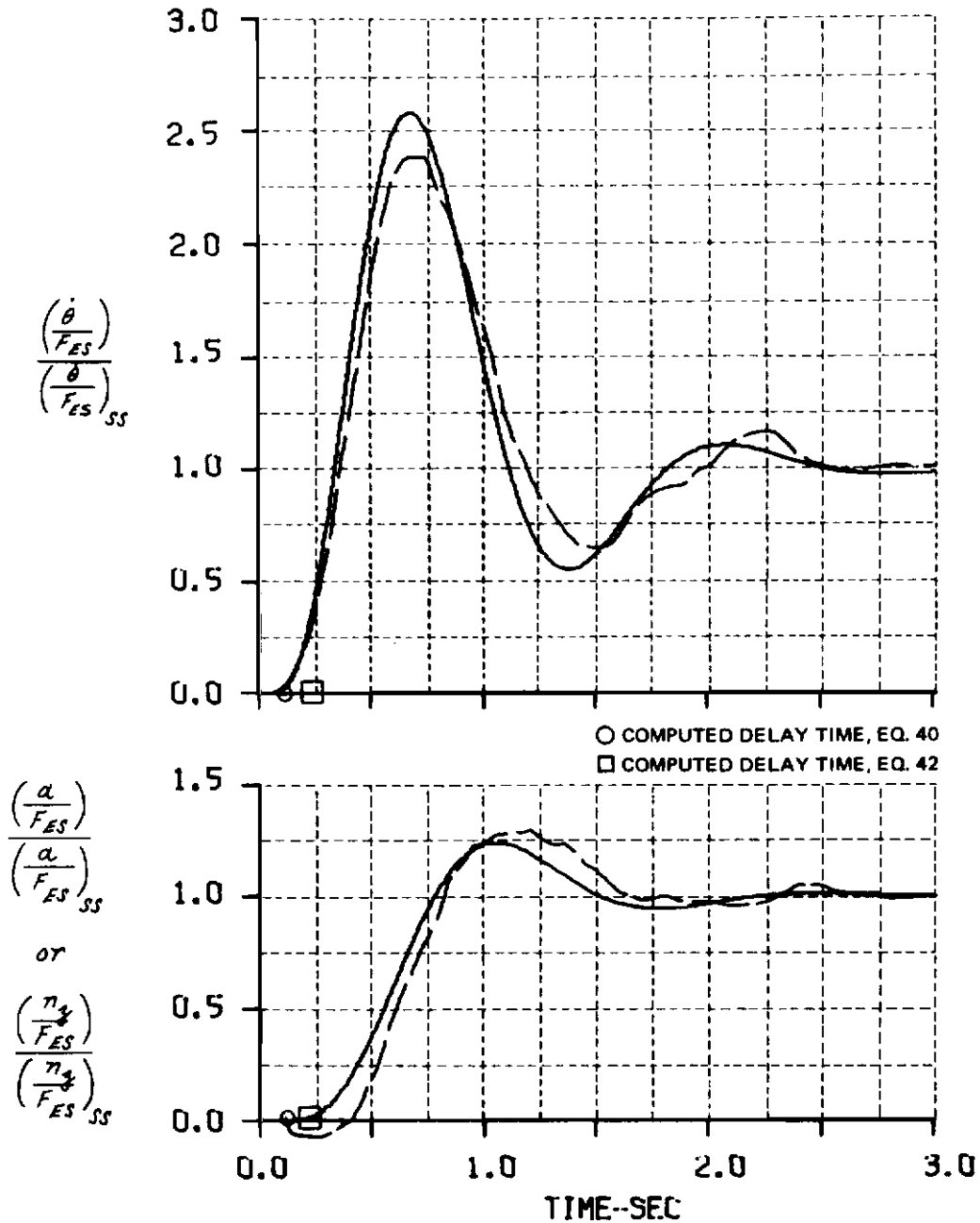
Figure A-27 COMPUTED AND MEASURED LONGITUDINAL SHORT PERIOD RESPONSES FOR A STEP ELEVATOR STICK FORCE INPUT CONF. C(S)-2(10)
