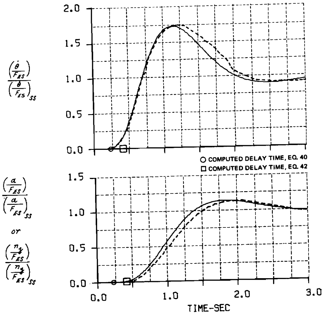
Figure A-12 COMPUTED AND MEASURED LONGITUDINAL SHORT PERIOD RESPONSES FOR A STEP ELEVATOR STICK FORCE INPUT CONF. A(S)-4(2.5)
