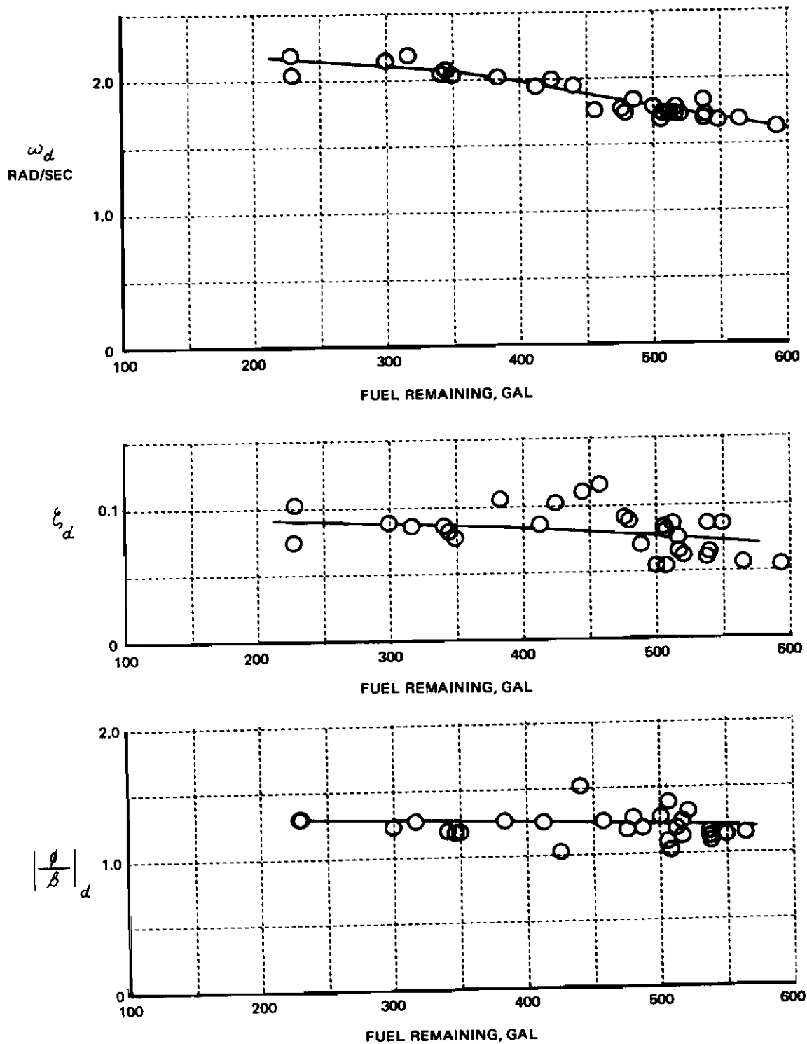
Figure 8 IN-FLIGHT MEASUREMENTS OF LATERAL-DIRECTIONAL MODE CHARACTERISTICS SIMULATED (UP-AND-AWAY FLIGHT CONDITION)
