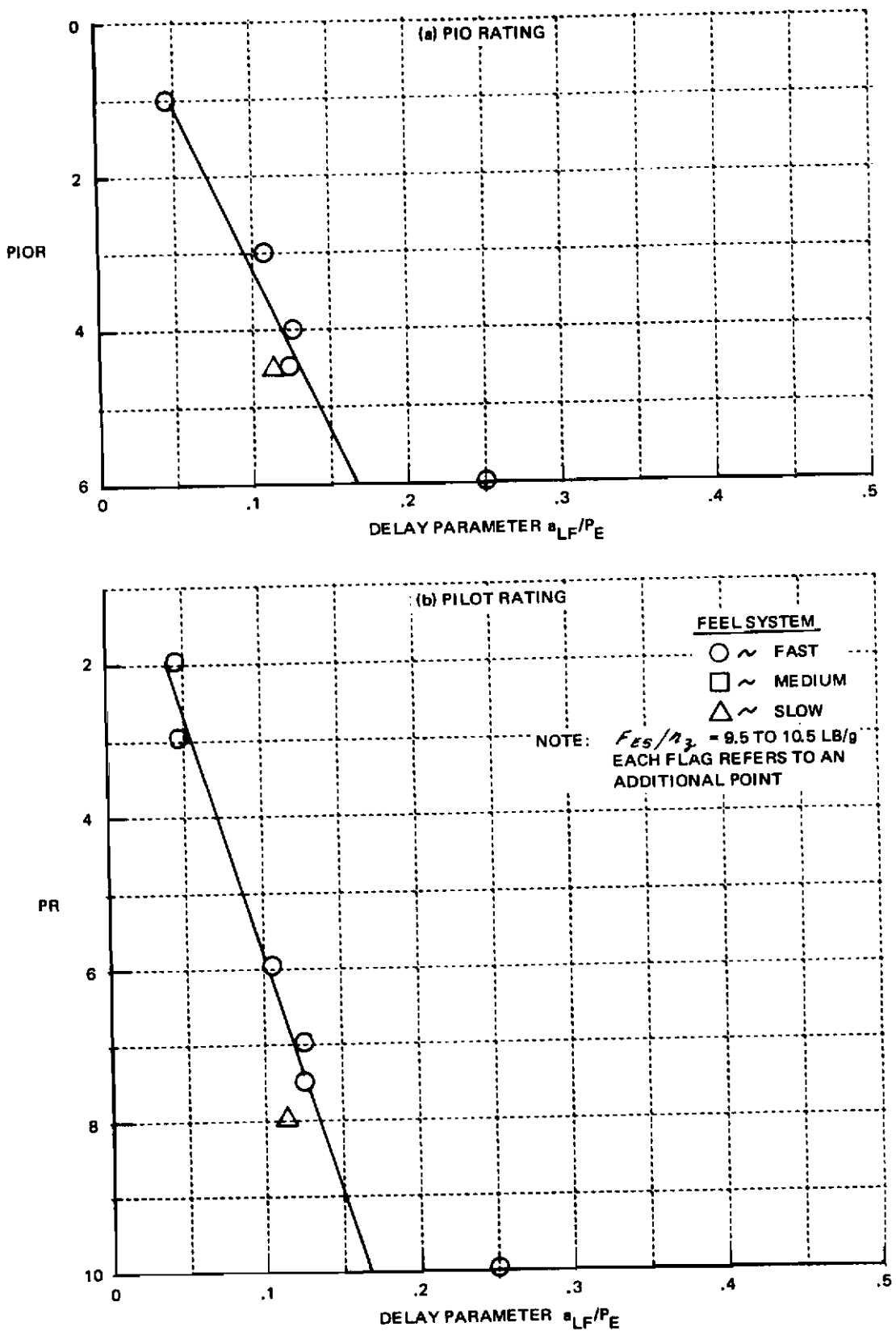
Figure 23 VARIATION OF PILOT RATING AND PIO RATING WITH DELAY PARAMETER (PILOT H - AIRPLANE CONF. B)
