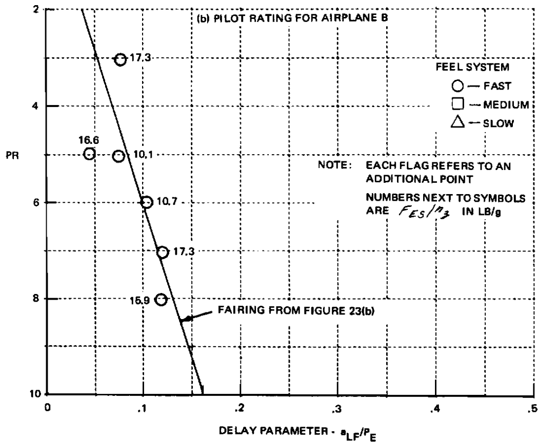
Figure 26 VARIATION OF PILOT RATING WITH DELAY PARAMETER (PILOT B - AIRPLANE CONF. A AND B)
