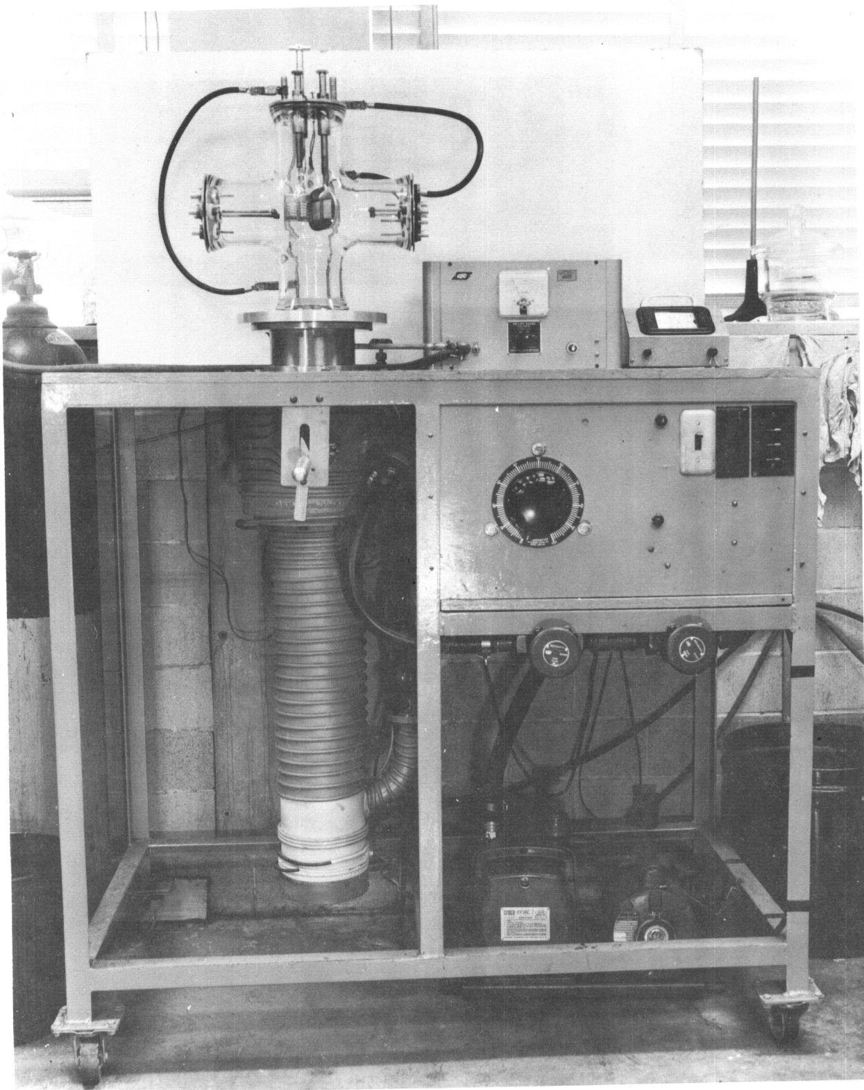
Figure 2 Vacuum System for Depositing Thin Reflective Films
