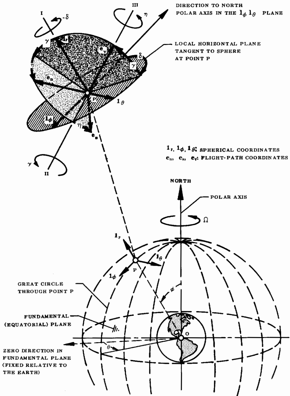
FIGURE 2 ROTATING-EARTH COORDINATE SYSTEM
