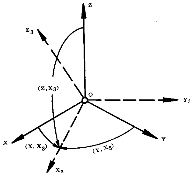
FIGURE 13 GENERAL ROTATION ABOUT ORIGIN — DIRECTION-COSINE DESCRIPTION OF ROTATION (DIRECTION ANGLES FOR X_3 AXIS)
