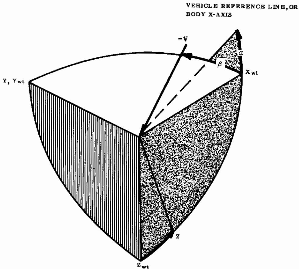
FIGURE 9 WIND-TUNNEL STABILITY AXES
