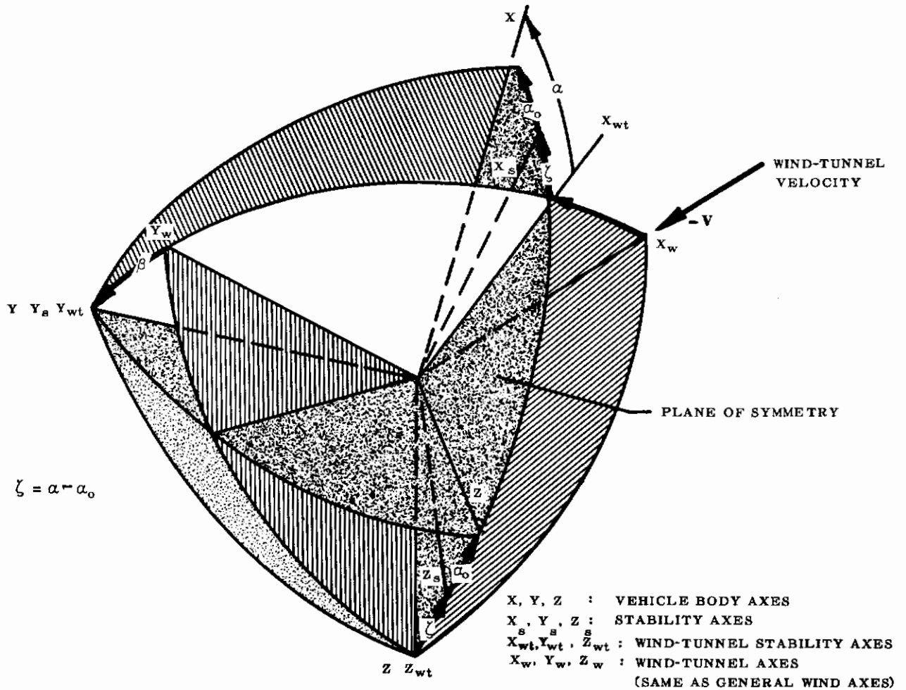
FIGURE 18 ROTATION FROM WIND-TUNNEL TO VEHICLE AXES—YAW-PITCH SEQUENCE
