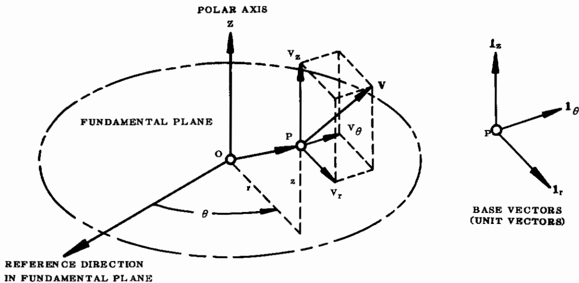
FIGURE 3 CYLINDRICAL-COORDINATE SYSTEM
