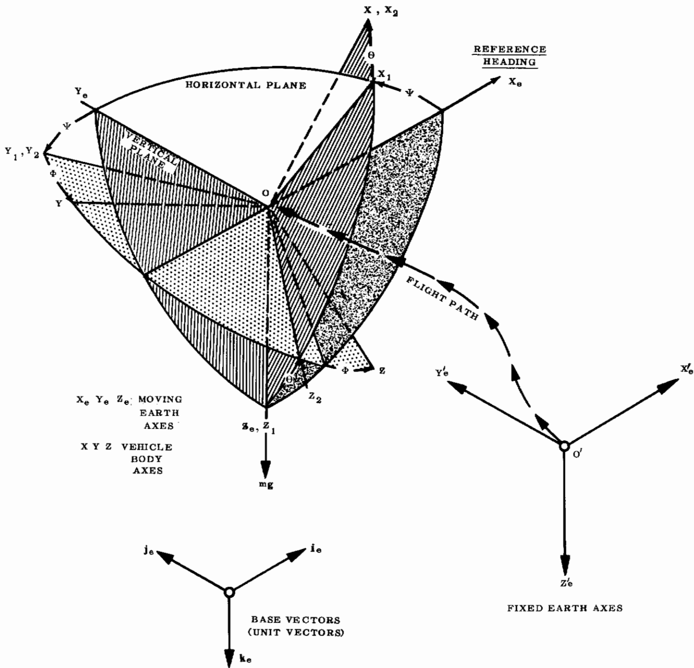
FIGURE 4 RELATIONSHIPS BETWEEN MOVING AND FIXED EARTH AXES, AND VEHICLE BODY AXES
