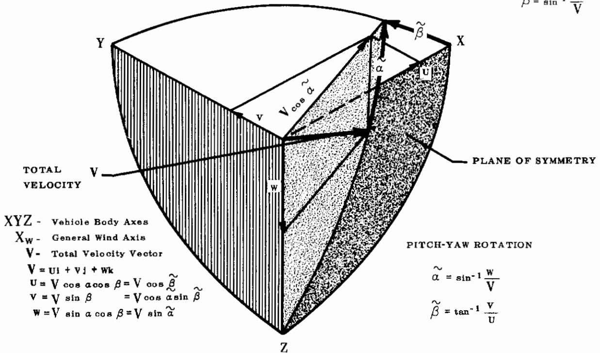
FIGURE 22 ANGLES OF ATTACK AND SIDESLIP
