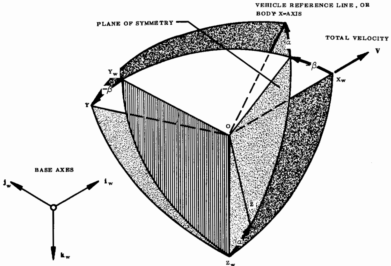
FIGURE 8 GENERAL WIND AXES
