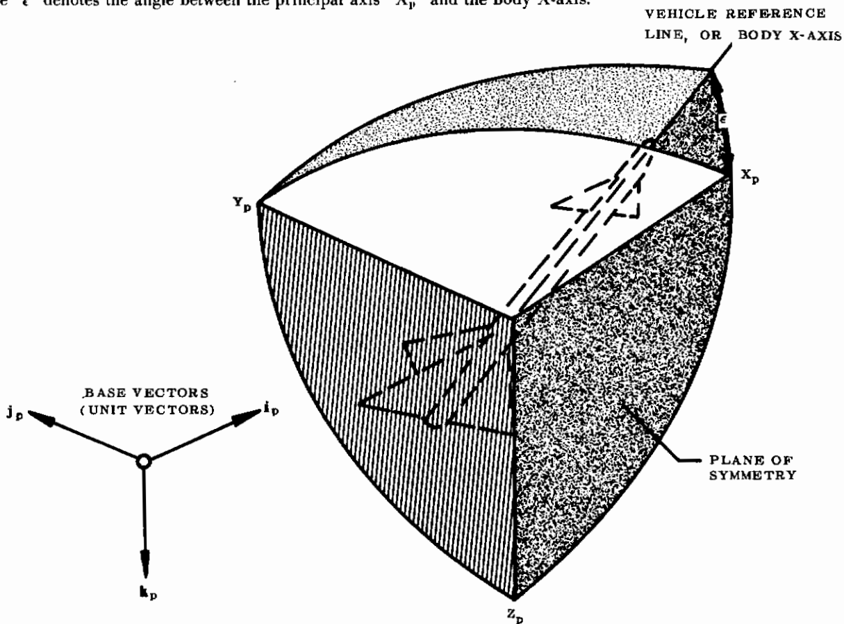
FIGURE 7 PRINCIPAL AXES
