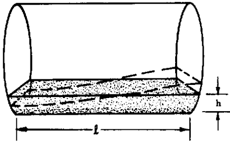
HORIZONTAL CIRCULAR CYLINDRICAL TANK (ref. 40)
