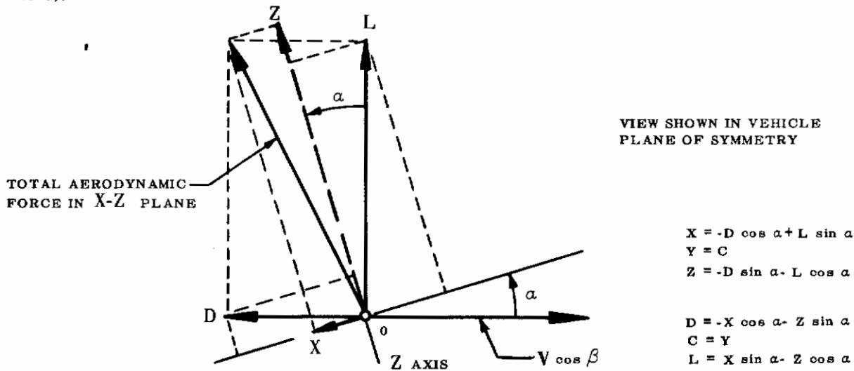
FIGURE 23 AERODYNAMIC-FORCE RESOLUTION
