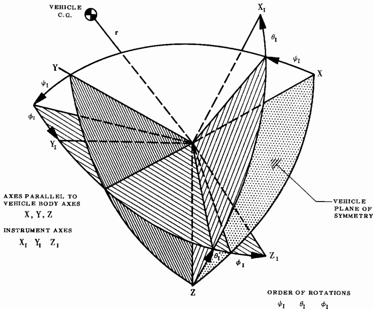
FIGURE 26 GENERAL INSTRUMENT AXES
