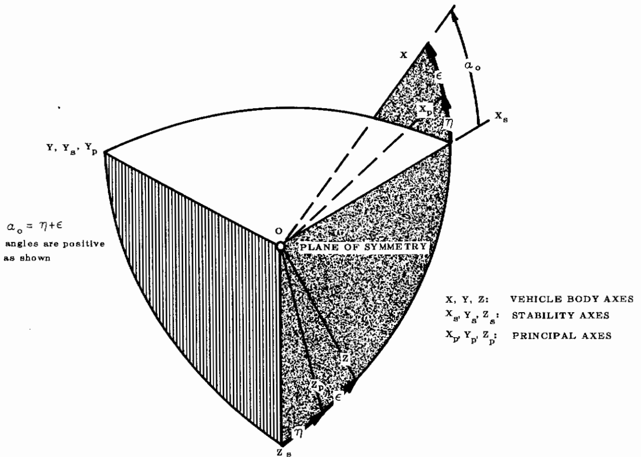
FIGURE 17 BODY - STABILITY - PRINCIPAL AXES ROTATION - PITCH
