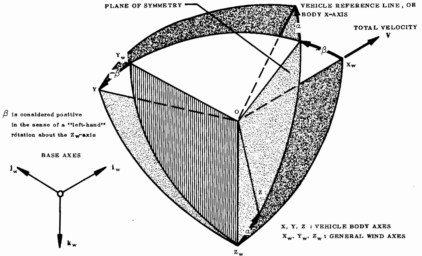
FIGURE 20 ROTATION FROM WIND TO BODY AXES — YAW - PITCH SEQUENCE
