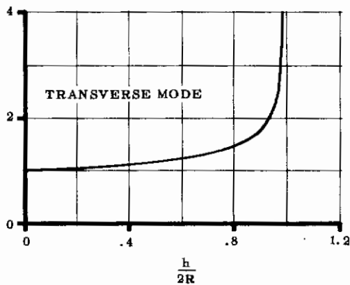
FIGURE 28 NATURAL FREQUENCY OF FUEL-SLOSH FUNDAMENTAL MODE FOR VARIOUS FUEL-TANK SHAPES
