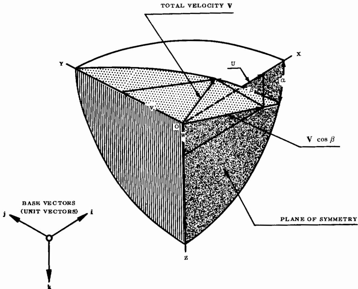
FIGURE 5 VEHICLE BODY AXES
