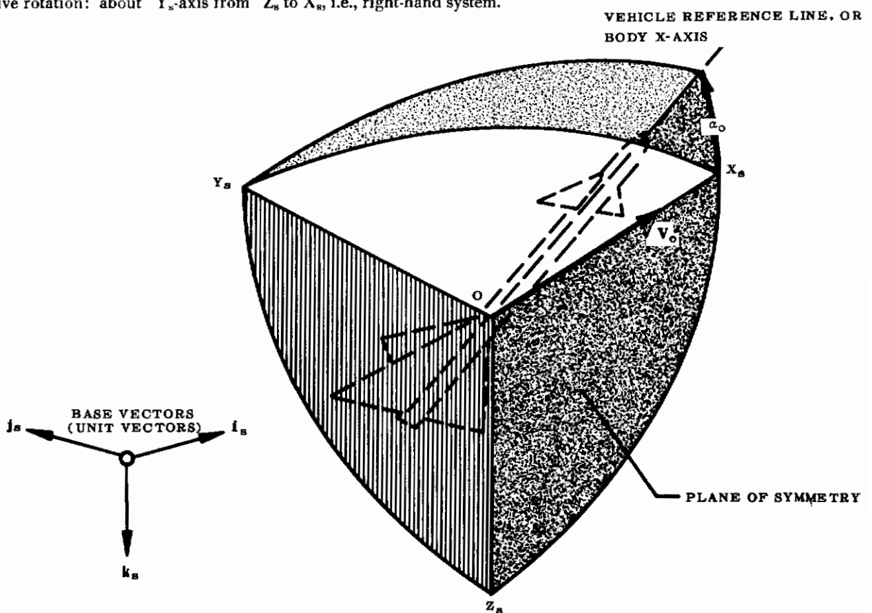
FIGURE 6 STABILITY AXES
