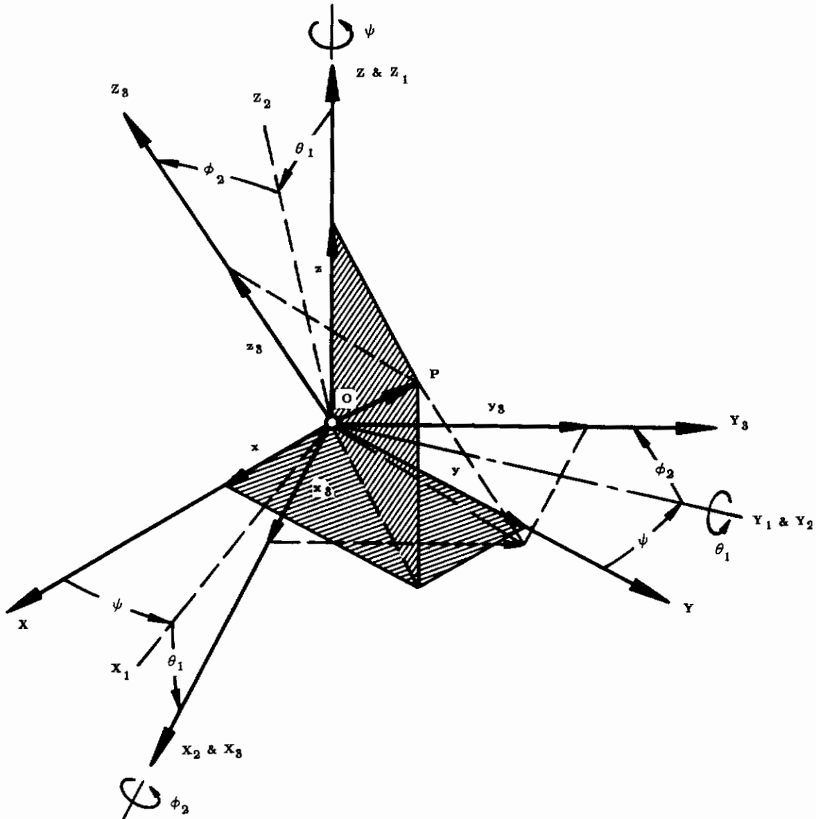
FIGURE 12 GENERAL ROTATION ABOUT ORIGIN — ORIENTATION-ANGLE DESCRIPTION OF ROTATION
