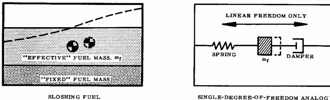
FIGURE 27 SINGLE-DEGREE-OF-FREEDOM ANALOG TO SLOSHING FUEL
