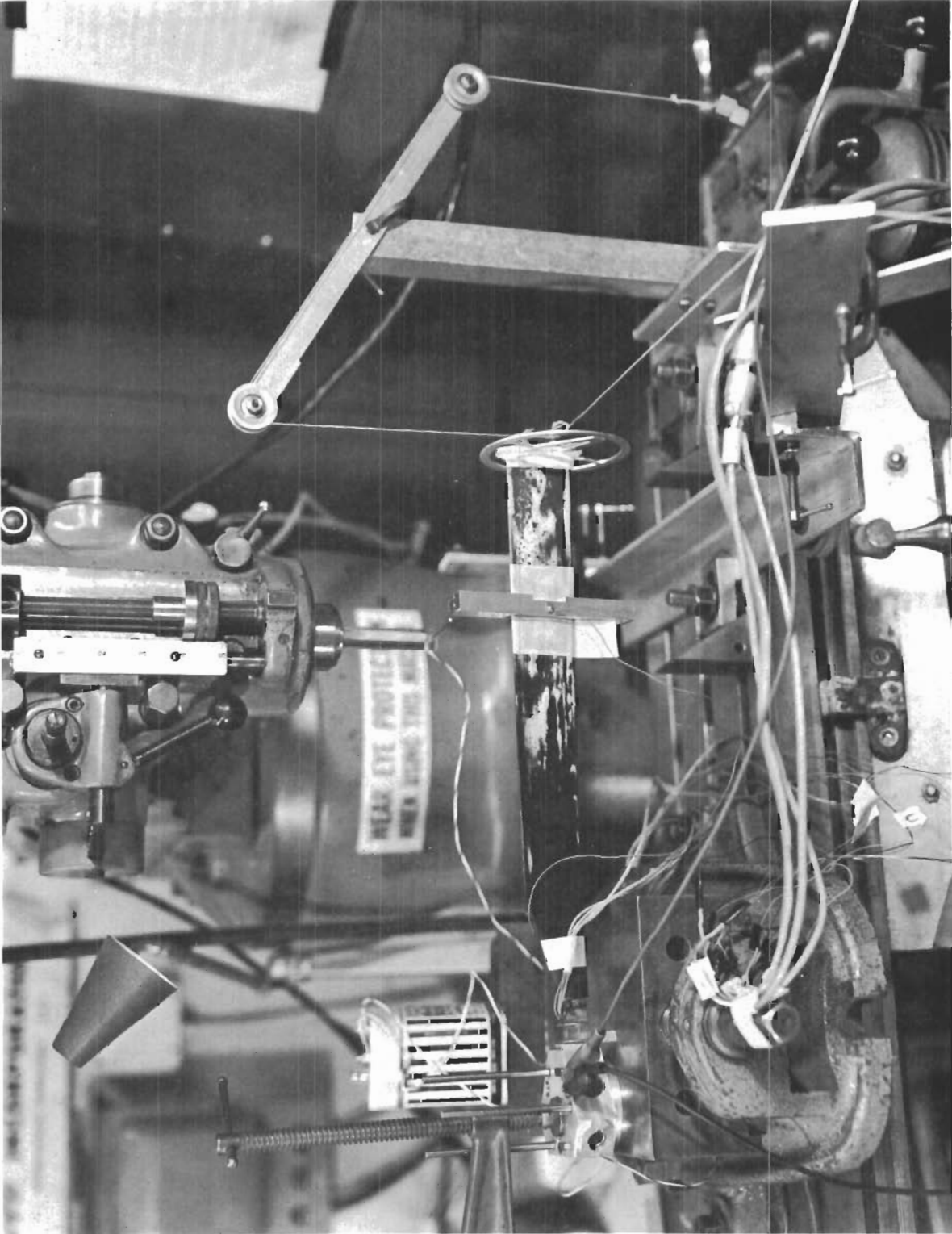
Figure 6. Blade Root and Hub Attachment.
