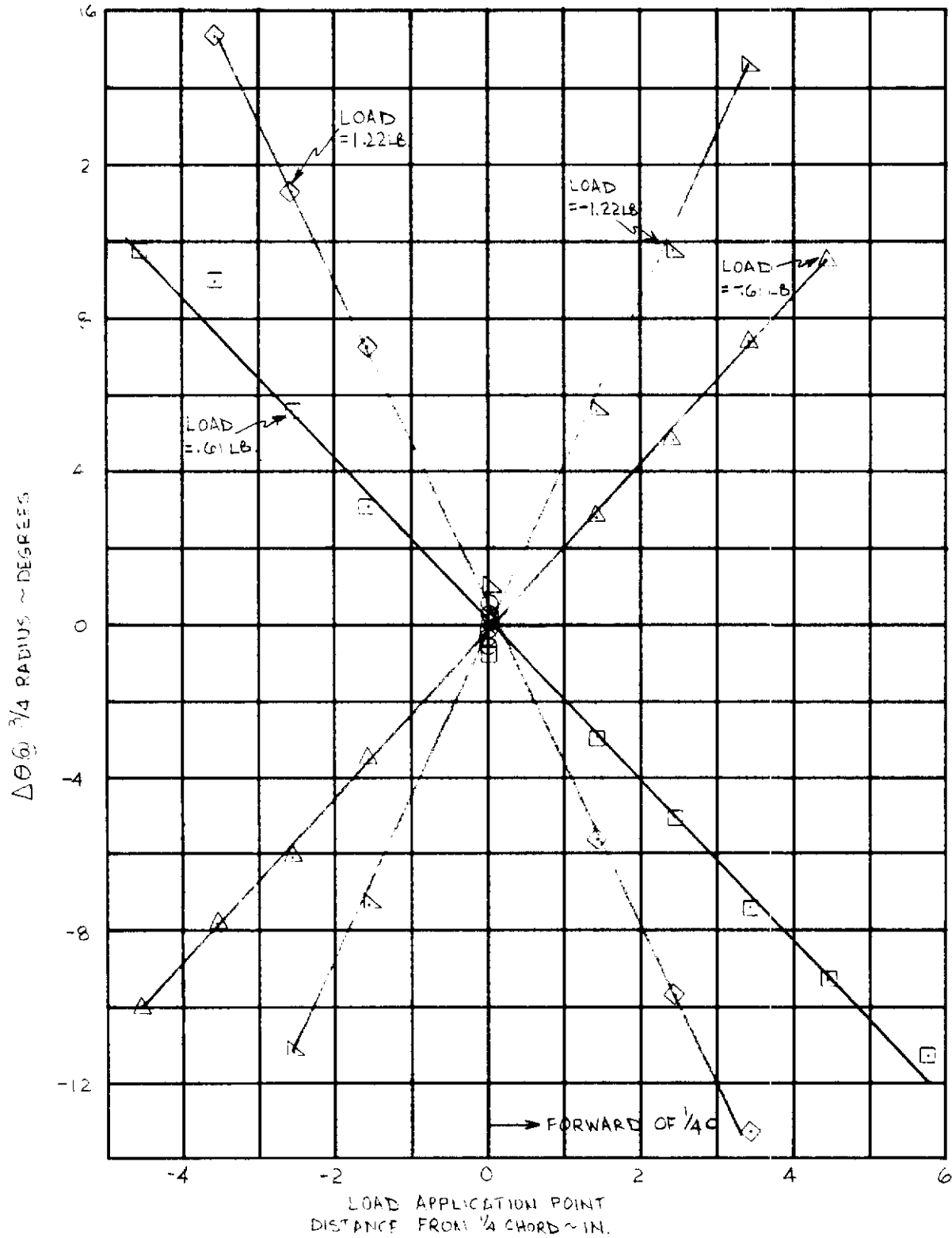
Figure 19. Blade No. 2 (Yellow) Shear Center Determination at 3/4 Radius.
