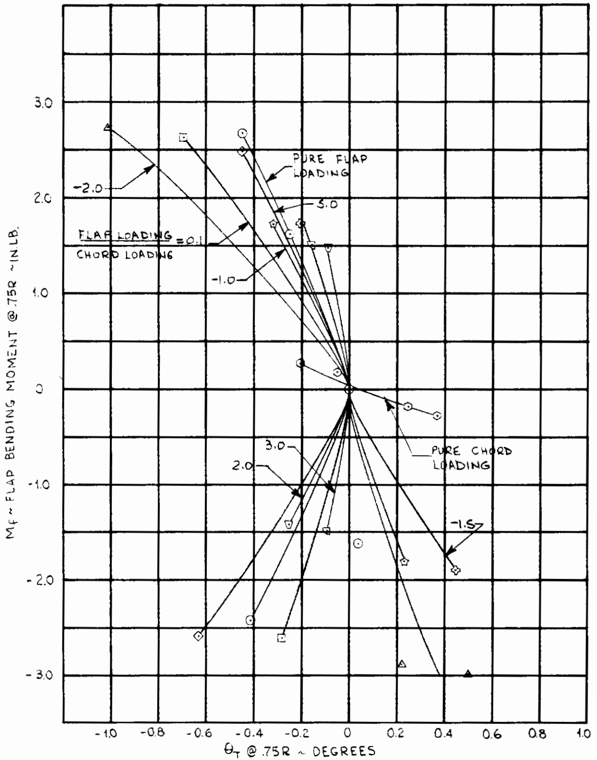
Figure 18. Blade No. 2 (Yellow) Deflection Data.
