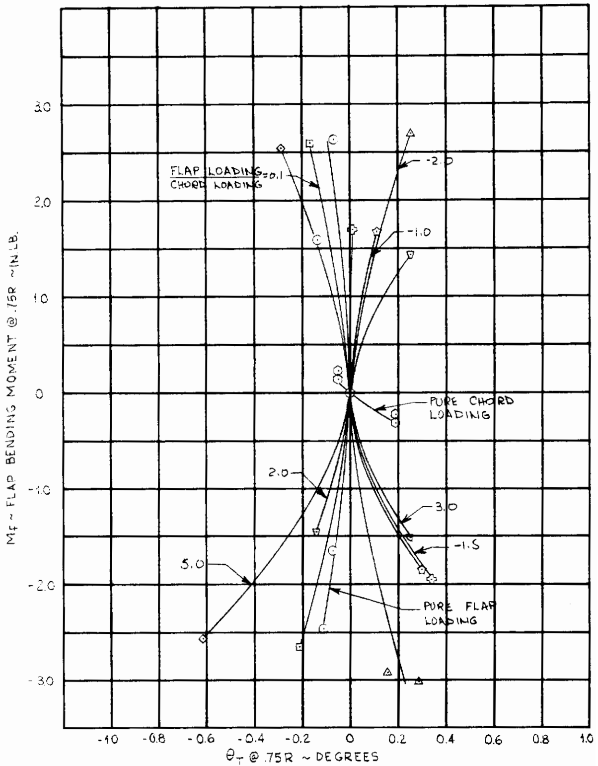
Figure 22. Blade No. 3 (Red) Deflection Data.
