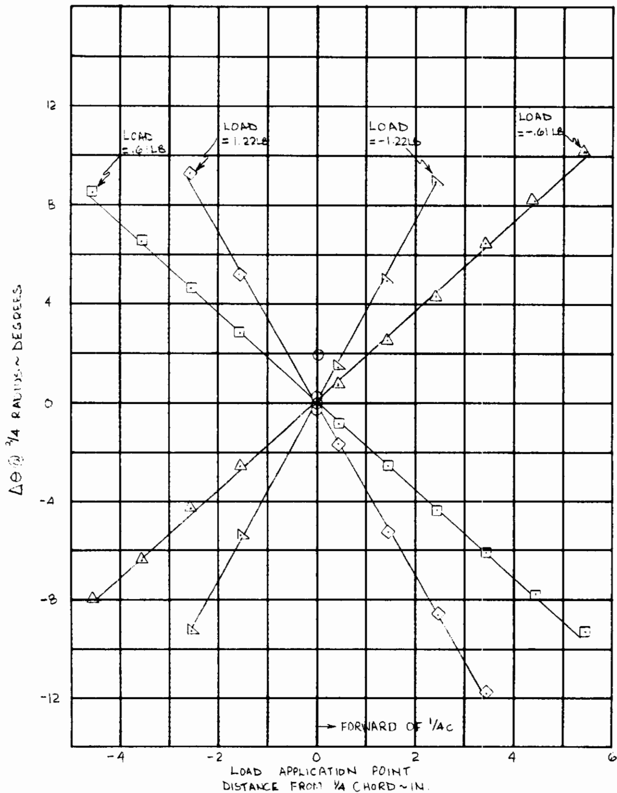
Figure 23. Blade No. 3 (Red) Shear Center Determination at 3/4 Radius.
