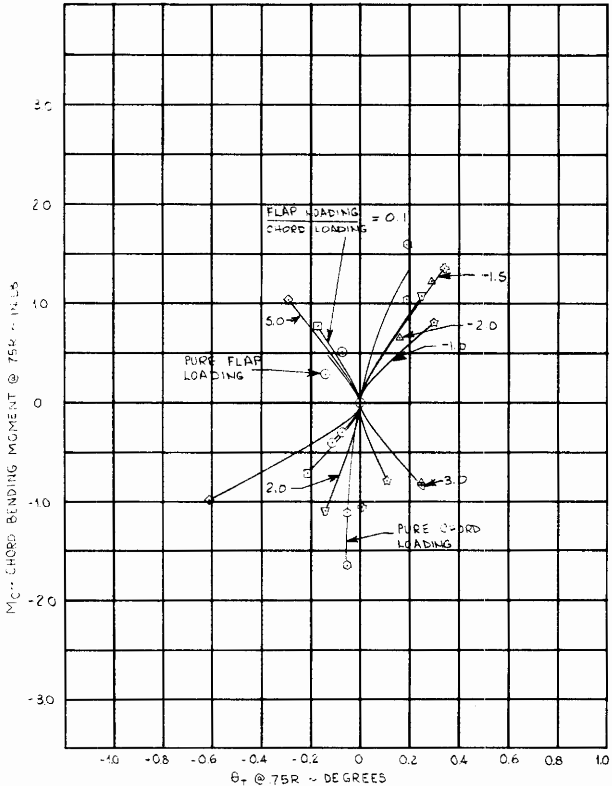
Figure 21. Blade No. 3 (Red) Deflection Data.
