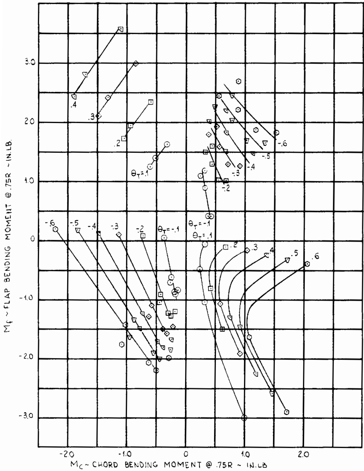
Figure 8. Blade No. 4 (Green) Deflection Data.
