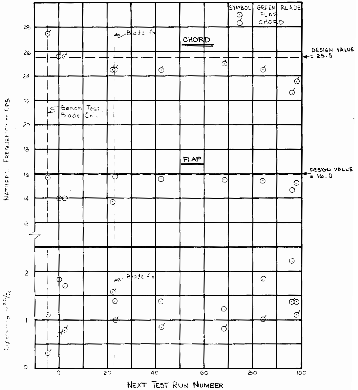
Figure 32. Blade Natural Frequencies and Damping From Static Disturbance Tests of Green Blade.
