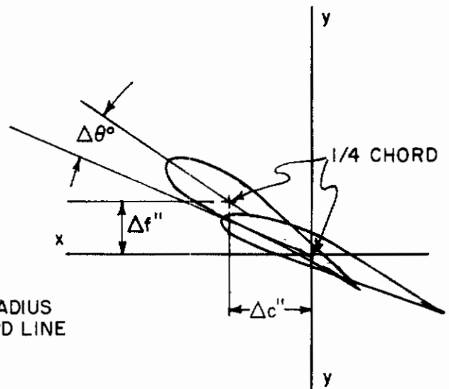
DEFLECTION DIAGRAM
