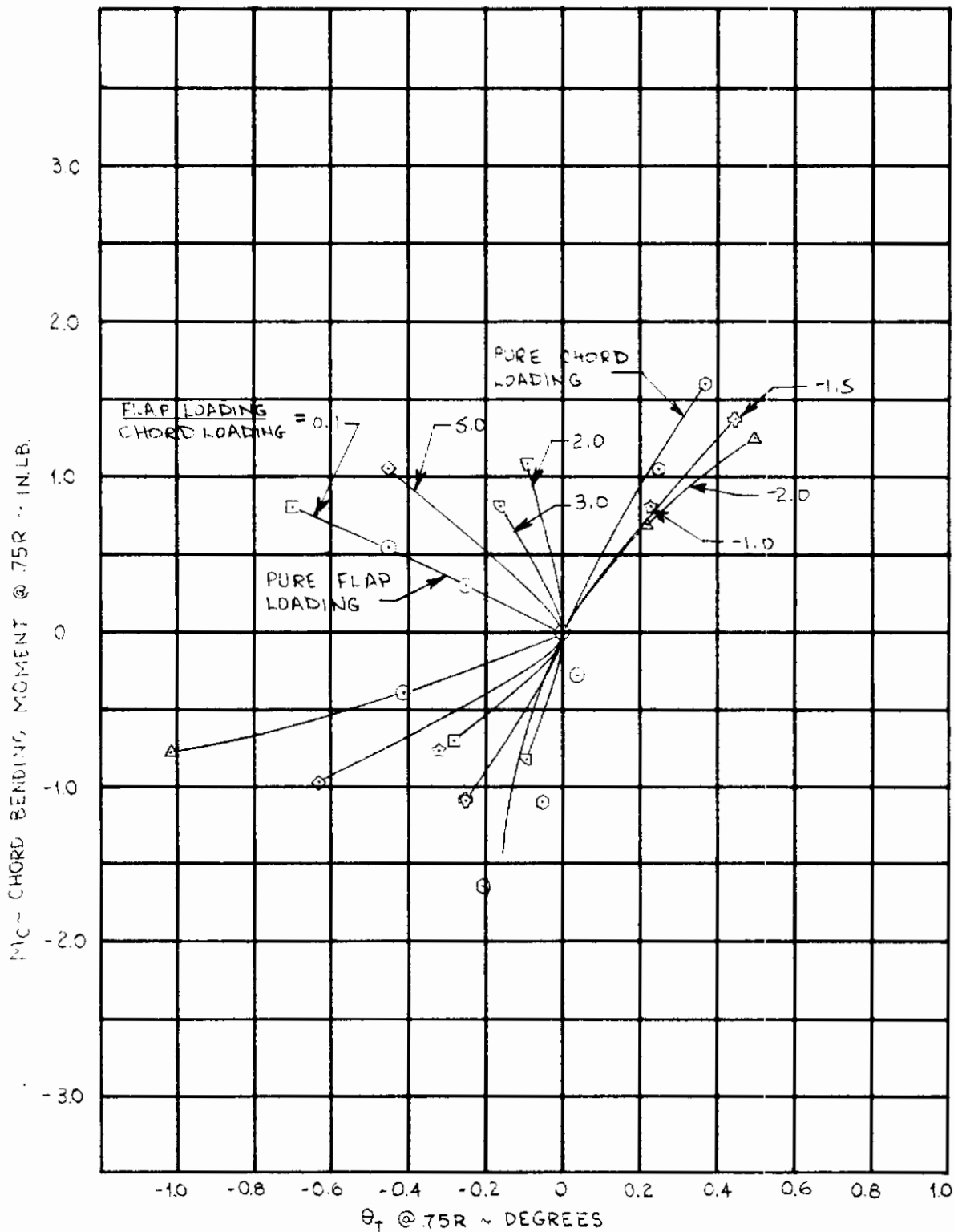
Figure 17. Blade No. 2 (Yellow) Deflection Data.
