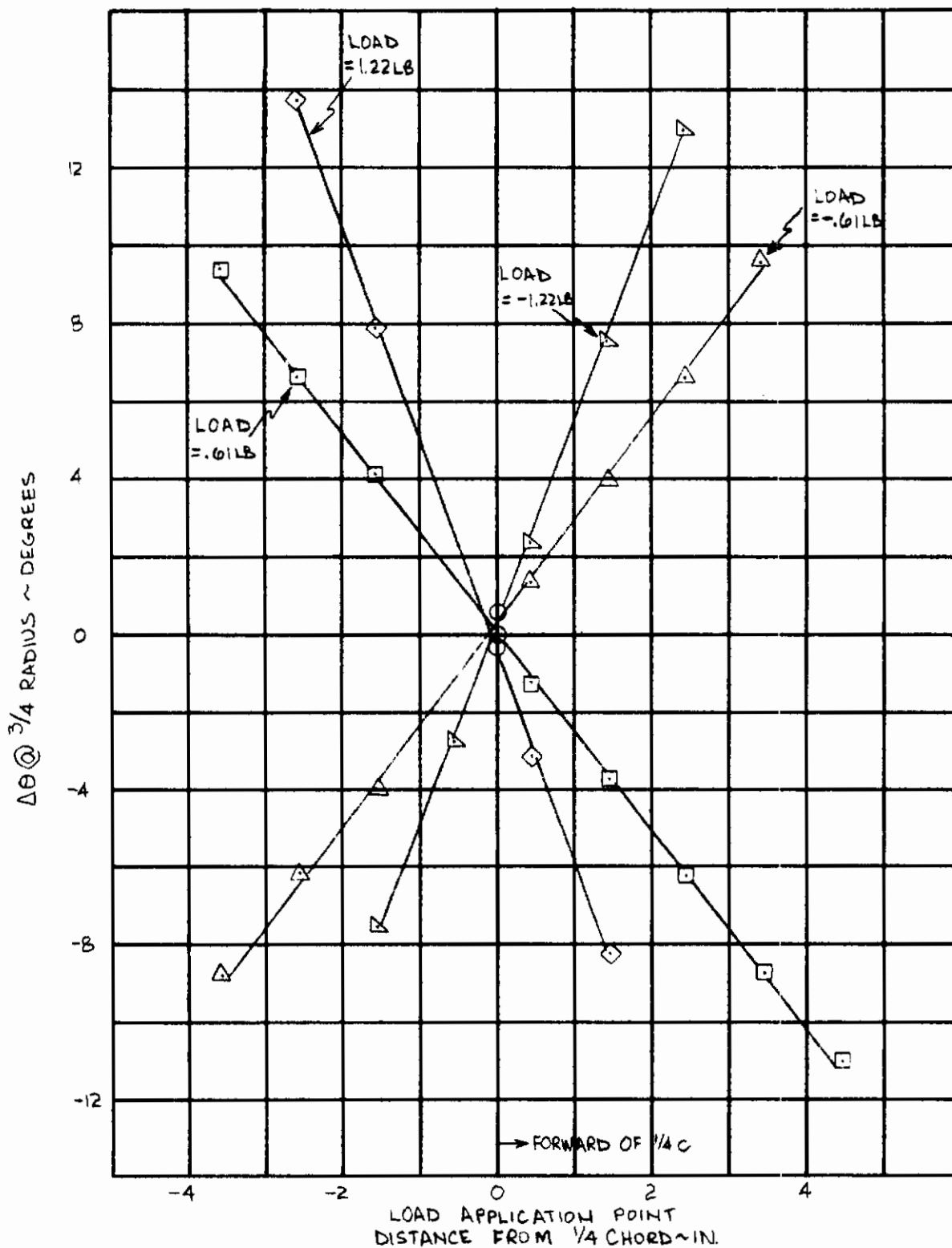
Figure 11. Blade No. 4 (Green) Shear Center Determination at 3/4 Radius.
