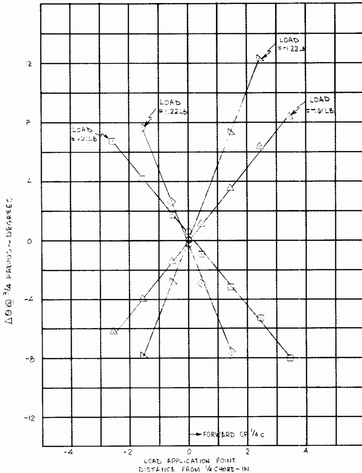
Figure 15. Blade No. 1 (Blue) Shear Center Determination at 3/4 Radius.
