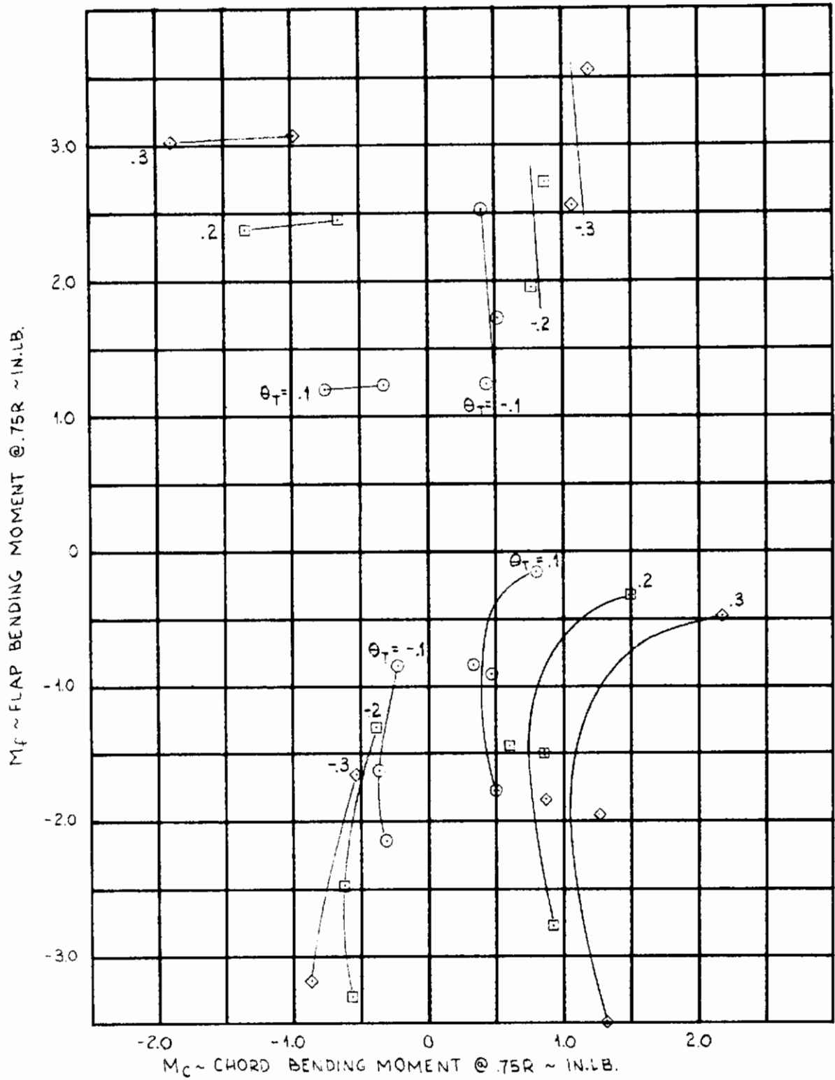
Figure 20. Blade No. 3 (Red) Deflection Data.
