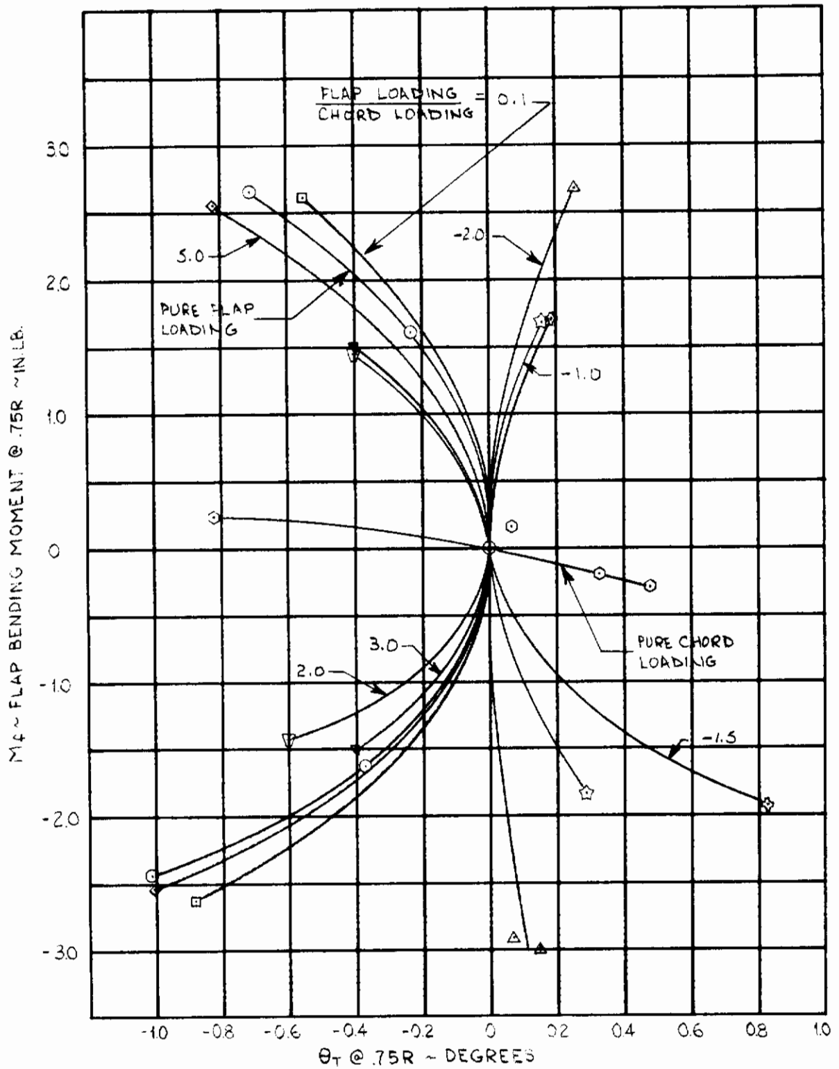
Figure 10. Blade No. 4 (Green) Deflection Data.
