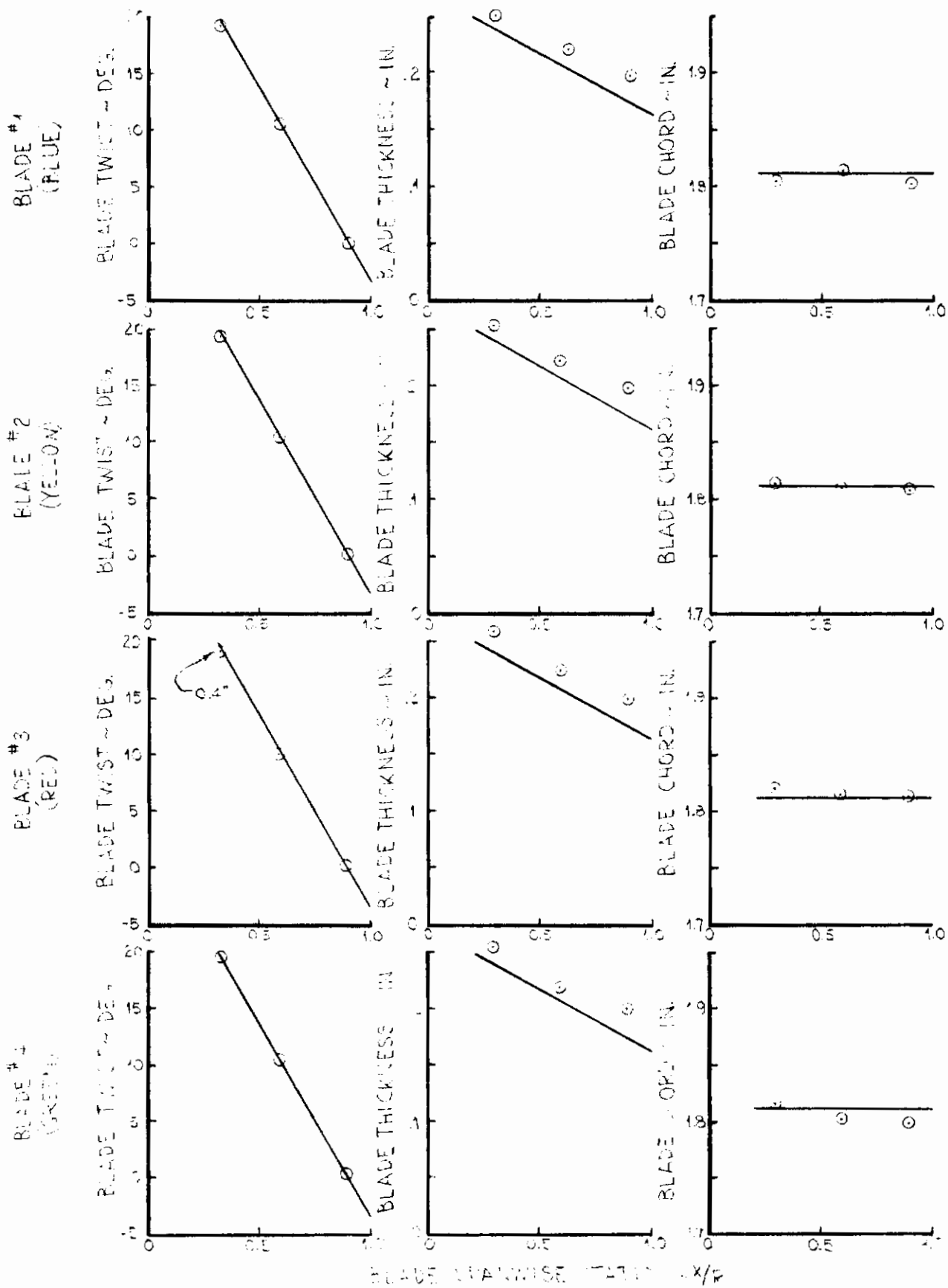
Figure 30. Blade Geometry Inspection Data.
