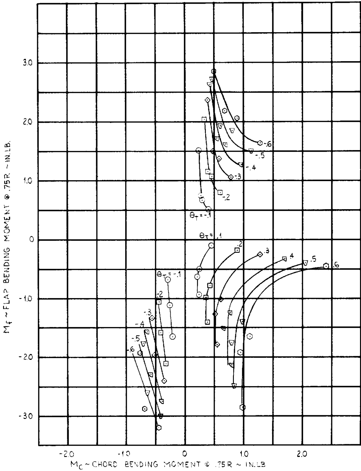
Figure 12. Blade No. 1 (Blue) Deflection Data.
