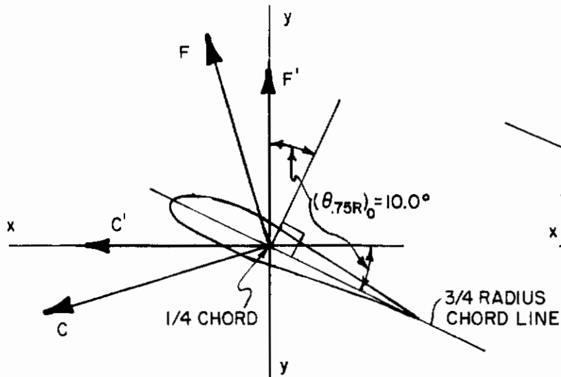
LOADING DIAGRAM
