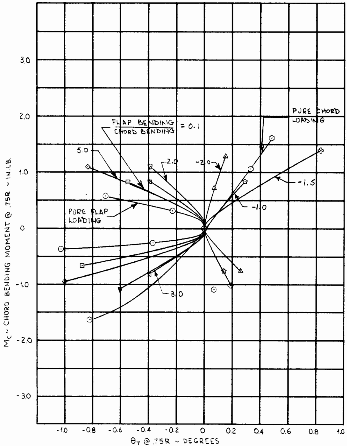
Figure 9. Blade No. 4 (Green) Deflection Data.
