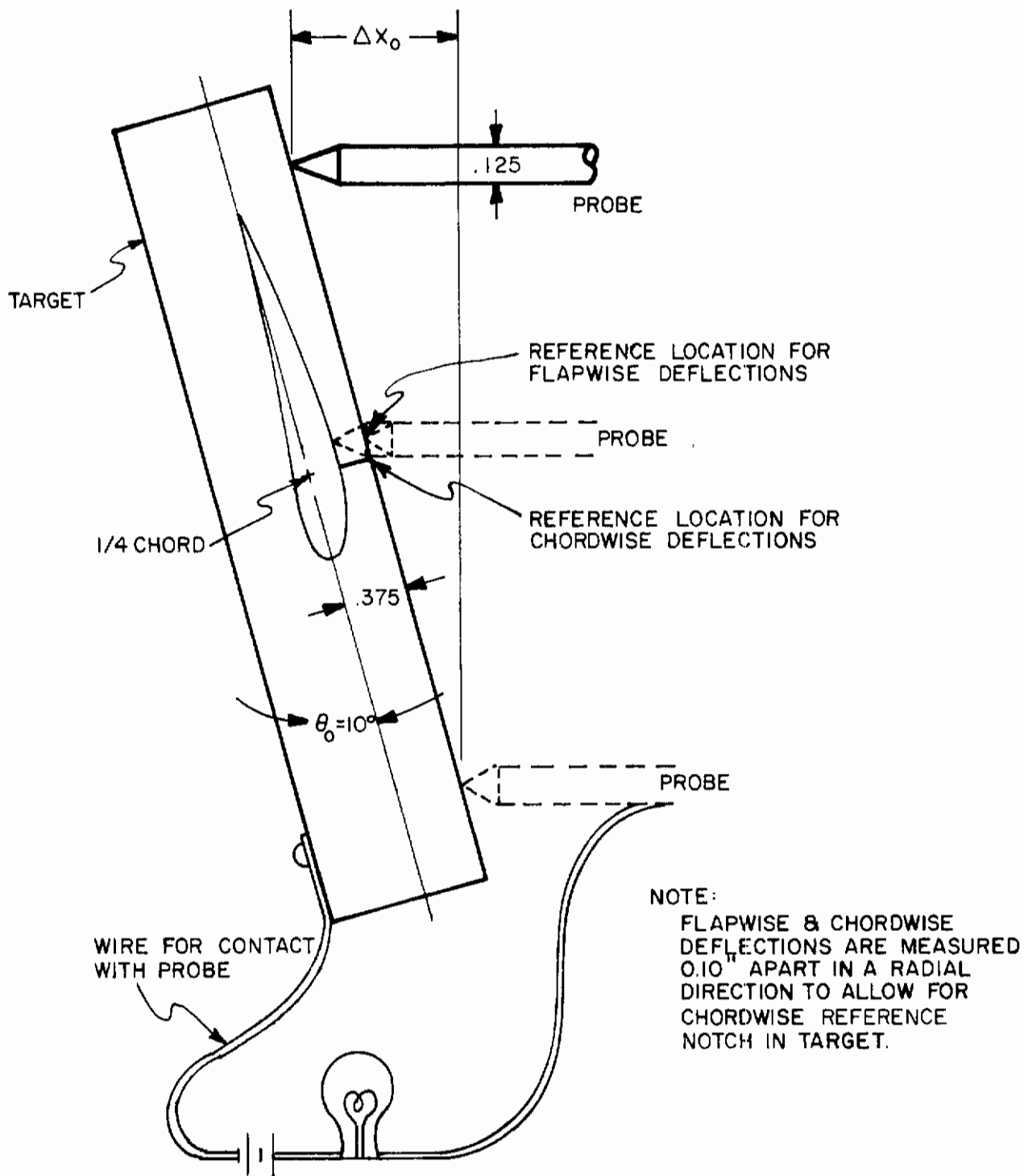
Figure 7. Setup to Obtain Reference Surfaces.
