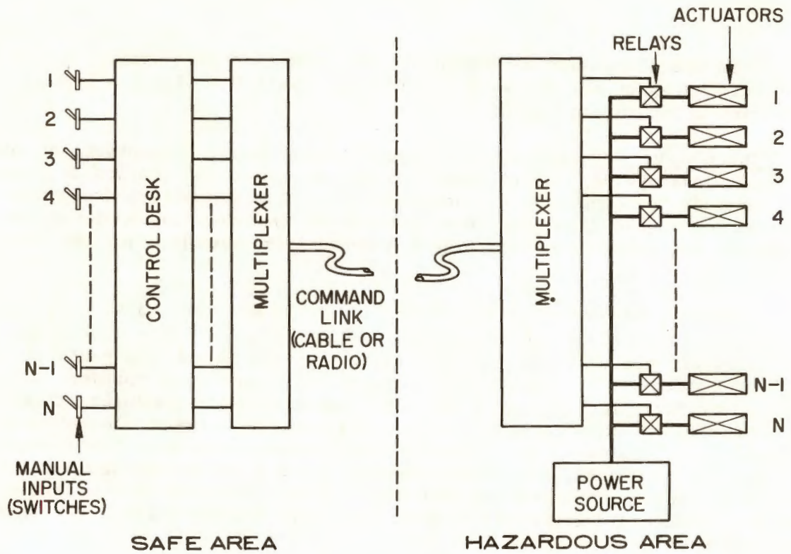
Figure 8. Command System Analysis
