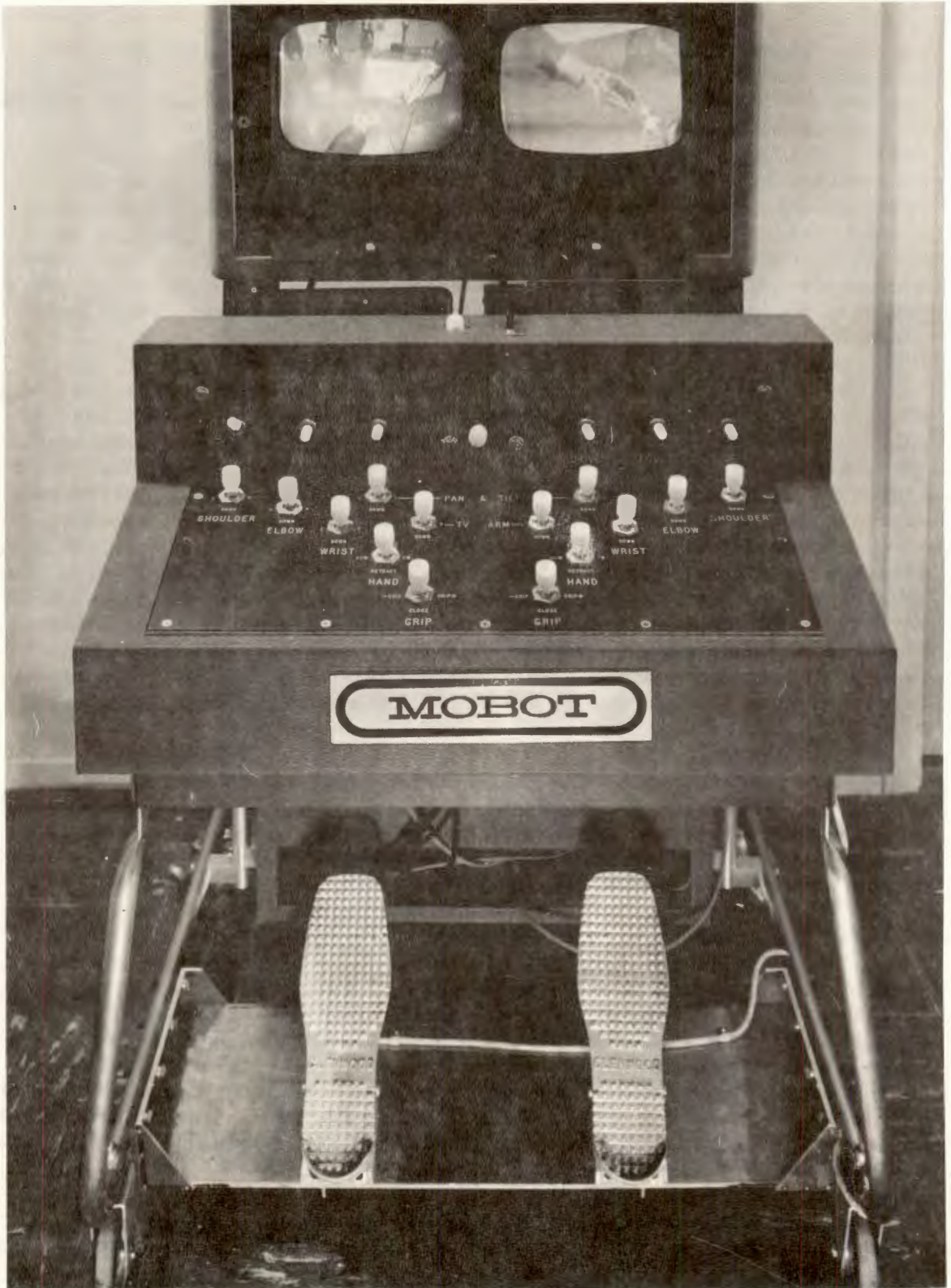
Figure 10. Mark II Control Console
