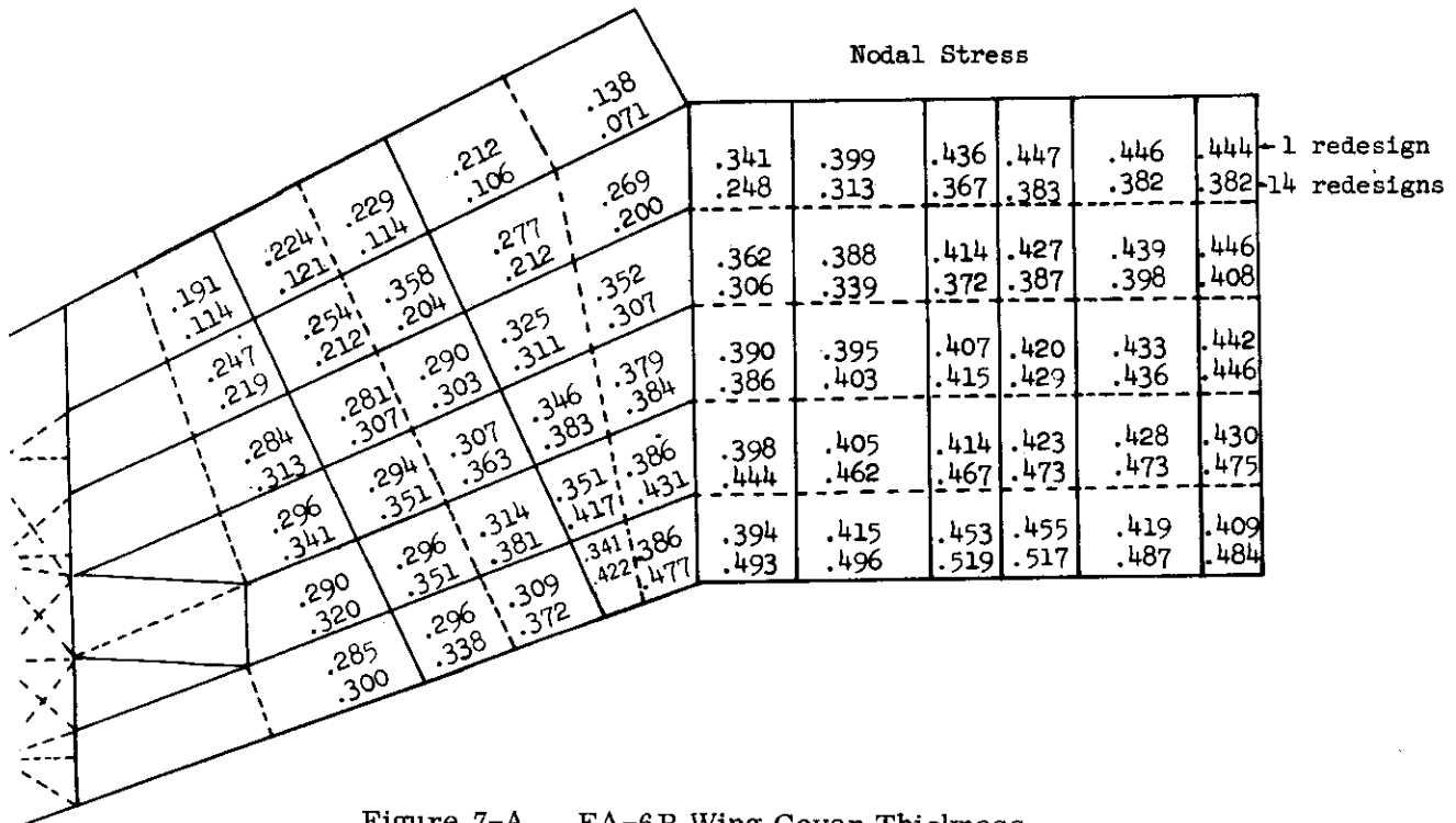
Figure 7-A. EA-6B Wing Cover Thickness
