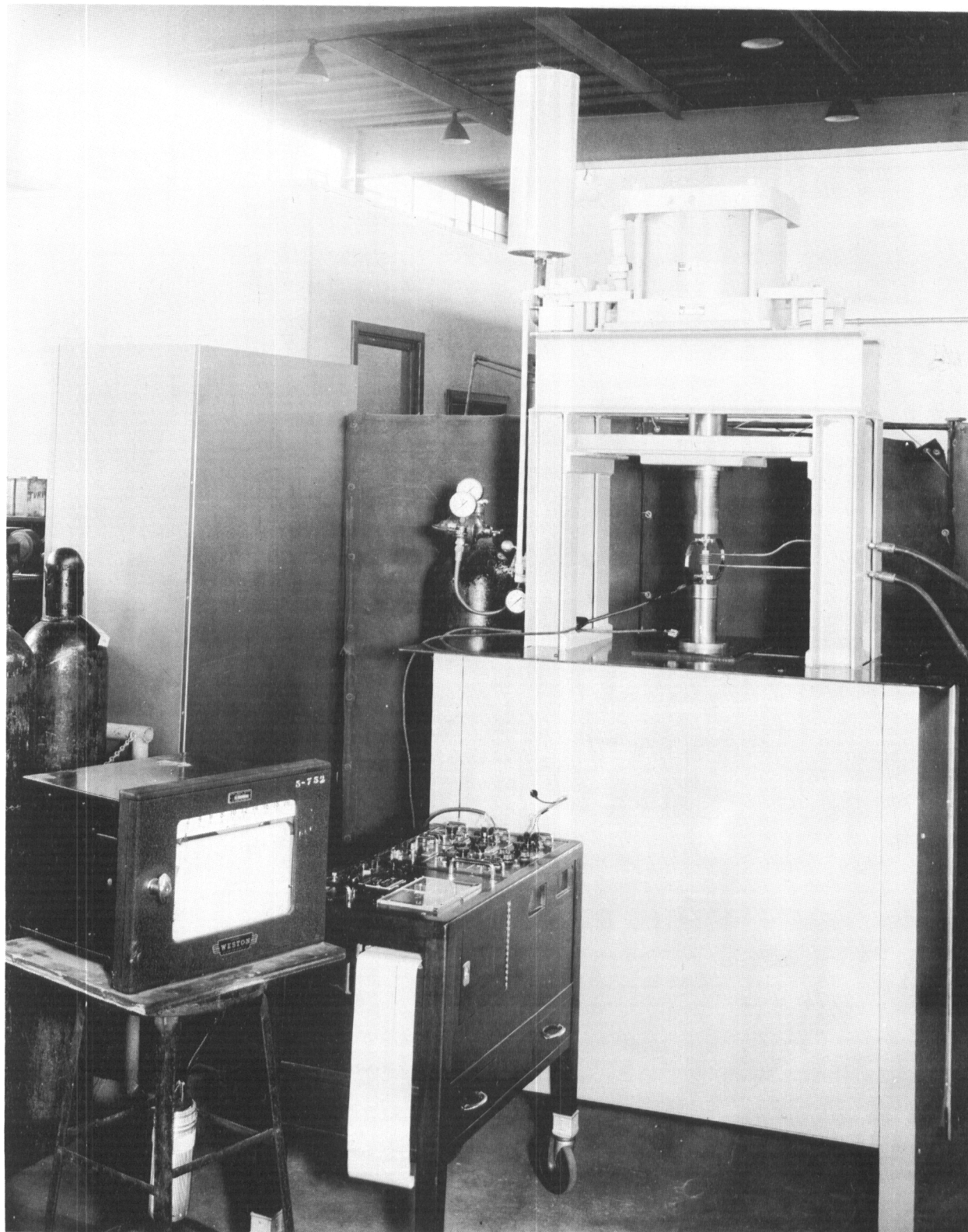
FIGURE 1. HOT-TENSION MACHINE AND AUXILIARY EQUIPMENT
