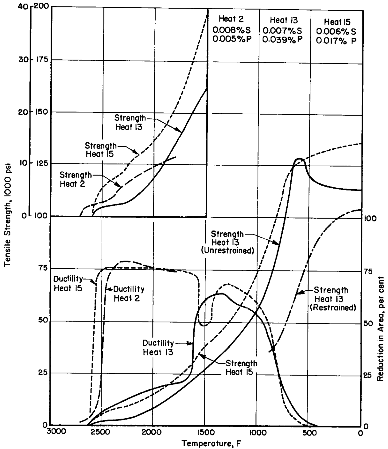
FIGURE 4. THE EFFECT OF PHOSPHORUS CONTENT ON THE HOT STRENGTH AND HOT DUCTILITY OF SAE 4340 STEEL
