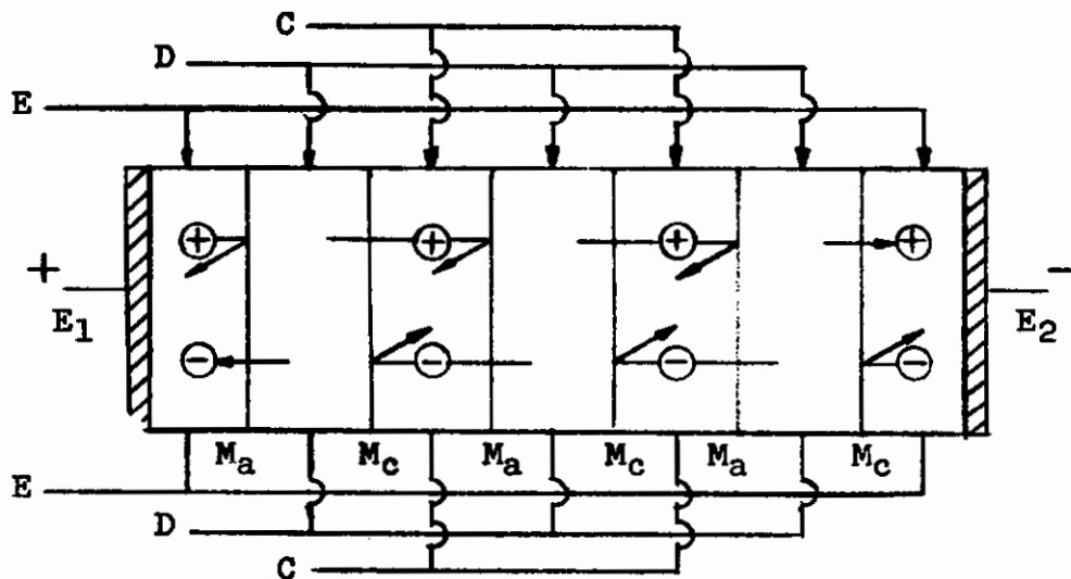
FIGURE 26 SCHEMATIC OF ELECTRODIALYSIS UNIT
