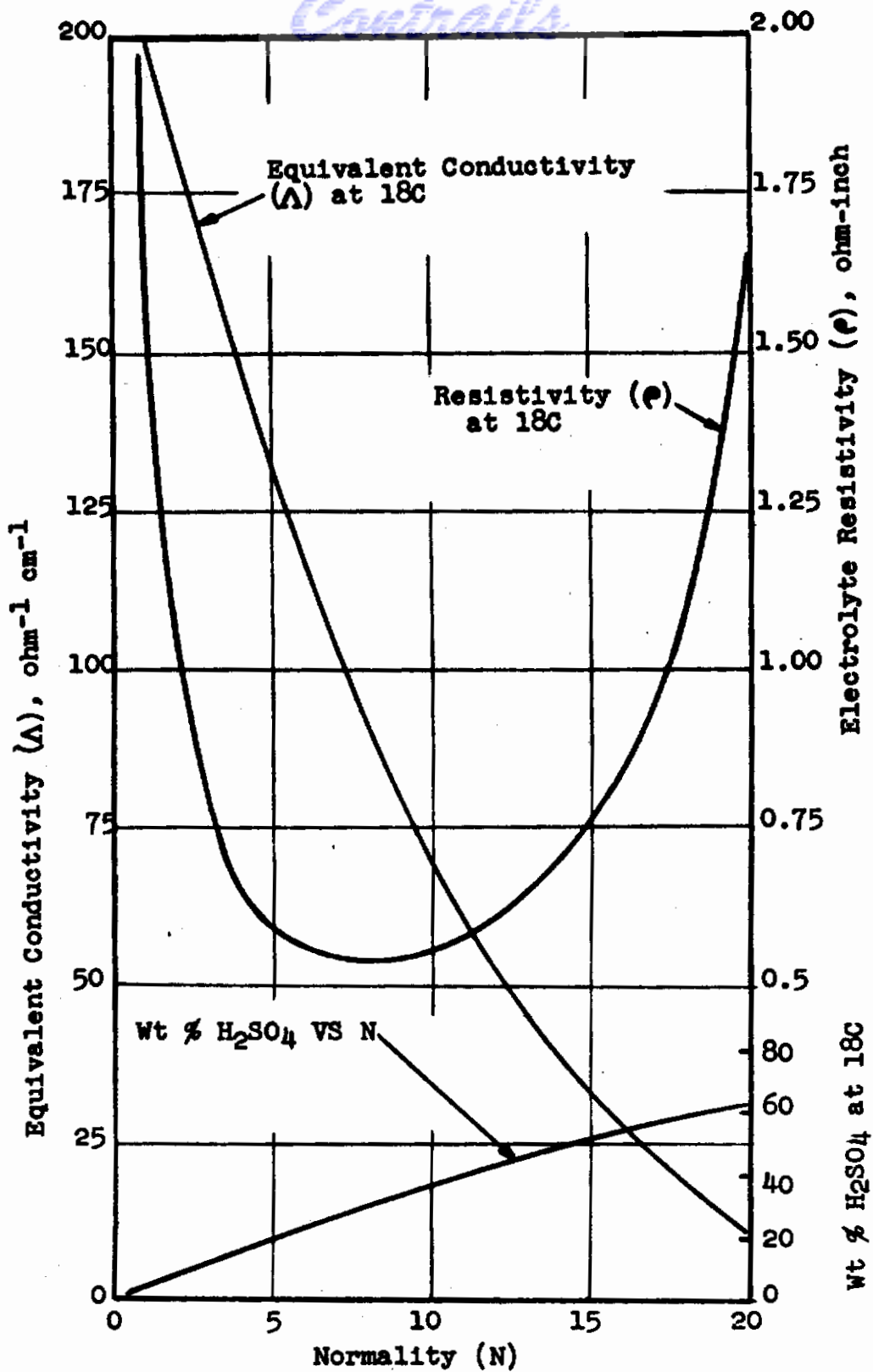
Figure 8 Effect of Electrolyte Concentration on Resistivity
