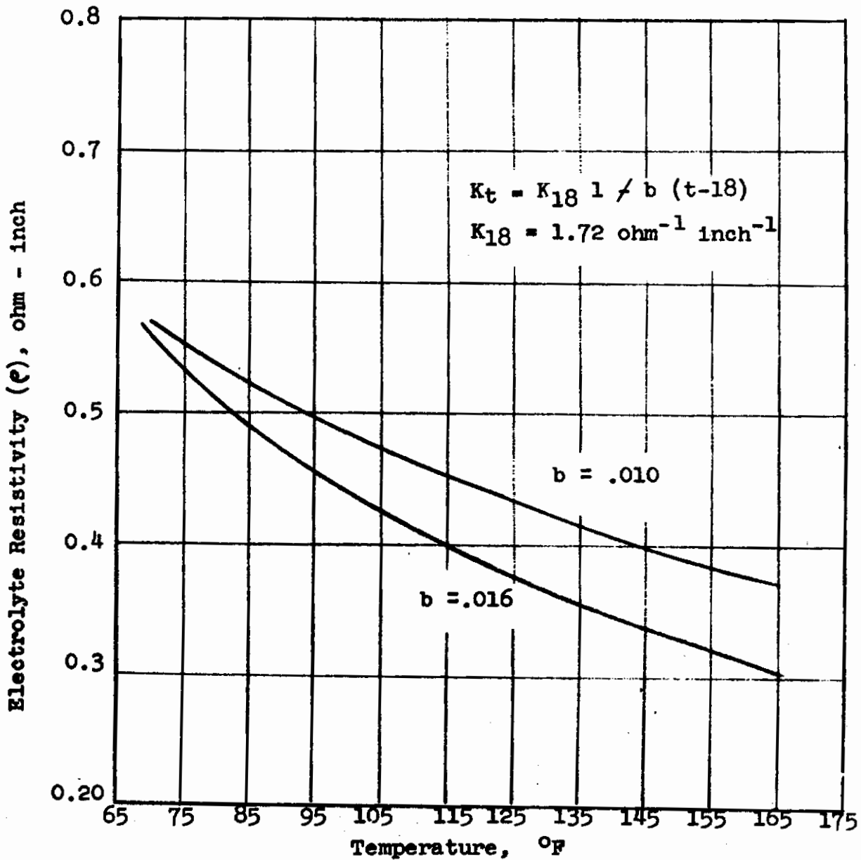
Figure 9 Effect of Temperature on Electrolyte Resistivity for 20 % H 2 SO 4
