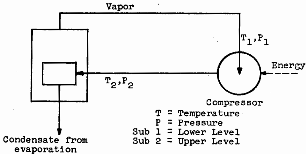
FIGURE 25 Schematic of Vapor Compression System
