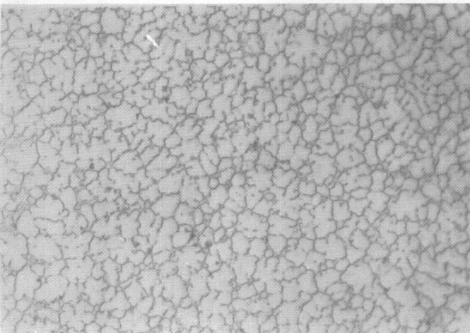
Neg. No. 33915 500X Alloy No. 73448 Etchant: Glycol
