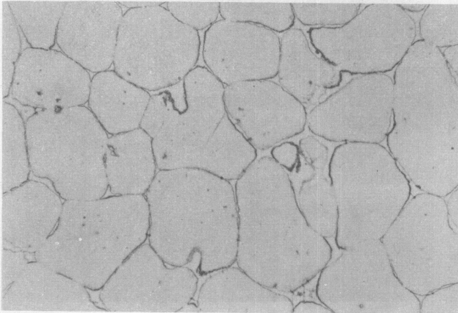
Neg. No. 33171 200X Alloy No. 73445 Etchant: Glycol AC
