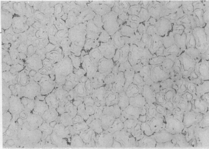
Neg. No. 33210 200X Alloy No. 73457 Etchant: Glycol AC
