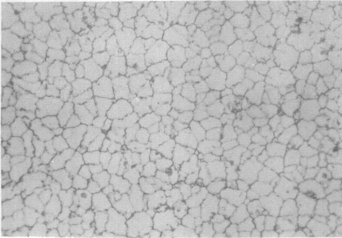
Neg. No. 33918 500X Alloy No. 73844 Etchant: Glycol
