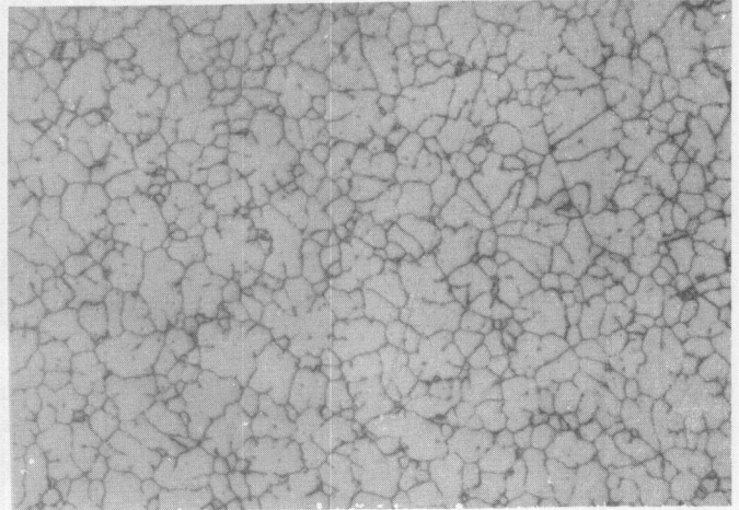
Neg. No. 33914 500X Alloy No. 73586 Etchant: Glycol
