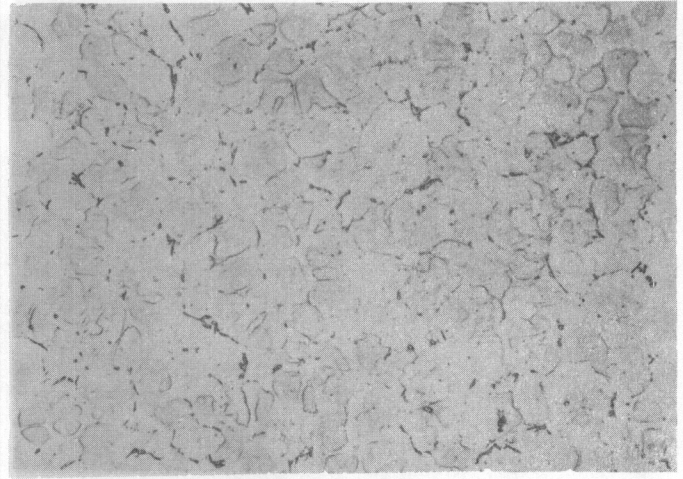
Neg. No. 33211 200X Alloy No. 73457 Etchant: Glycol SHT
