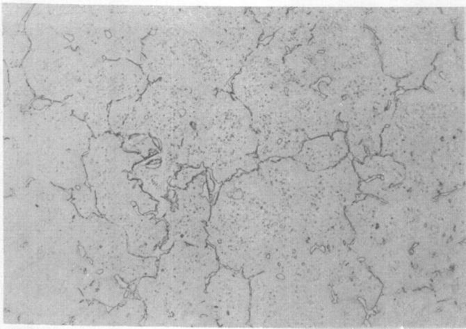
Neg. No. 33177 200X Alloy No. 73447 Etchant: Glycol AC
