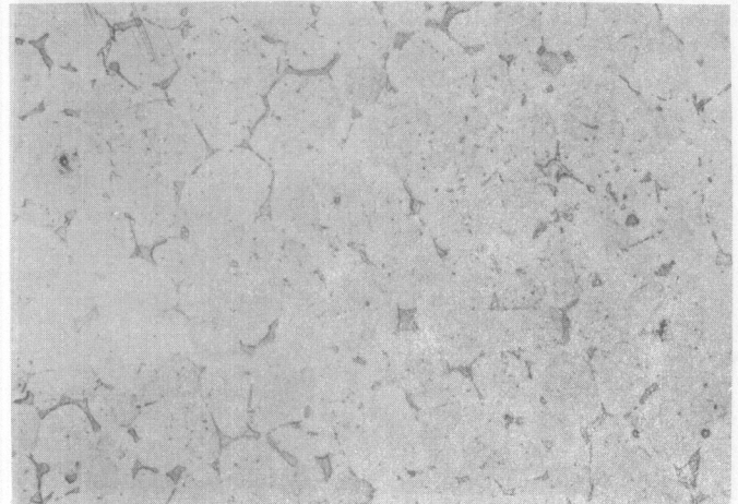
Neg. No. 33203 200X Alloy No. 73453 Etchant: Glycol SHT
