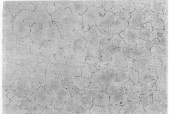
Neg. No. 33205 200X Alloy No. 73454 Etchant: Glycol SHT
