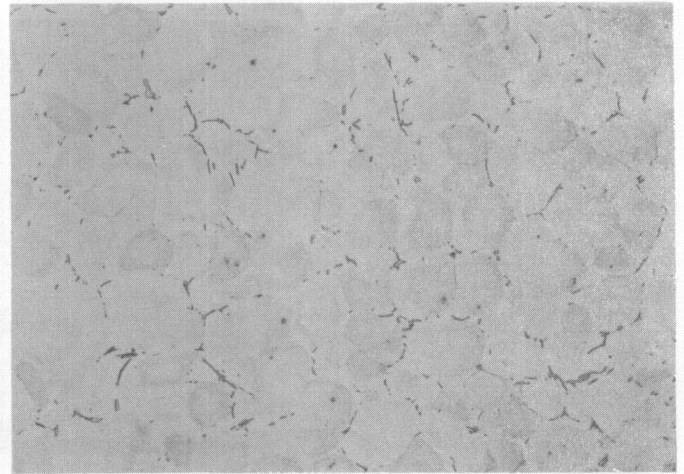
Neg. No. 33213 200X Alloy No. 73458 Etchant: Glycol SHT
