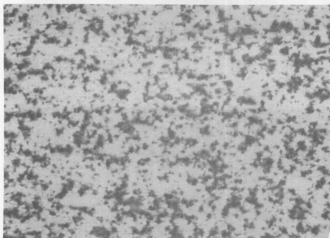
Neg. No. 33221 500X Alloy No. 73448 Etchant: Acetic Picral Ingot
