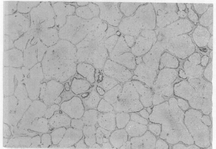
Neg. No. 33174 200X Alloy No. 73446 Etchant: Glycol SHT
