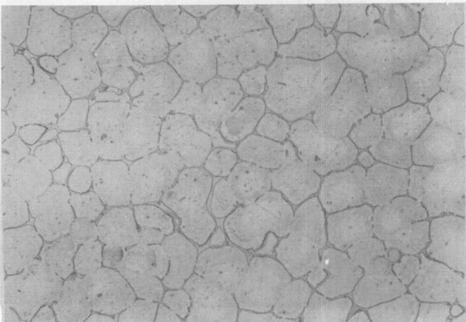
Neg. No. 33204 200X Alloy No. 73454 Etchant: Glycol AC
