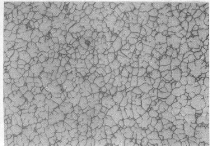
Neg. No. 33917 500X Alloy No. 73454 Etchant: Glycol
