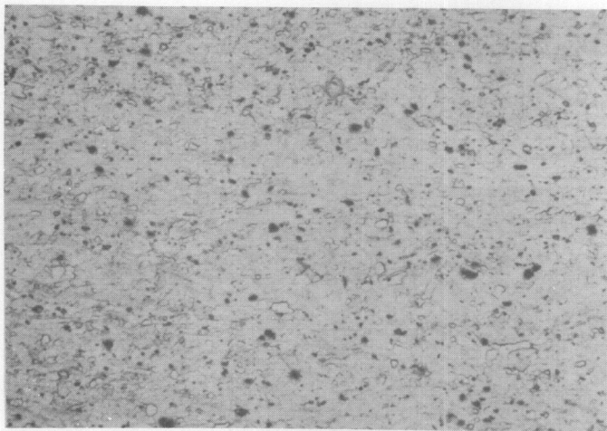
Neg. No. 33225 Alloy No. 73586 Etchant: Acetic Picral Ingot
