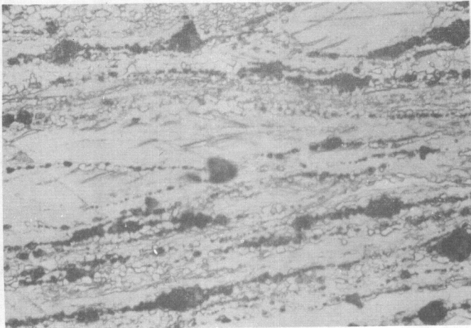
Neg. No. 33216 500X Alloy No. 73445 Etchant: Acetic Picral Ingot
