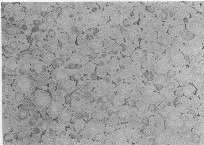
Neg. No. 33212 200X Alloy No. 73458 Etchant: Glycol AC
