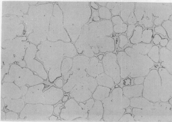
Neg. No. 33173 200X Alloy No. 73446 Etchant: Glycol AC
