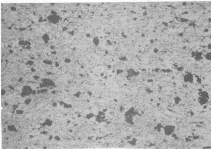
Neg. No. 33223 500X Alloy No. 73445 Etchant: Acetic Picral Ingot
