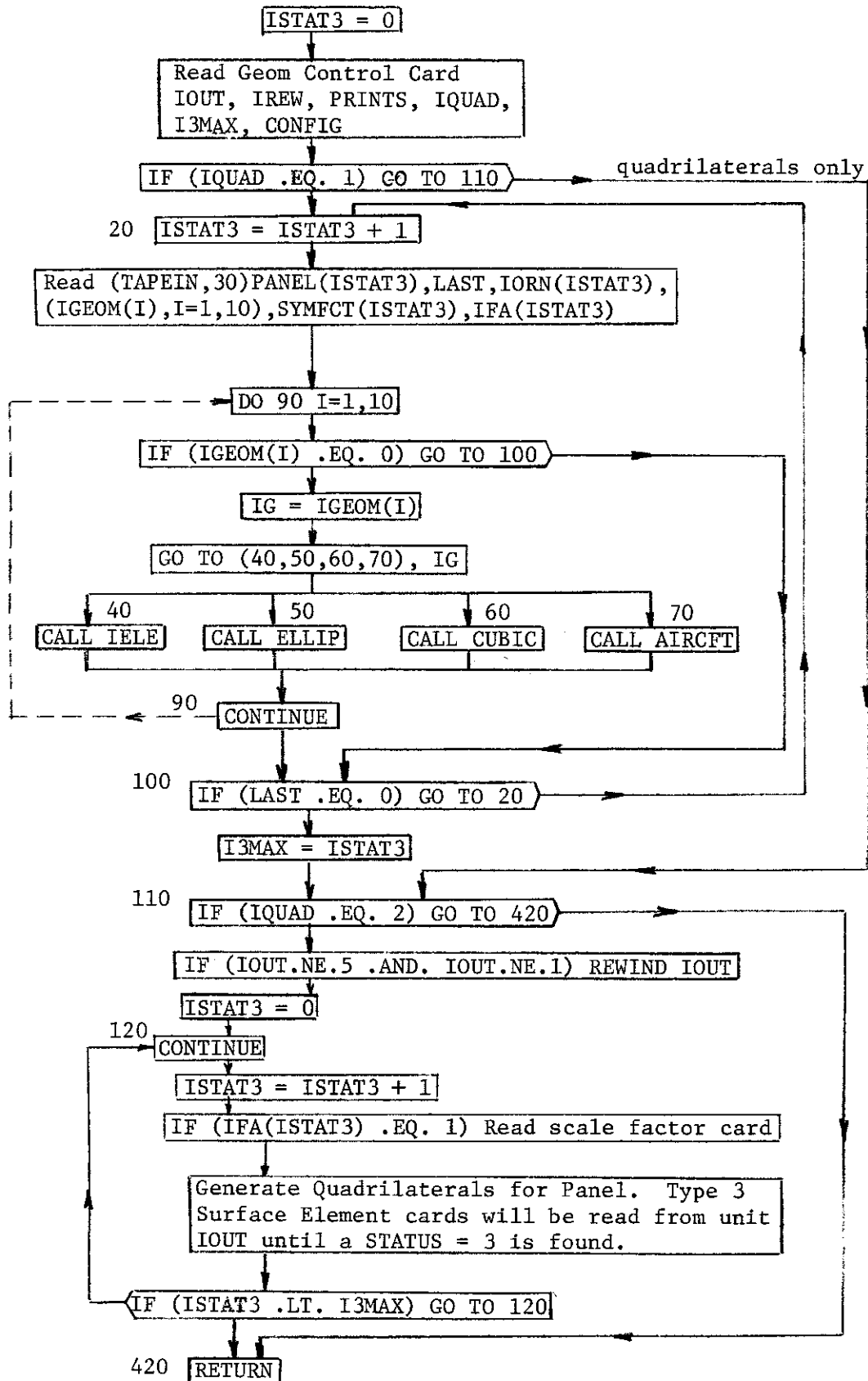
Figure 3. Geometry Input and Usage Flow Chart.
