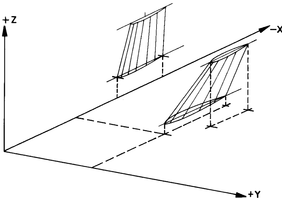
Figure 12. Fin Geometry Generation.
