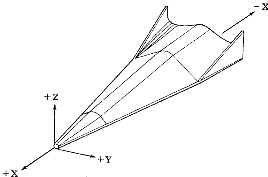
Figure 4. Input Geometry Coordinate System.
