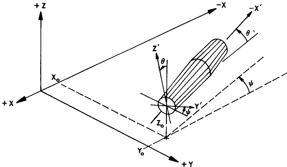
Figure 11. Pod or Nacelle Geometry.
