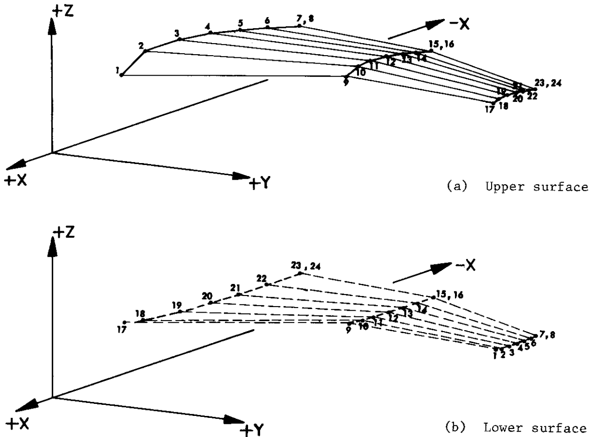
Figure 9. Points and Elements Generated for Wing Surface.
