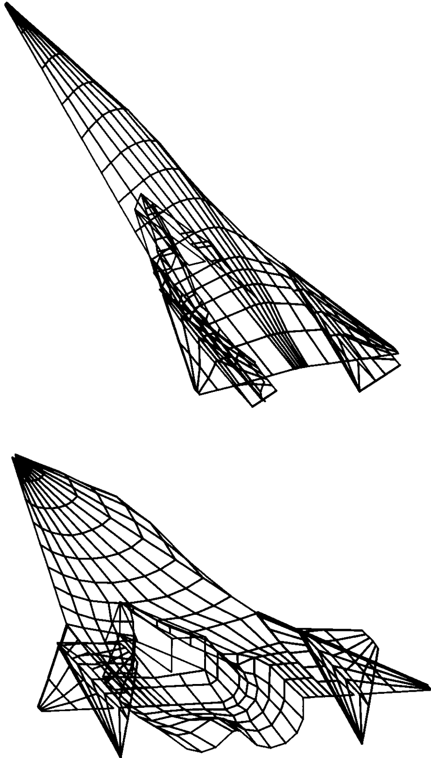
Figure B-4 (cont.) Geometry Checkout Using Off-Line SD-4060 Program.
