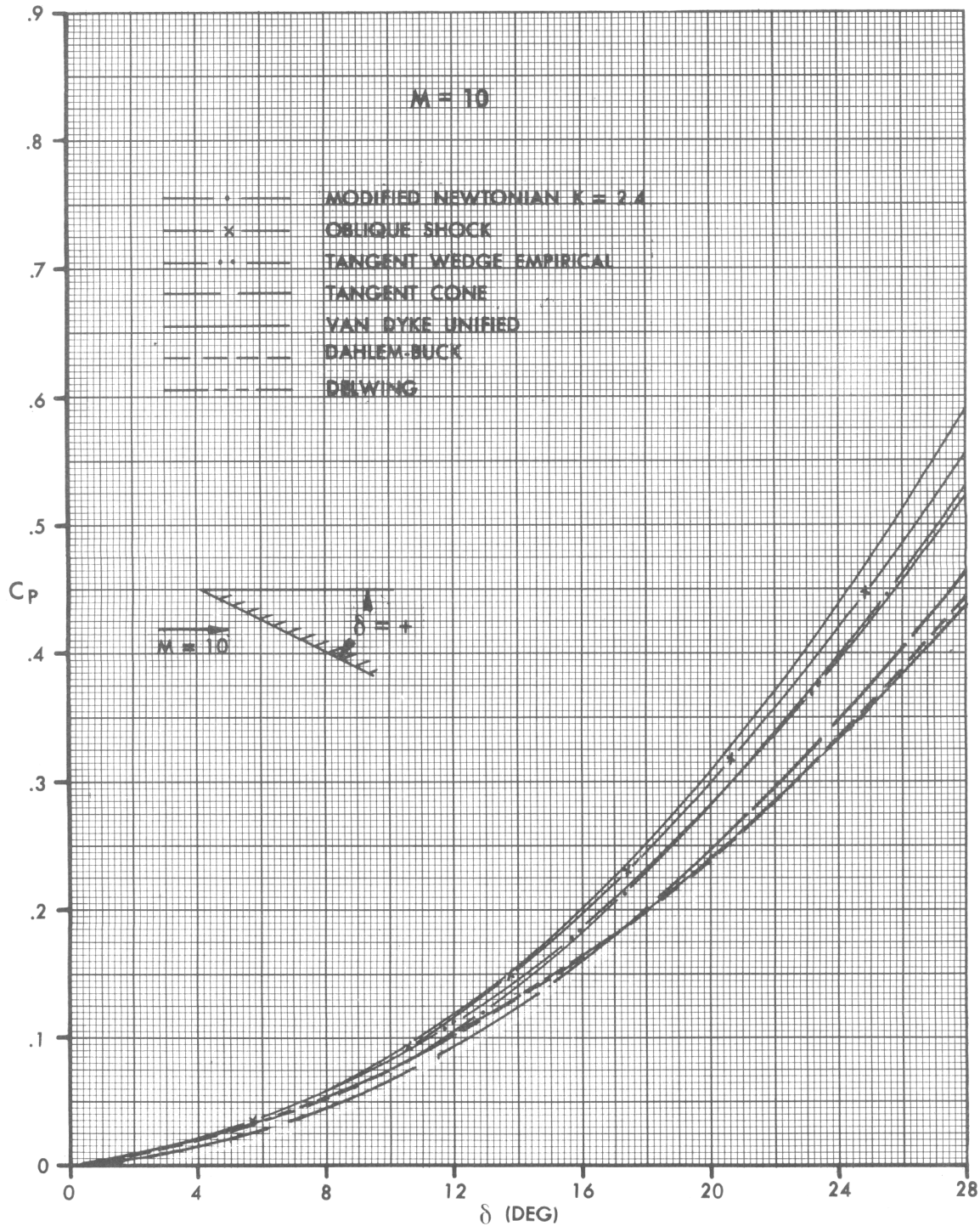
Figure A-5. Comparison of Pressure Prediction Methods for Sharp Bodies in Compression Type Flow
