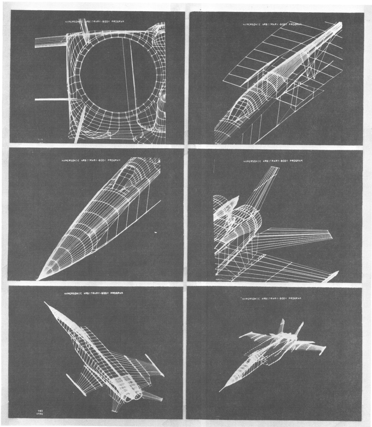
Figure B-2. Geometry Checkout With IBM 2250.
