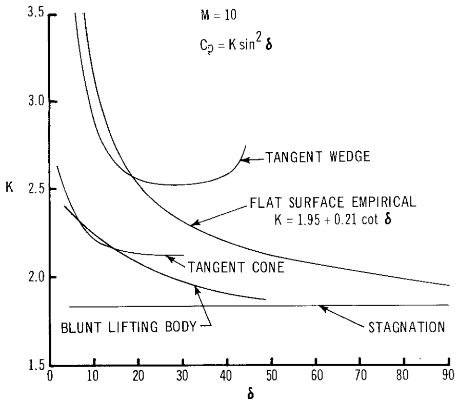
Figure A-17. Modified Newtonian Correlation Factors
