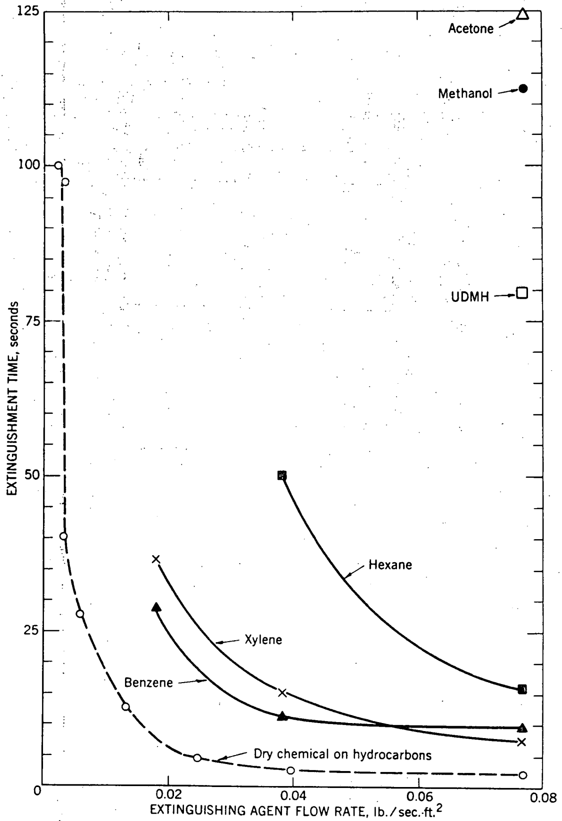
FIGURE 46. Minimum application rates of foam and of dry chemical for extinguishment of hydrocarbon and nonhydrocarbon fuel fires.
