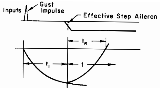
Sketch 4. Recovery from a Gust Upset
