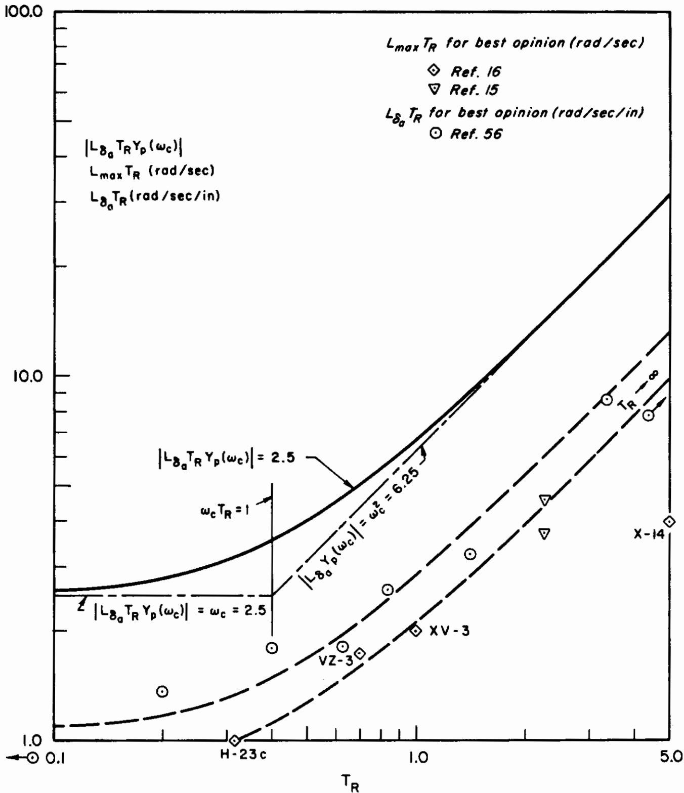
Figure 17. Gain at Crossover Frequency, \omega_c = 2.5 Rad/Sec
