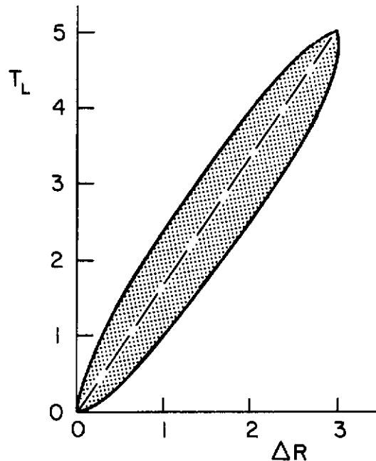
Sketch 1. Approximate Variation of Incremental Rating with T_L
