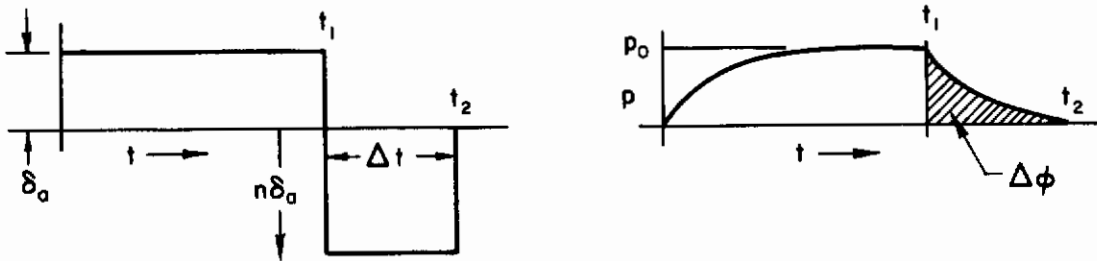
Sketch 5. Quick-Stop Maneuver
