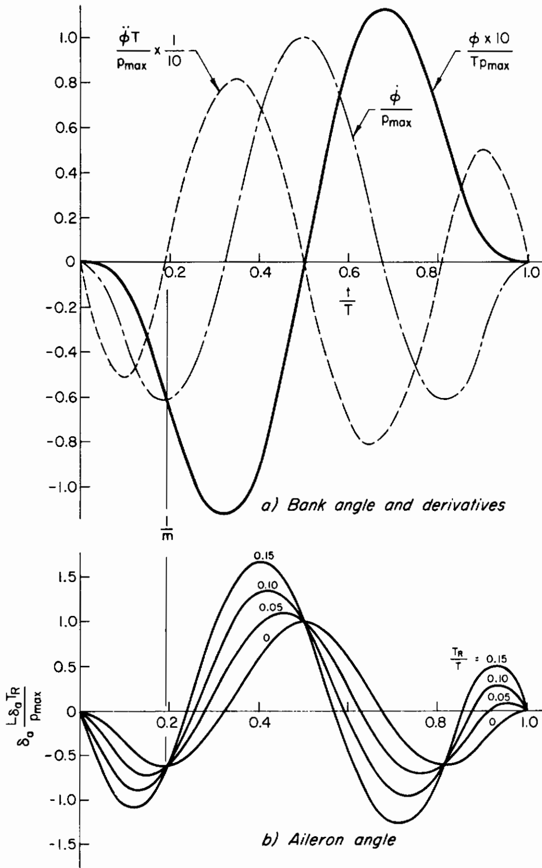
Figure 7. Bank Angle and Aileron Time Histories for Sidestep
