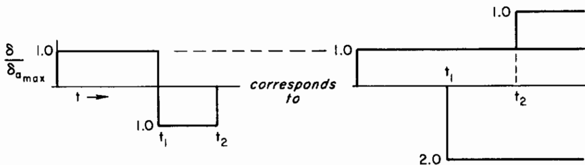
Sketch 3. Maximum-Performance Bank and Stop Aileron Inputs
