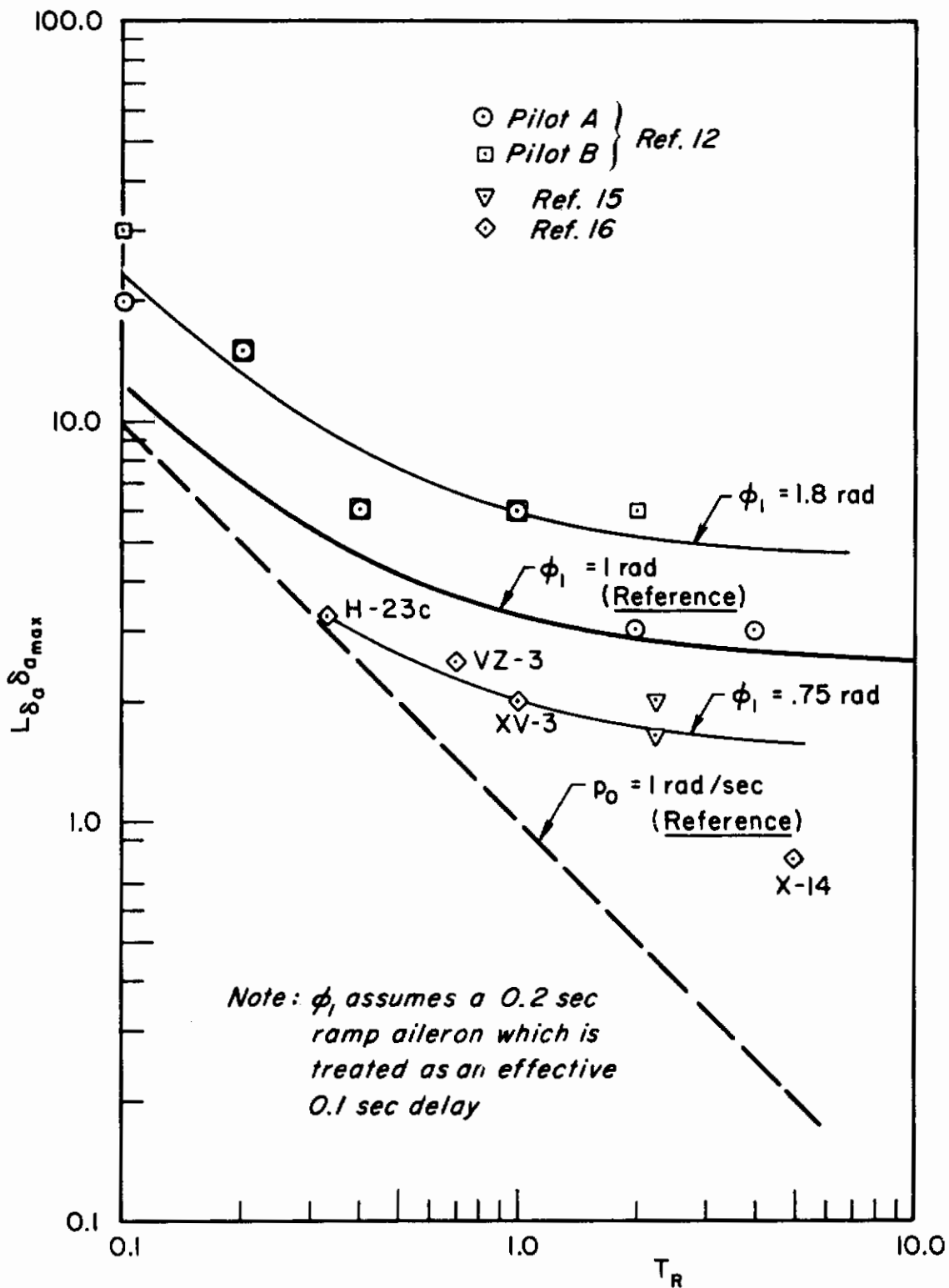
Figure 15. Roll Power—Best Opinion Correlations
