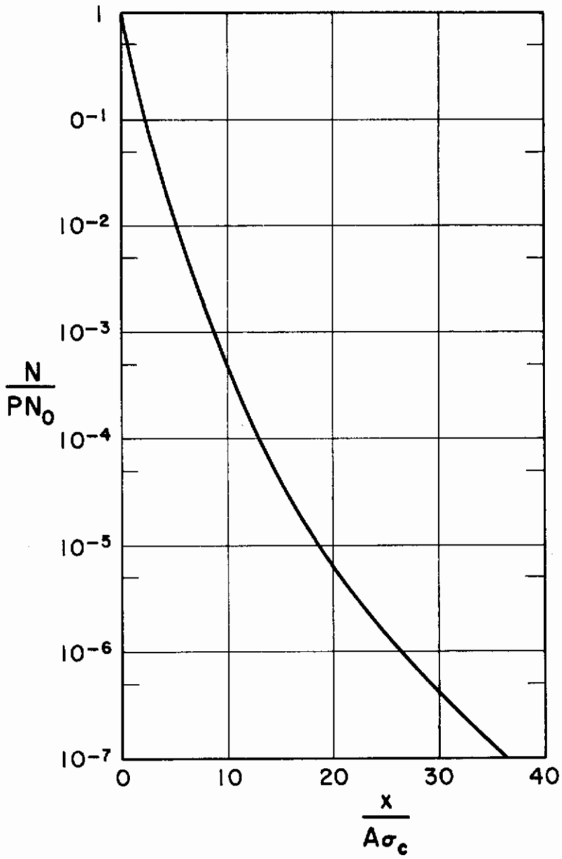
Figure 1. "Universal" Curve for Load Exceedance.
