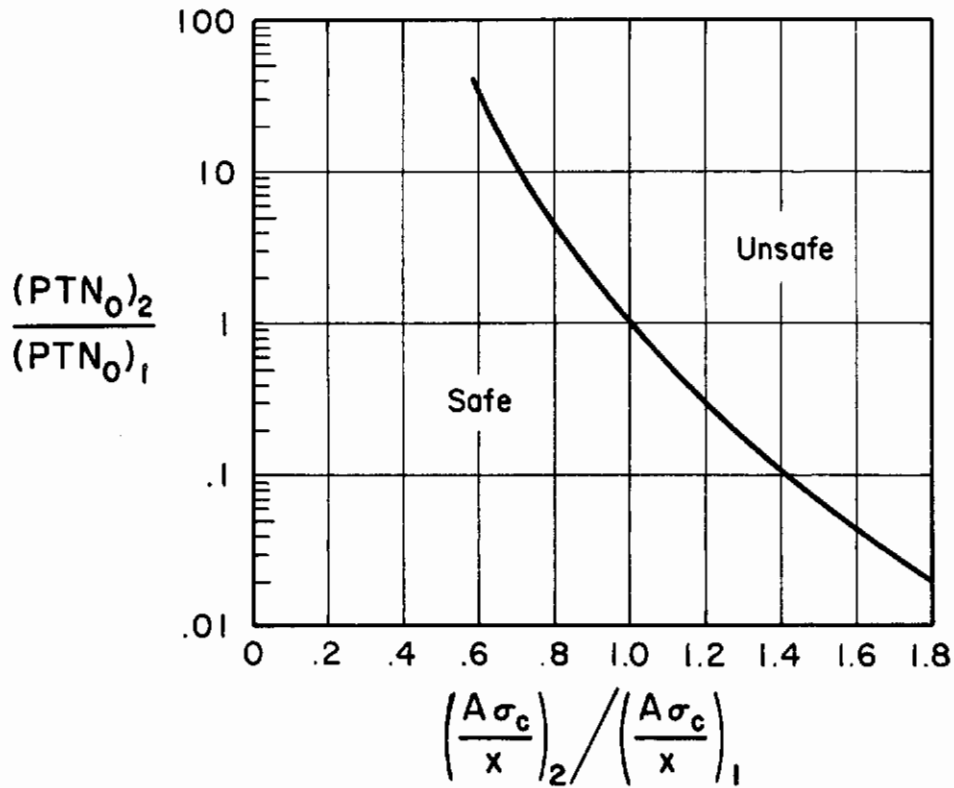
Figure 5. Gust Design by Comparison (Note, stresswise, adding metal lowers A).
