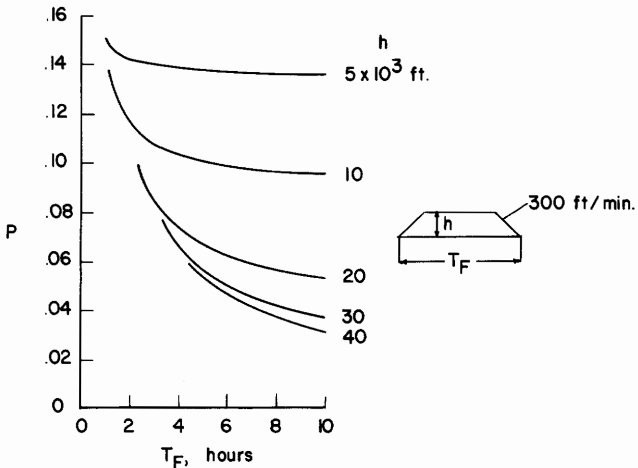
Figure 3. Proportion of Time in Turbulence for a Given Mission.
