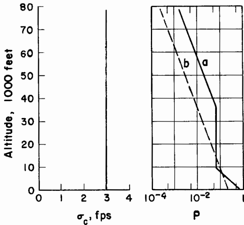
Figure 2. Tentative \sigma_c and P Values.
