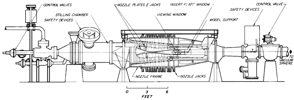
Assembly
