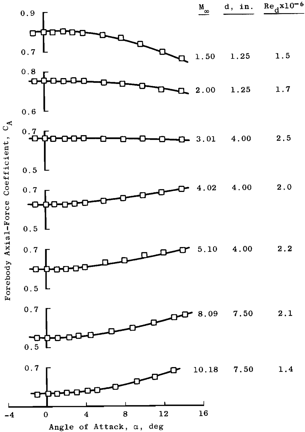
b. Configuration HB-2
