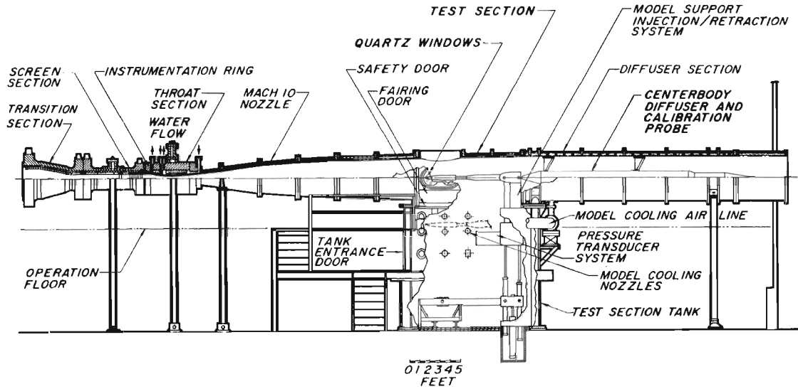
Tunnel Assembly
