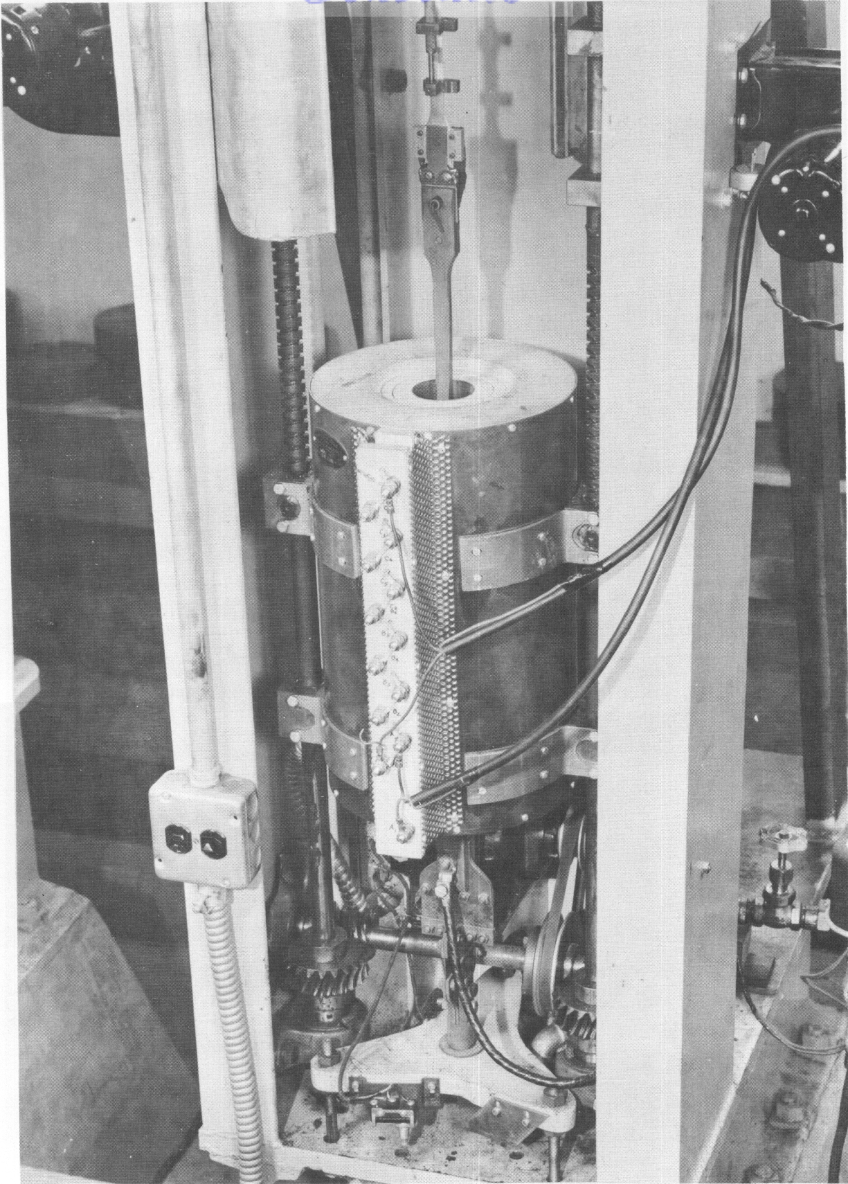
Figure 4. LOWER SPECIMEN MOUNTING AND SPIDER
