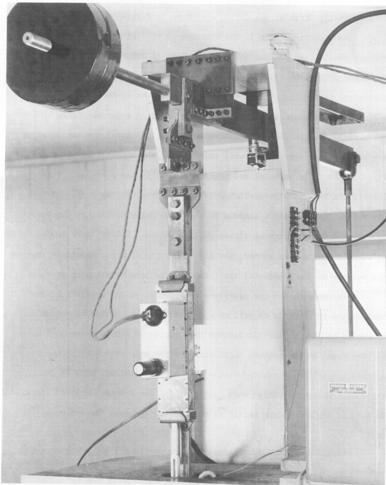
Figure 2. FULCRUM AND ALIGNMENT FLEXURE PLATES AND STRAIN GAGE
