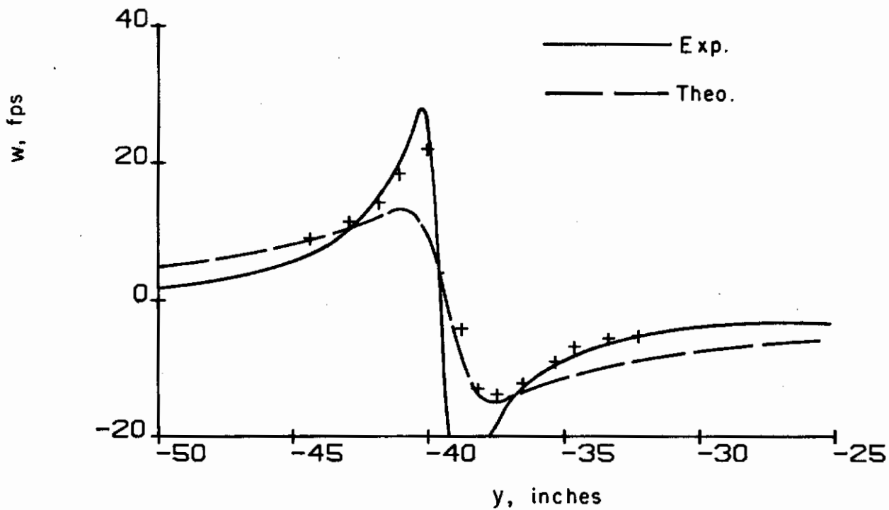
Figure 44. Configuration 1; comparison of measured and computed horizontal and vertical velocities ( x = 100 in., z = 69.1 in.)
