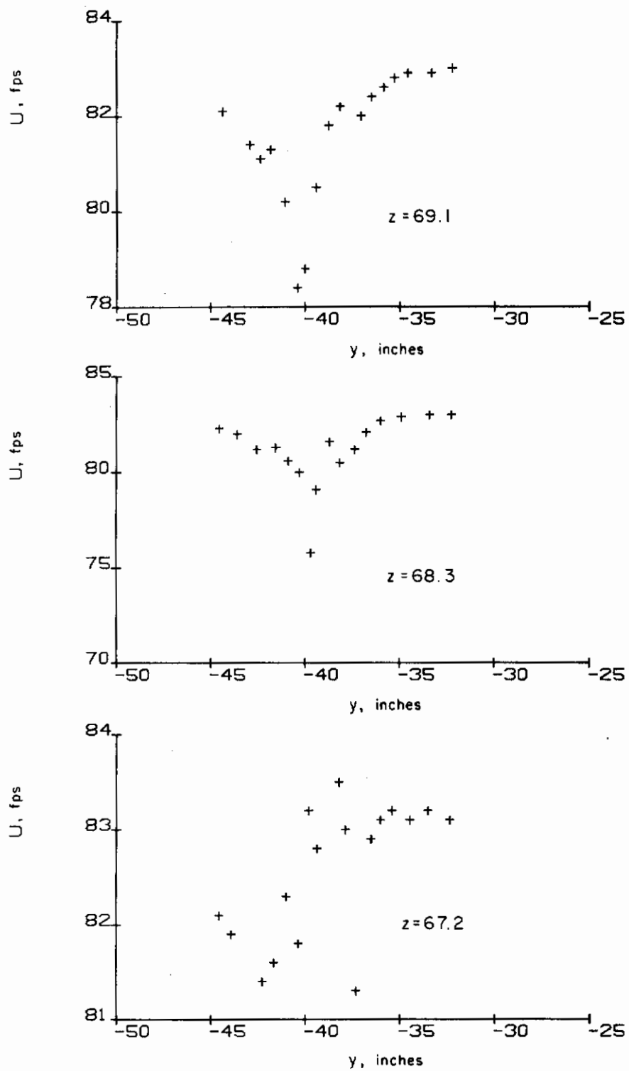
Figure 45. Configuration 1; measured axial velocities ( x = 100 in.)
