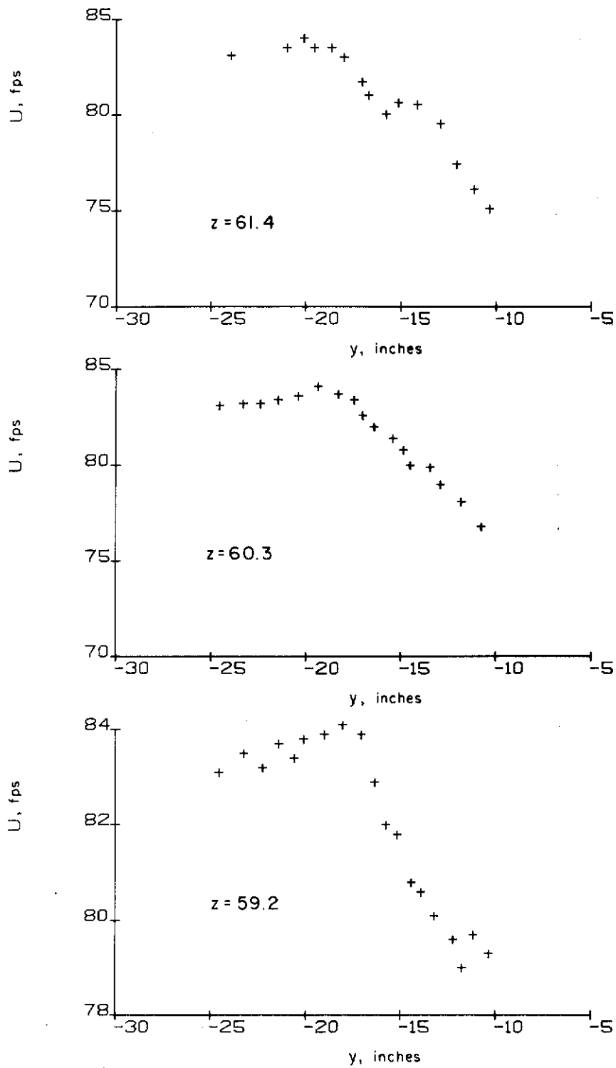
Figure 53. Configuration 2; measured axial velocities ( x = 50 in.)
