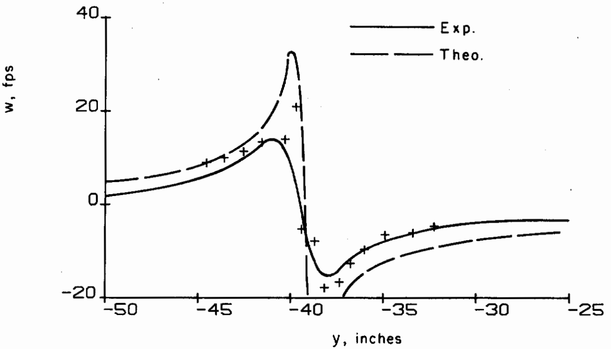
Figure 43. Configuration 1; comparison of measured and computed horizontal and vertical velocities ( x = 100 in., z = 68.3 in.)
