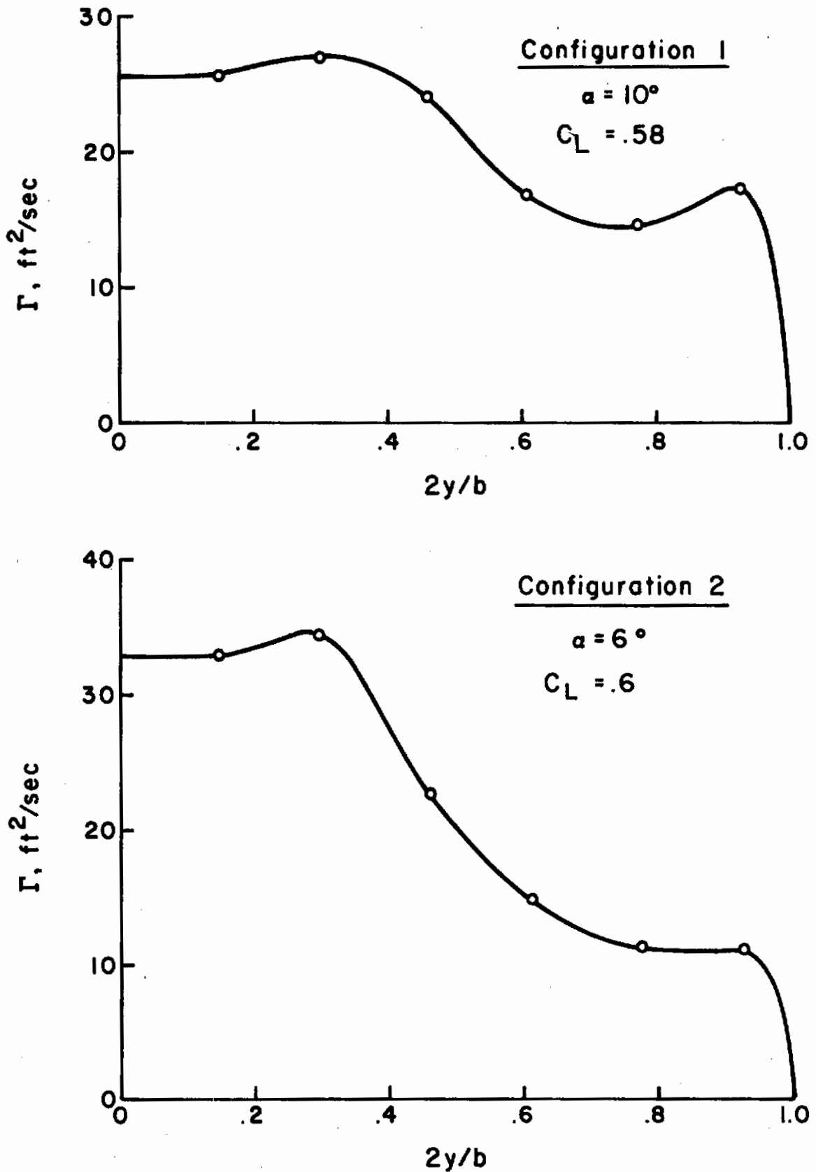
Figure 24. Lift distributions from wing surface pressure measurements
