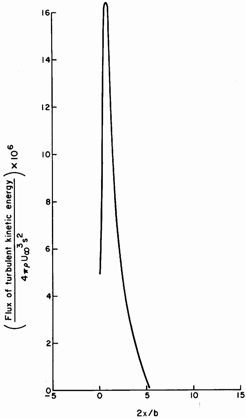
Figure 71. Computed flux of turbulent kinetic energy
