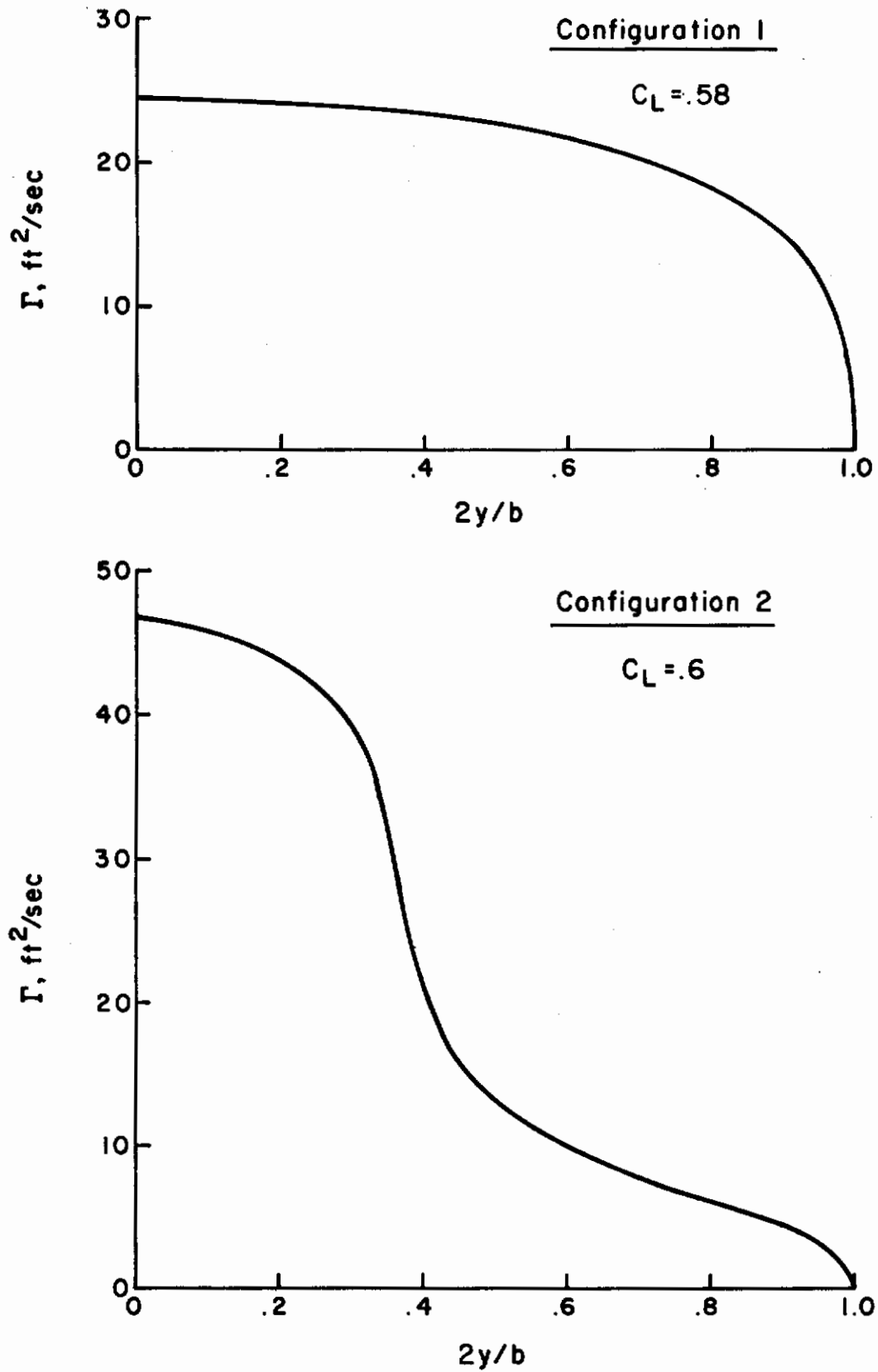
Figure 25. Lift distributions from lifting surface theory
