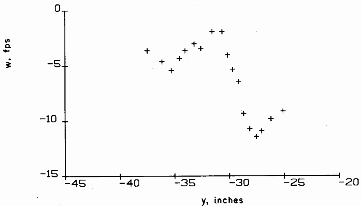
Figure B-2c. Configuration 3; flap vortex. Measured horizontal and vertical velocities ( x = 50 in., z = 68.4 in.)
