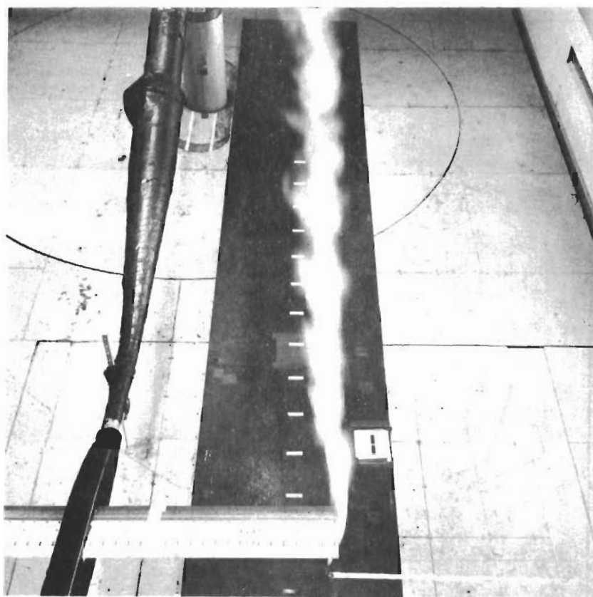
Figure 26. Smoke visualization; configuration 1; overhead view
