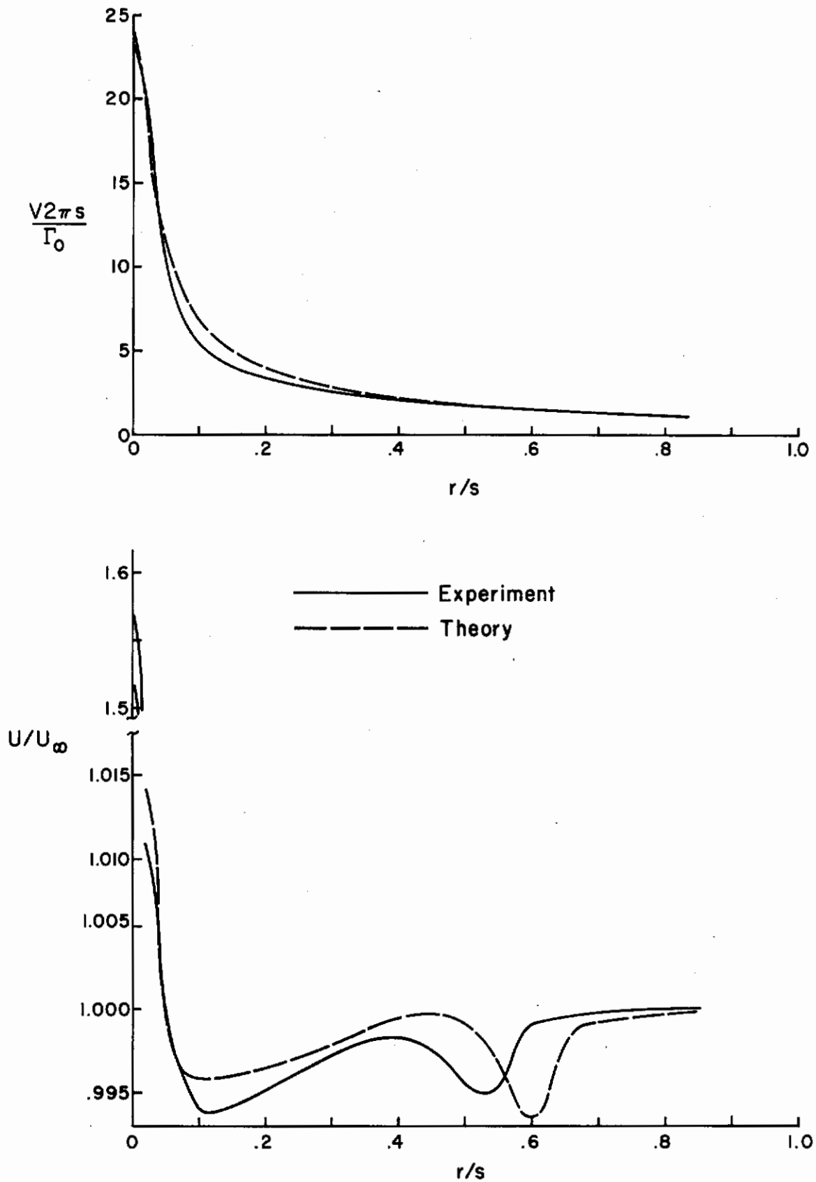
Figure 65. The downstream structure of the tip vortex for configuration 1
