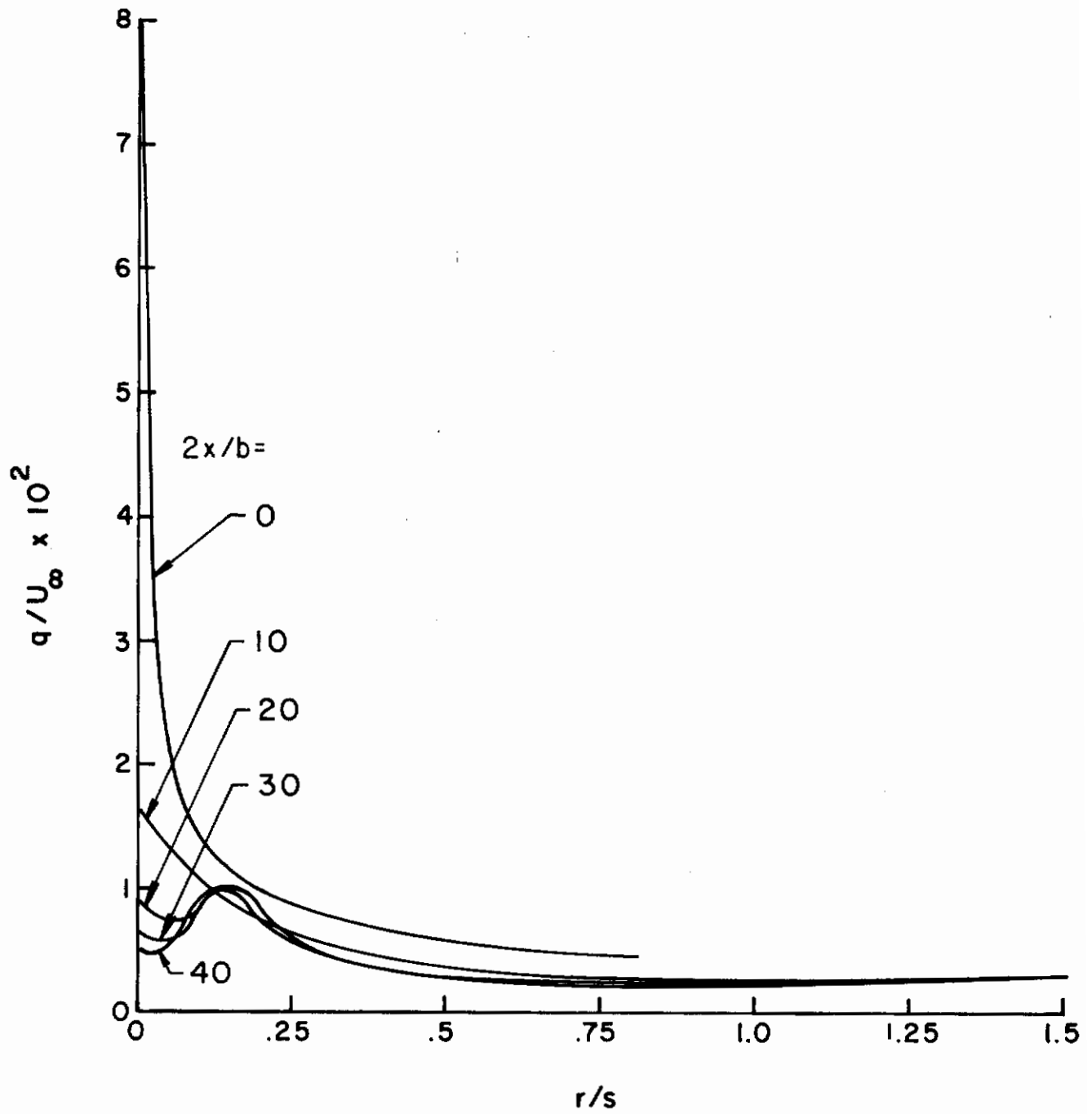
Figure 69. Computed distribution of q' = \sqrt{u'^2 + v'^2 + w'^2}
