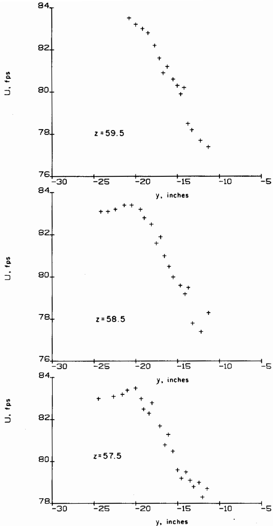
Figure 61. Configuration 2; measured axial velocities (x = 100 in.)
