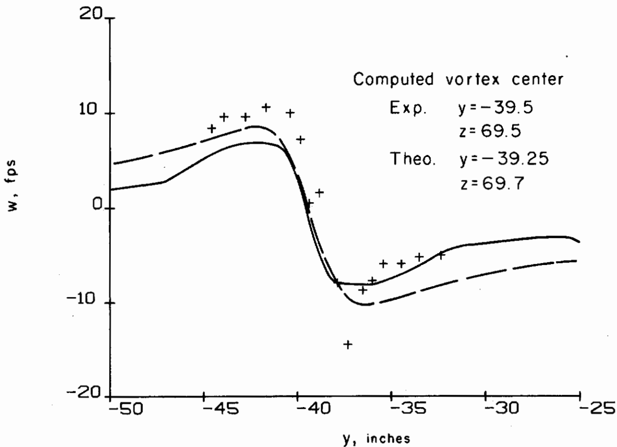
Figure 42. Configuration 1; comparison of measured and computed horizontal and vertical velocities ( x = 100 in., z = 67.2 in.)
