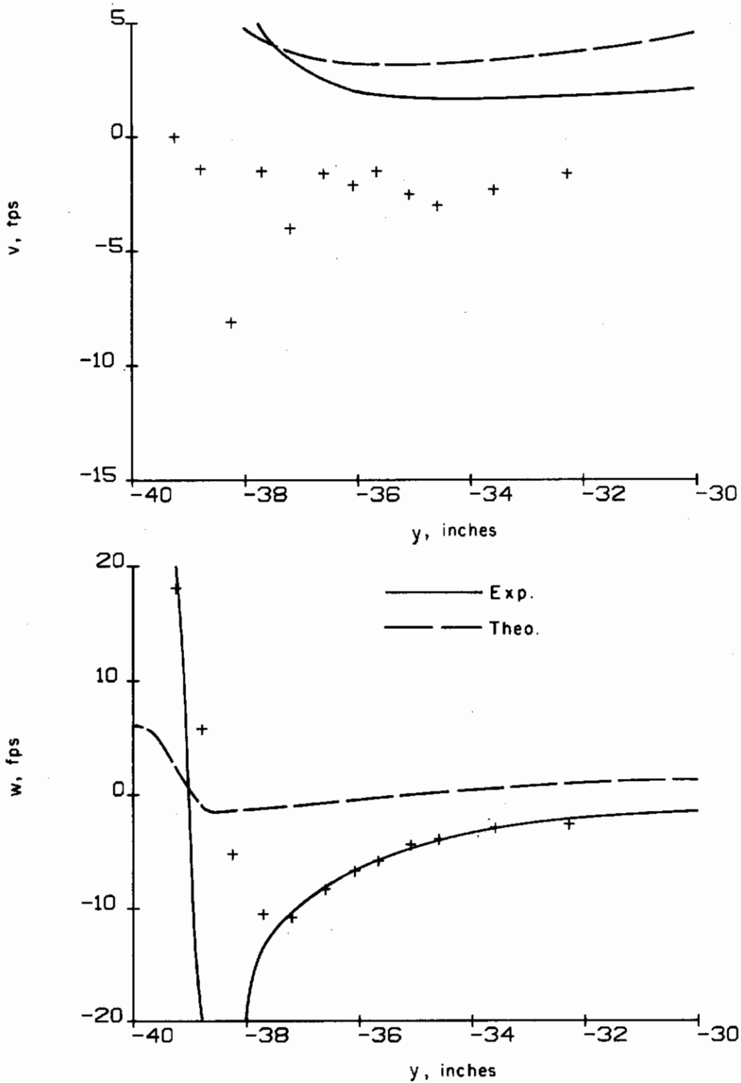
Figure 56. Configuration 2; tip vortex. Comparison of measured and computed horizontal and vertical velocities ( x = 100 in., z = 72.5 in.)
