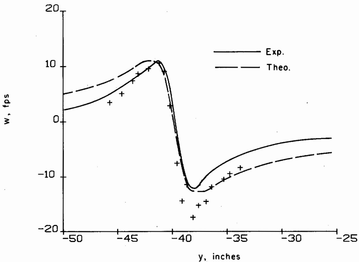
Figure 38. Configuration 1; comparison of measured and computed horizontal and vertical velocities ( x = 50 in., z = 67.95 in.)
