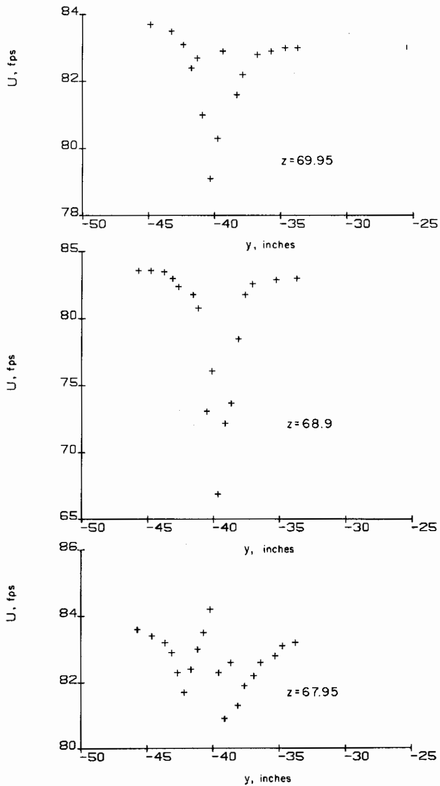
Figure 41. Configuration 1; measured axial velocities (x = 50 in.)
