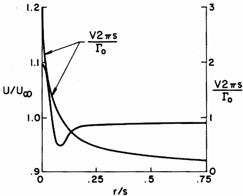
Figure 7. Examples of drag distributions which result in regions of axial velocity excess and defect in the vortex
