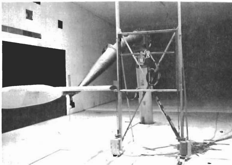
Figure 23. The wake traversing mechanism mounted with the hot-film probe 5 chords downstream of the trailing edge
