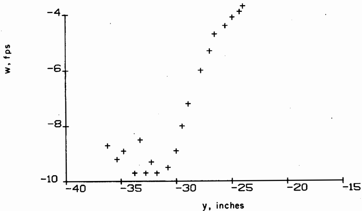
Figure B-4a. Configuration 4; flap vortex. Measured horizontal and vertical velocities ( x = 50 in., z = 48.8 in.)
