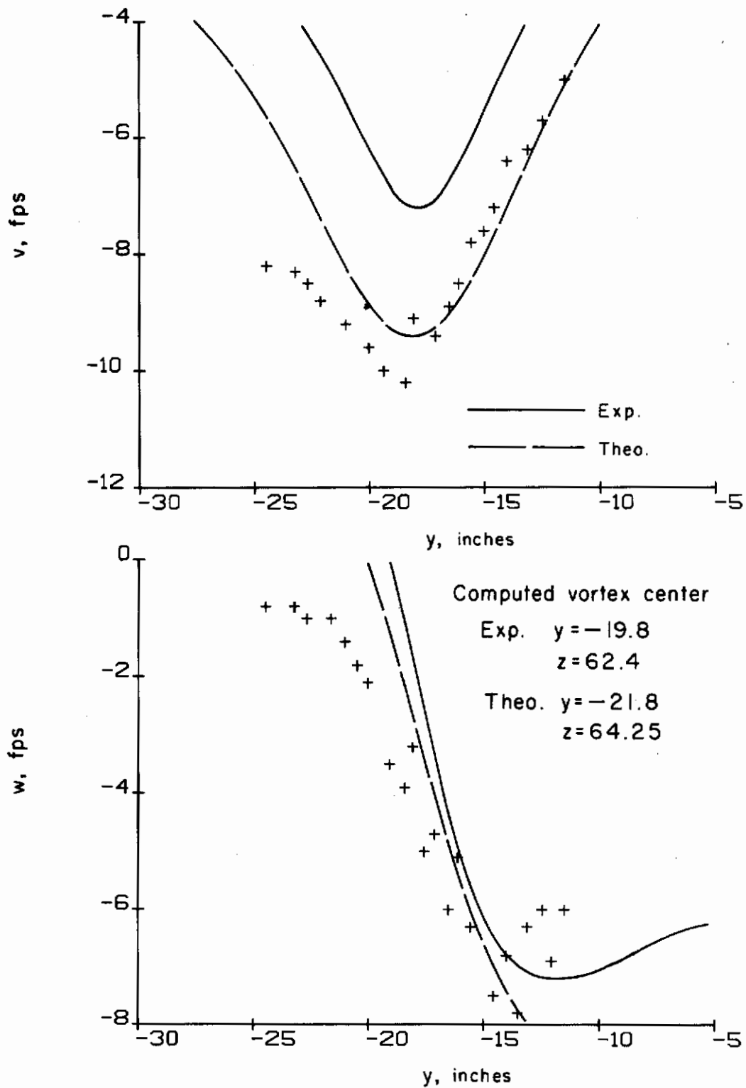
Figure 58. Configuration 2; flap vortex. Comparison of measured and computed horizontal and vertical velocities ( x = 100 in., z = 57.5 in.)
