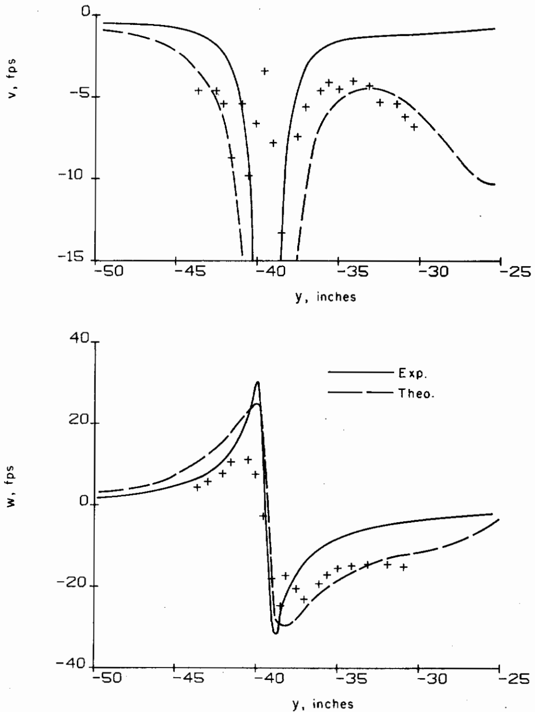
Figure B-3b. Configuration 4; tip vortex. Comparison of measured and computed horizontal and vertical velocities ( x = 50 in., z = 55.4 in.)
