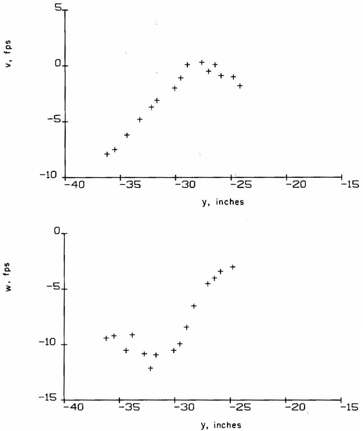
Figure B-4b. Configuration 4; flap vortex. Measured horizontal and vertical velocities ( x = 50 in., z = 49.9 in.)
