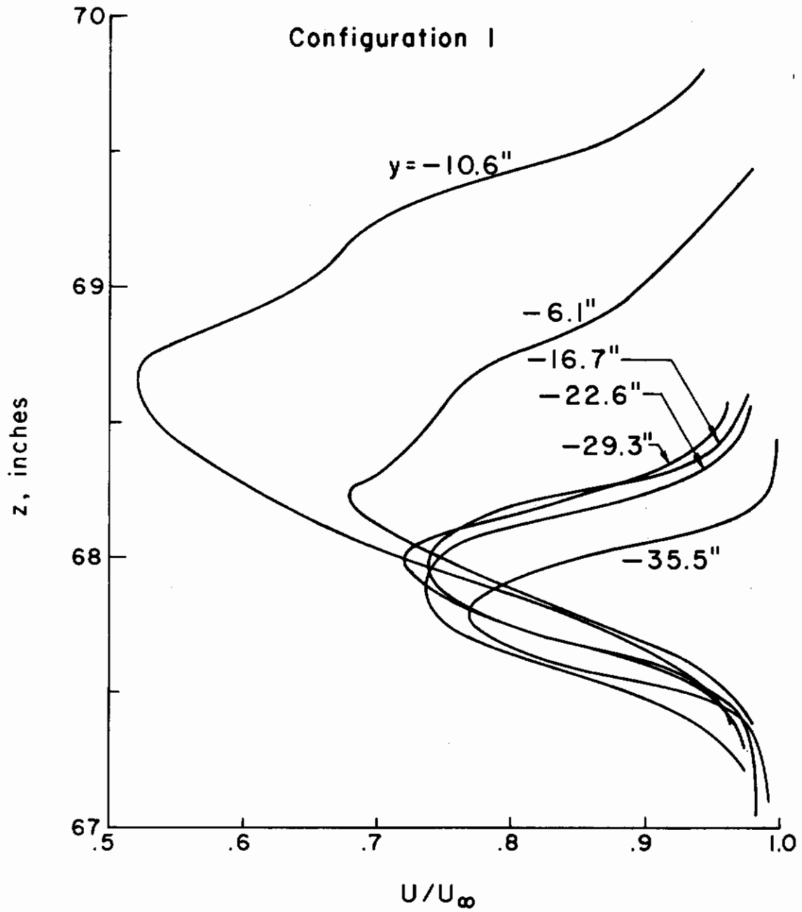
Figure 35. Paired measured axial velocity defect; z = 3 in.
