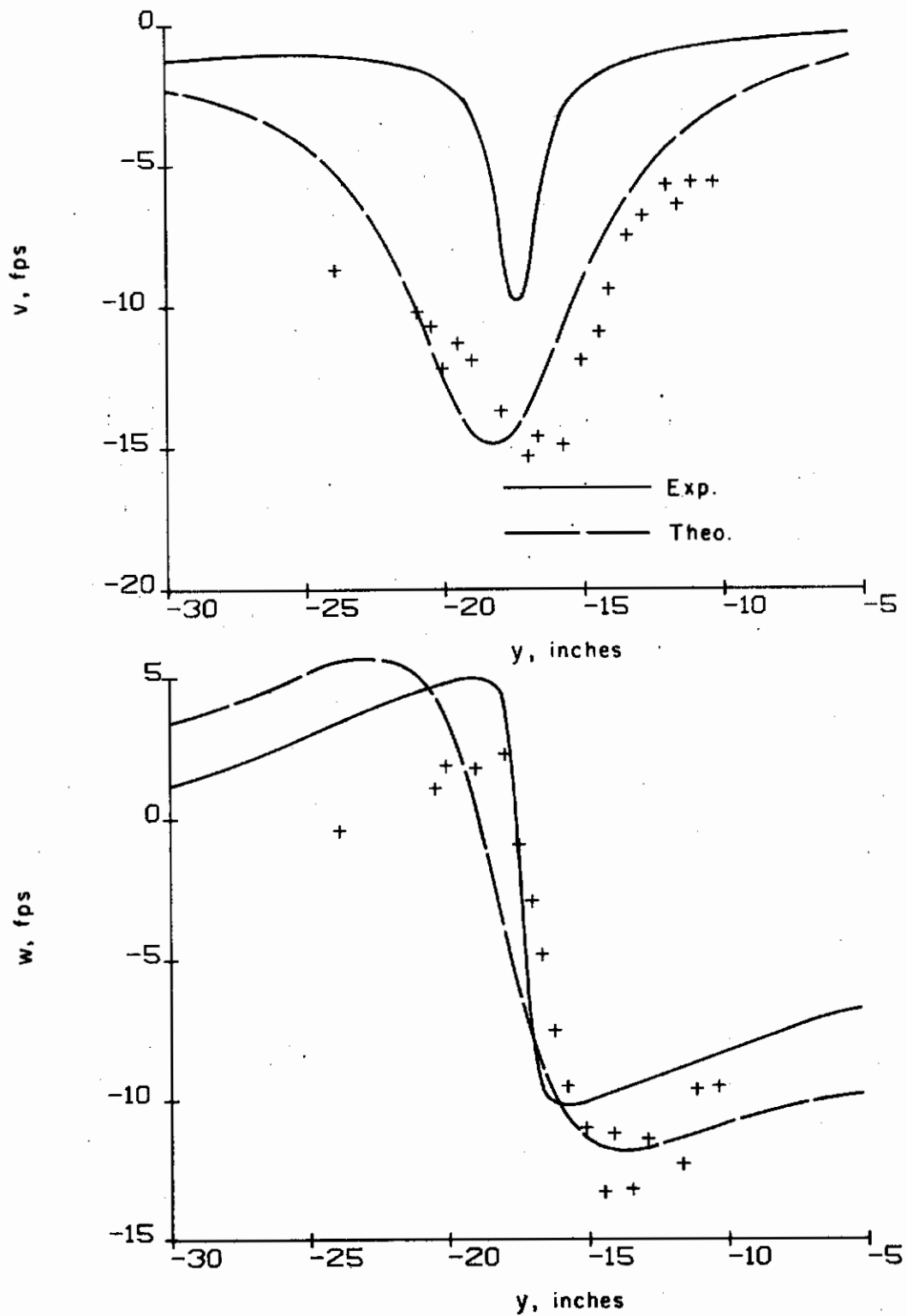
Figure 52. Configuration 2; flap vortex. Comparison of measured and computed horizontal and vertical velocities ( x = 50 in., 61.4 in.)
