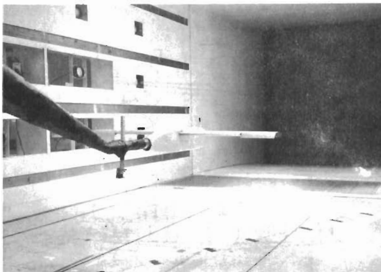
Figure 22. Model test configuration 4
