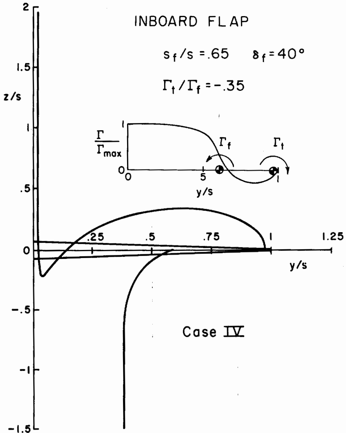
Figure 13. Vortex centroid locations as seen from downstream; pairs of opposite sign. Weak interaction between pairs; pairs diverge.
