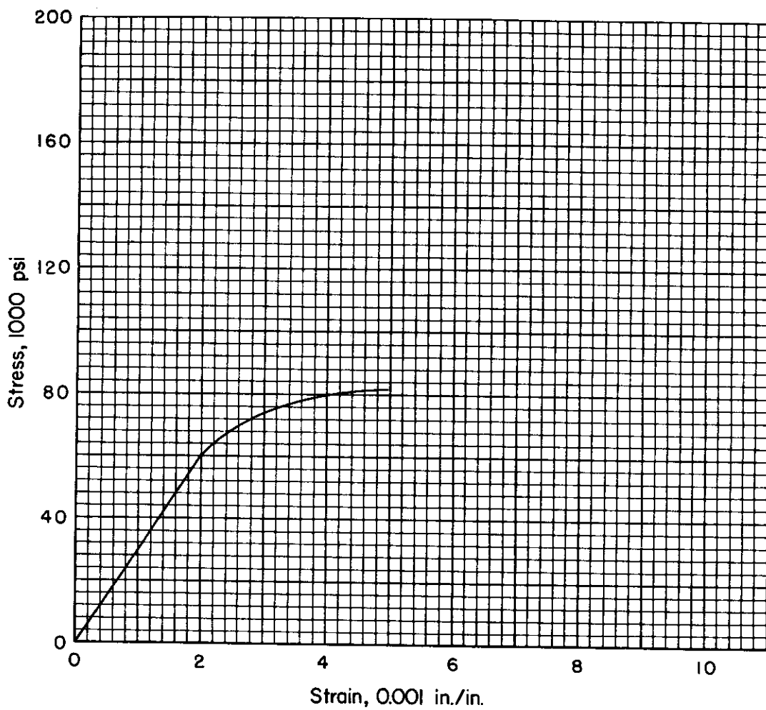
FIGURE 2. STRESS-STRAIN CURVE FOR NORMALIZED AND AGED 2800 STEEL AT ROOM TEMPERATURE
