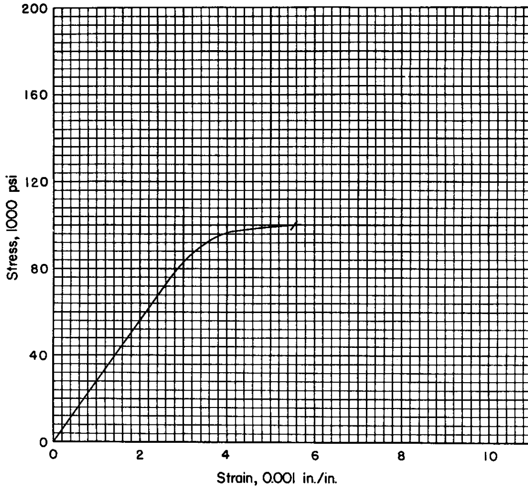
FIGURE 11. STRESS-STRAIN CURVE FOR ANNEALED AND AGE-HARDENED NI-SPAN C IRON-NICKEL ALLOY AT ROOM TEMPERATURE
