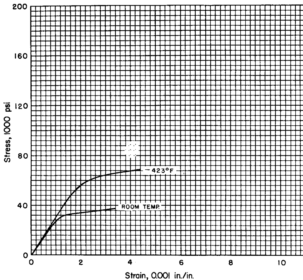
FIGURE 3. STRESS-STRAIN CURVES FOR ANNEALED 304 STAINLESS STEEL AT ROOM TEMPERATURE AND -423 F
