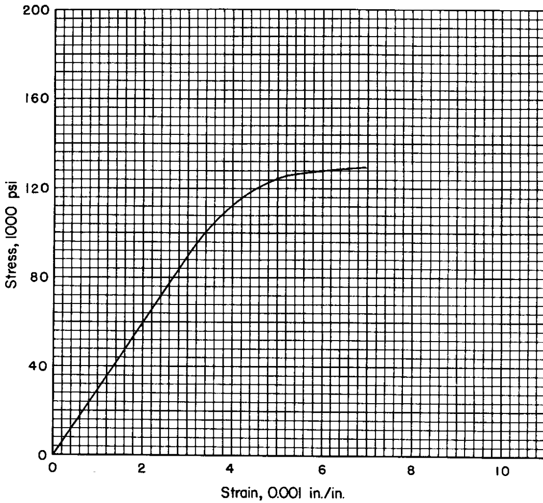
FIGURE 7. STRESS-STRAIN CURVE FOR COLD-ROLLED INCONEL NICKEL ALLOY AT ROOM TEMPERATURE
